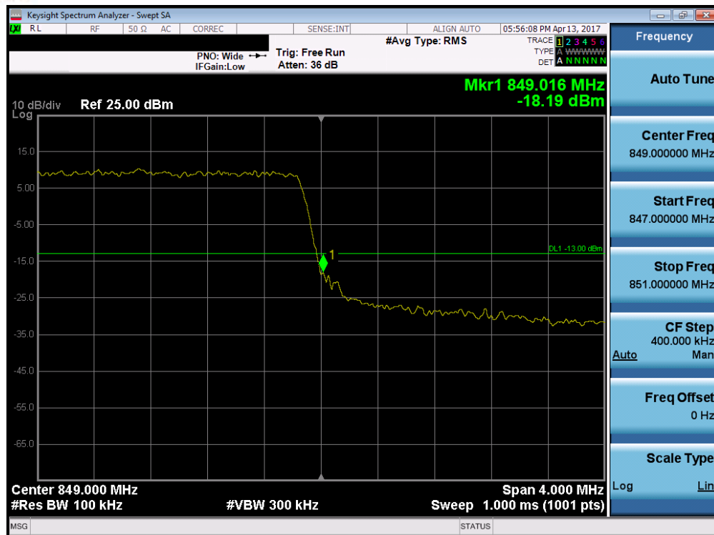
Plot 7-107. Upper Band Edge Plot (Band 5 - 3.0MHz QPSK - RB Size 15)
