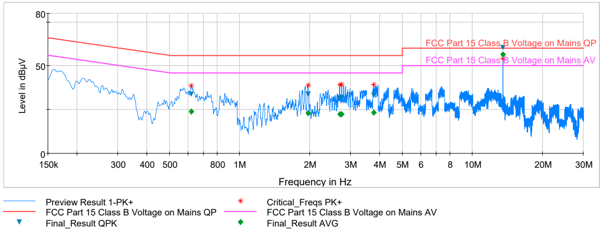
Plot 7-1. Line-Conducted Test Plot with Antenna Connected (L1)
