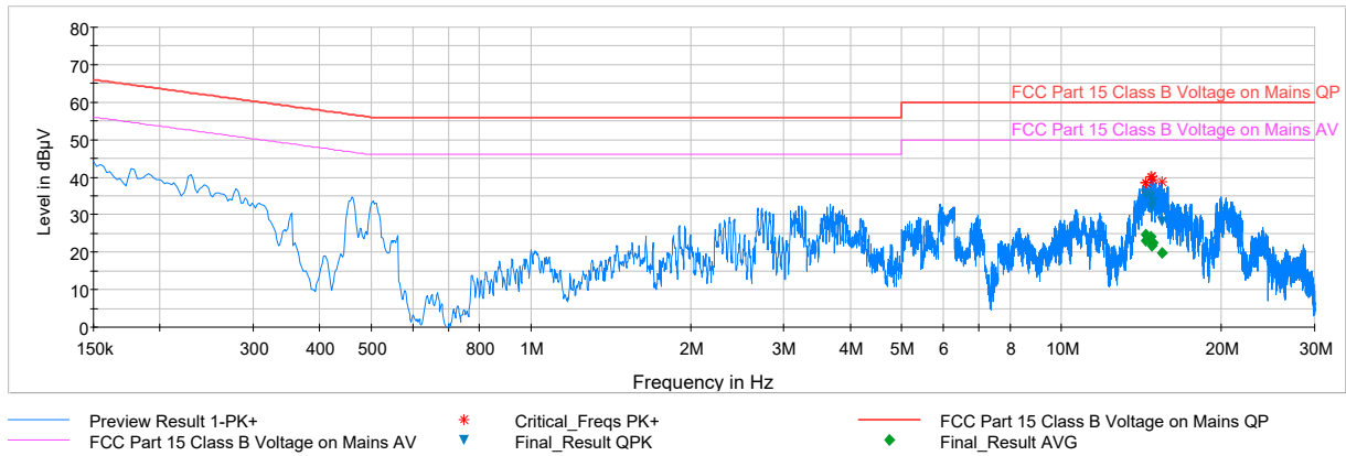
Plot 7-4. Line-Conducted Test Plot with Antenna Terminated in 50Ω (N)
