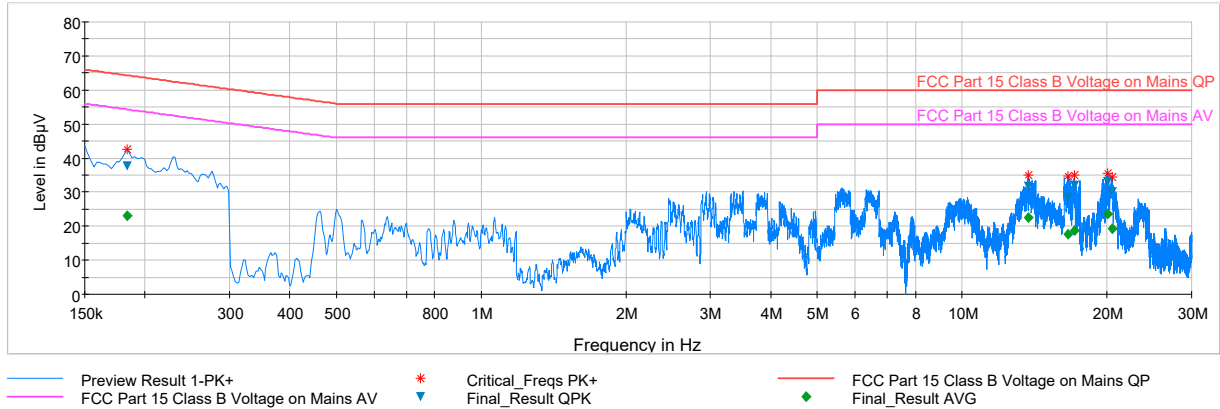
Plot 7-3. Line-Conducted Test Plot with Antenna Terminated in 50Ω (L1)
