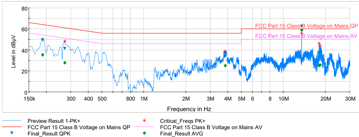
Plot 7-2. Line-Conducted Test Plot with Antenna Connected (N)
