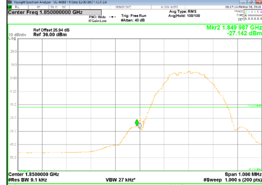
GSM1900 EGPRS Low channel
