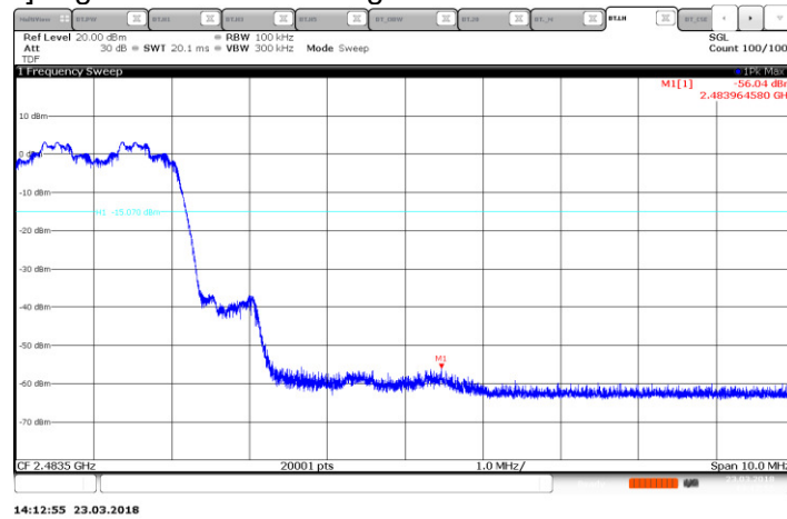
[8PSK Hopping Mode] High Channel BandEdge
