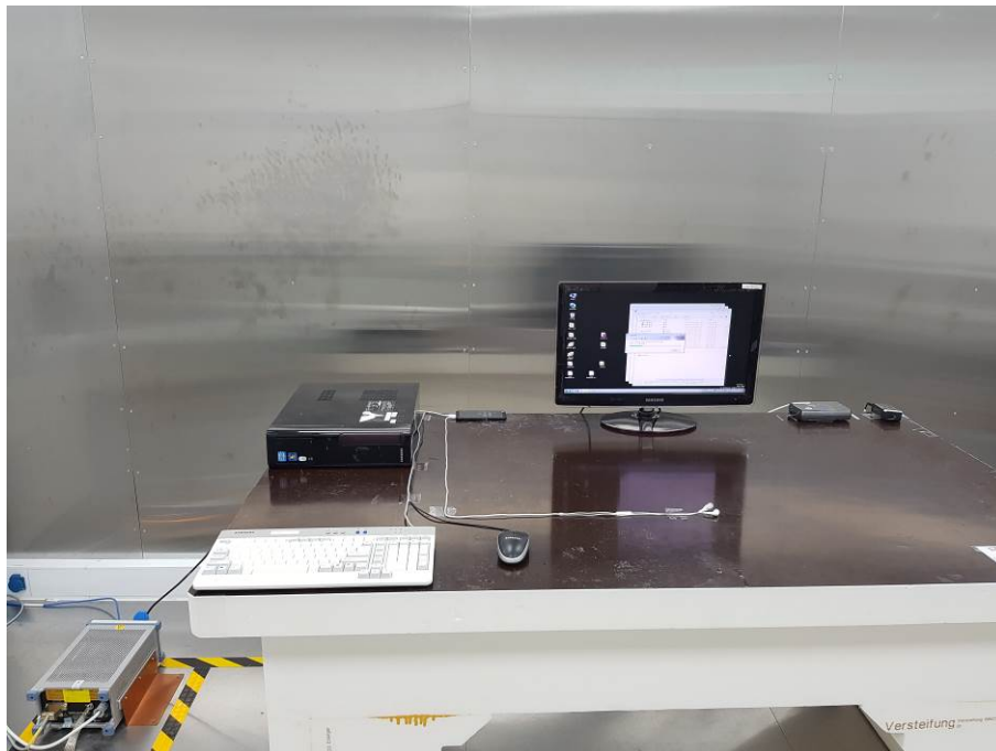
[ Conducted Disturbance – Front ]
