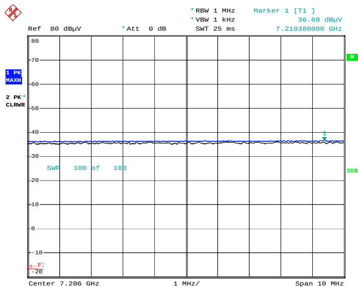
Radiated Spurious Emissions plot – Average Reading (GFSK, Ch.0 3rd Harmonic, Z-H)
