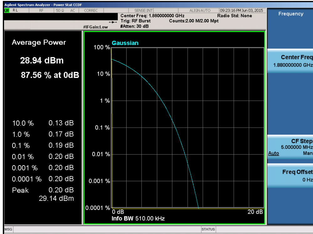
Plot 6-54. Peak-Average Ratio Plot (PCS GSM Mode – Ch. 661)
