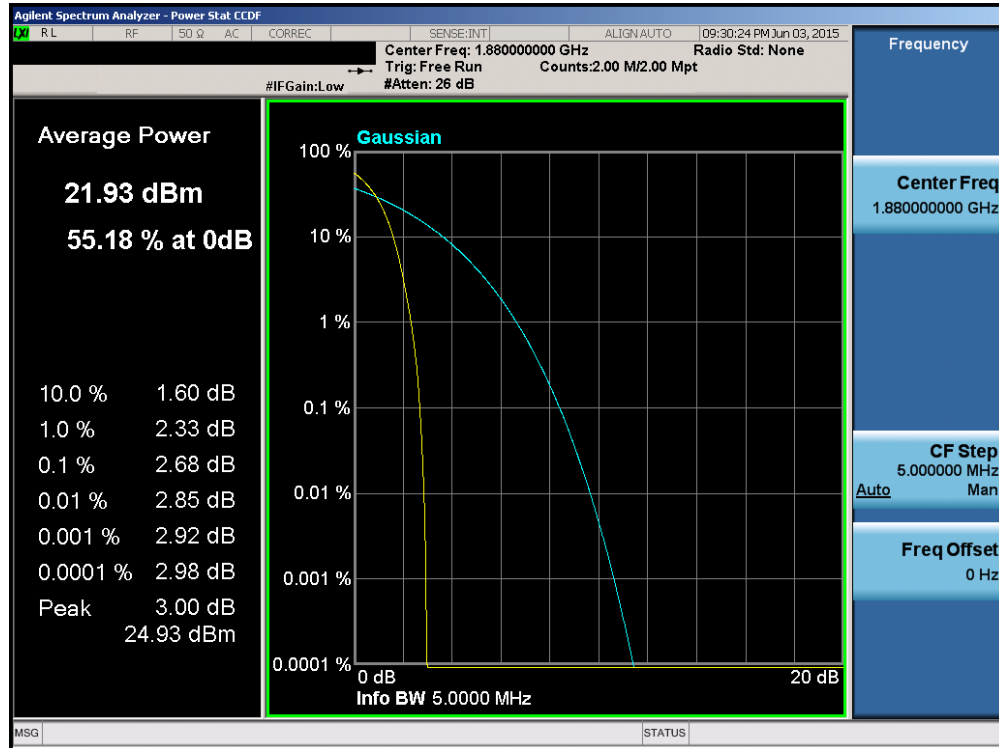
Plot 6-56. Peak-Average Ratio Plot (PCS WCDMA Mode – Ch. 9400)
