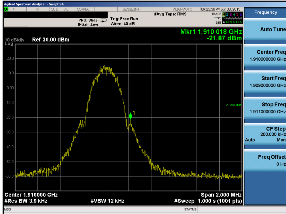
Plot 6-46. Band Edge Plot (PCS GSM Mode – Ch. 810)
