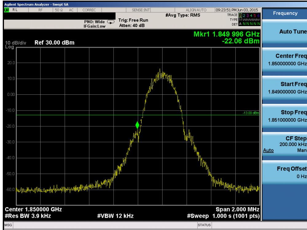
Plot 6-44. Band Edge Plot (PCS GSM Mode – Ch. 512)
