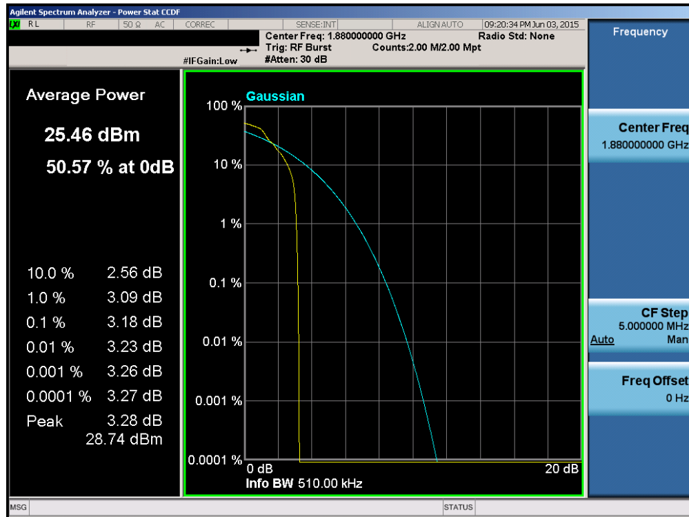
Plot 6-55. Peak-Average Ratio Plot (EDGE1900 Mode – Ch. 661)
