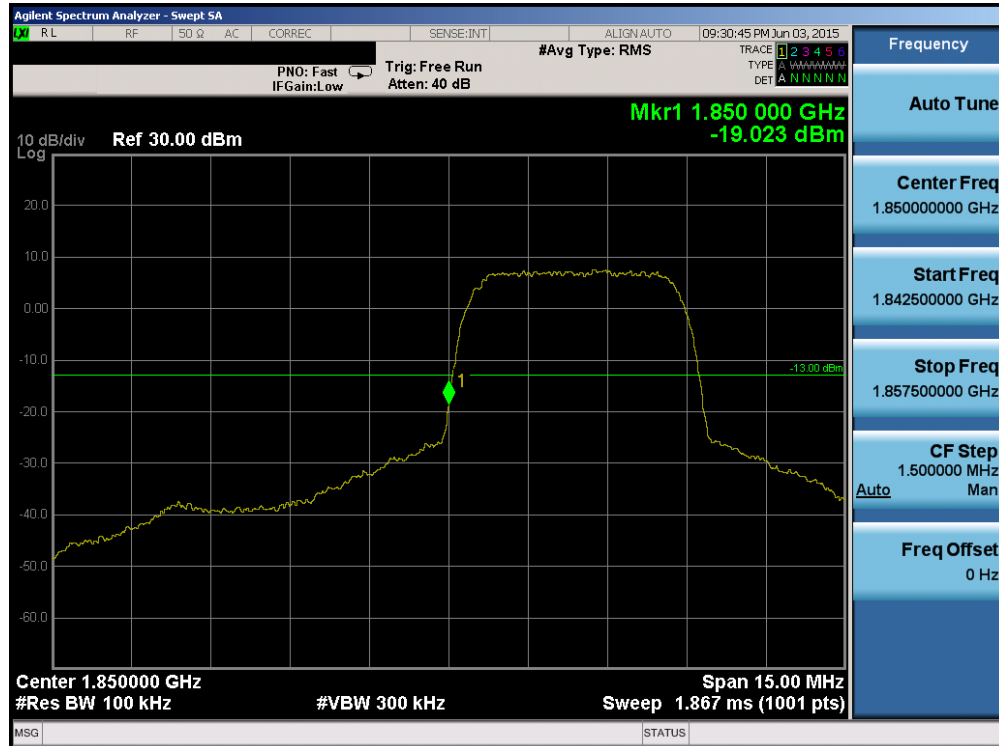
Plot 6-50. Band Edge Plot (PCS WCDMA Mode – Ch. 9262)
