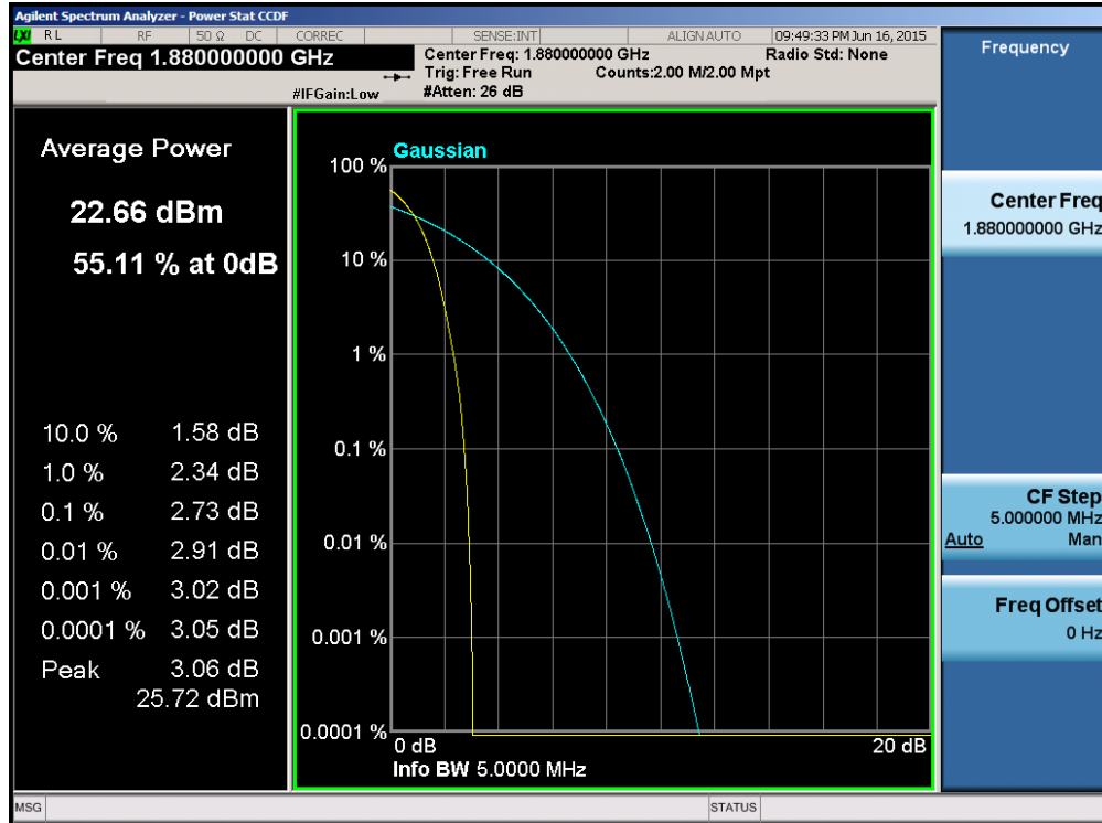
Plot 6-55. Peak-Average Ratio Plot (PCS WCDMA Mode – Ch. 9400)
