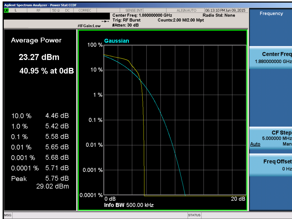
Plot 6-54. Peak-Average Ratio Plot (EDGE1900 Mode – Ch. 661)
