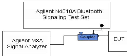
Figure 6-2. Test Instrument & Measurement Setup
