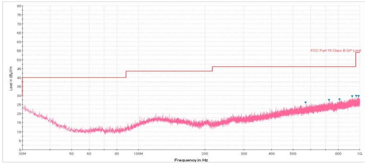
Plot 6-52. Radiated Spurious Plot below 1GHz (Pol. H)
