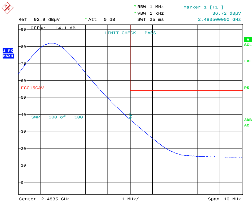
Plot 6-50. Radiated Restricted Upper Band Edge Measurement (Average)
