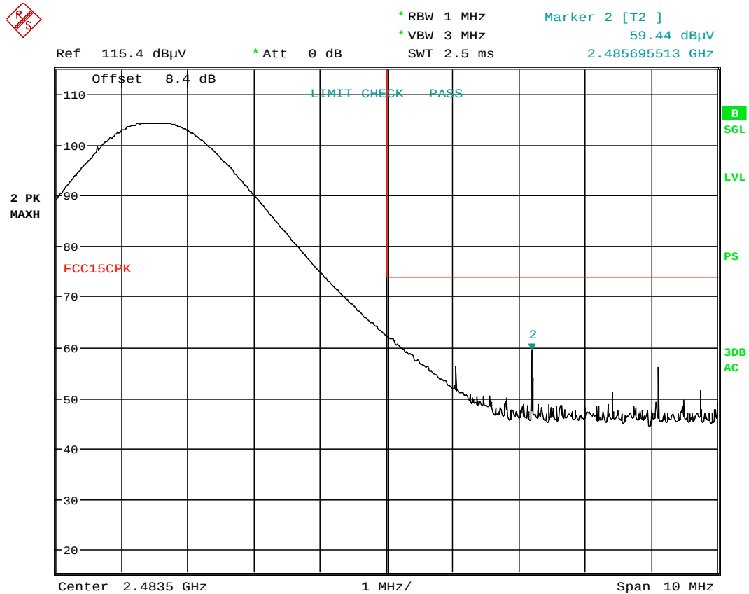
Plot 6-51. Radiated Restricted Upper Band Edge Measurement (Peak)
