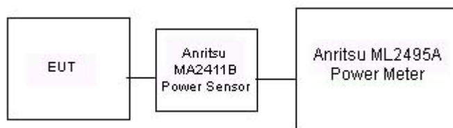
Figure 6-1. Test Instrument & Measurement Setup for Power Meter Measurements
