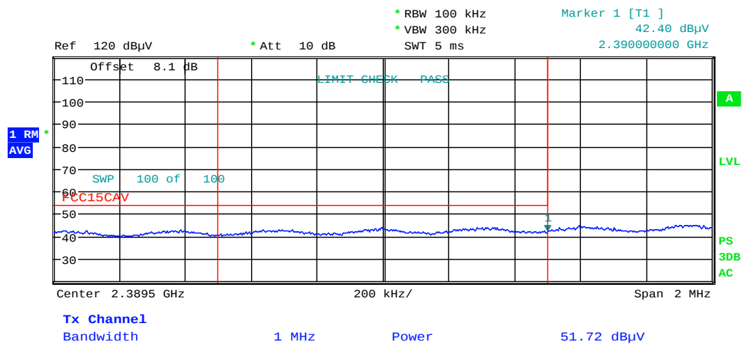
Plot 6-39. Radiated Restricted Lower Band Edge Measurement (Average)
