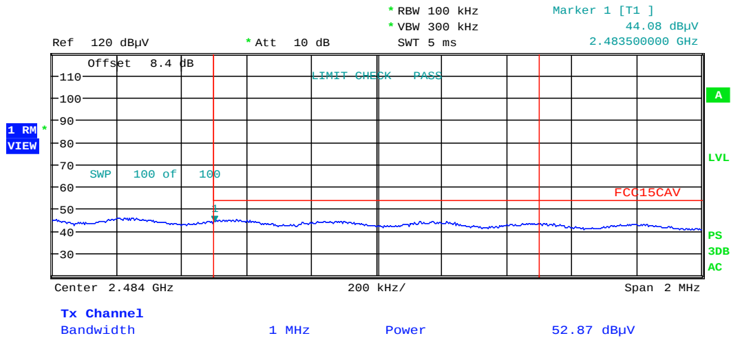
Plot 6-41. Radiated Restricted Upper Band Edge Measurement (Average)
