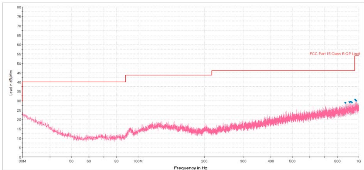
Plot 6-44. Radiated Spurious Plot below 1GHz (Pol. V)
