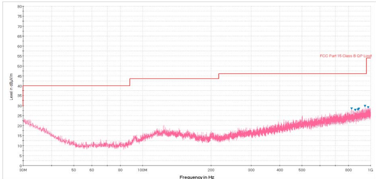
Plot 6-43. Radiated Spurious Plot below 1GHz (Pol. H)
