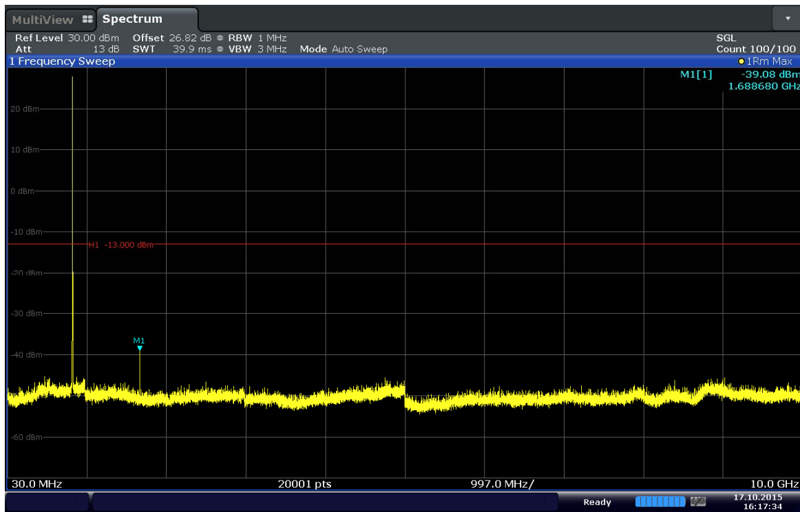
Plot 6-27. Conducted Spurious Plot (Band 5–5.0MHz–QPSK–RB Size 1–RB Offset 0–Ch.20625)
