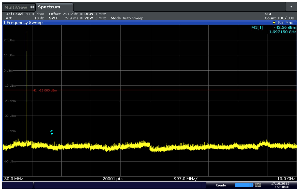
Plot 6-21. Conducted Spurious Plot (Band 5–1.4MHz–QPSK–RB Size 3–RB Offset 3–Ch.20643)
