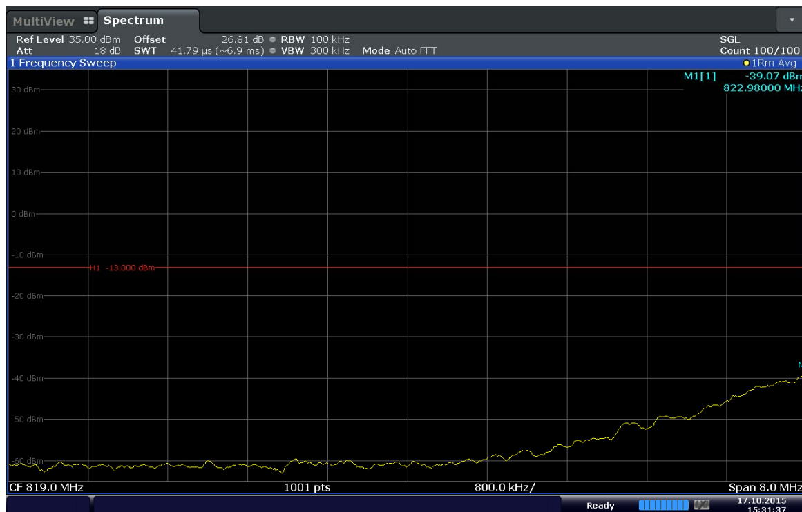
Plot 6-40. Extended Lower Band Edge Plot (Band5 – 1.4MHz – QPSK – RB Size 6)
