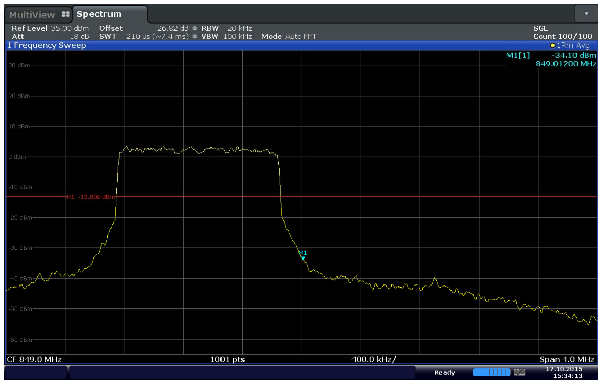
Plot 6-41. Upper Band Edge Plot (Band5 – 1.4MHz – QPSK – RB Size 6)
