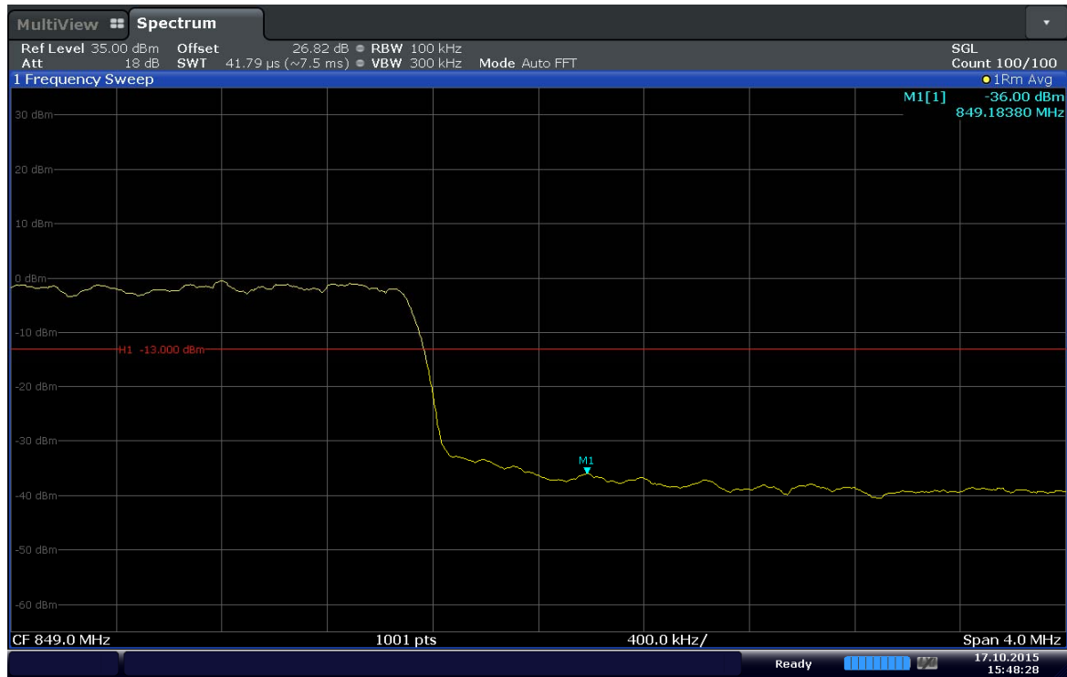
Plot 6-53. Upper Band Edge Plot (Band 5 – 10.0MHz – QPSK – RB Size 50)
