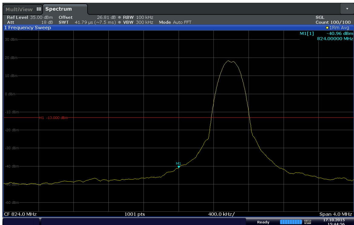
Plot 6-52. Lower Band Edge Plot (Band 5 – 10.0MHz – QPSK – RB Size 1 – RB Offset 0)
