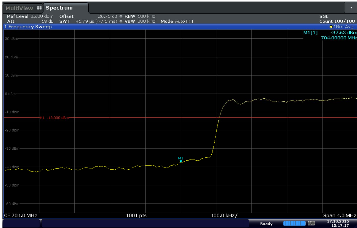
Plot 6-35. Lower Band Edge Plot (Band17 – 10MHz – QPSK – RB Size 50)
