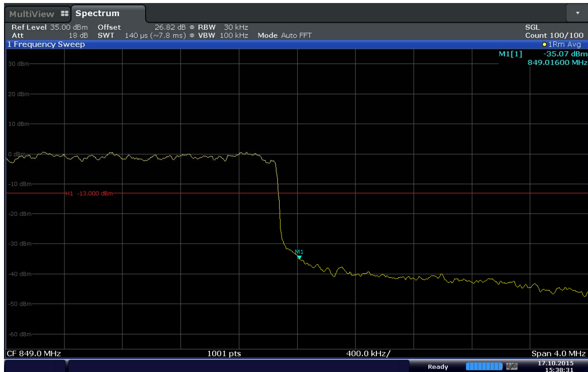
Plot 6-45. Upper Band Edge Plot (Band 5 – 3.0MHz – QPSK – RB Size 15)
