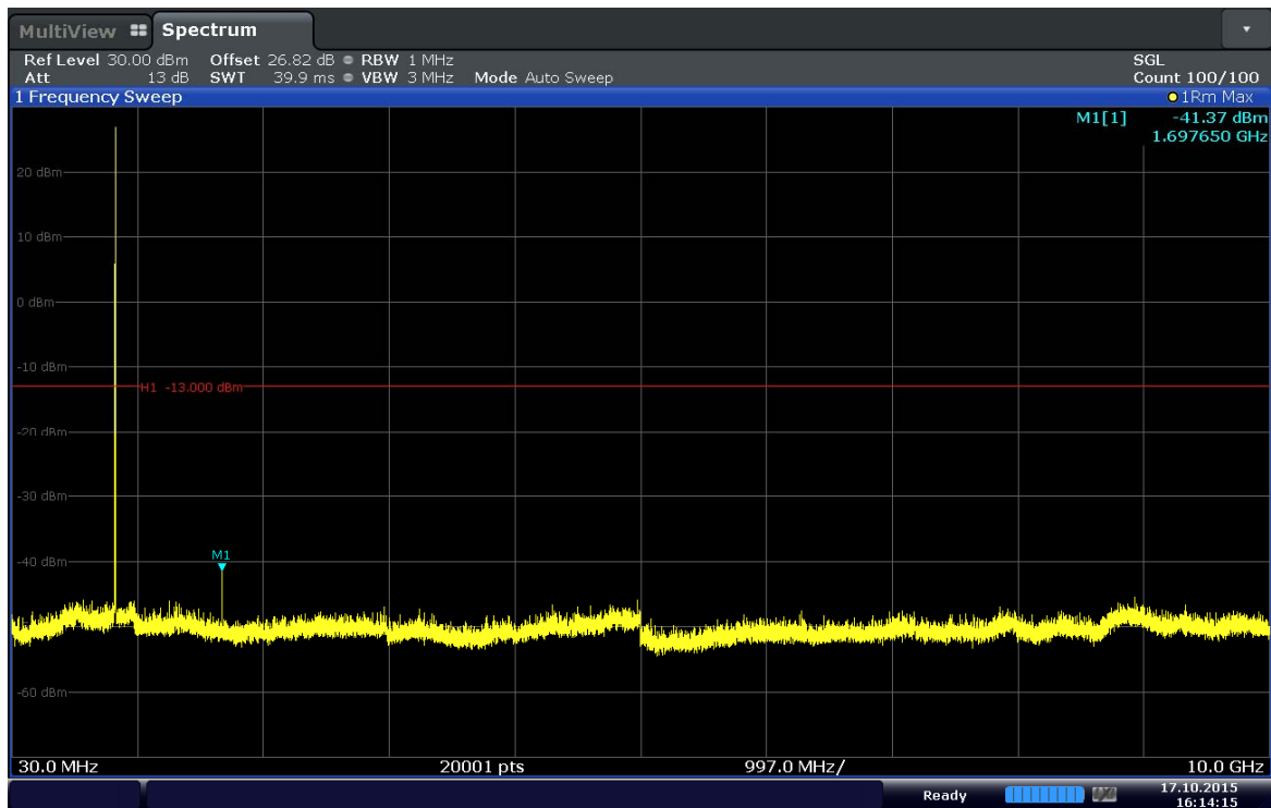
Plot 6-24. Conducted Spurious Plot (Band 5–3.0MHz–QPSK–RB Size 1–RB Offset 14–Ch.20635)
