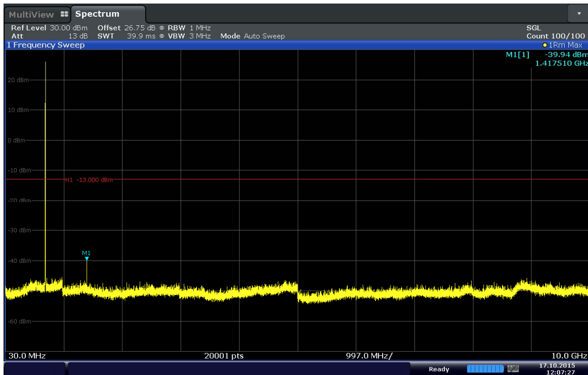
Plot 6-16. Conducted Spurious Plot (Band 17–10MHz–QPSK–RB Size 1–RB Offset 24–Ch.23780)
