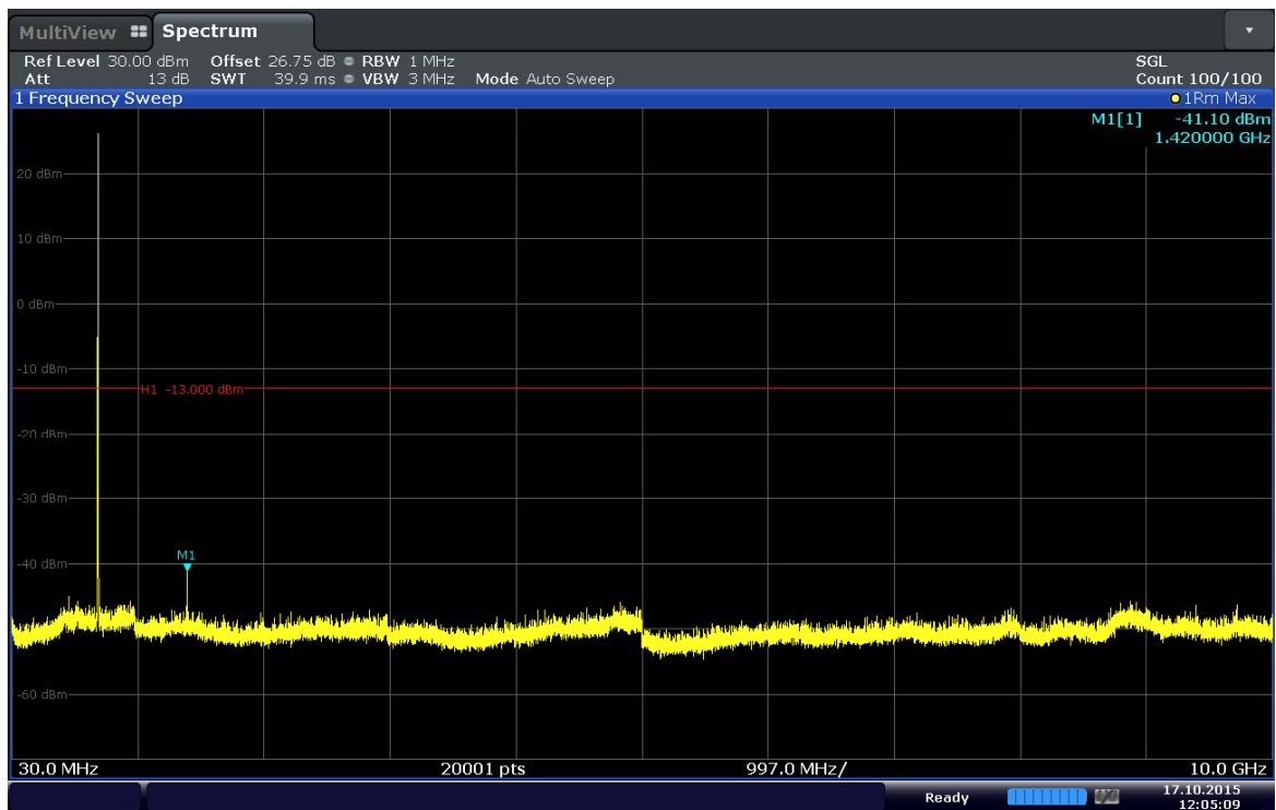
Plot 6-14. Conducted Spurious Plot (Band 17–5MHz–QPSK–RB Size 1–RB Offset 12–Ch.23790)
