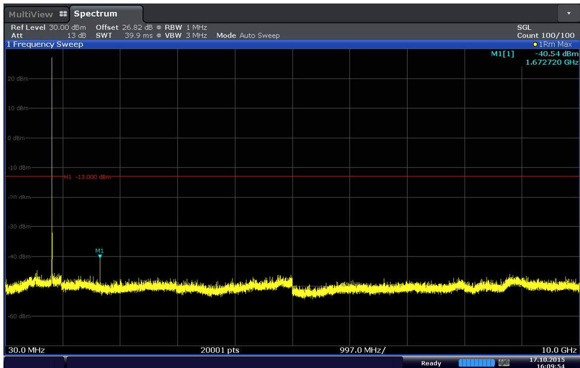
Plot 6-20. Conducted Spurious Plot (Band 5–1.4MHz–QPSK–RB Size 1–RB Offset 2–Ch.20525)
