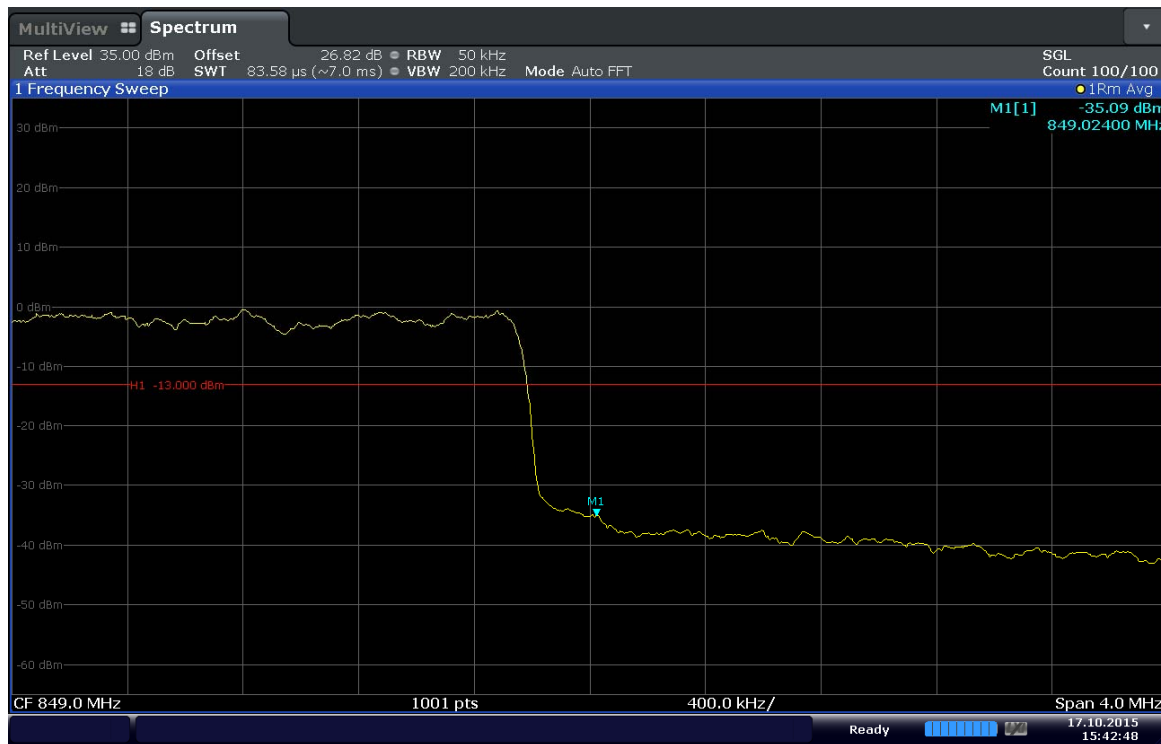
Plot 6-49. Upper Band Edge Plot (Band 5 – 5.0MHz – QPSK – RB Size 25)
