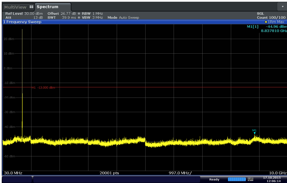
Plot 6-15. Conducted Spurious Plot (Band 17–5MHz–QPSK–RB Size 1–RB Offset 12–Ch.23825)
