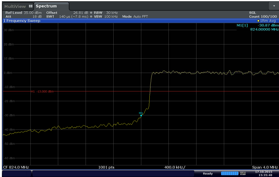
Plot 6-43. Lower Band Edge Plot (Band 5 – 3.0MHz – QPSK – RB Size 15)
