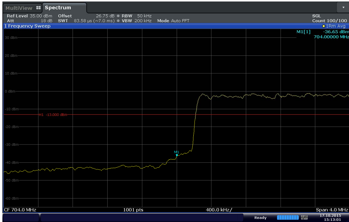
Plot 6-31. Lower Band Edge Plot (Band17 – 5MHz – QPSK – RB Size 25)
