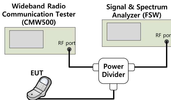
Figure 6-2. Test Instruments & Measurement Setup
