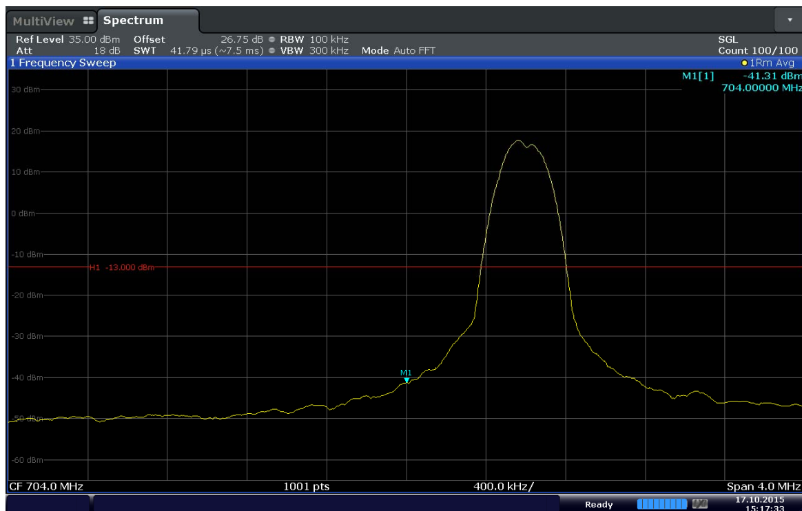
Plot 6-36. Lower Band Edge Plot (Band17 – 10MHz – QPSK – RB Size 1 – RB Offset 0)
