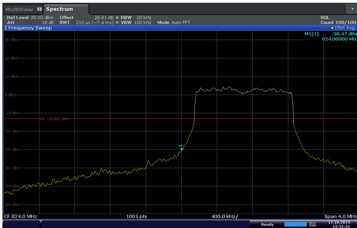
Plot 6-39. Lower Band Edge Plot (Band5 – 1.4MHz – QPSK – RB Size 6)
