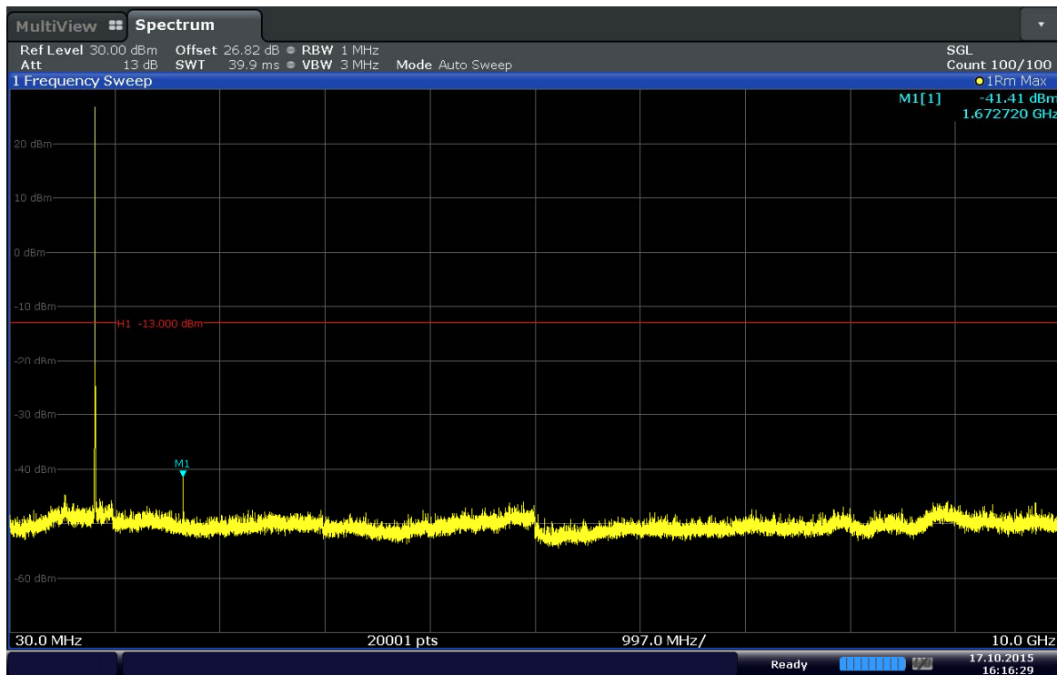
Plot 6-26. Conducted Spurious Plot (Band 5–5.0MHz–QPSK–RB Size 1–RB Offset 12–Ch.20525)
