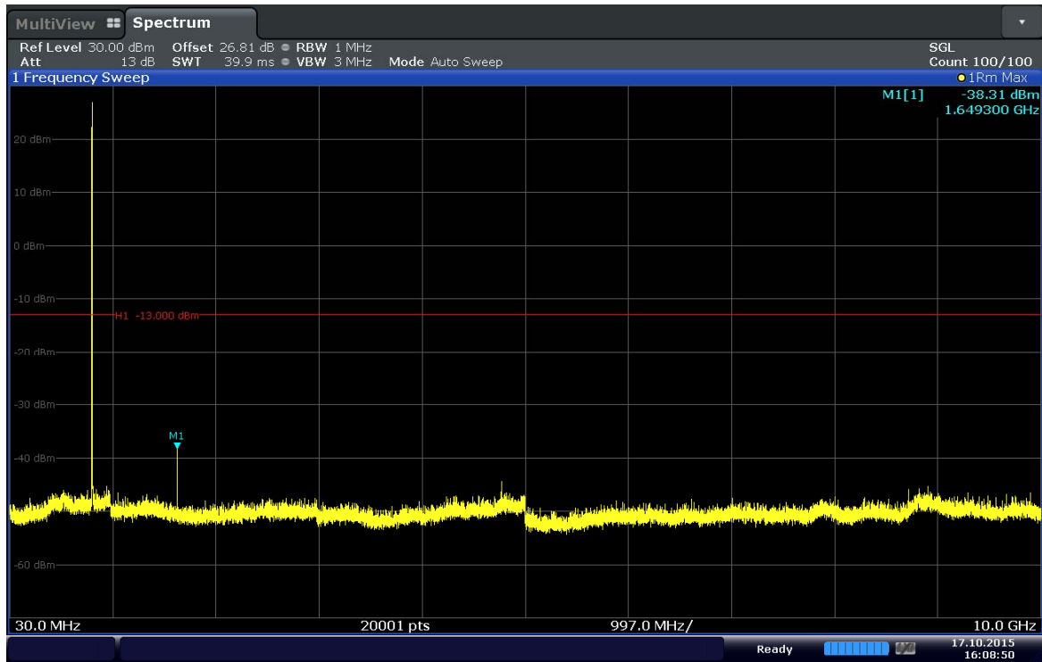
Plot 6-19. Conducted Spurious Plot (Band 5–1.4MHz–QPSK–RB Size 1–RB Offset 2–Ch.20407)
