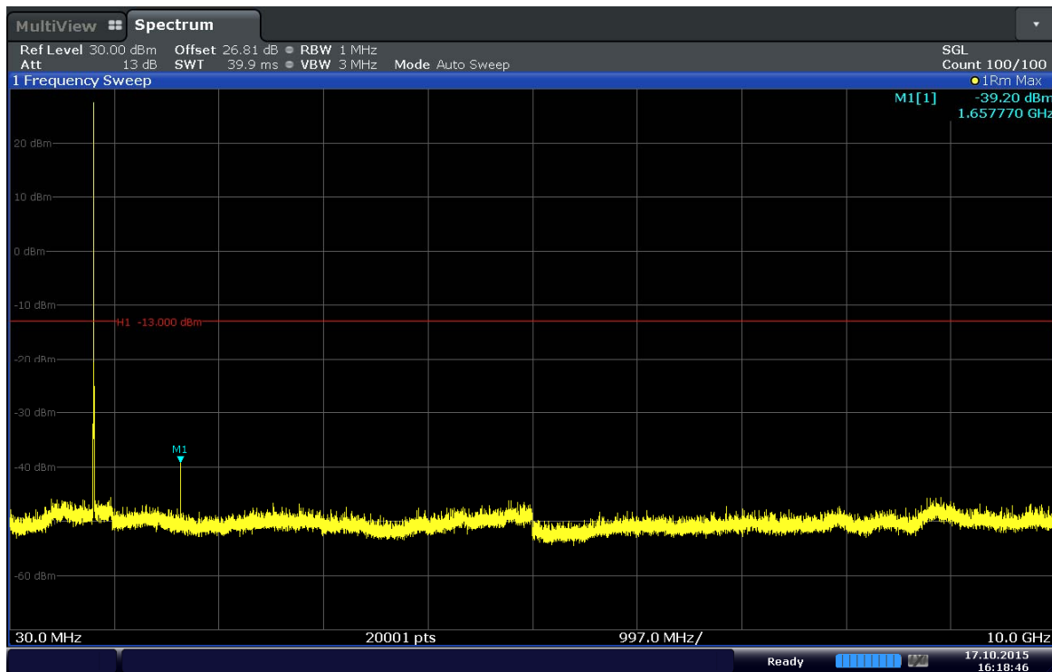
Plot 6-28. Conducted Spurious Plot (Band 5–10.0MHz–QPSK–RB Size 1–RB Offset 25–Ch.20450)
