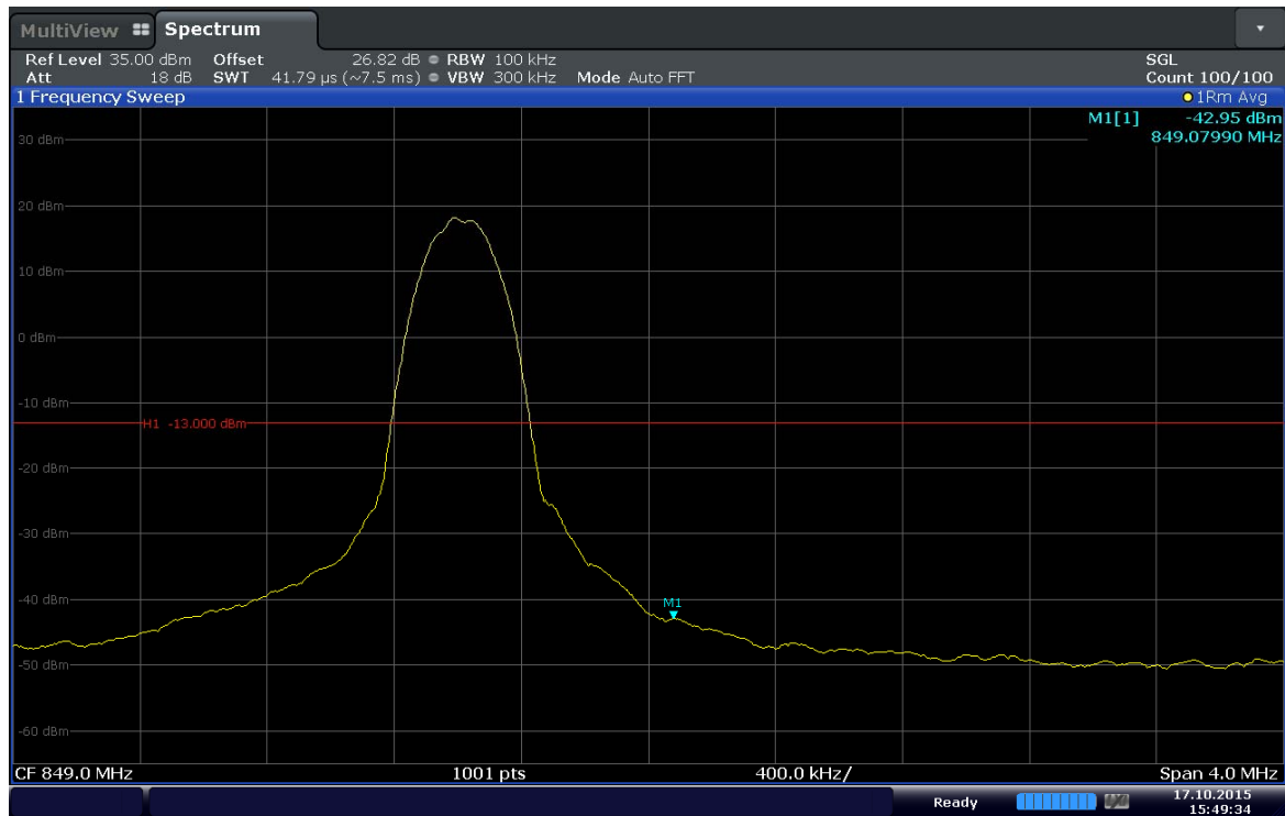
Plot 6-54. Upper Band Edge Plot (Band 5 – 10.0MHz – QPSK – RB Size 1 – RB Offset 49)
