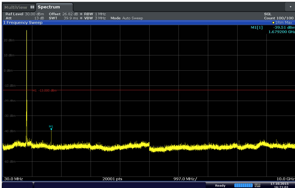
Plot 6-30. Conducted Spurious Plot (Band 5–10.0MHz–QPSK–RB Size 1–RB Offset 0–Ch.20600)
