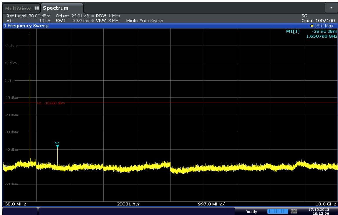
Plot 6-22. Conducted Spurious Plot (Band 5–3.0MHz–QPSK–RB Size 1–RB Offset 7–Ch.20415)
