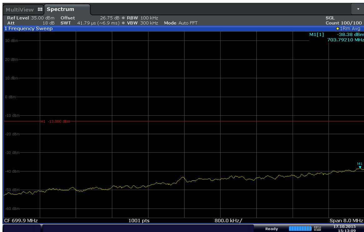
Plot 6-32.Extended Lower Band Edge Plot (Band17 – 5MHz – QPSK – RB Size 25)
