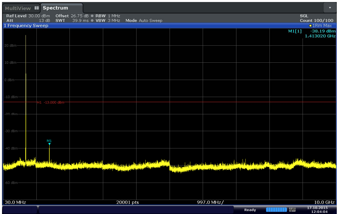
Plot 6-13. Conducted Spurious Plot (Band 17–5MHz–QPSK–RB Size 1–RB Offset 12–Ch.23755)
