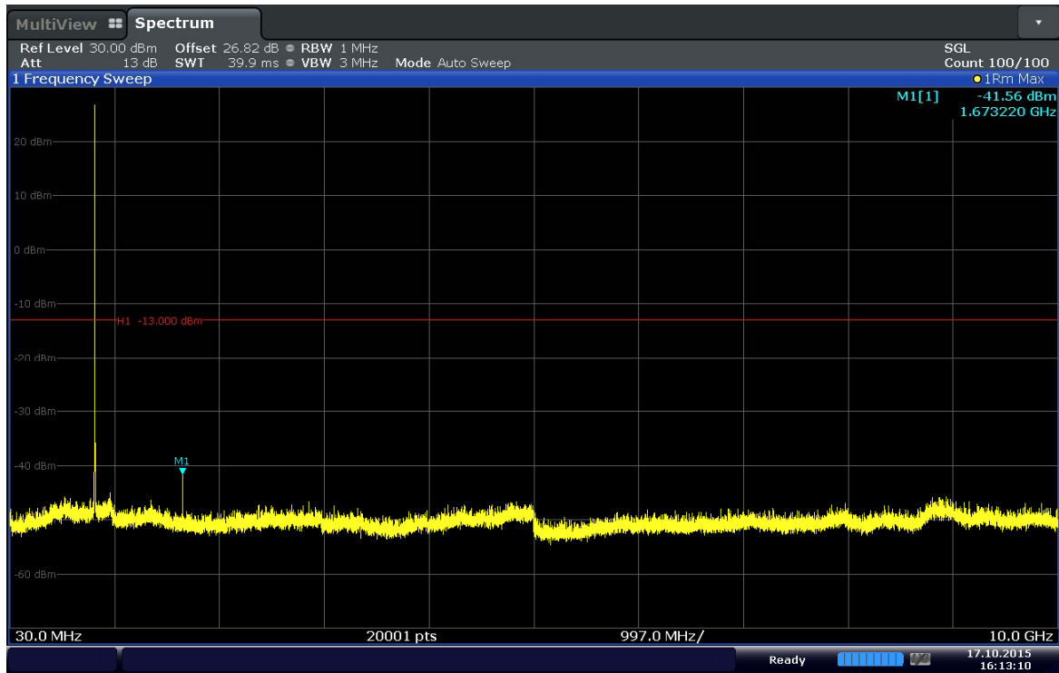
Plot 6-23. Conducted Spurious Plot (Band 5–3.0MHz–QPSK–RB Size 1–RB Offset 7–Ch.20525)
