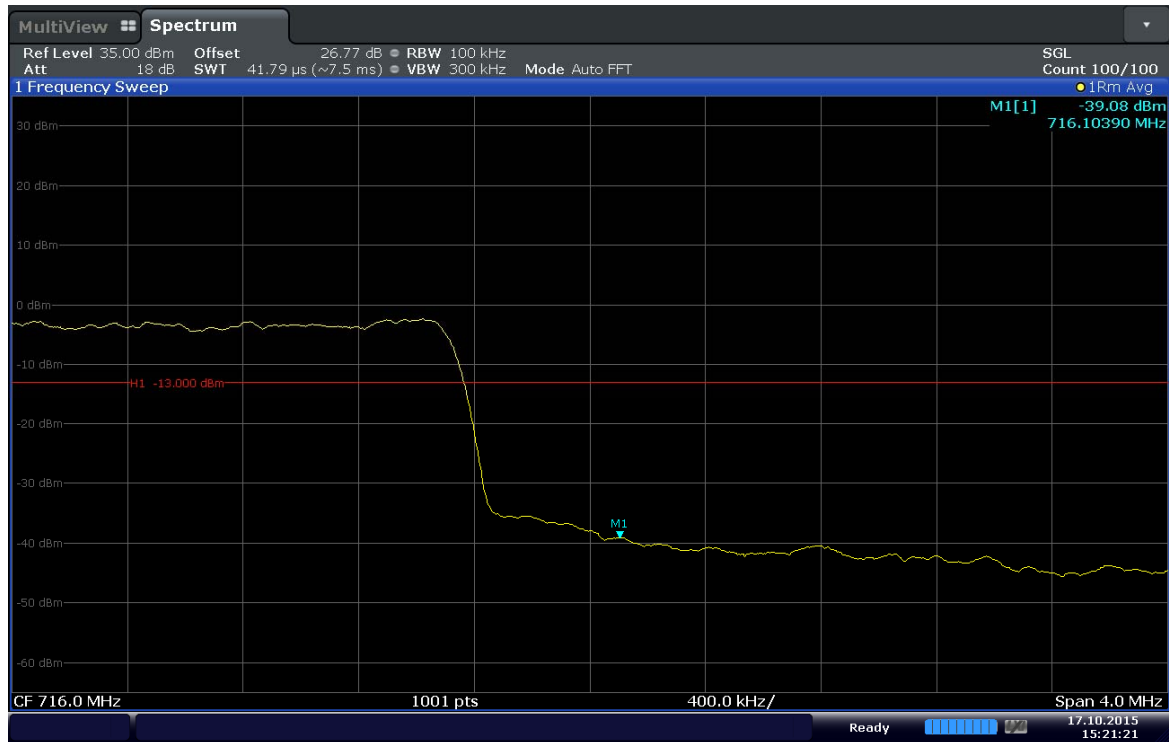
Plot 6-37. Upper Band Edge Plot (Band17 – 10MHz – QPSK – RB Size 50)
