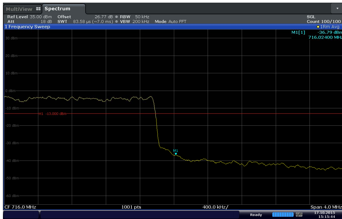
Plot 6-33. Upper Band Edge Plot (Band17 – 5MHz – QPSK – RB Size 25)
