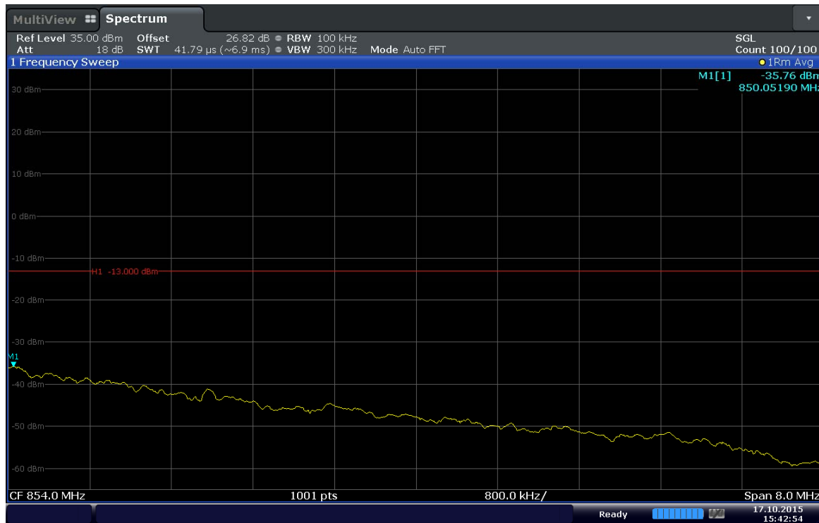
Plot 6-50. Extended Upper Band Edge Plot (Band 5 – 5.0MHz – QPSK – RB Size 25)
