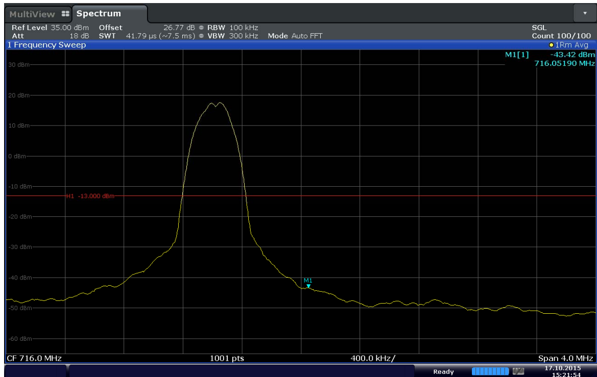
Plot 6-38. Upper Band Edge Plot (Band17 – 10MHz – QPSK – RB Size 1 – RB Offset 49)
