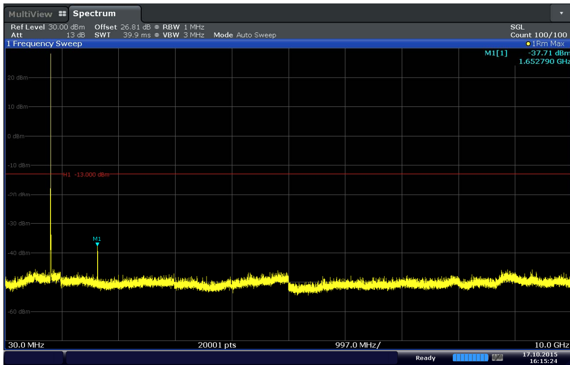
Plot 6-25. Conducted Spurious Plot (Band 5–5.0MHz–QPSK–RB Size 1–RB Offset 12–Ch.20425)
