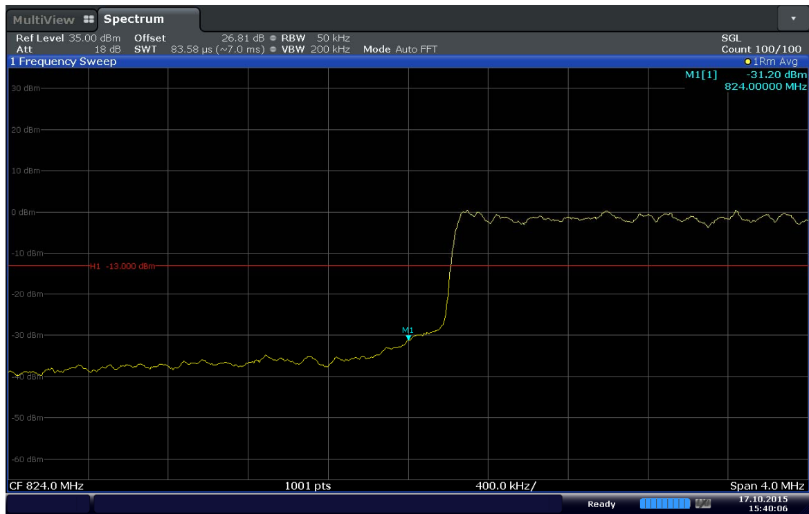
Plot 6-47. Lower Band Edge Plot (Band 5 – 5.0MHz – QPSK – RB Size 25)
