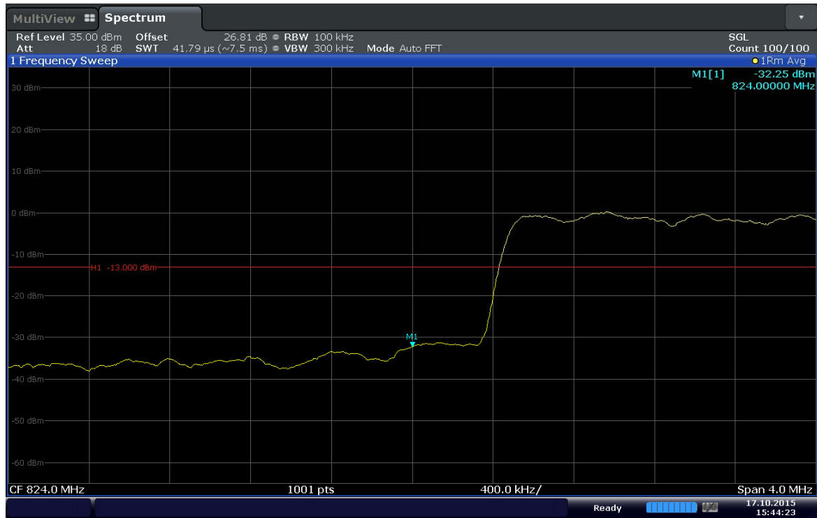
Plot 6-51. Lower Band Edge Plot (Band 5 – 10.0MHz – QPSK – RB Size 50)
