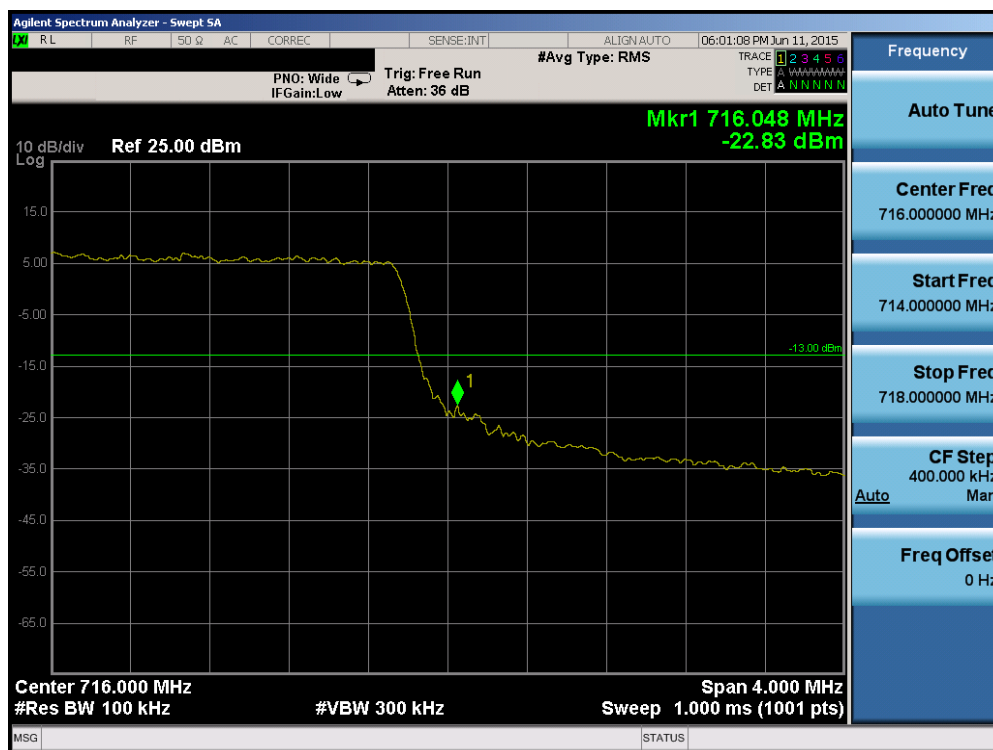
Plot 6-74. Upper Band Edge Plot (Band 17 – 5.0MHz QPSK – RB Size 25)
