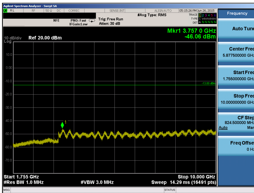
Plot 6-36. Conducted Spurious Plot (AWS WCDMA Mode – Ch. 1312)
