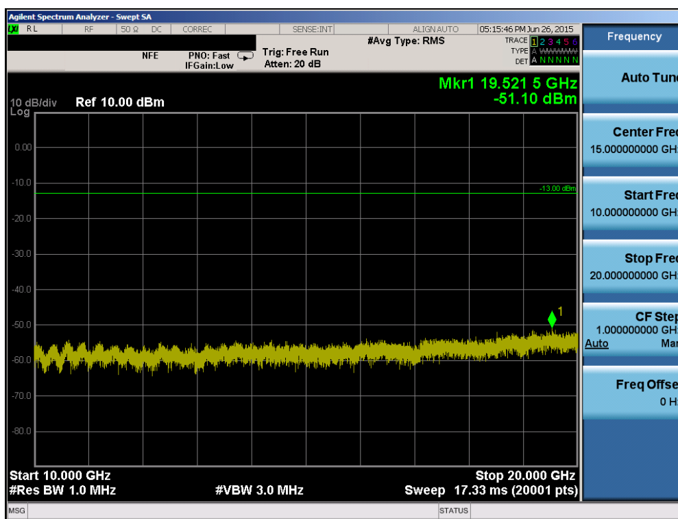
Plot 6-37. Conducted Spurious Plot (AWS WCDMA Mode – Ch. 1312)
