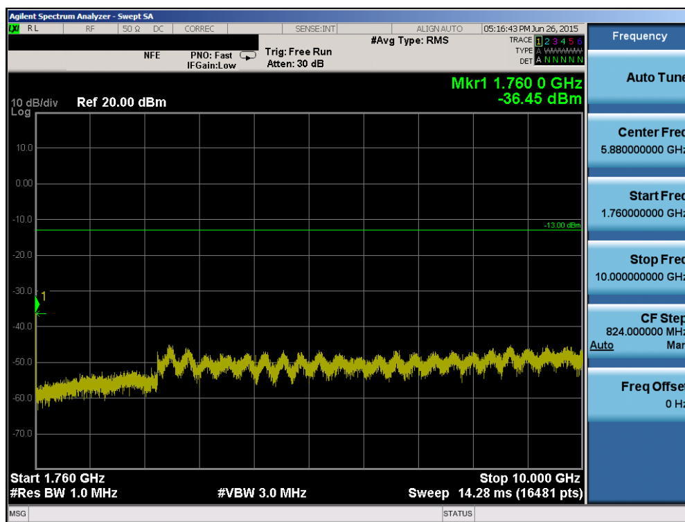
Plot 6-42. Conducted Spurious Plot (AWS WCDMA Mode – Ch. 1862)
