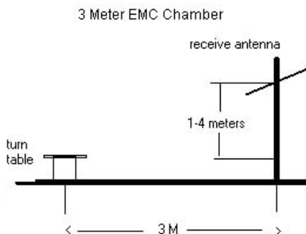
Figure 6-2. Test Instrument & Measurement Setup
