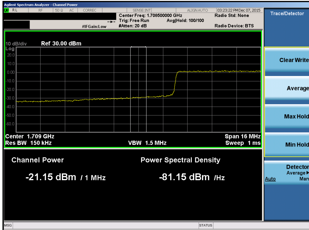
Plot 7-149. Lower Extended Band Edge Plot (Band 4 – 20.0MHz QPSK – RB Size 100)
