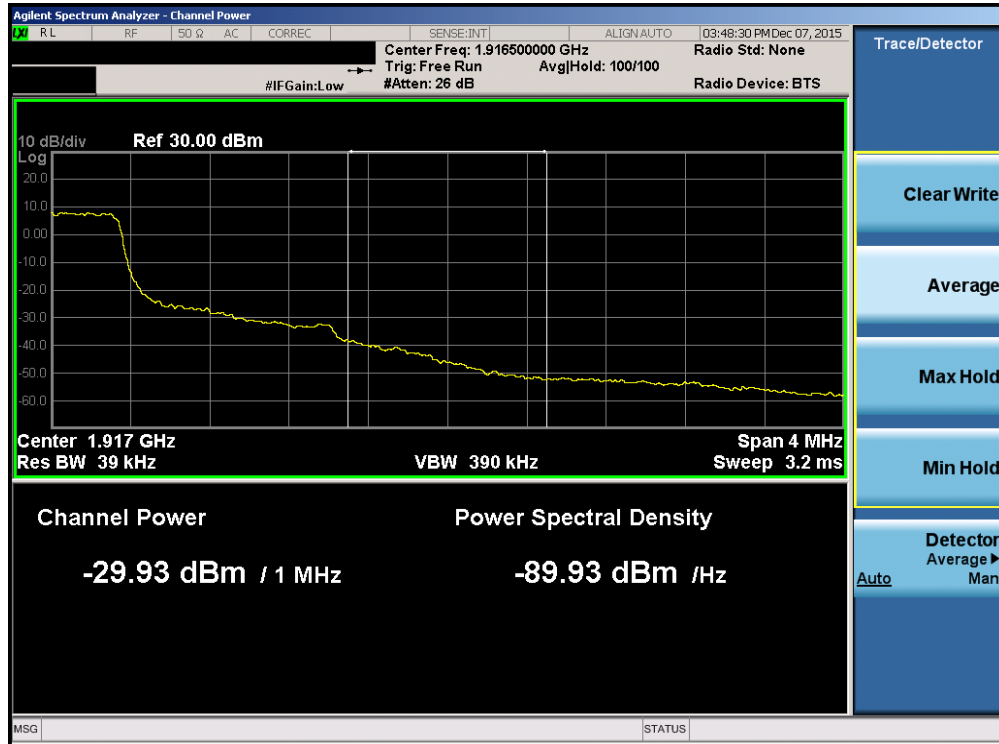
Plot 7-155. Upper Extended Band Edge Plot (Band 2/25 – 1.4MHz QPSK – RB Size 6)
