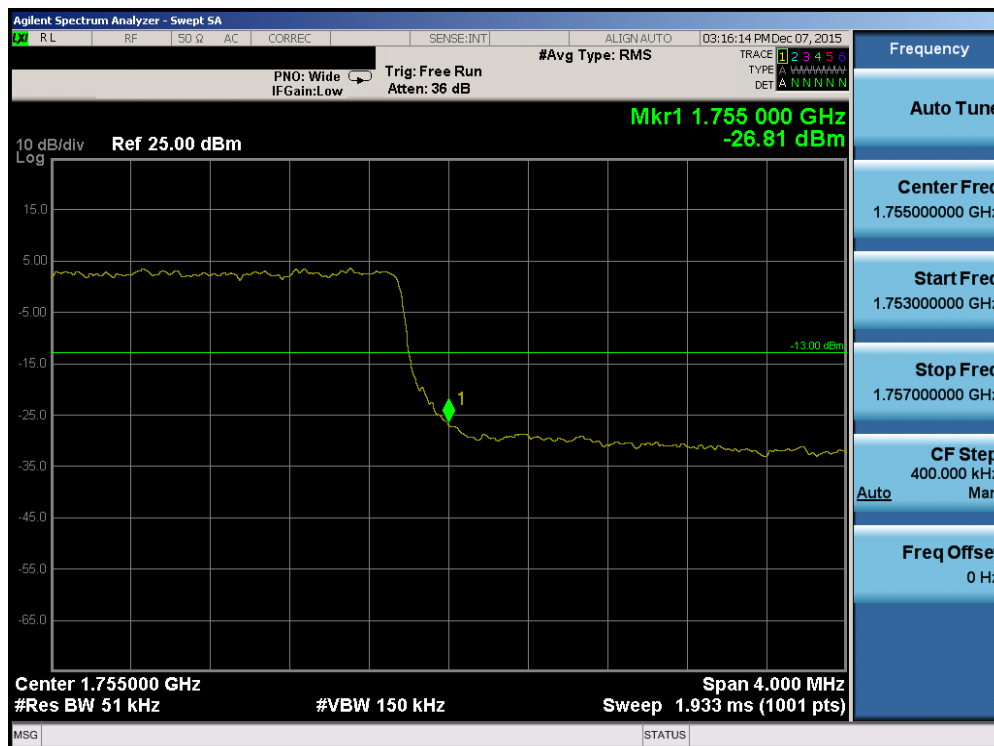
Plot 7-138. Upper Band Edge Plot (Band 4 – 5.0MHz QPSK – RB Size 25)
