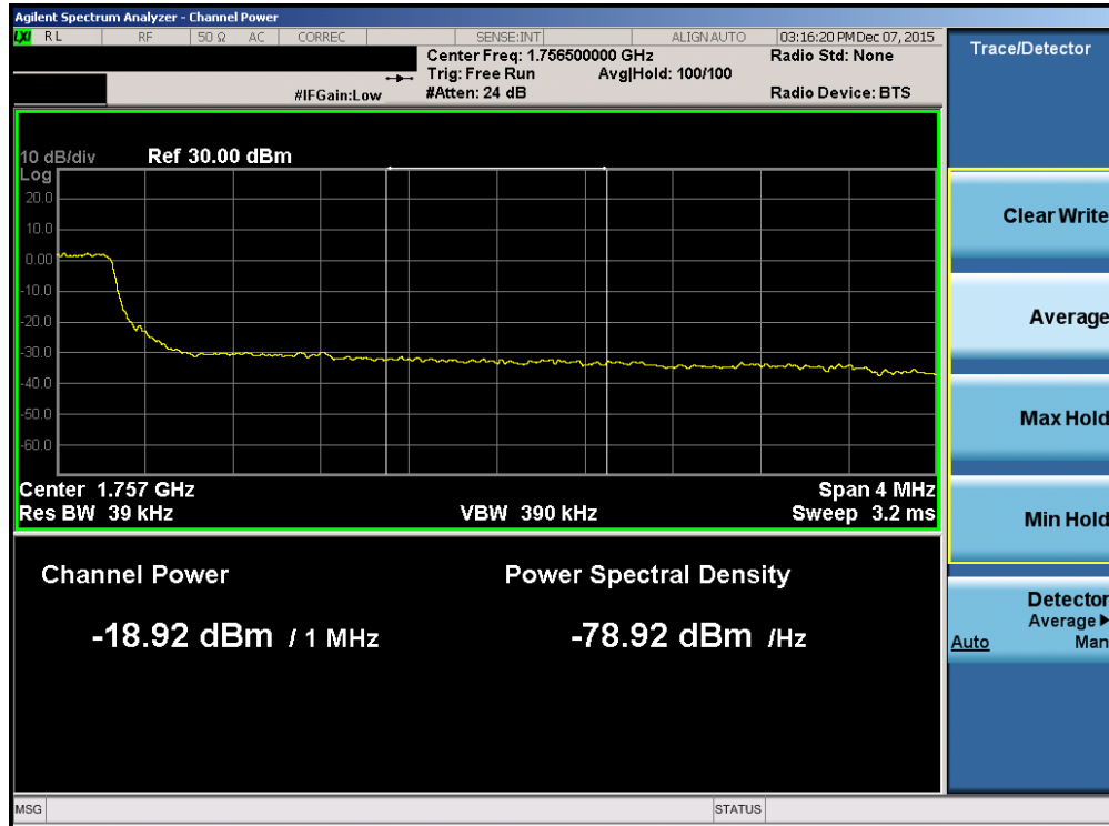
Plot 7-139. Upper Extended Band Edge Plot (Band 4 – 5.0MHz QPSK – RB Size 25)
