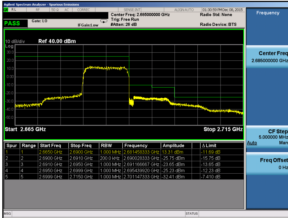
Plot 7-179. Upper ACP Plot (Band 41 – 10.0MHz QPSK – RB Size 50)
