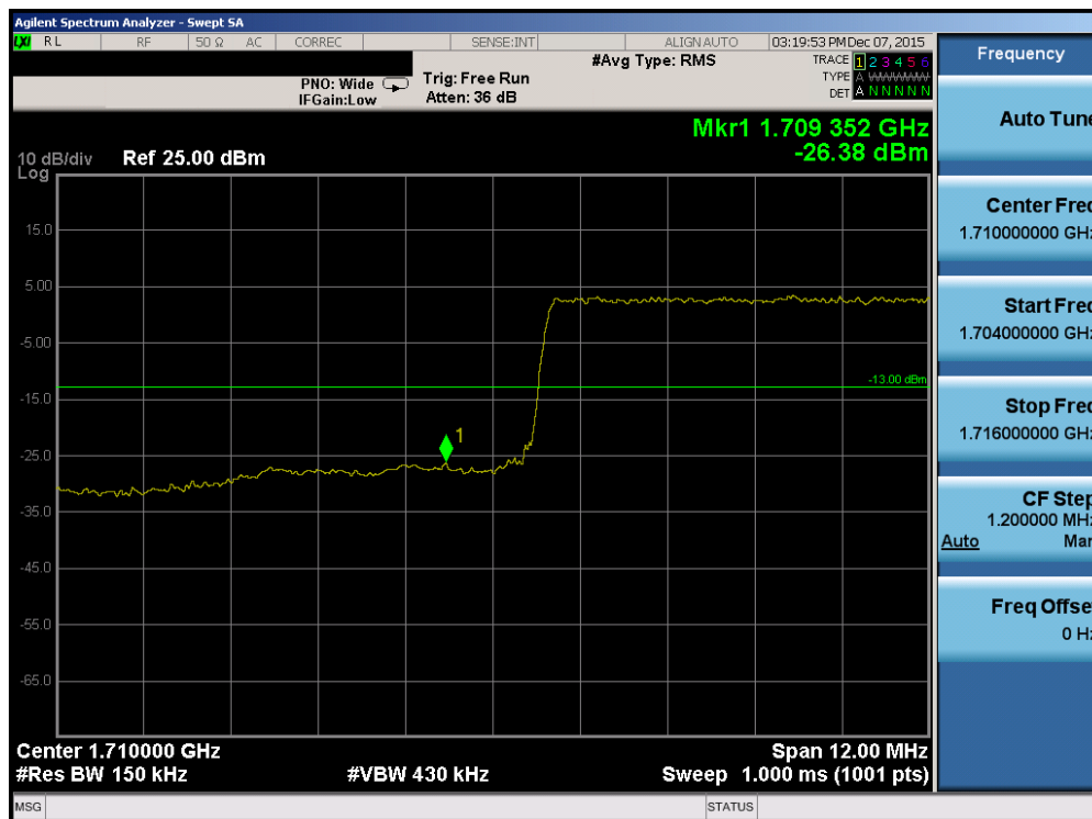
Plot 7-144. Lower Band Edge Plot (Band 4 – 15.0MHz QPSK – RB Size 75)
