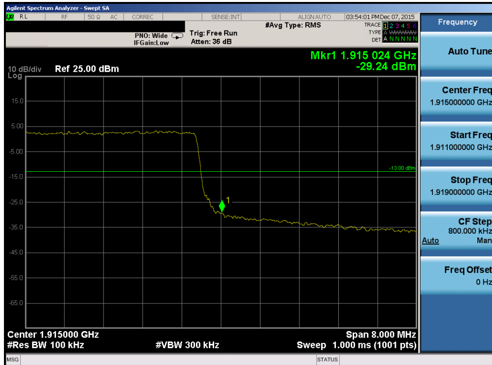
Plot 7-166. Upper Band Edge Plot (Band 2/25 – 10.0MHz QPSK – RB Size 50)
