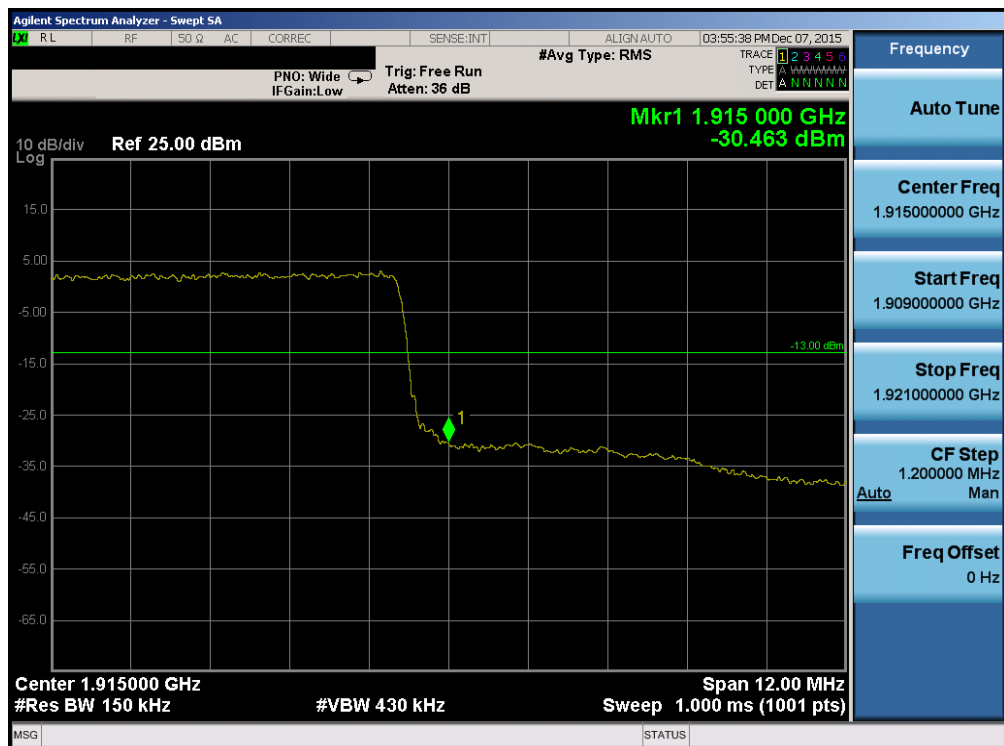
Plot 7-170. Upper Band Edge Plot (Band 2/25 – 15.0MHz QPSK – RB Size 75)
