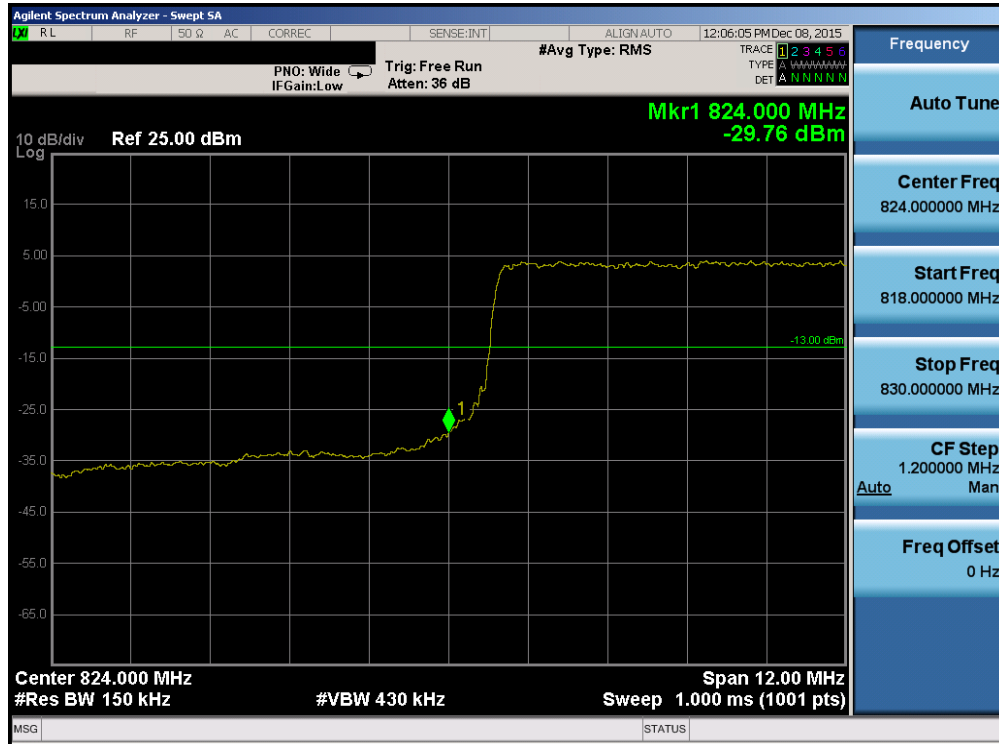
Plot 7-125. Lower Band Edge Plot (Band 26 – 15.0MHz QPSK – RB Size 75)
