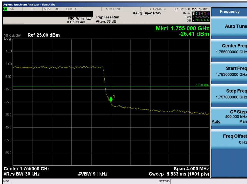
Plot 7-134. Upper Band Edge Plot (Band 4 – 3.0MHz QPSK – RB Size 15)
