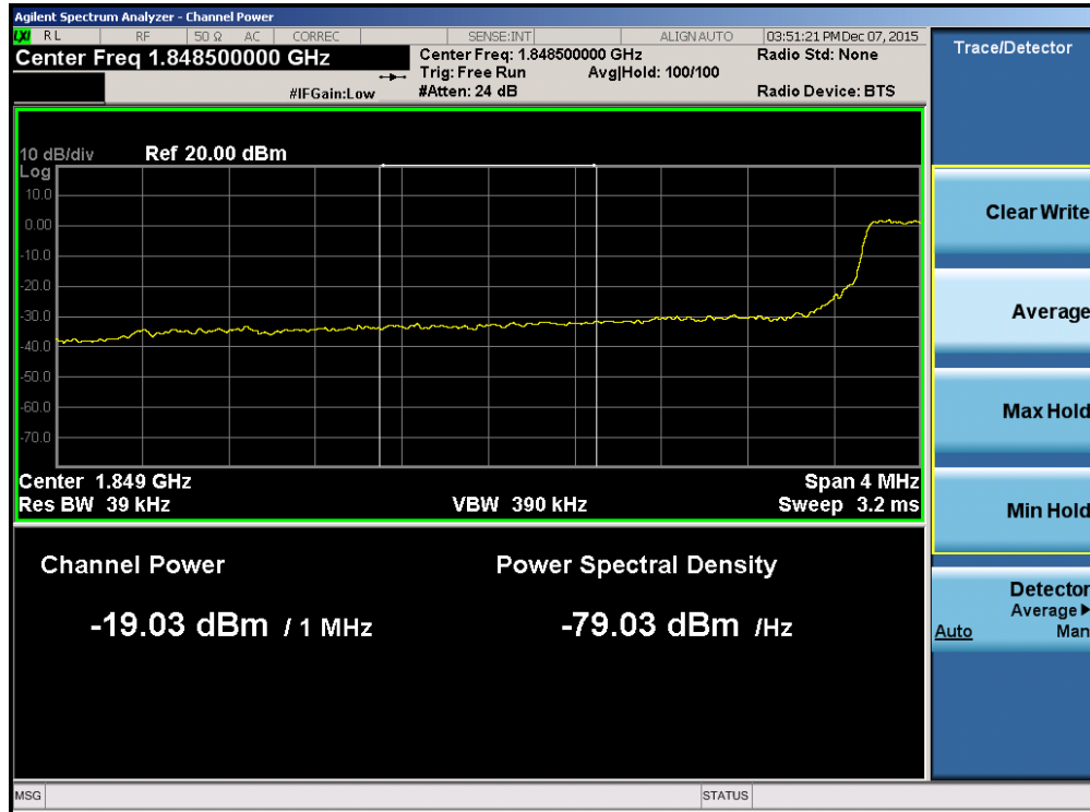
Plot 7-161. Lower Extended Band Edge Plot (Band 2/25 – 5.0MHz QPSK – RB Size 25)
