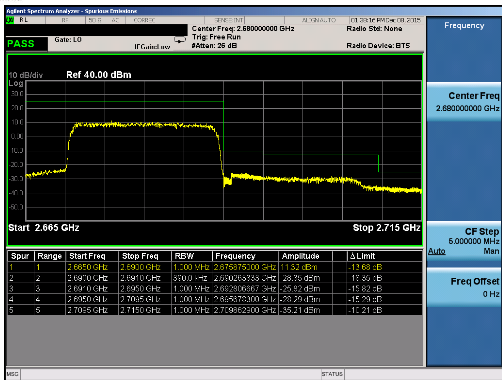
Plot 7-183. Upper ACP Plot (Band 41 – 20.0MHz QPSK – RB Size 100)
