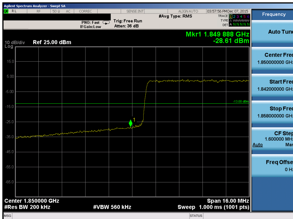
Plot 7-172. Lower Band Edge Plot (Band 2/25 – 20.0MHz QPSK – RB Size 100)
