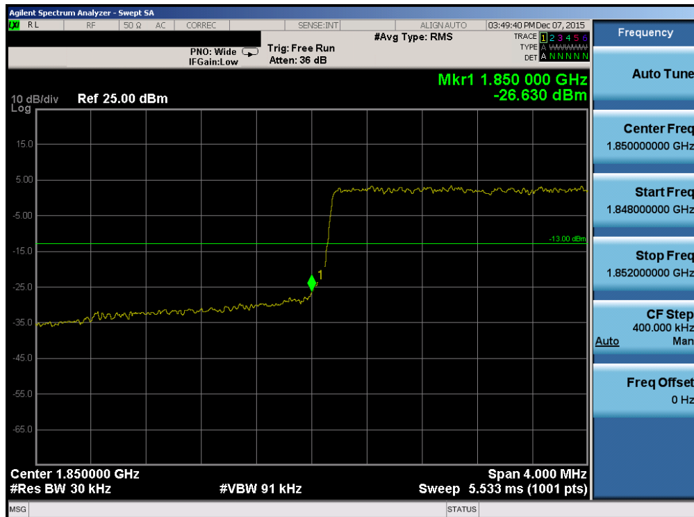
Plot 7-156. Lower Band Edge Plot (Band 2/25 – 3.0MHz QPSK – RB Size 15)
