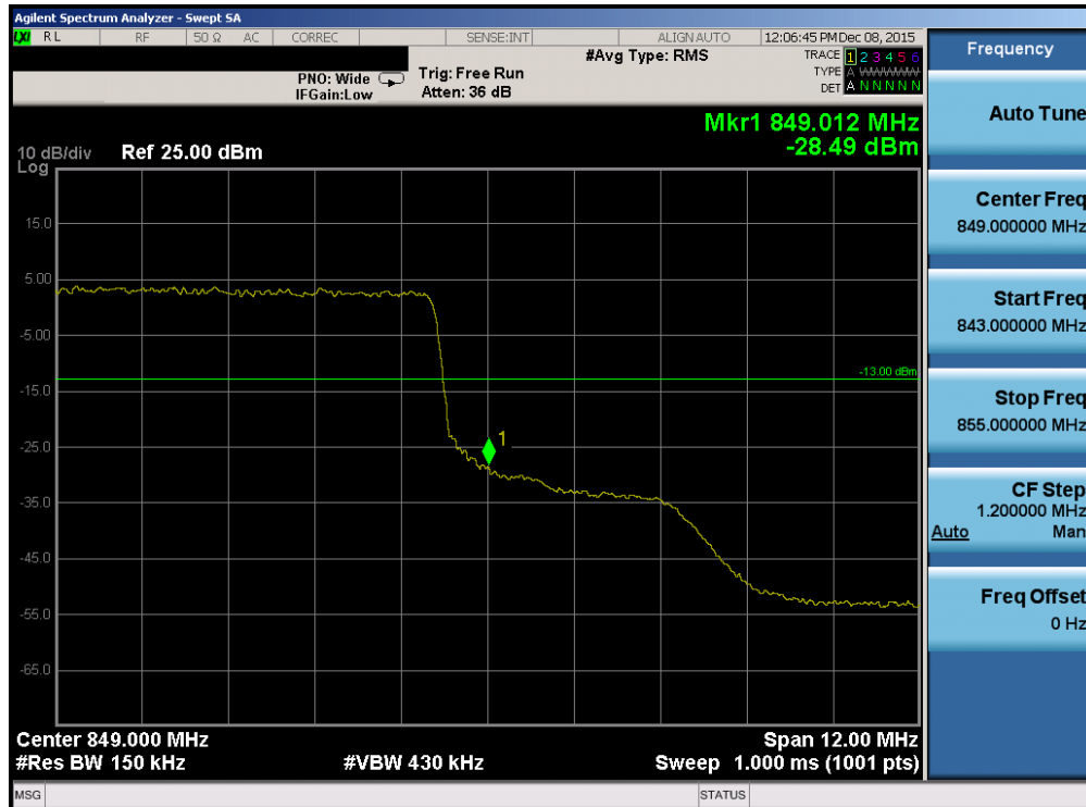
Plot 7-126. Upper Band Edge Plot (Band 26 – 15.0MHz QPSK – RB Size 75)
