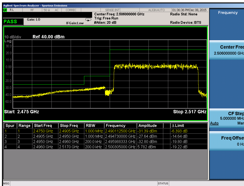
Plot 7-182. Lower ACP Plot (Band 41 – 20.0MHz QPSK – RB Size 100)
