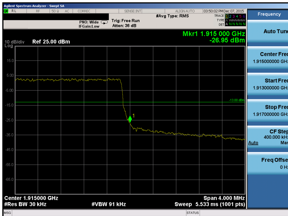
Plot 7-158. Upper Band Edge Plot (Band 2/25 – 3.0MHz QPSK – RB Size 15)
