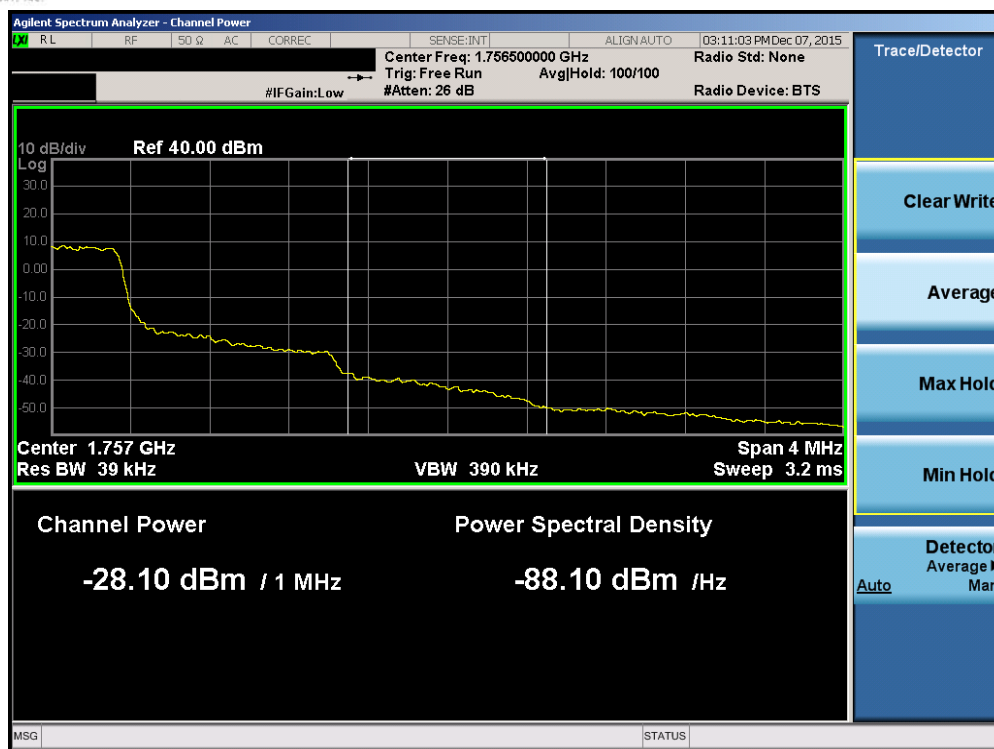
Plot 7-131. Upper Extended Band Edge Plot (Band 4 – 1.4MHz QPSK – RB Size 6)
