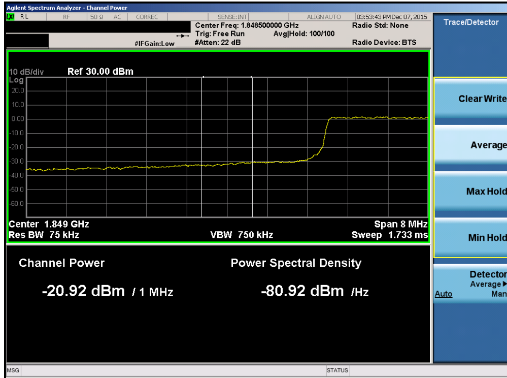
Plot 7-165. Lower Extended Band Edge Plot (Band 2/25 – 10.0MHz QPSK – RB Size 50)
