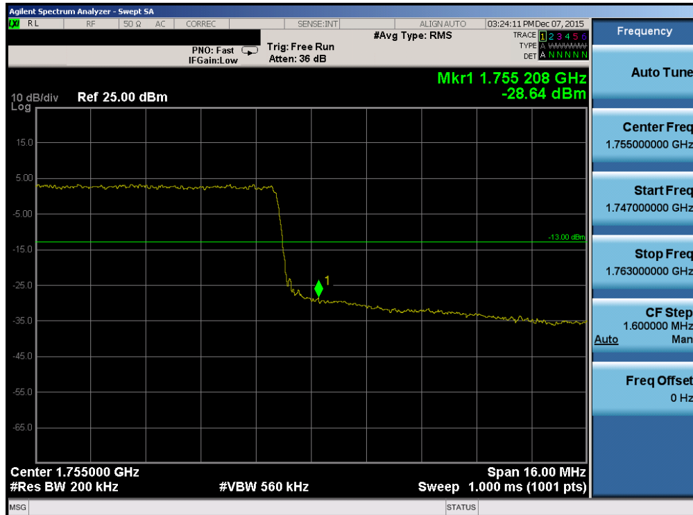
Plot 7-150. Upper Band Edge Plot (Band 4 – 20.0MHz QPSK – RB Size 100)
