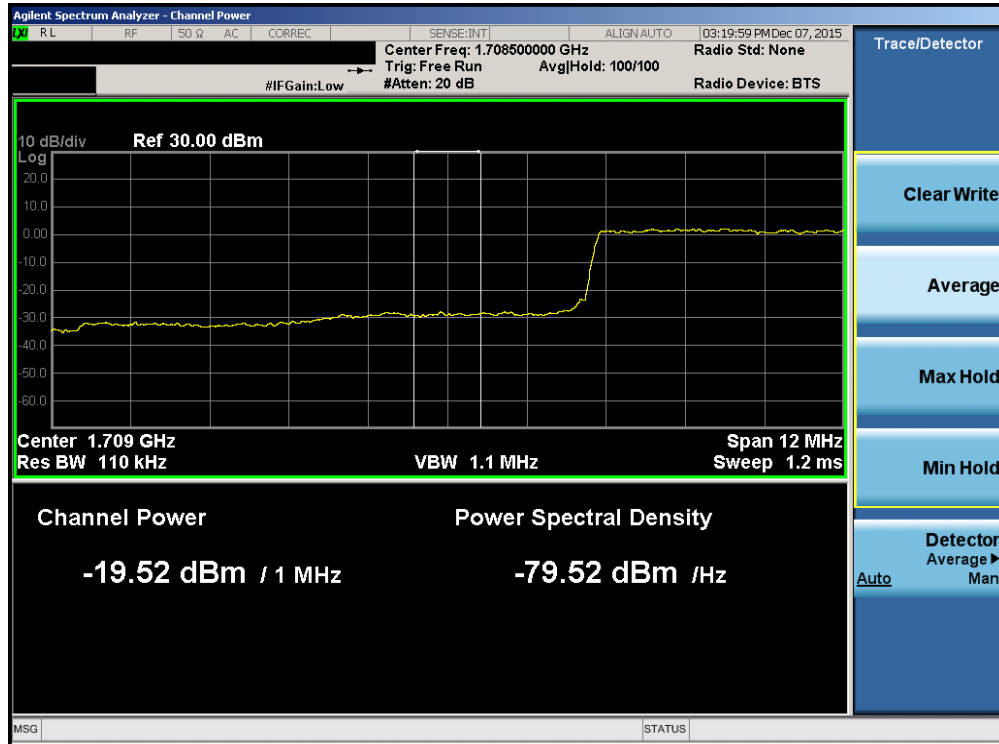
Plot 7-145. Lower Extended Band Edge Plot (Band 4 – 15.0MHz QPSK – RB Size 75)
