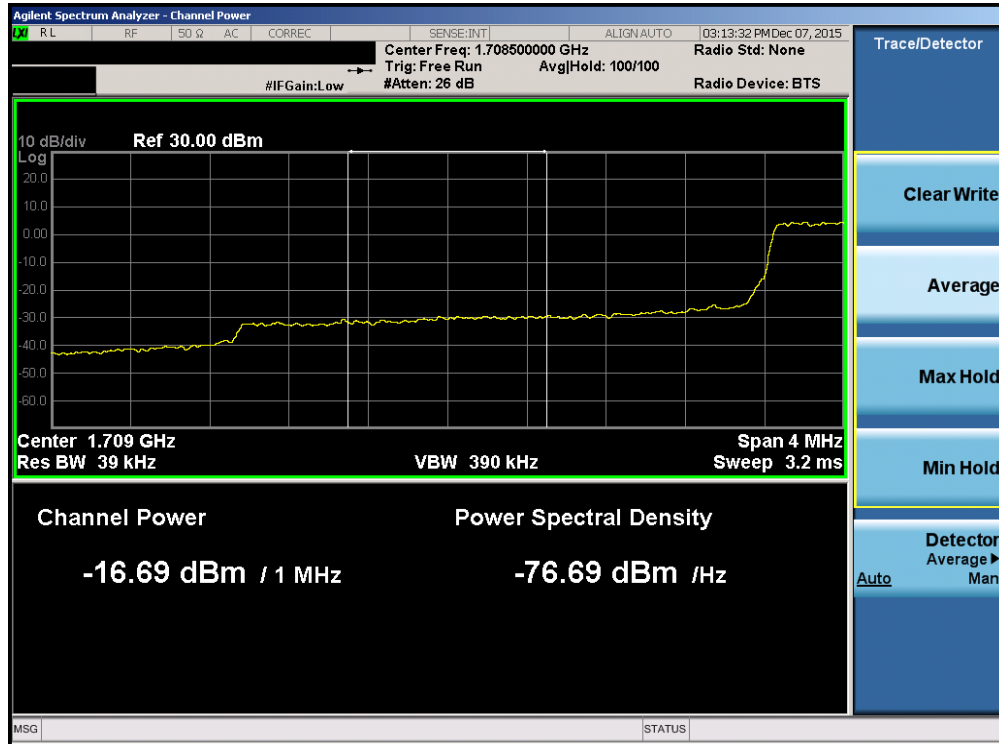
Plot 7-133. Lower Extended Band Edge Plot (Band 4 – 3.0MHz QPSK – RB Size 15)
