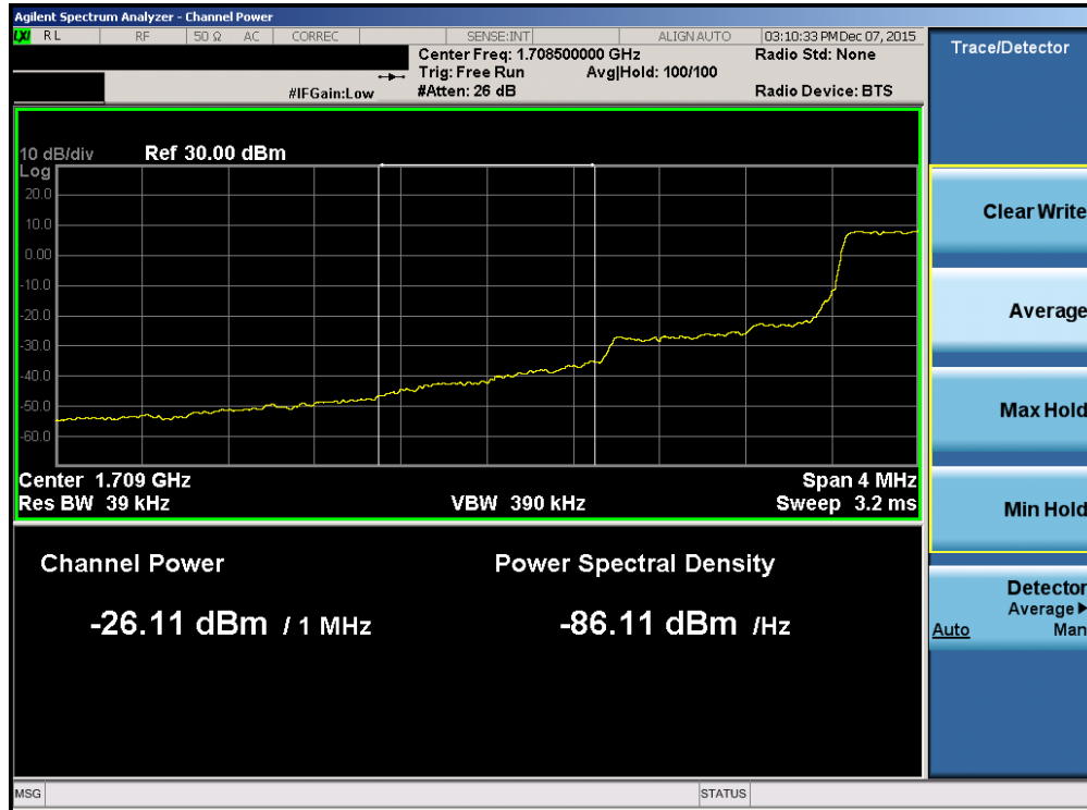
Plot 7-129. Lower Extended Band Edge Plot (Band 4 – 1.4MHz QPSK – RB Size 6)
