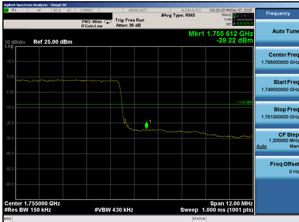
Plot 7-146. Upper Band Edge Plot (Band 4 – 15.0MHz QPSK – RB Size 75)
