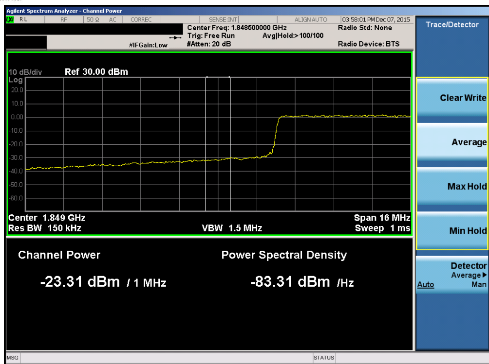
Plot 7-173. Lower Extended Band Edge Plot (Band 2/25 – 20.0MHz QPSK – RB Size 100)
