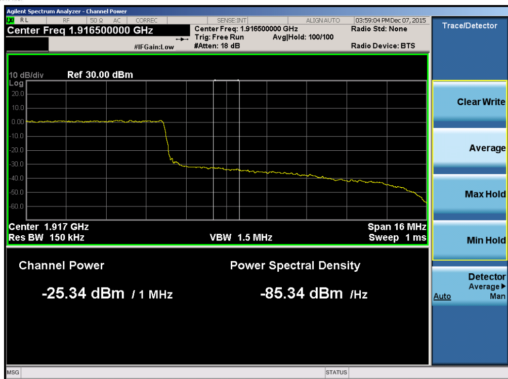
Plot 7-175. Upper Extended Band Edge Plot (Band 2/25 – 20.0MHz QPSK – RB Size 100)
