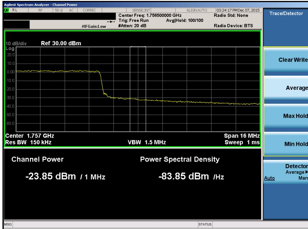
Plot 7-151. Upper Extended Band Edge Plot (Band 4 – 20.0MHz QPSK – RB Size 100)
