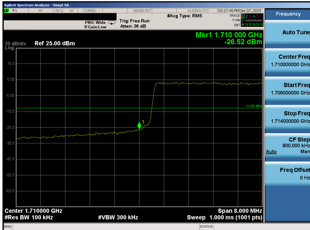
Plot 7-140. Lower Band Edge Plot (Band 4 – 10.0MHz QPSK – RB Size 50)
