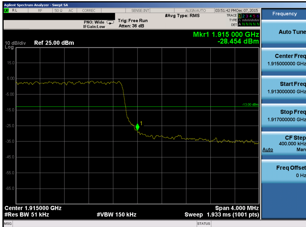
Plot 7-162. Upper Band Edge Plot (Band 2/25 – 5.0MHz QPSK – RB Size 25)
