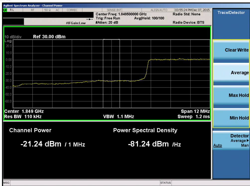
Plot 7-169. Lower Extended Band Edge Plot (Band 2/25 – 15.0MHz QPSK – RB Size 75)
