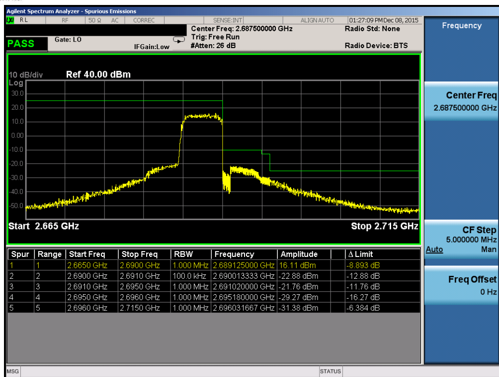
Plot 7-177. Upper ACP Plot (Band 41 – 5.0MHz QPSK – RB Size 25)
