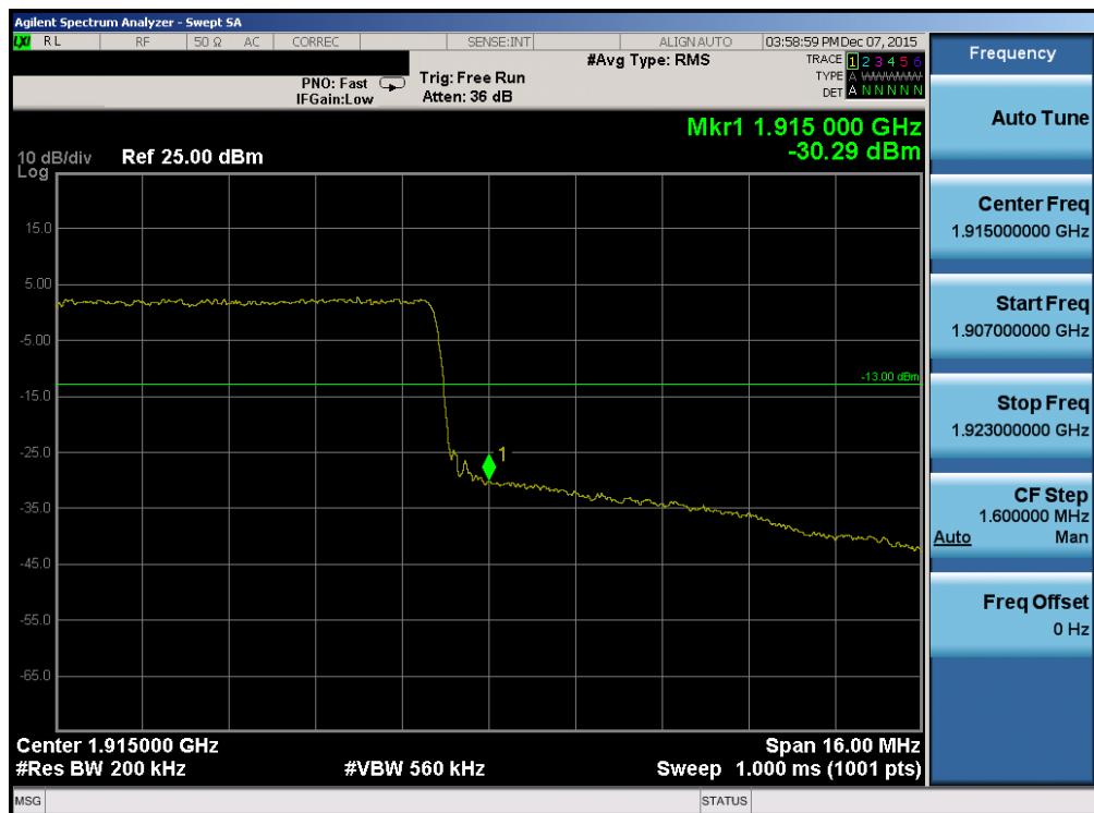
Plot 7-174. Upper Band Edge Plot (Band 2/25 – 20.0MHz QPSK – RB Size 100)
