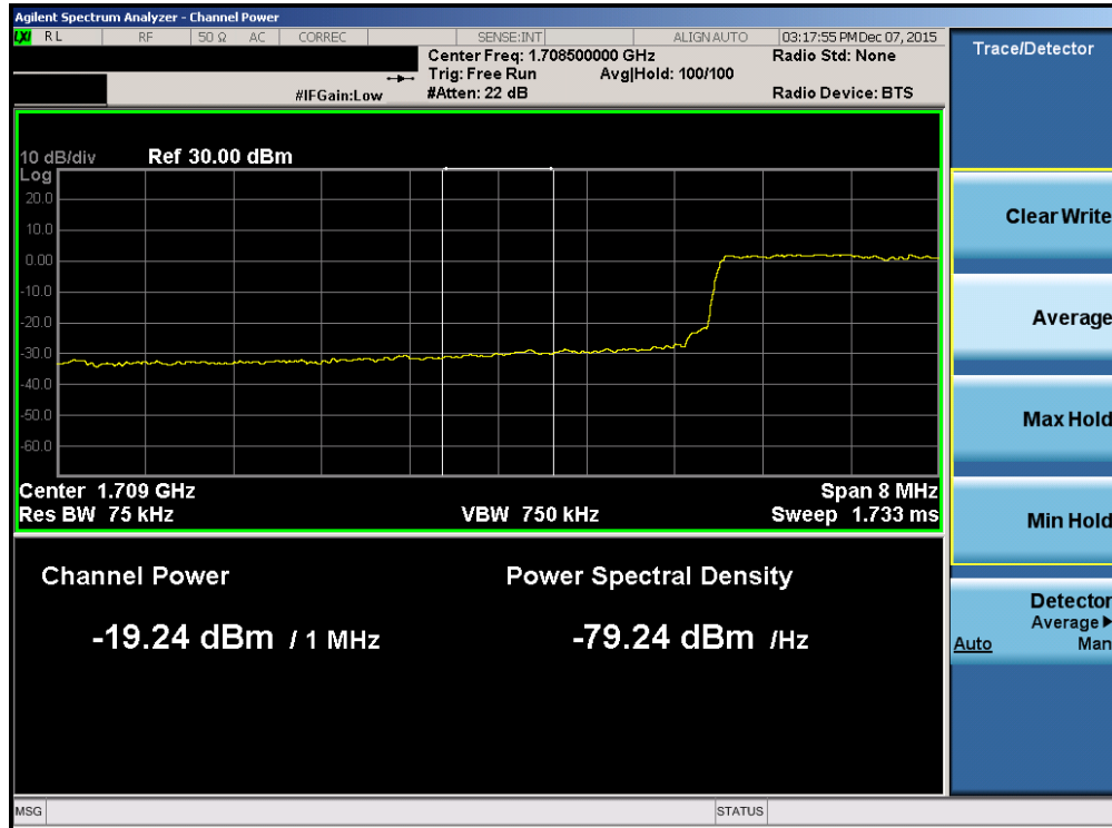
Plot 7-141. Lower Extended Band Edge Plot (Band 4 – 10.0MHz QPSK – RB Size 50)
