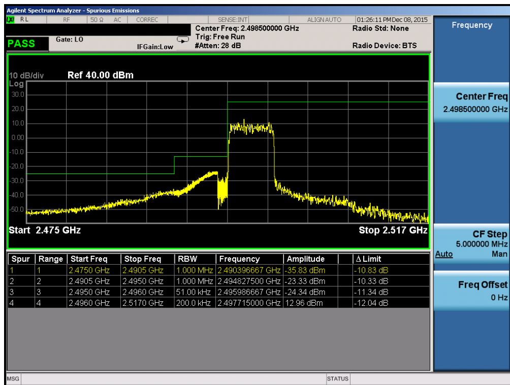
Plot 7-176. Lower ACP Plot (Band 41 – 5.0MHz QPSK – RB Size 25)
