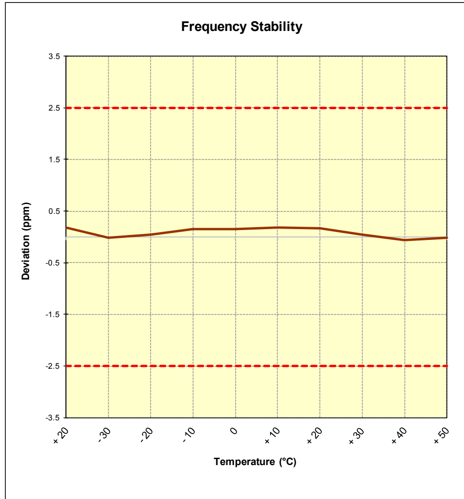
Figure 7-9. Frequency Stability Graph (Band 5/26)
