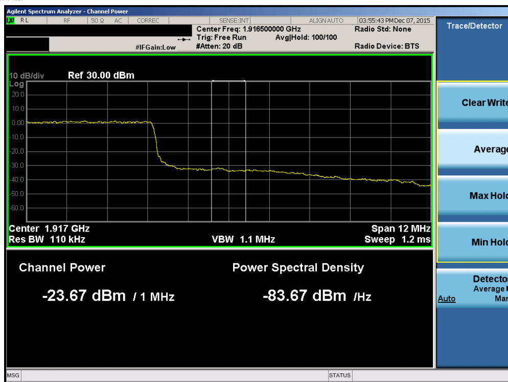
Plot 7-171. Upper Extended Band Edge Plot (Band 2/25 – 15.0MHz QPSK – RB Size 75)
