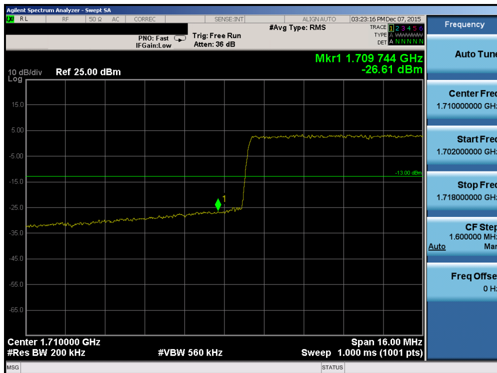
Plot 7-148. Lower Band Edge Plot (Band 4 – 20.0MHz QPSK – RB Size 100)
