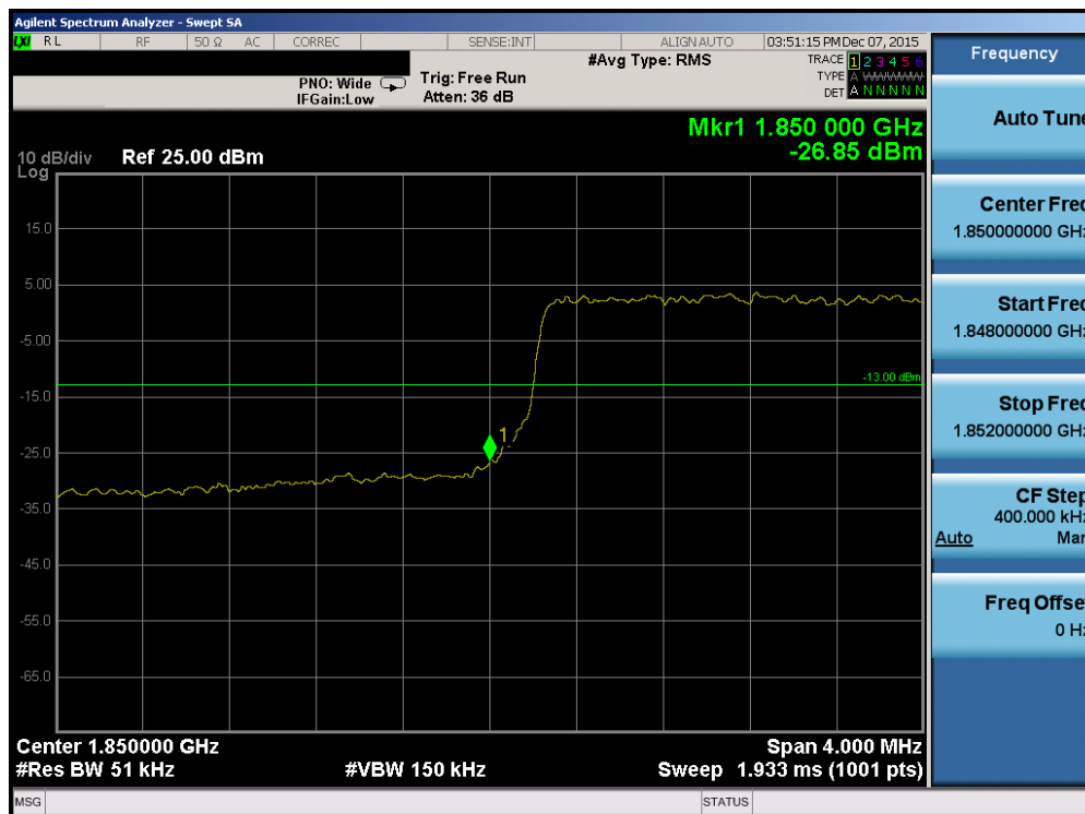
Plot 7-160. Lower Band Edge Plot (Band 2/25 – 5.0MHz QPSK – RB Size 25)
