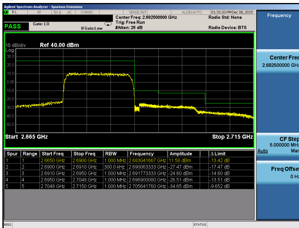
Plot 7-181. Upper ACP Plot (Band 41 – 15.0MHz QPSK – RB Size 75)
