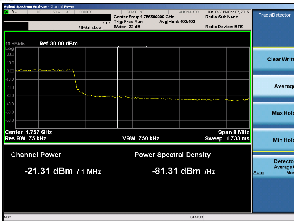
Plot 7-143. Upper Extended Band Edge Plot (Band 4 – 10.0MHz QPSK – RB Size 50)
