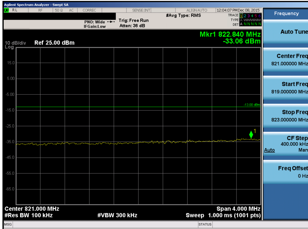
Plot 7-123. Lower Extended Band Edge Plot (Band 5/26 – 10.0MHz QPSK – RB Size 50)
