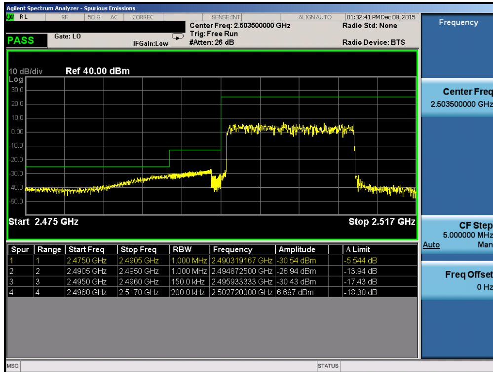
Plot 7-180. Lower ACP Plot (Band 41 – 15.0MHz QPSK – RB Size 75)
