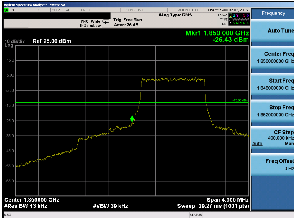
Plot 7-152. Lower Band Edge Plot (Band 2/25 – 1.4MHz QPSK – RB Size 6)
