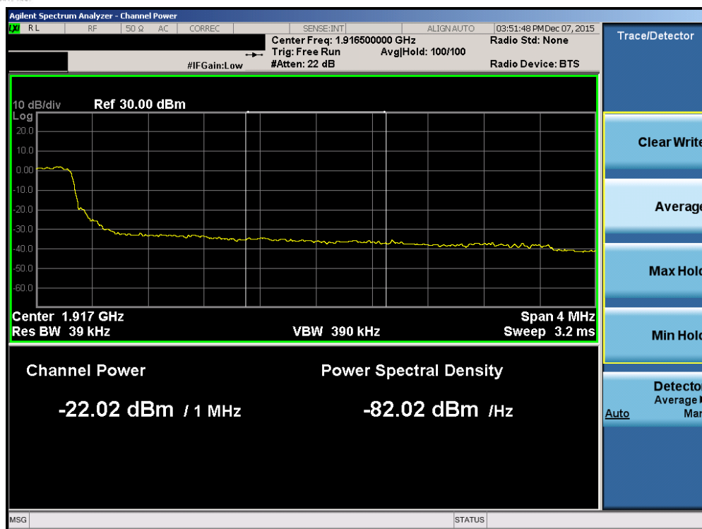
Plot 7-163. Upper Extended Band Edge Plot (Band 2/25 – 5.0MHz QPSK – RB Size 25)
