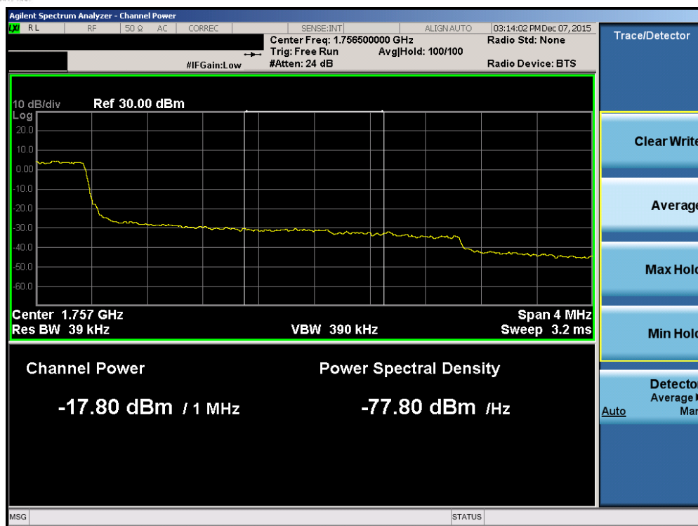
Plot 7-135. Upper Extended Band Edge Plot (Band 4 – 3.0MHz QPSK – RB Size 15)
