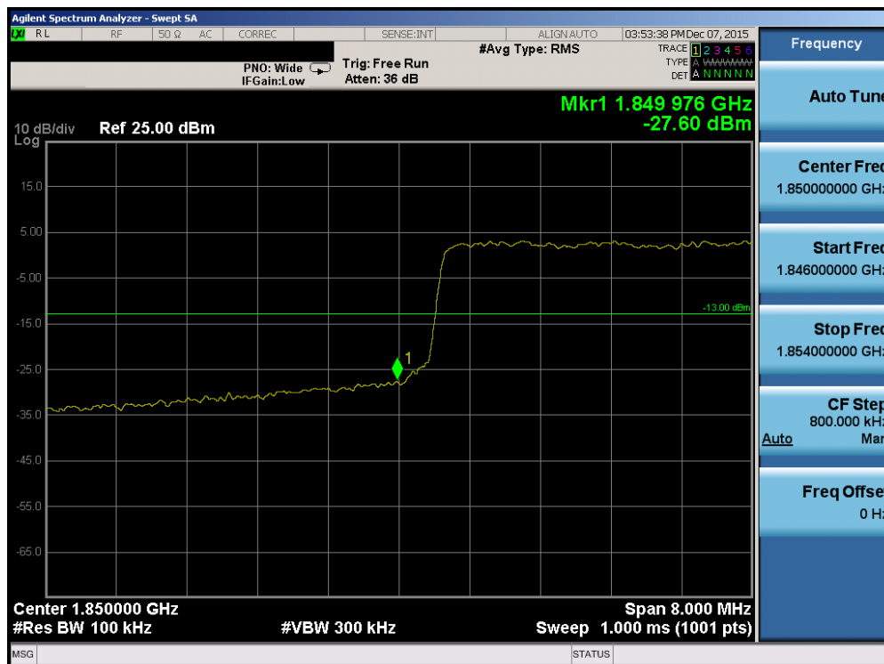
Plot 7-164. Lower Band Edge Plot (Band 2/25 – 10.0MHz QPSK – RB Size 50)
