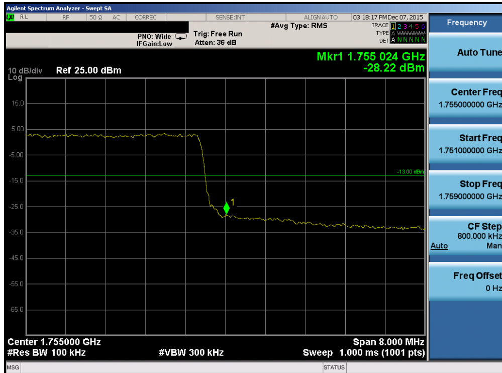
Plot 7-142. Upper Band Edge Plot (Band 4 – 10.0MHz QPSK – RB Size 50)
