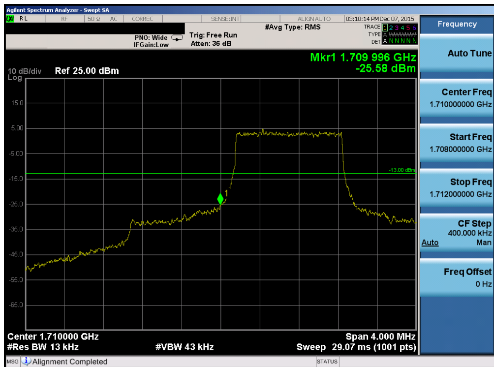
Plot 7-128. Lower Band Edge Plot (Band 4 – 1.4MHz QPSK – RB Size 6)
