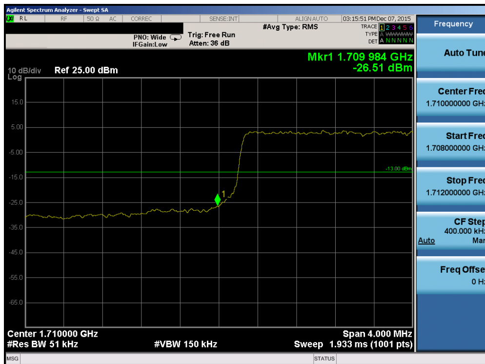
Plot 7-136. Lower Band Edge Plot (Band 4 – 5.0MHz QPSK – RB Size 25)
