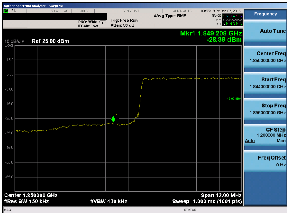
Plot 7-168. Lower Band Edge Plot (Band 2/25 – 15.0MHz QPSK – RB Size 75)
