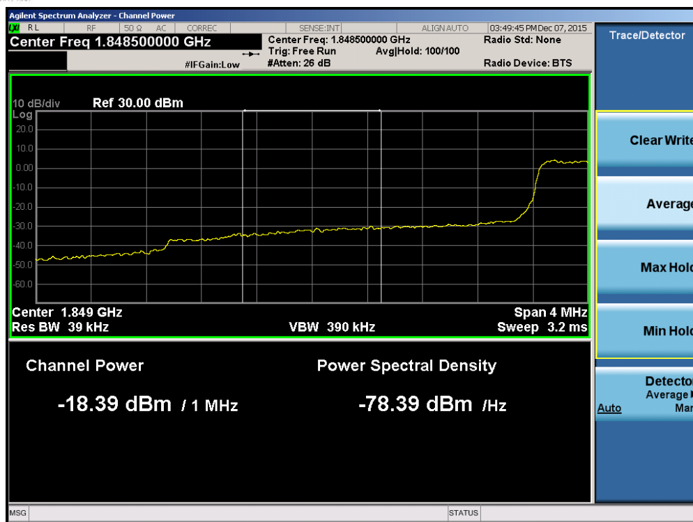
Plot 7-157. Lower Extended Band Edge Plot (Band 2/25 – 3.0MHz QPSK – RB Size 15)
