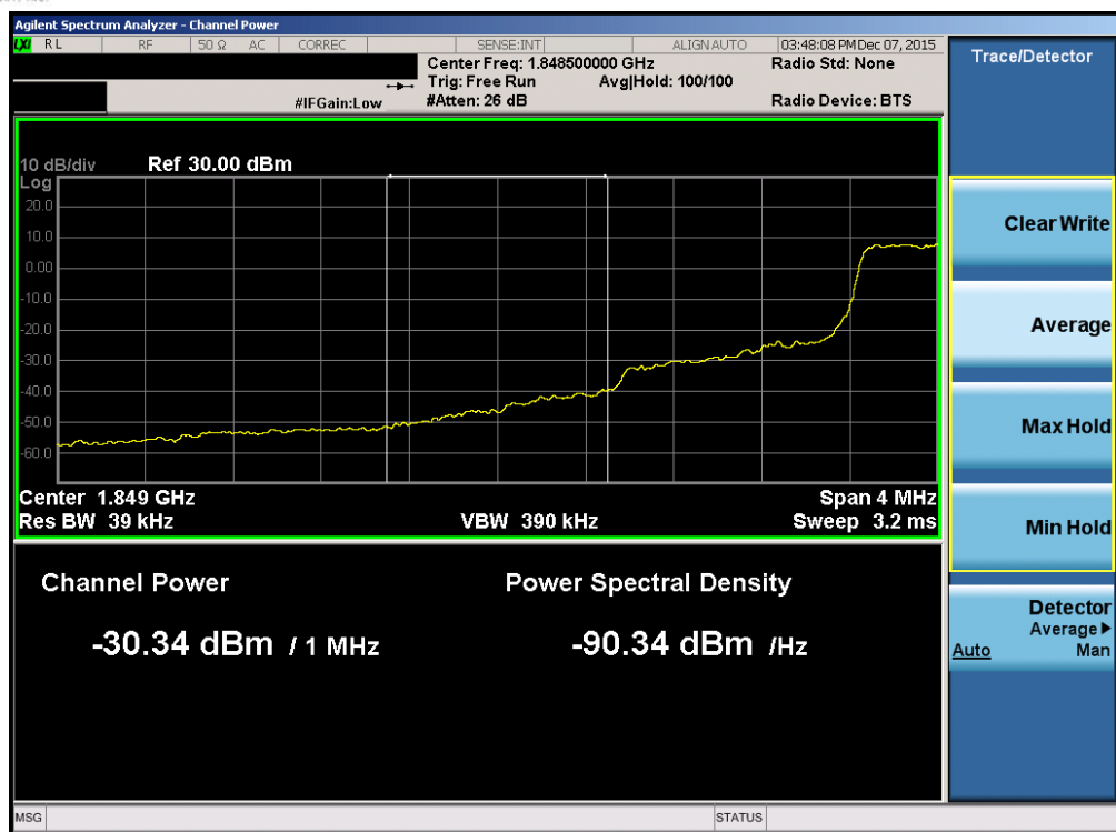
Plot 7-153. Lower Extended Band Edge Plot (Band 2/25 – 1.4MHz QPSK – RB Size 6)
