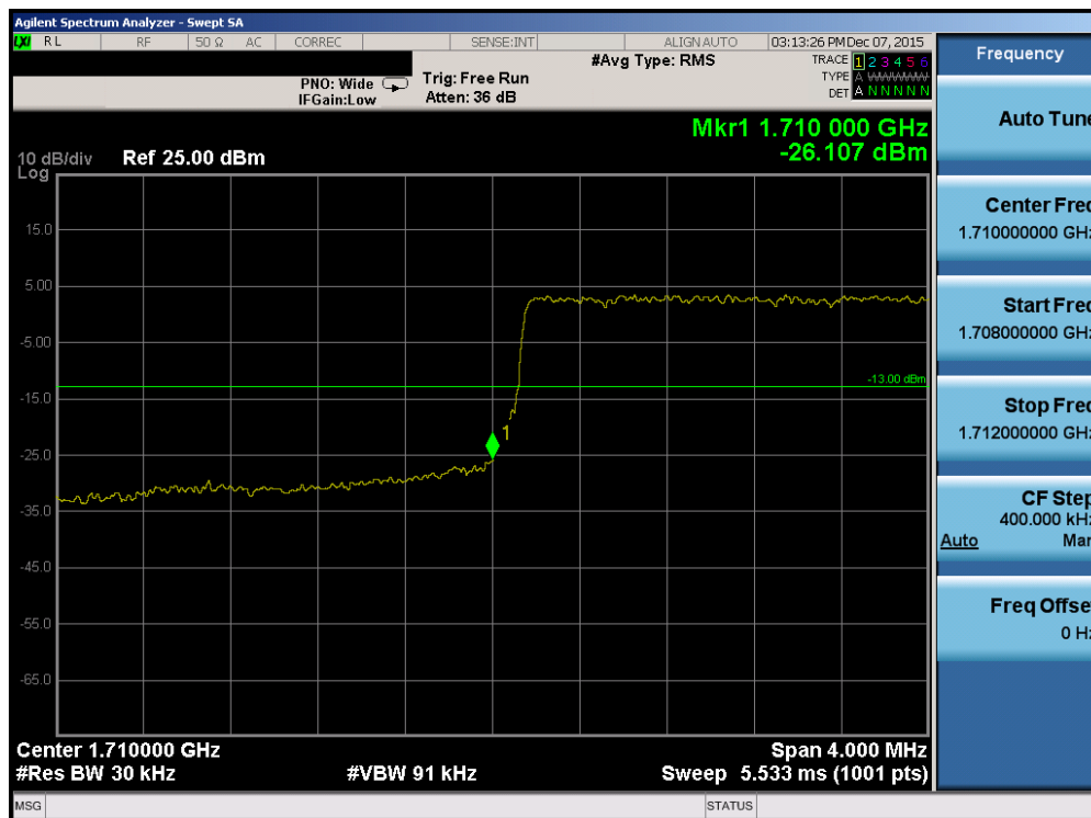
Plot 7-132. Lower Band Edge Plot (Band 4 – 3.0MHz QPSK – RB Size 15)
