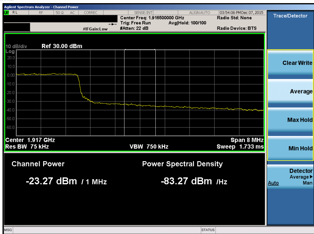
Plot 7-167. Upper Extended Band Edge Plot (Band 2/25 – 10.0MHz QPSK – RB Size 50)
