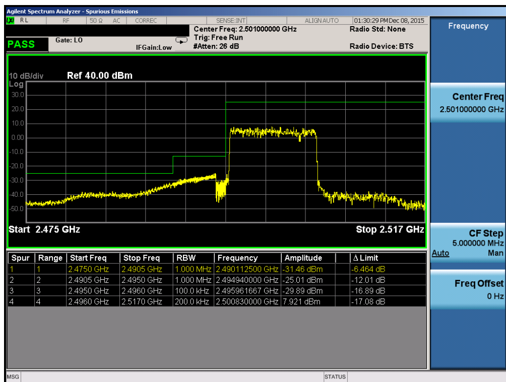
Plot 7-178. Lower ACP Plot (Band 41 – 10.0MHz QPSK – RB Size 50)
