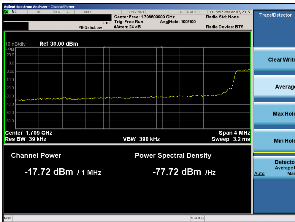
Plot 7-137. Lower Extended Band Edge Plot (Band 4 – 5.0MHz QPSK – RB Size 25)
