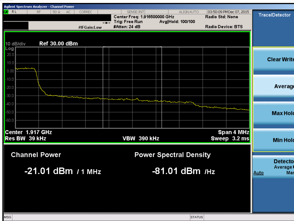
Plot 7-159. Upper Extended Band Edge Plot (Band 2/25 – 3.0MHz QPSK – RB Size 15)
