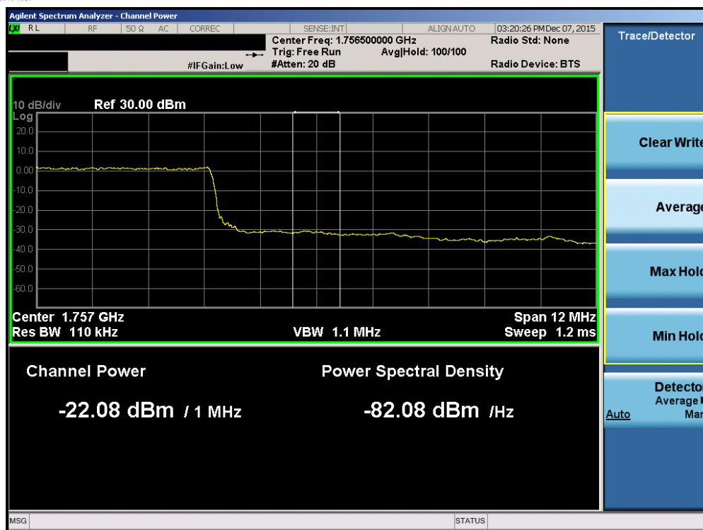
Plot 7-147. Upper Extended Band Edge Plot (Band 4 – 15.0MHz QPSK – RB Size 75)
