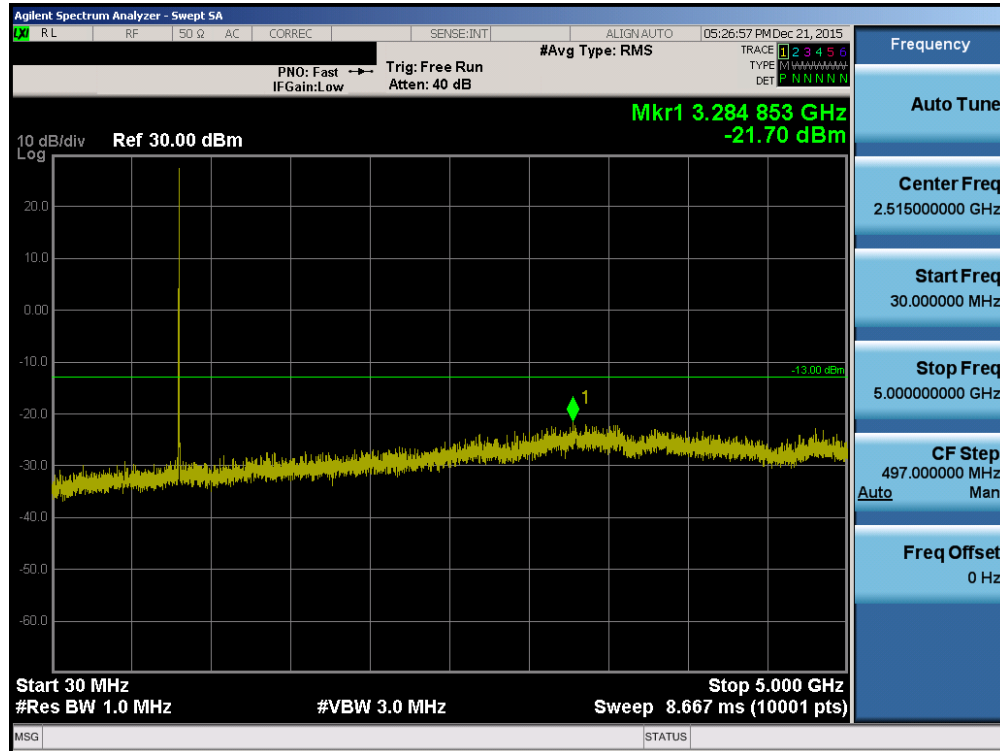
Plot 7-13. Conducted Spurious Plot (CDMA Ch. 684)
