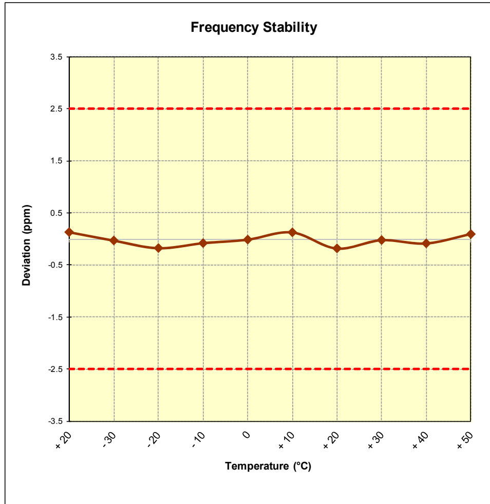
Figure 7-5. CDMA BC10 Frequency Stability Graph (Ch. 476)
