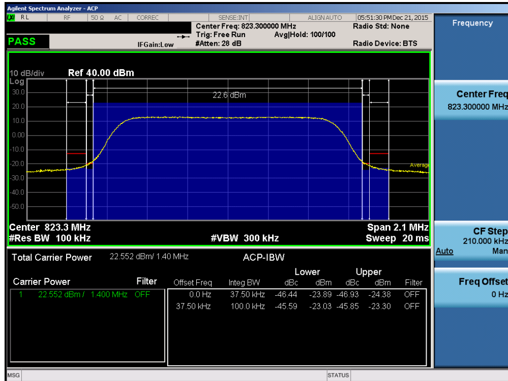
Plot 7-22. Channel Edge Plot (LTE Band 26 1.4MHz QPSK – RB Size 6 – High Channel)
