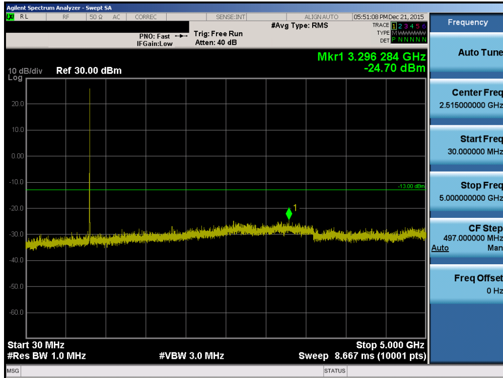
Plot 7-17. Conducted Spurious Plot (LTE Band 26 10MHz QPSK – RB Size 1, RB Offset 0 – High Channel)
