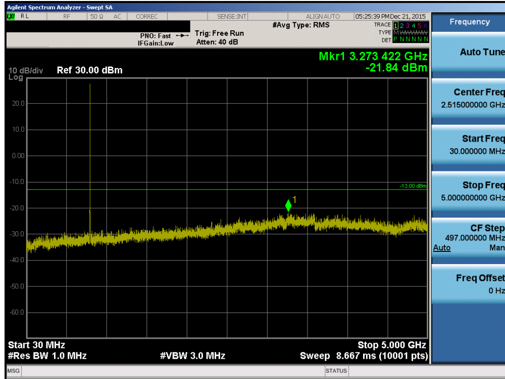
Plot 7-11. Conducted Spurious Plot (CDMA Ch. 476)
