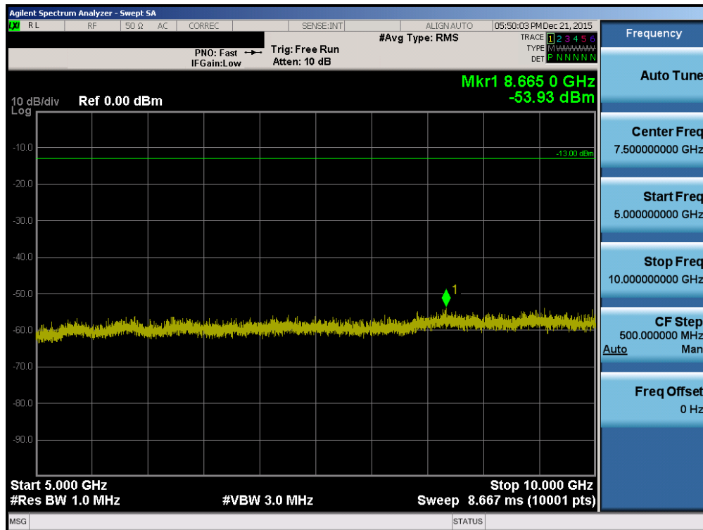
Plot 7-16. Conducted Spurious Plot (LTE Band 26 10MHz QPSK – RB Size 1, RB Offset 0 – Low Channel)
