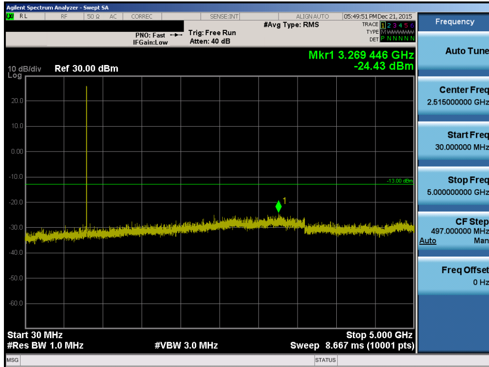
Plot 7-15. Conducted Spurious Plot (LTE Band 26 10MHz QPSK – RB Size 1, RB Offset 0 – Low Channel)
