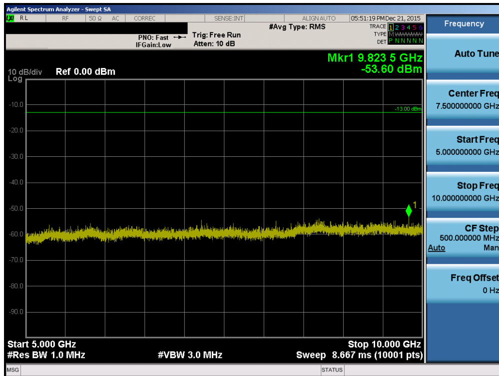
Plot 7-18. Conducted Spurious Plot (LTE Band 26 10MHz QPSK – RB Size 1, RB Offset 0 – High Channel)
