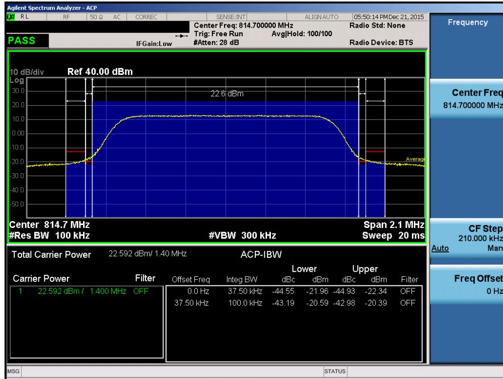
Plot 7-21. Channel Edge Plot (LTE Band 26 1.4MHz QPSK – RB Size 6– Low Channel)
