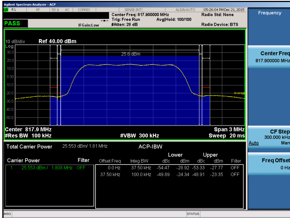
Plot 7-19. Channel Edge Plot (CDMA Ch. 476)
