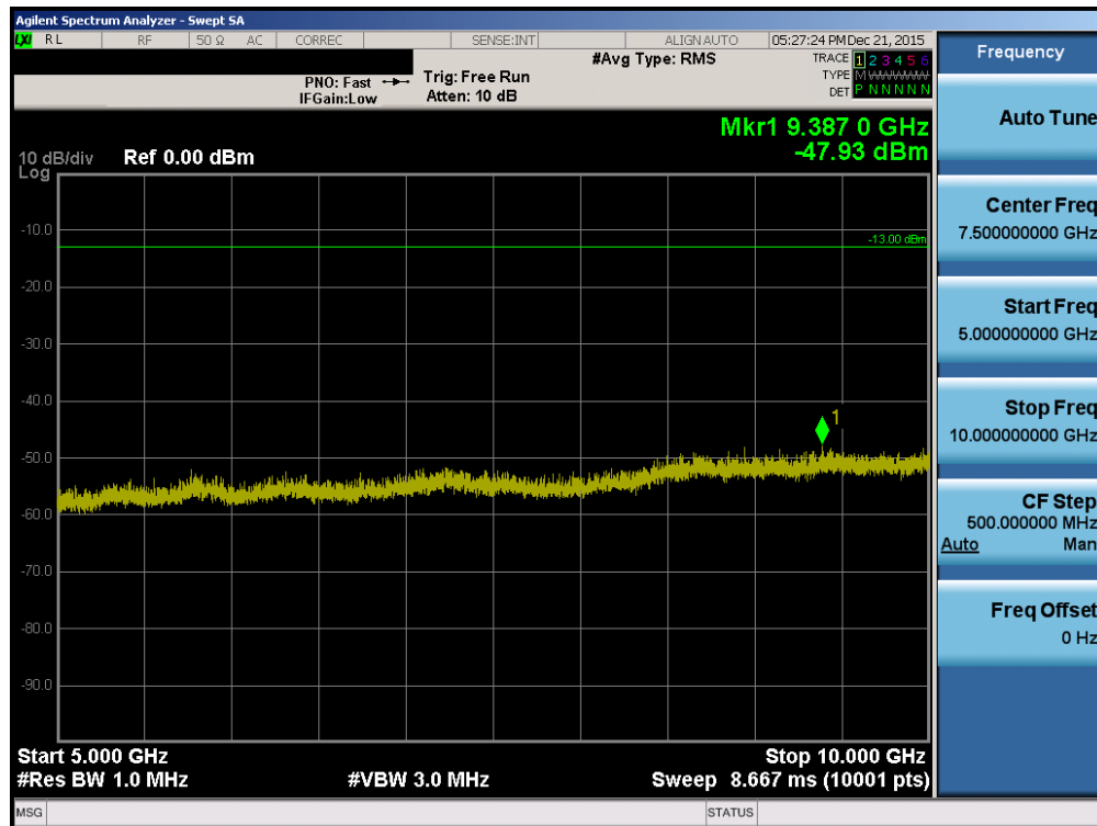
Plot 7-14. Conducted Spurious Plot (CDMA Ch. 684)
