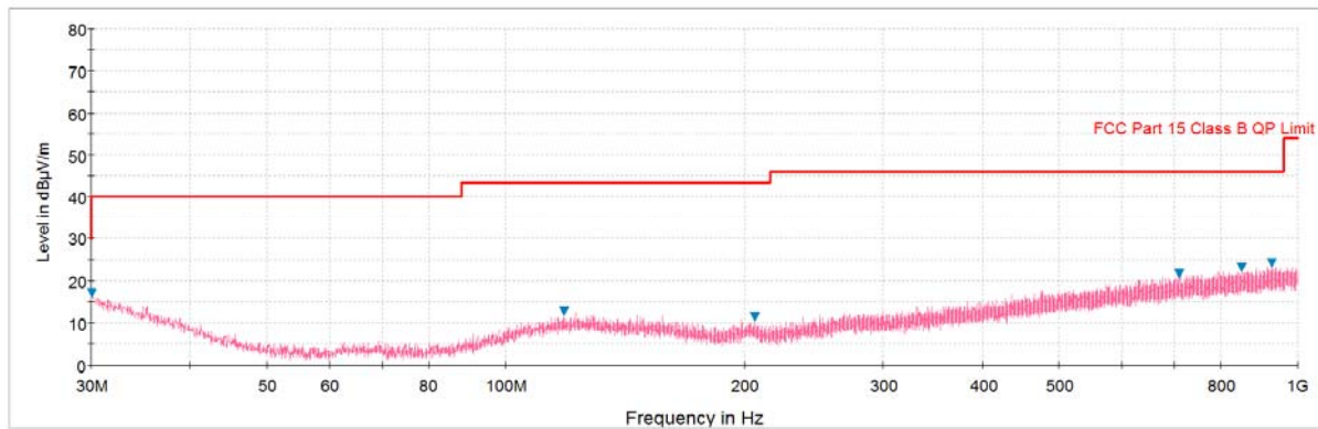
Plot 7-49. Radiated Spurious Plot below 1GHz (Pol. V)
