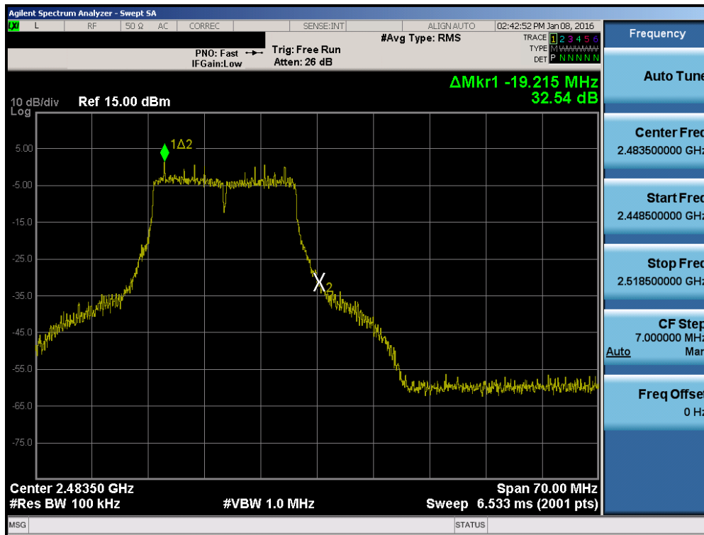
Plot 7-27. Band Edge Plot (802.11n (2.4GHz) – Ch. 13)
