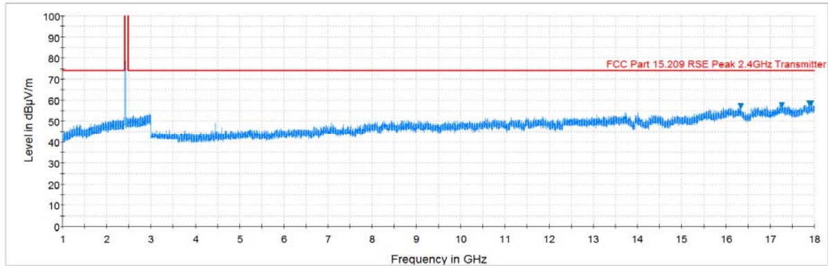
Plot 7-34. Radiated Spurious Plot above 1GHz (802.11b – Ch. 1, Ant. Pol. H)
