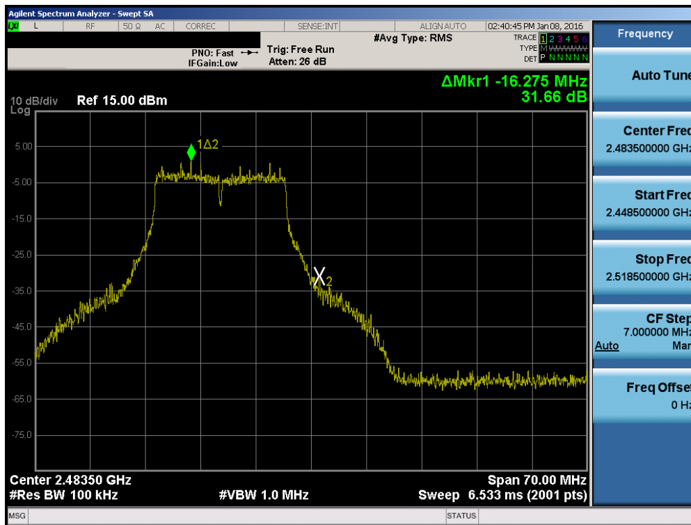
Plot 7-24. Band Edge Plot (802.11g – Ch. 13)
