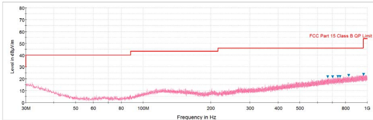
Plot 7-48. Radiated Spurious Plot below 1GHz (Pol. H)
