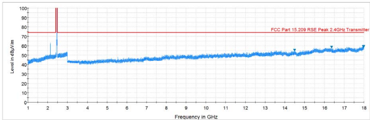
Plot 7-38. Radiated Spurious Plot above 1GHz (802.11b – Ch. 11, Ant. Pol. H)
