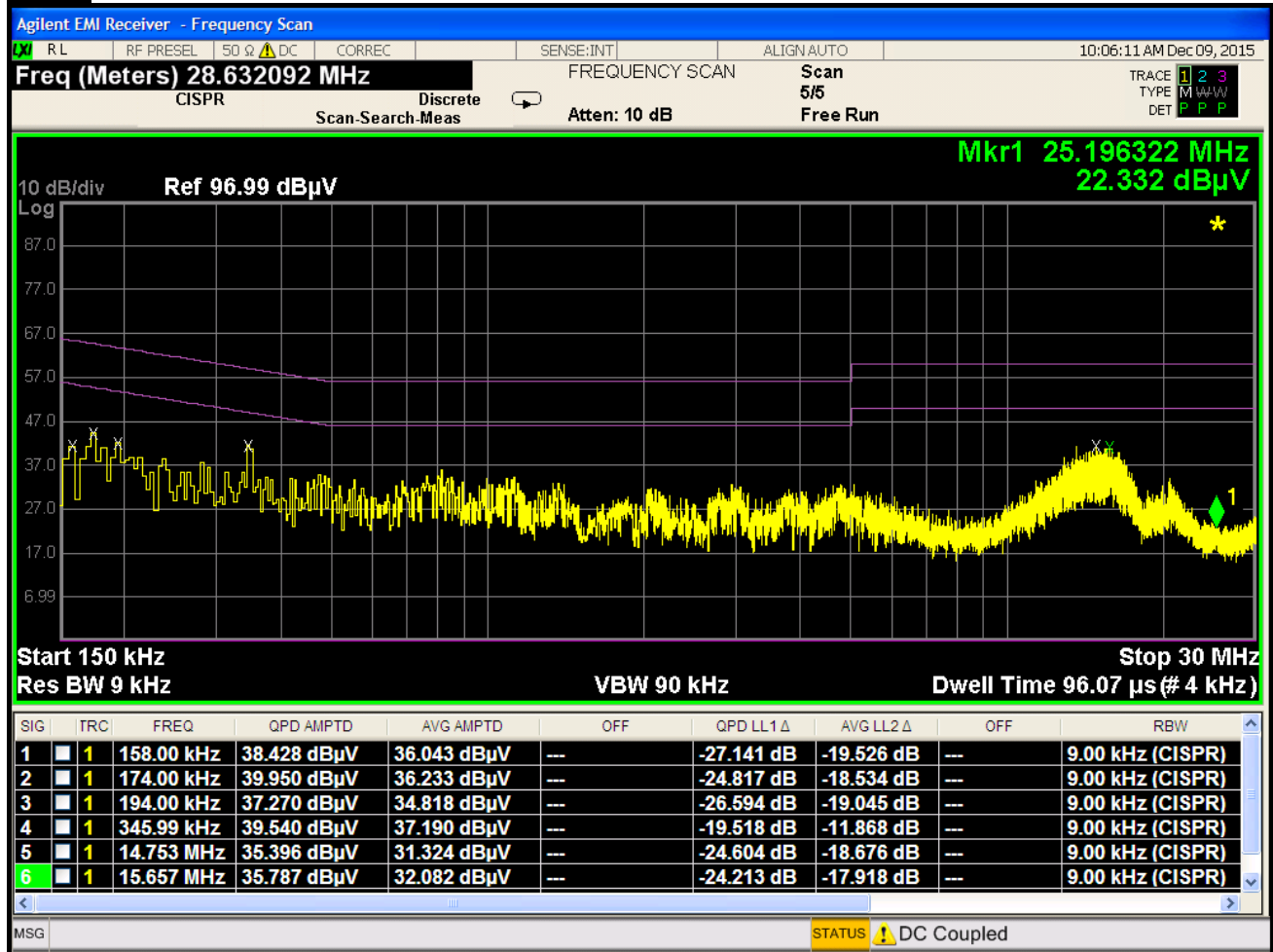
Plot 7-51. Line Conducted Plot with 802.11b (N)
