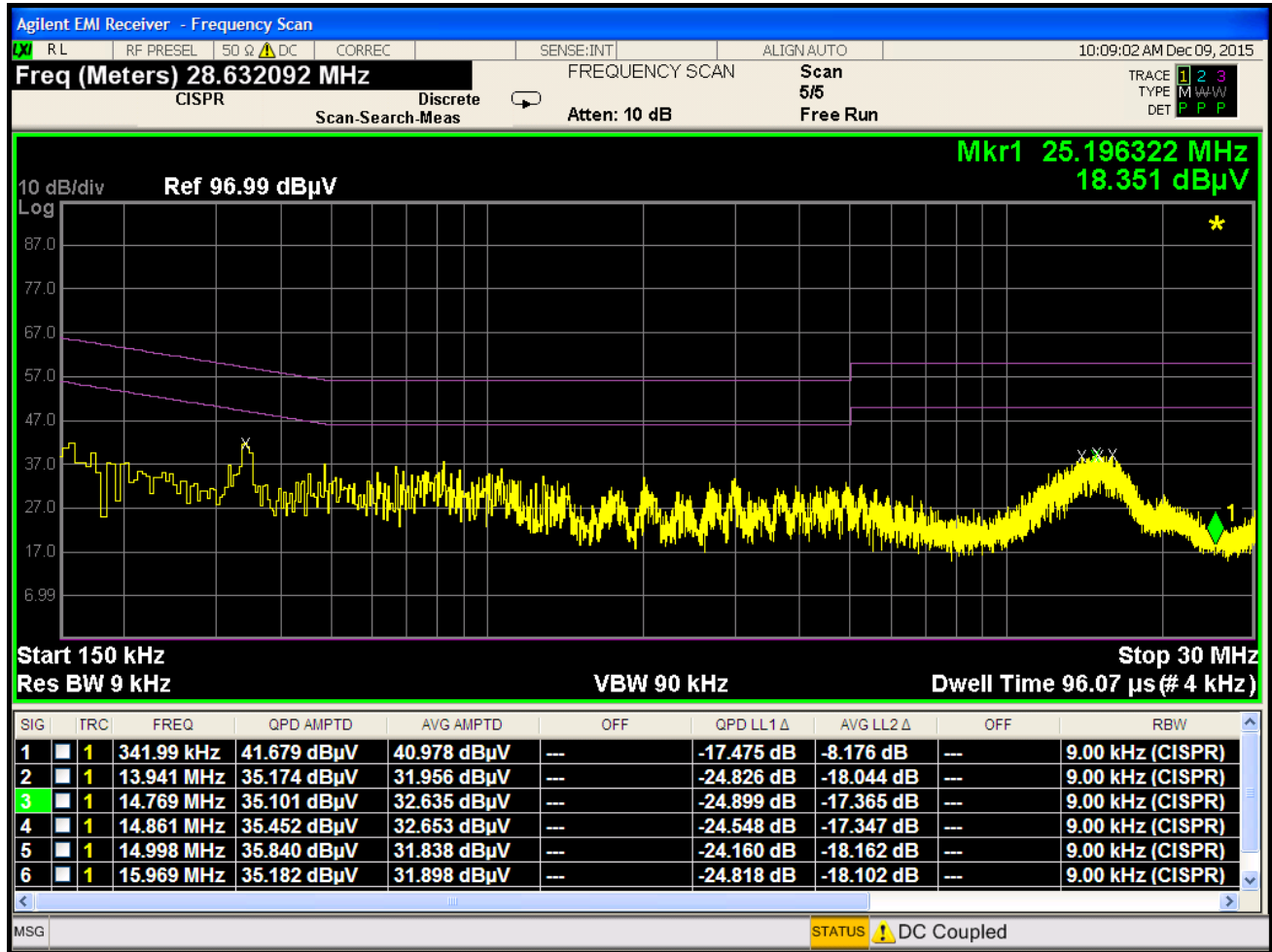
Plot 7-50. Line Conducted Plot with 802.11b (L1)
