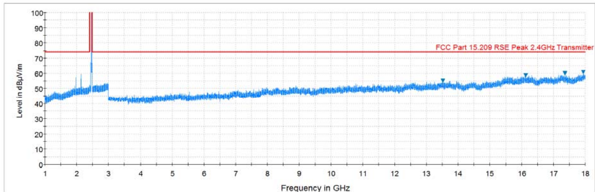
Plot 7-39. Radiated Spurious Plot above 1GHz (802.11b – Ch. 11, Ant. Pol. V)
