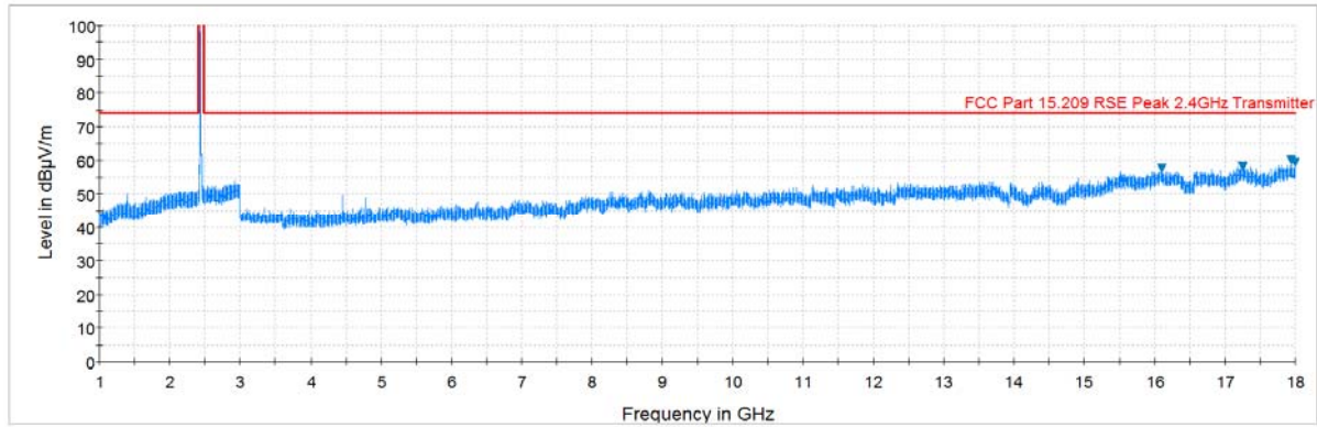
Plot 7-37. Radiated Spurious Plot above 1GHz (802.11b – Ch. 6, Ant. Pol. V)
