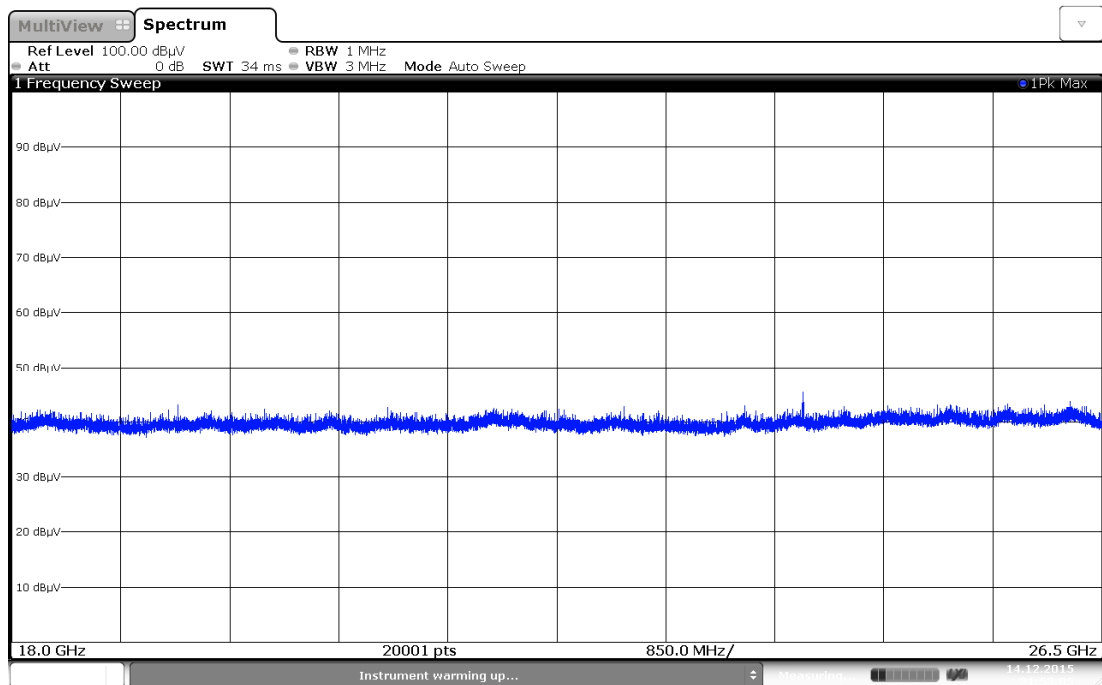
Plot 7-41. Radiated Spurious Plot above 18GHz (Pol. V)
