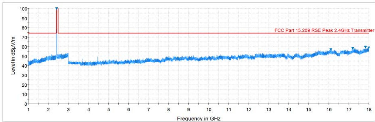
Plot 7-35. Radiated Spurious Plot above 1GHz (802.11b – Ch. 1, Ant. Pol. V)
