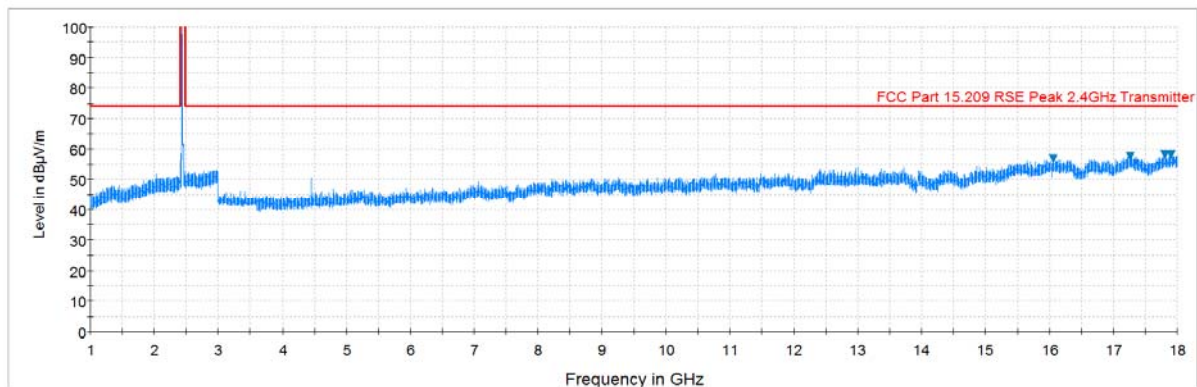
Plot 7-36. Radiated Spurious Plot above 1GHz (802.11b – Ch. 6, Ant. Pol. H)
