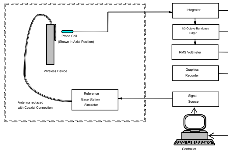
Figure 5-12 Audio Magnetic Field Test Setup
