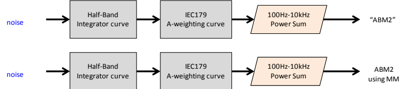
Figure 5-8 ABM2 Validation Block Diagram
