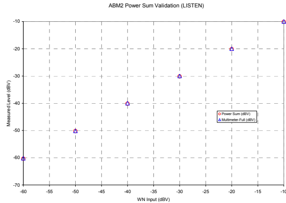
Figure 5-9 ABM2 Power Sum Validation
