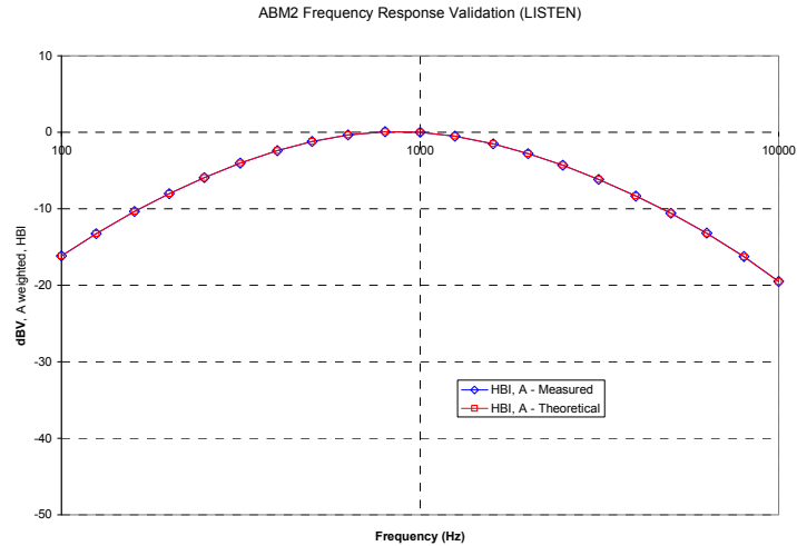
Figure 5-7 ABM2 Frequency Response Validation
