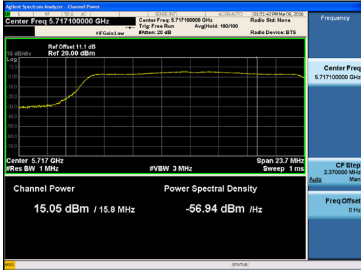
802.11ac UNII 2C Band Average Power CH.144
