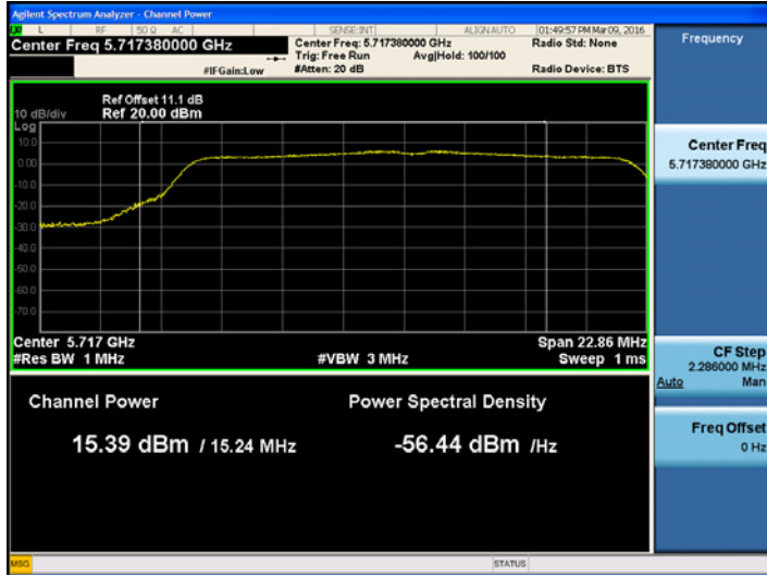
802.11n_20MHz BW UNII 2C Band Average Power CH.144
