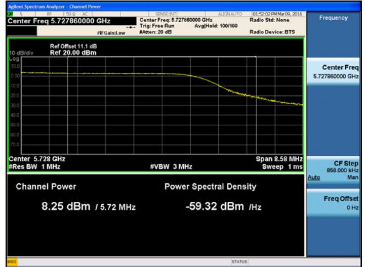
802.11ac UNII 3 Band Average Power CH.144
