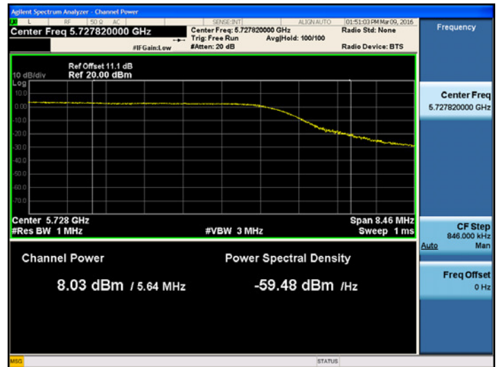
802.11n_20MHz BW UNII 3 Band Average Power CH.144
