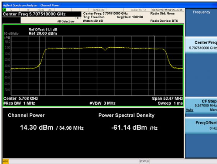
802.11ac_40MHz BW UNII 2C Band Average Power CH.142
