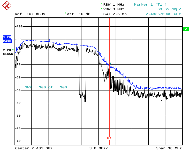
Radiated Restricted Band Edges plot – Peak Reading (802.11n Ch.13)
