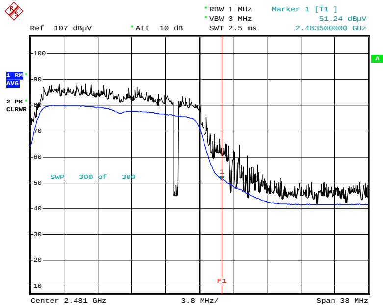
Radiated Restricted Band Edges plot – Average Reading (802.11n Ch.13)
