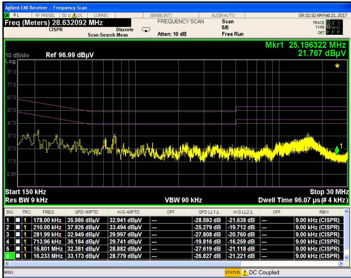
Plot 7-20. Line Conducted Plot with Bluetooth LE (L1)
