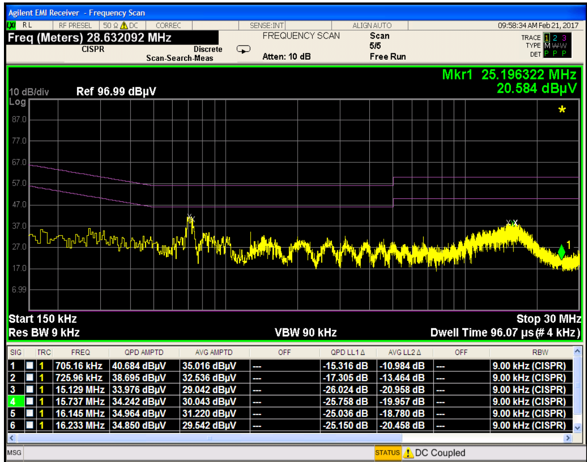
Plot 7-21. Line Conducted Plot with Bluetooth LE (N)
