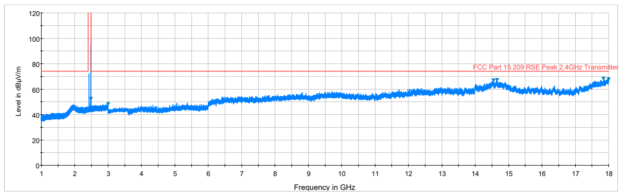
Plot 7-46. Radiated Spurious Plot above 1GHz (BT – Ch. 78, Ant. Pol. H)
