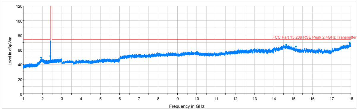
Plot 7-42. Radiated Spurious Plot above 1GHz (BT – Ch. 0, Ant. Pol. H)
