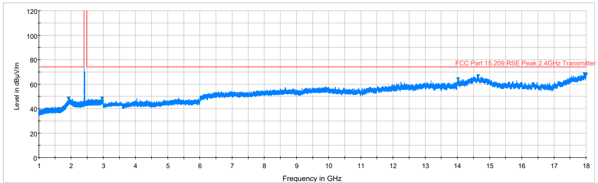
Plot 7-43. Radiated Spurious Plot above 1GHz (BT – Ch. 0, Ant. Pol. V)
