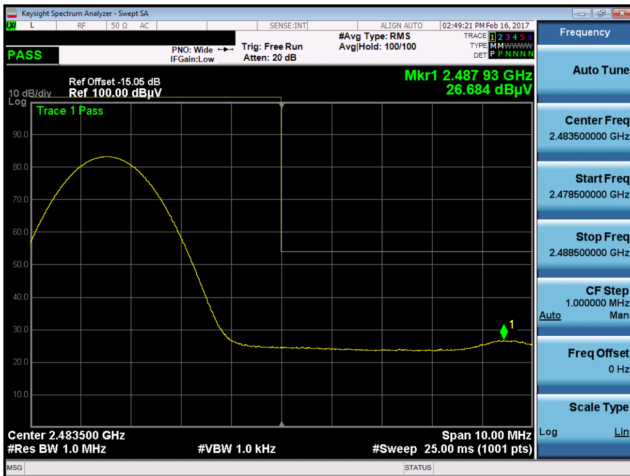
Plot 7-50. Radiated Restricted Upper Band Edge Measurement (Average)
