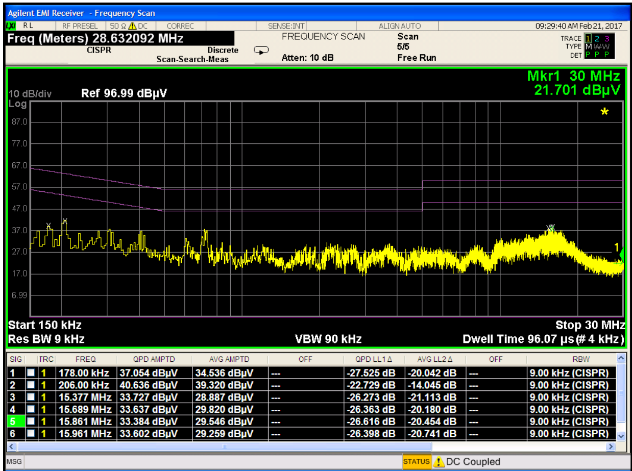
Plot 7-52. Line-Conducted Test Plot (L1)
