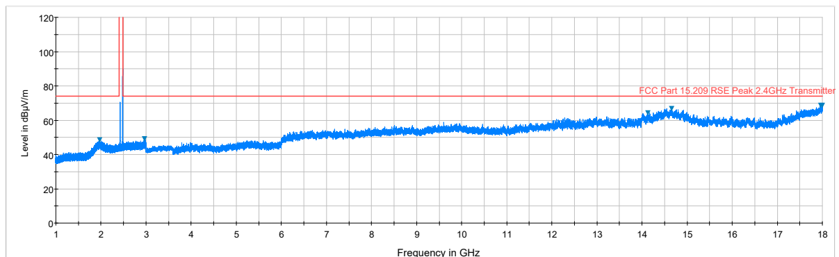
Plot 7-47. Radiated Spurious Plot above 1GHz (BT – Ch. 78, Ant. Pol. V)
