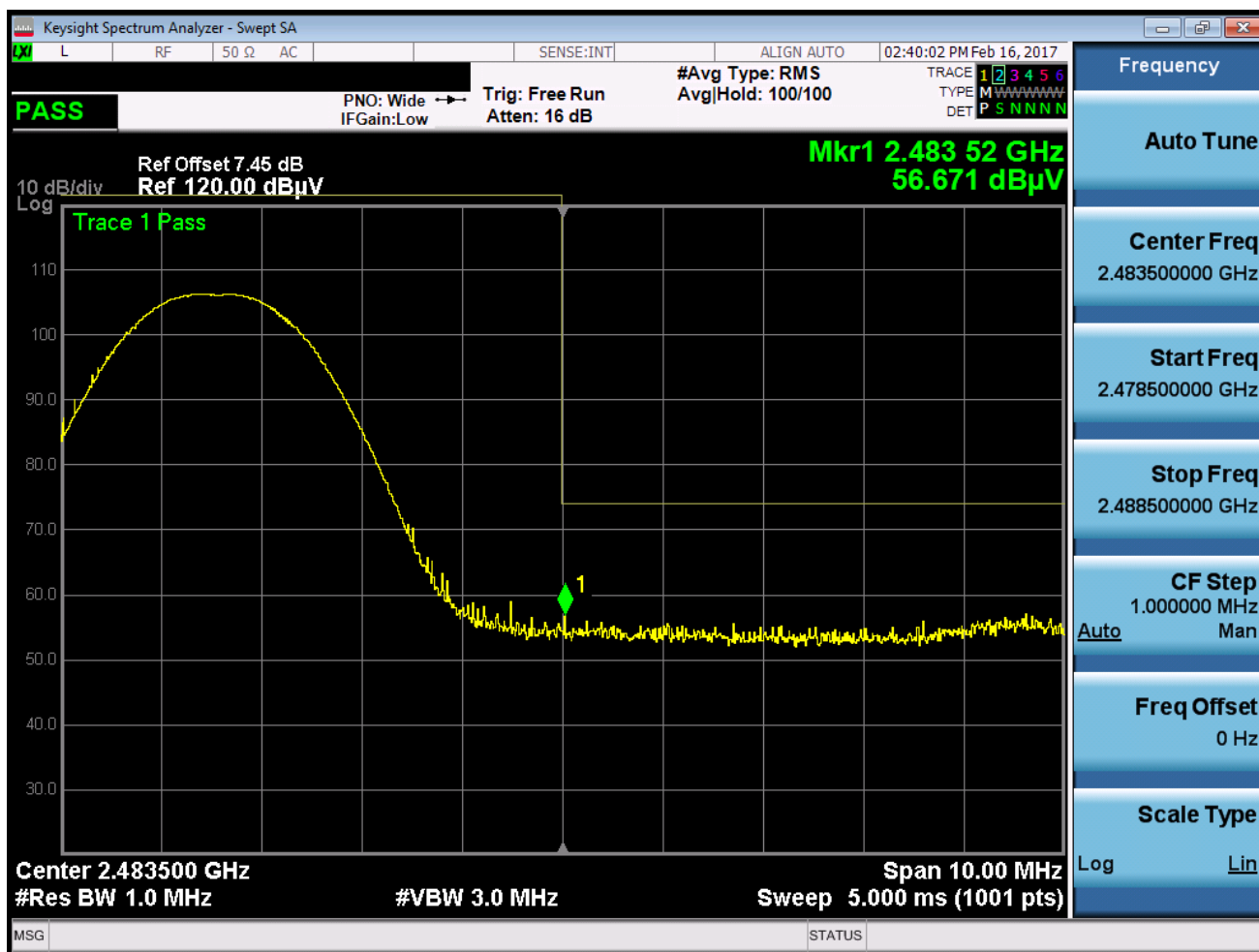
Plot 7-51. Radiated Restricted Upper Band Edge Measurement (Peak)
