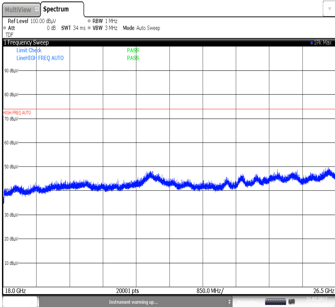
Plot 7-49. Radiated Spurious Plot above 18GHz (Pol. V)
