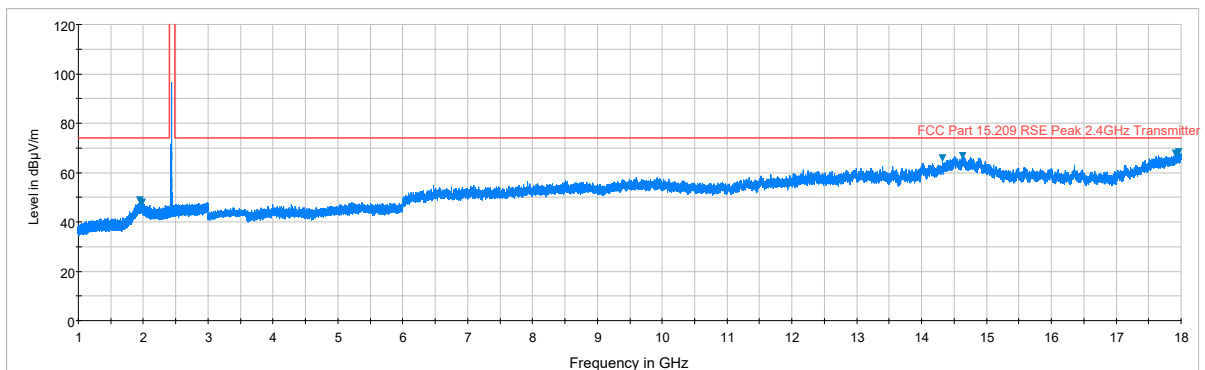
Plot 7-44. Radiated Spurious Plot above 1GHz (BT – Ch. 39, Ant. Pol. H)
