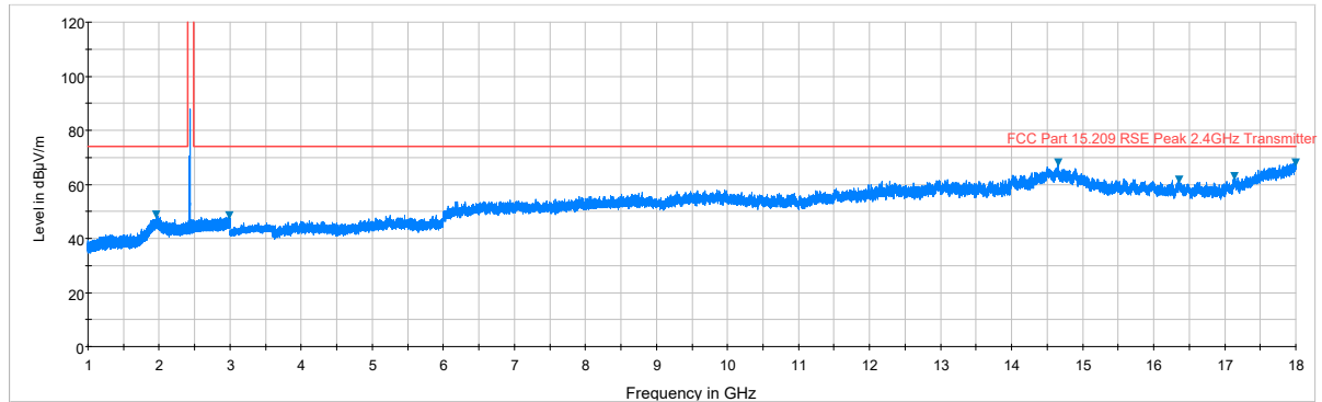
Plot 7-45. Radiated Spurious Plot above 1GHz (BT – Ch. 39, Ant. Pol. V)
