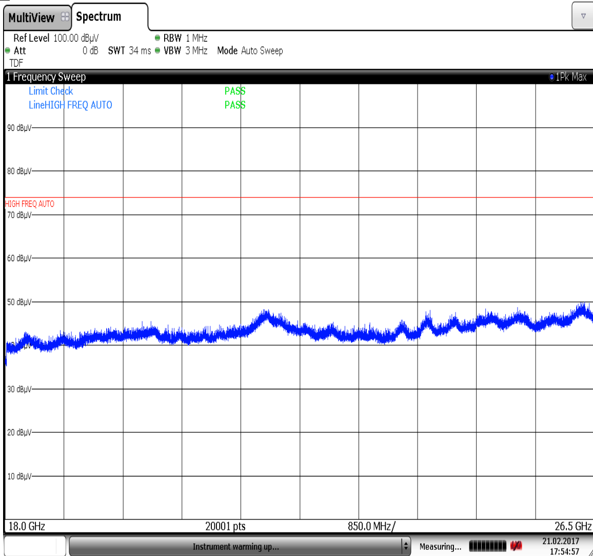
Plot 7-48. Radiated Spurious Plot above 18GHz (Pol. H)
