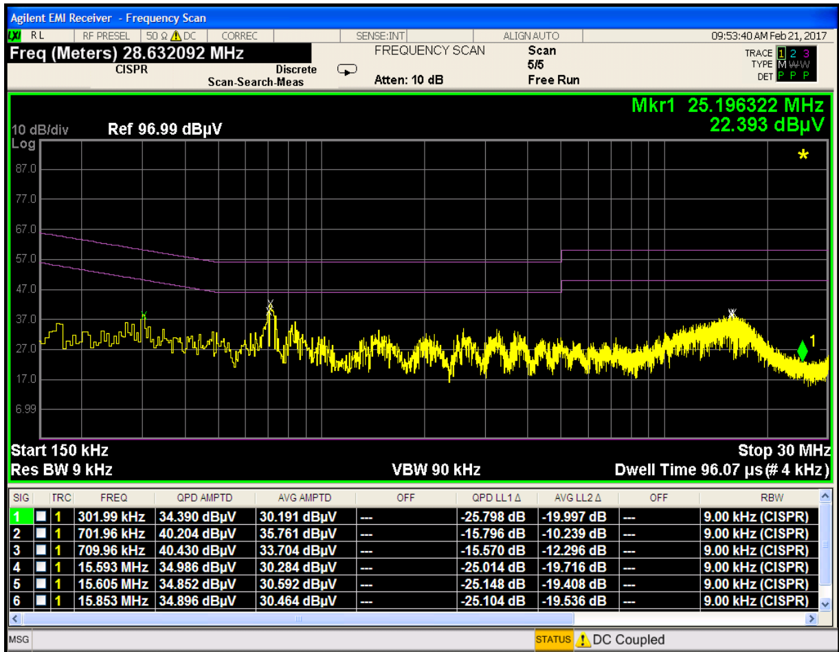
Plot 7-53. Line-Conducted Test Plot (N)
