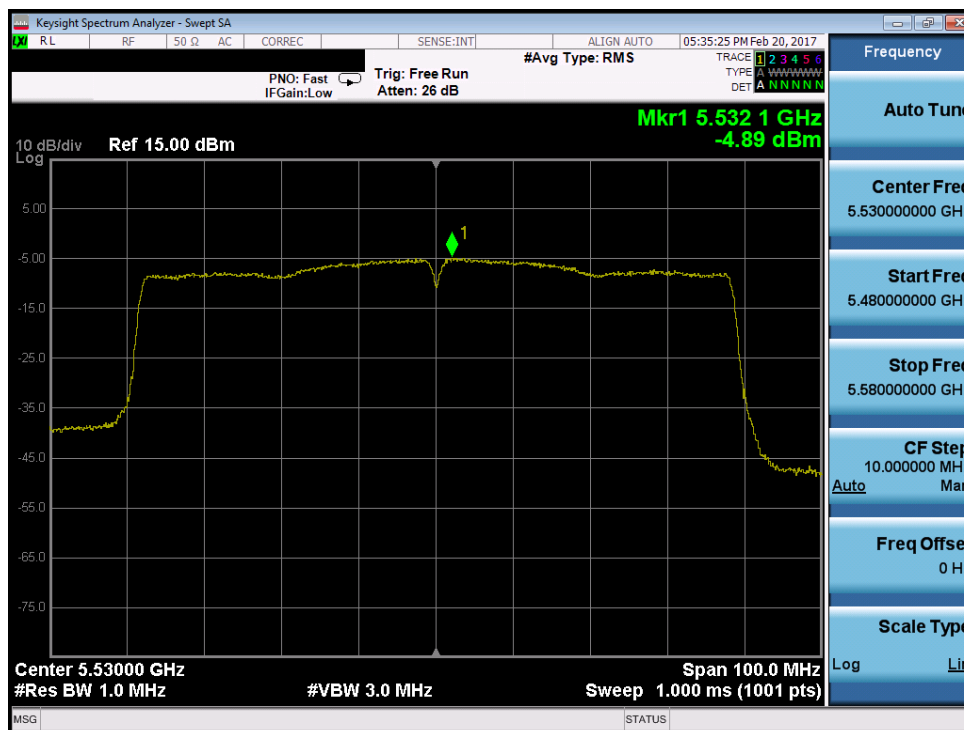
Plot 7-67. Power Spectral Density Plot (80MHz BW 802.11a/n/ac (UNII Band 2C) – Ch. 106)
