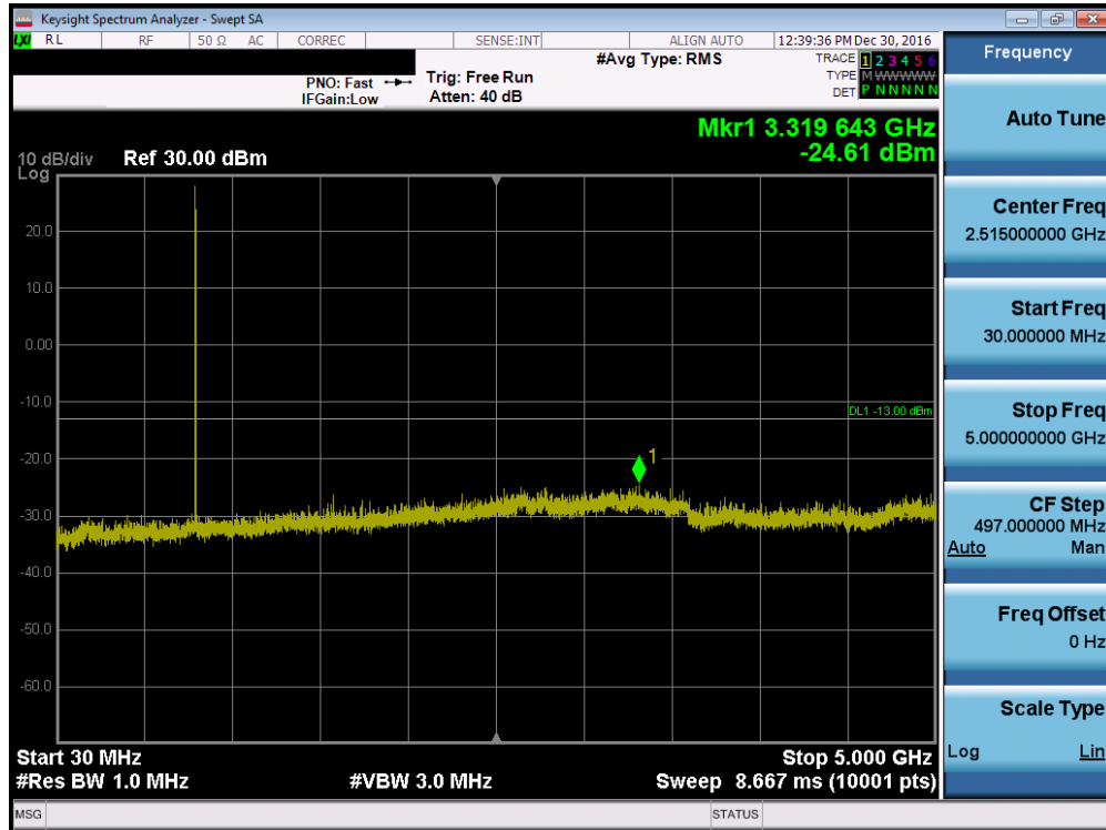
Plot 7-17. Conducted Spurious (LTE Band 26, 5MHz QPSK – RB Size 1, RB Offset 0 – Low Channel)
