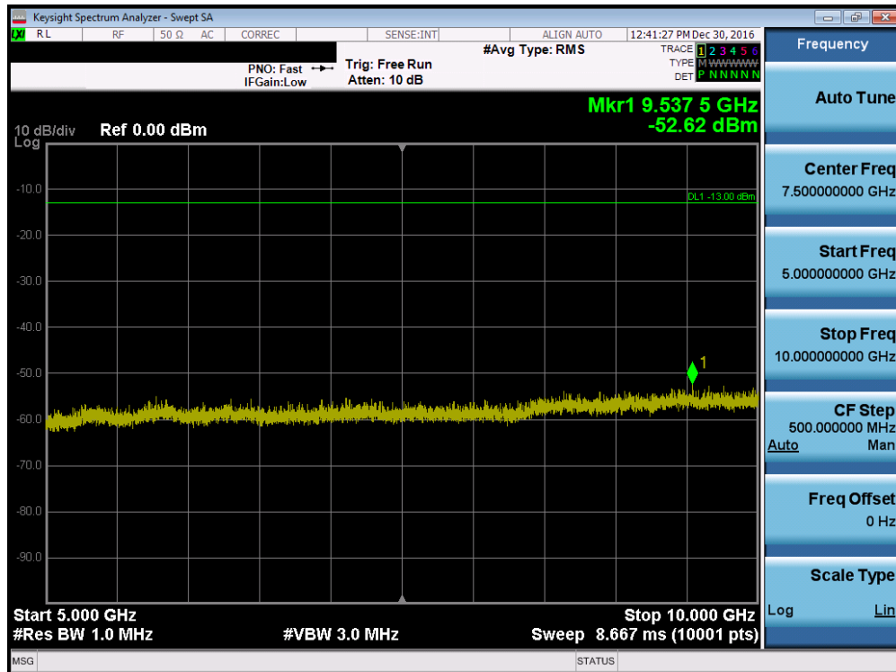
Plot 7-20. Conducted Spurious (LTE Band 26, 5MHz QPSK – RB Size 1, RB Offset 0 – High Channel)
