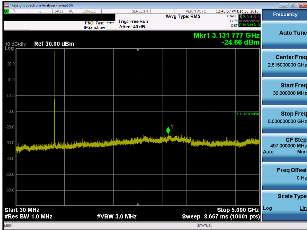
Plot 7-19. Conducted Spurious (LTE Band 26, 5MHz QPSK – RB Size 1, RB Offset 0 – High Channel)
