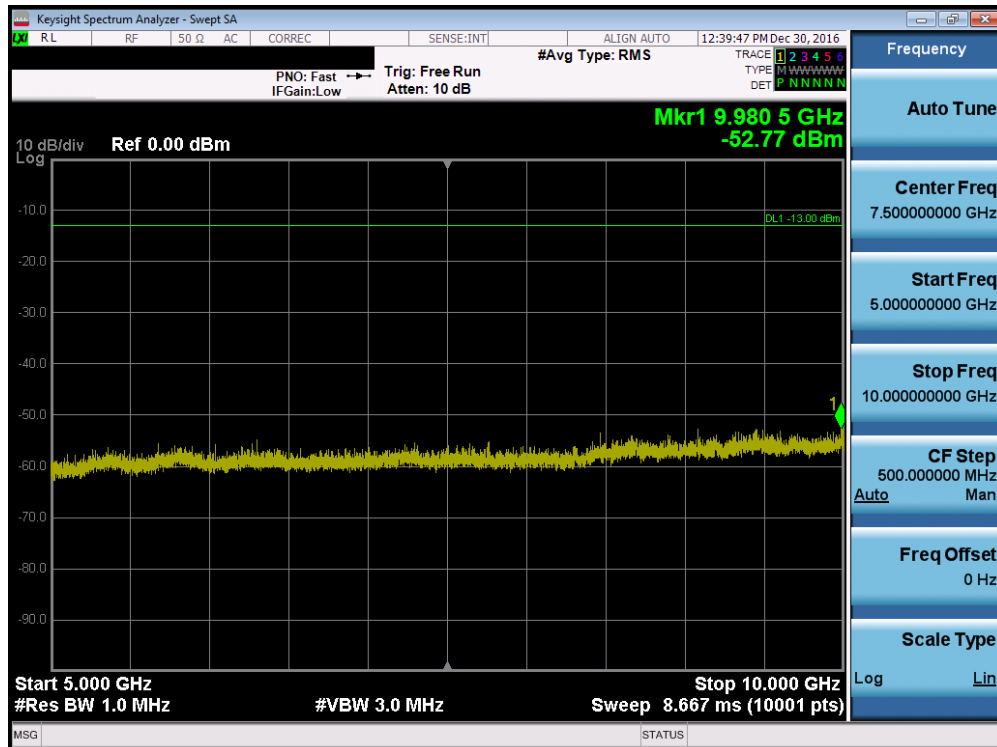
Plot 7-18. Conducted Spurious (LTE Band 26, 5MHz QPSK – RB Size 1, RB Offset 0 – Low Channel)
