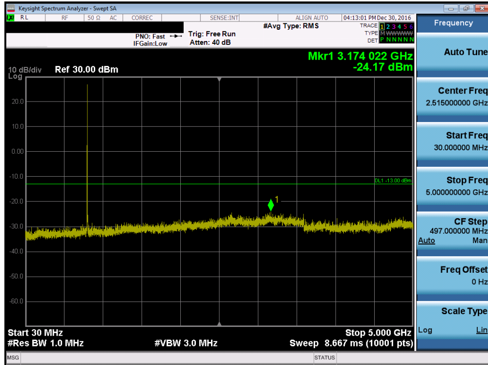
Plot 7-15. Conducted Spurious Plot (CDMA, Ch. 684)
