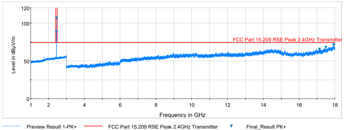
Plot 7-42. Radiated Spurious Plot above 1GHz (BT – Ch. 39, Ant. Pol. H)
