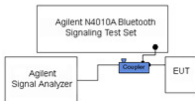
Figure 7-5. Test Instrument & Measurement Setup
