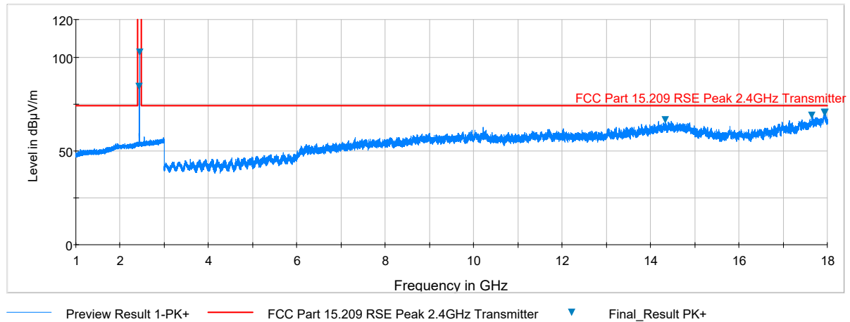
Plot 7-43. Radiated Spurious Plot above 1GHz (BT – Ch. 39, Ant. Pol. H)
