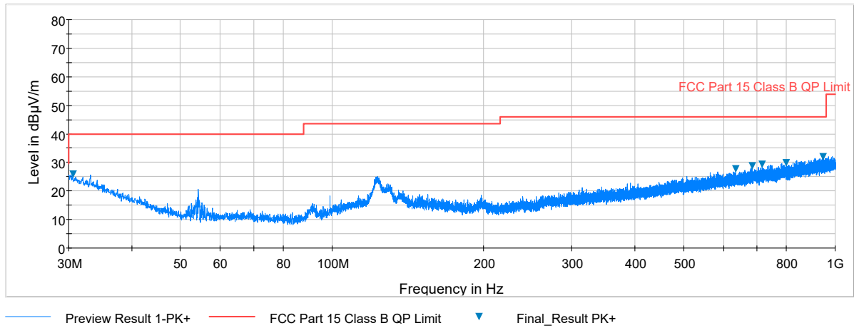
Plot 7-48. Radiated Spurious Plot below 1GHz (Pol. H)
