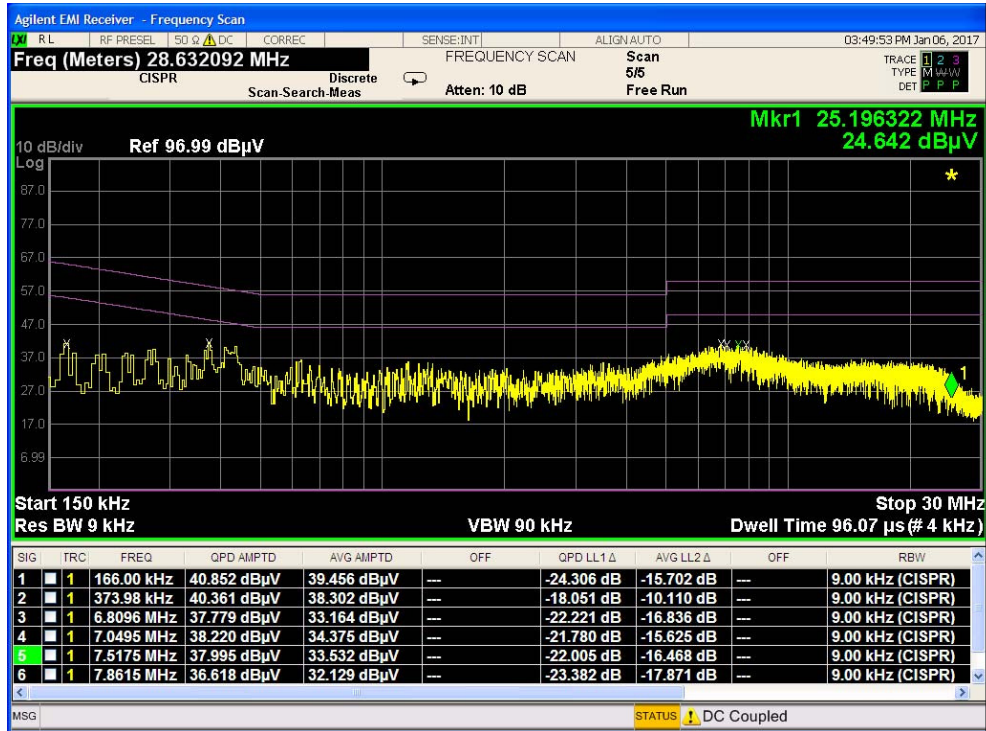
Plot 7-50. Line-Conducted Test Plot (L1)
