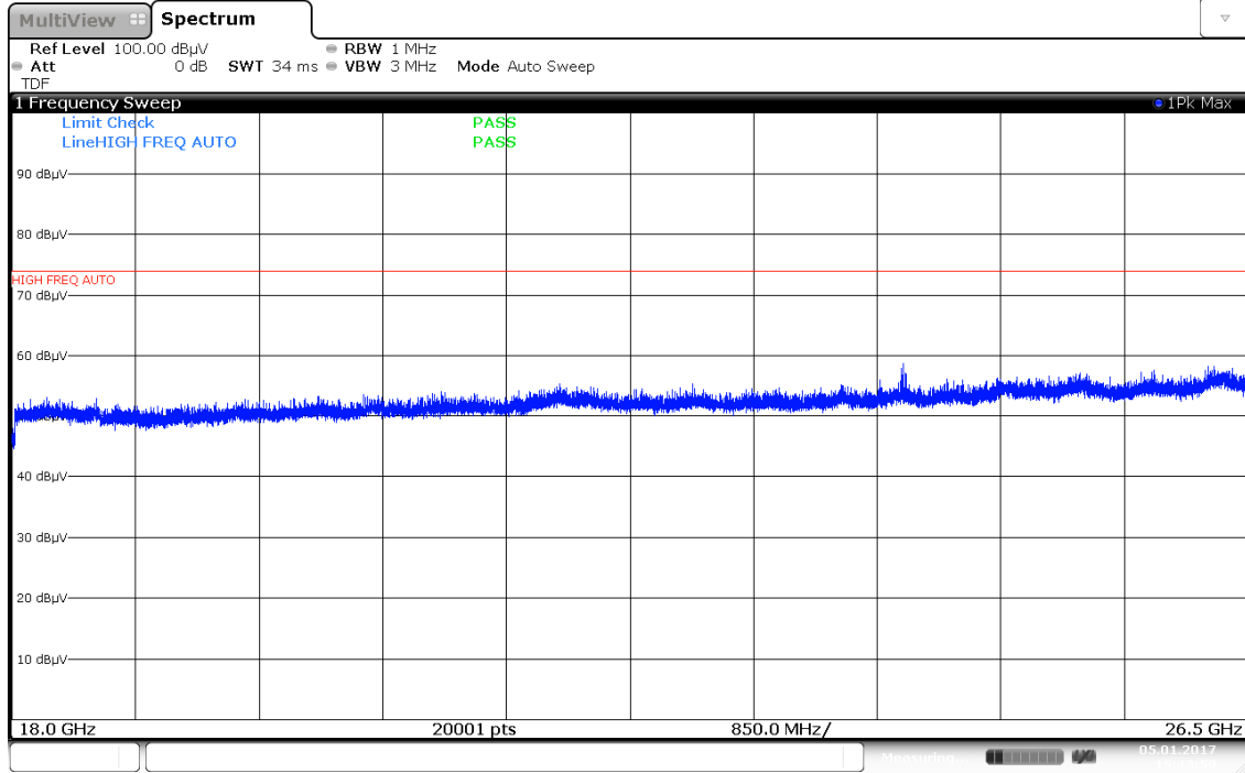
Plot 7-44. Radiated Spurious Plot above 18GHz (Pol. H)
