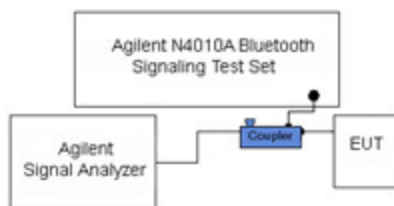
Figure 7-7. Test Instrument & Measurement Setup
