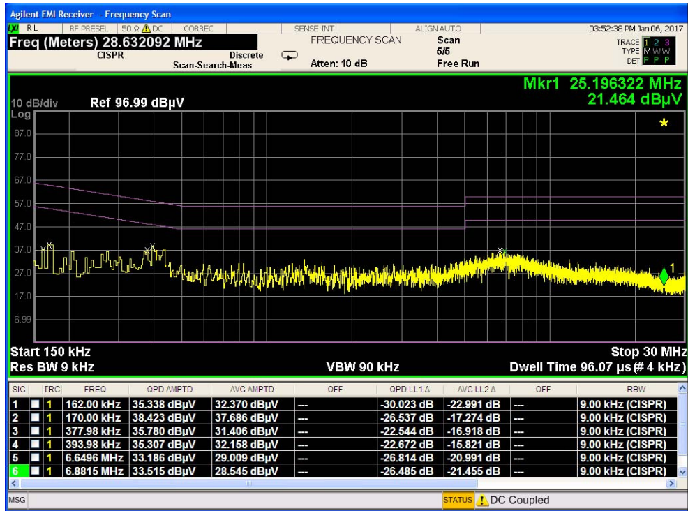
Plot 7-51. Line-Conducted Test Plot (N)
