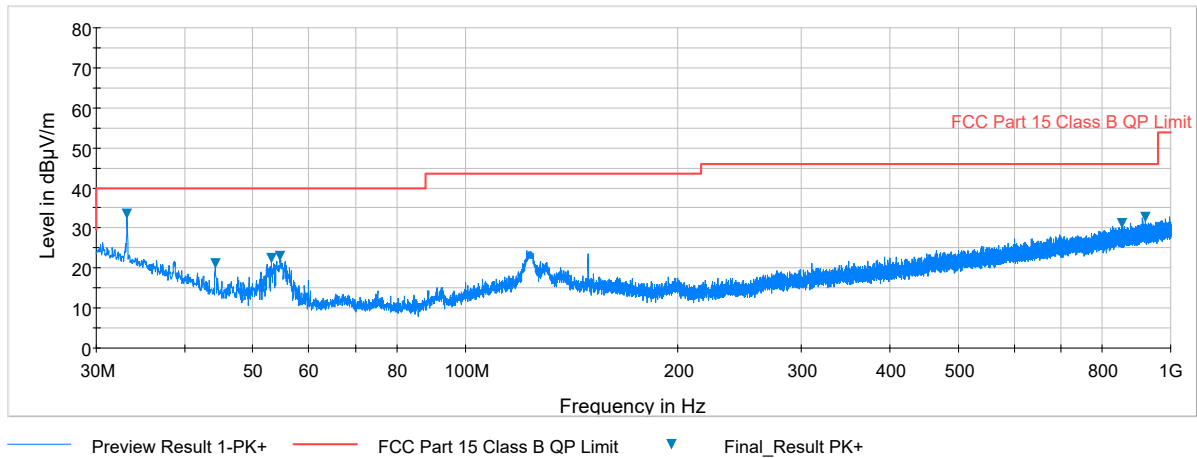
Plot 7-49. Radiated Spurious Plot below 1GHz (Pol. V)
