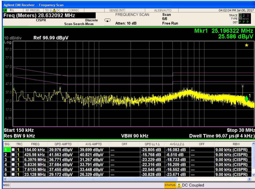
Plot 7-6. Line-Conducted Test Plot (L1)
