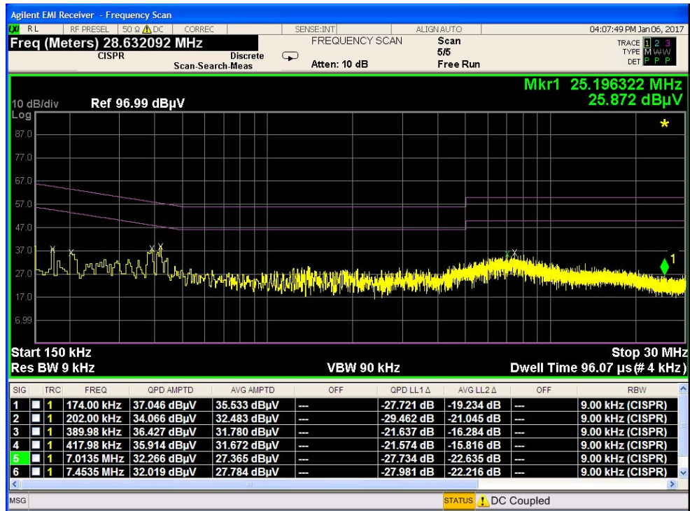
Plot 7-42. Line Conducted Plot with 802.11b (N)
