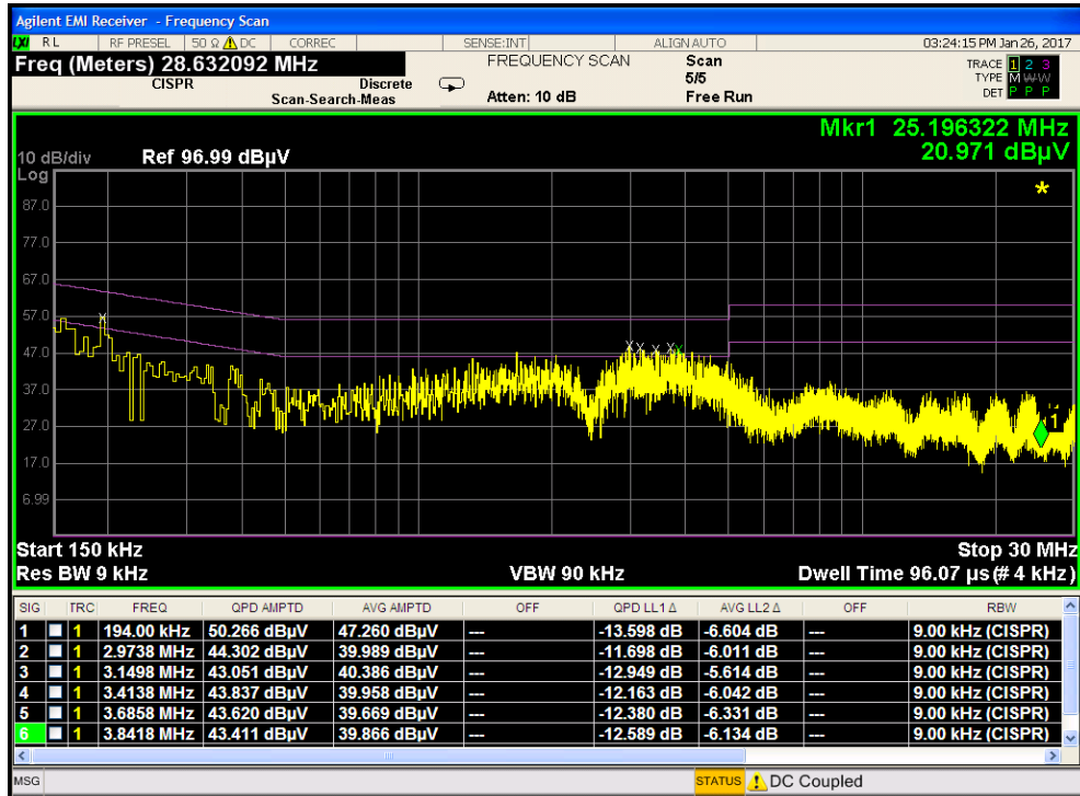
Plot 7-41. Line Conducted Plot with 802.11b (L1)
