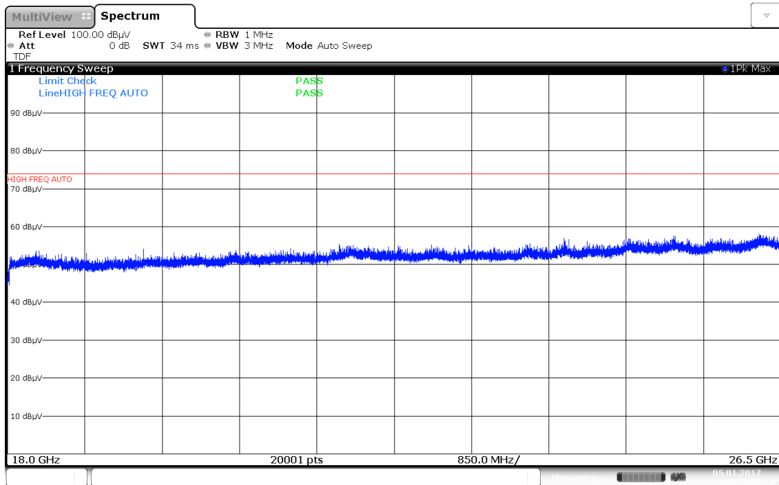
Plot 7-34. Radiated Spurious Plot above 18GHz (Pol. V)
