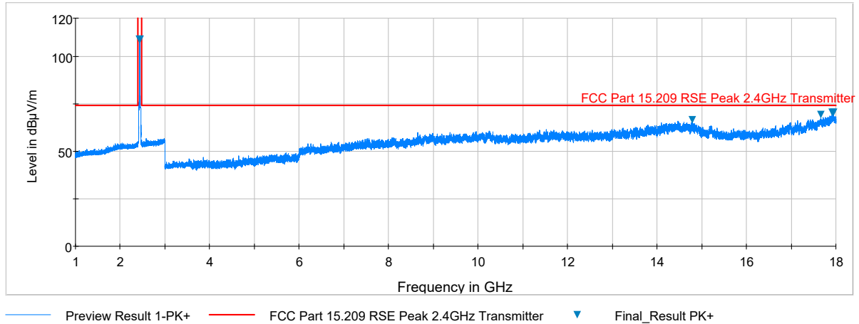
Plot 7-31. Radiated Spurious Plot above 1GHz (802.11b – Ch. 6, Ant. Pol. H)
