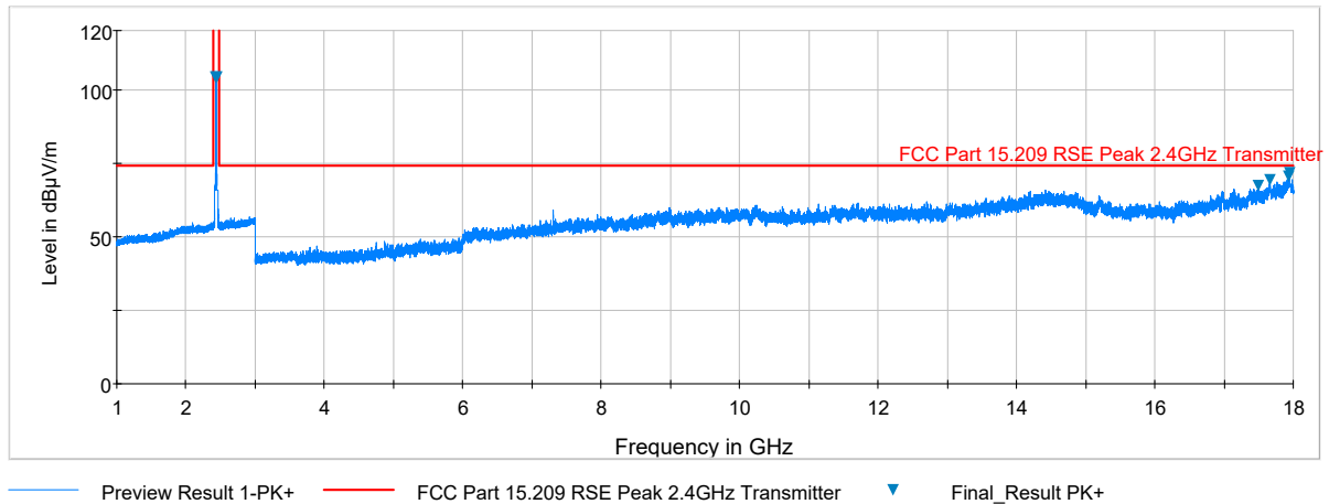
Plot 7-32. Radiated Spurious Plot above 1GHz (802.11b – Ch. 6, Ant. Pol. V)
