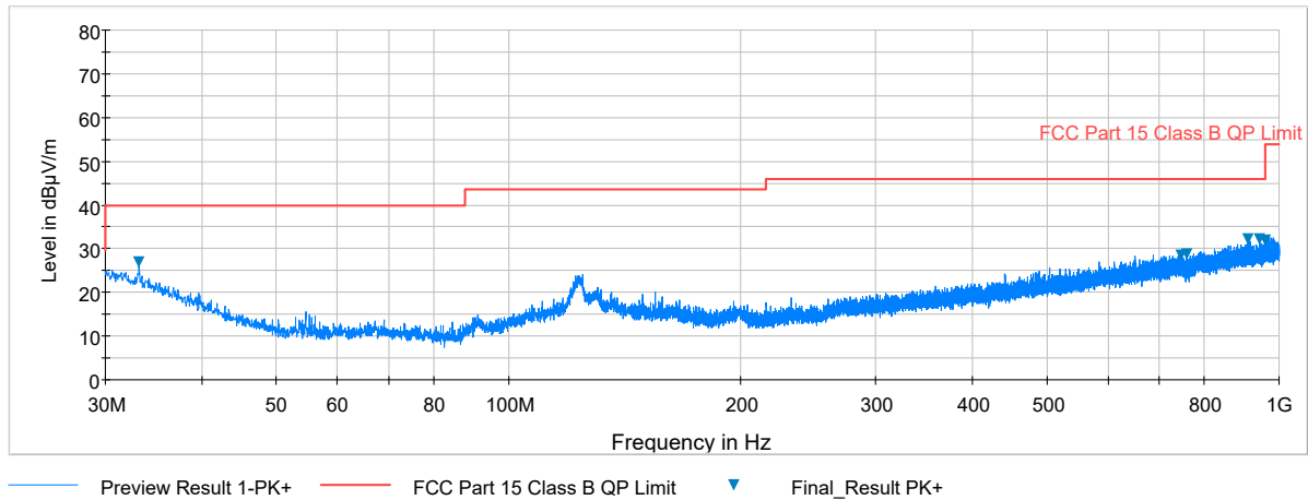
Plot 7-39. Radiated Spurious Plot below 1GHz (Pol. H)
