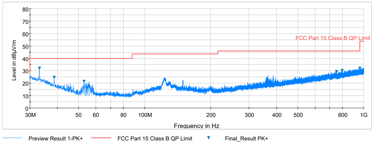
Plot 7-40. Radiated Spurious Plot below 1GHz (Pol. V)
