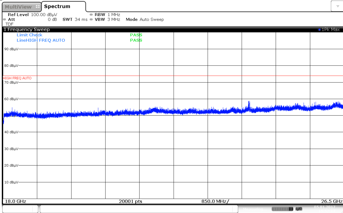
Plot 7-33. Radiated Spurious Plot above 18GHz (Pol. H)
