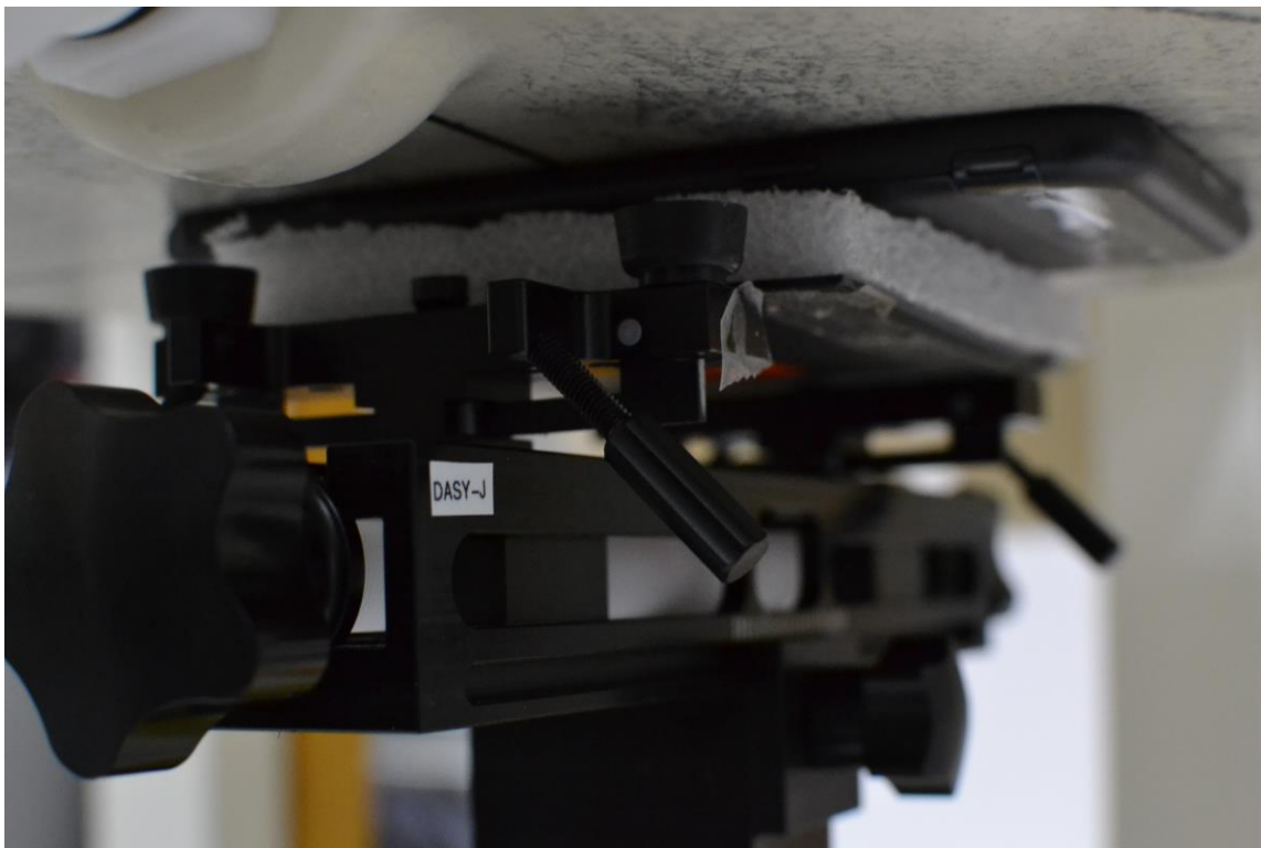
SAR Test Setup Photo 11- Front at 0.0 cm (Phablet)
