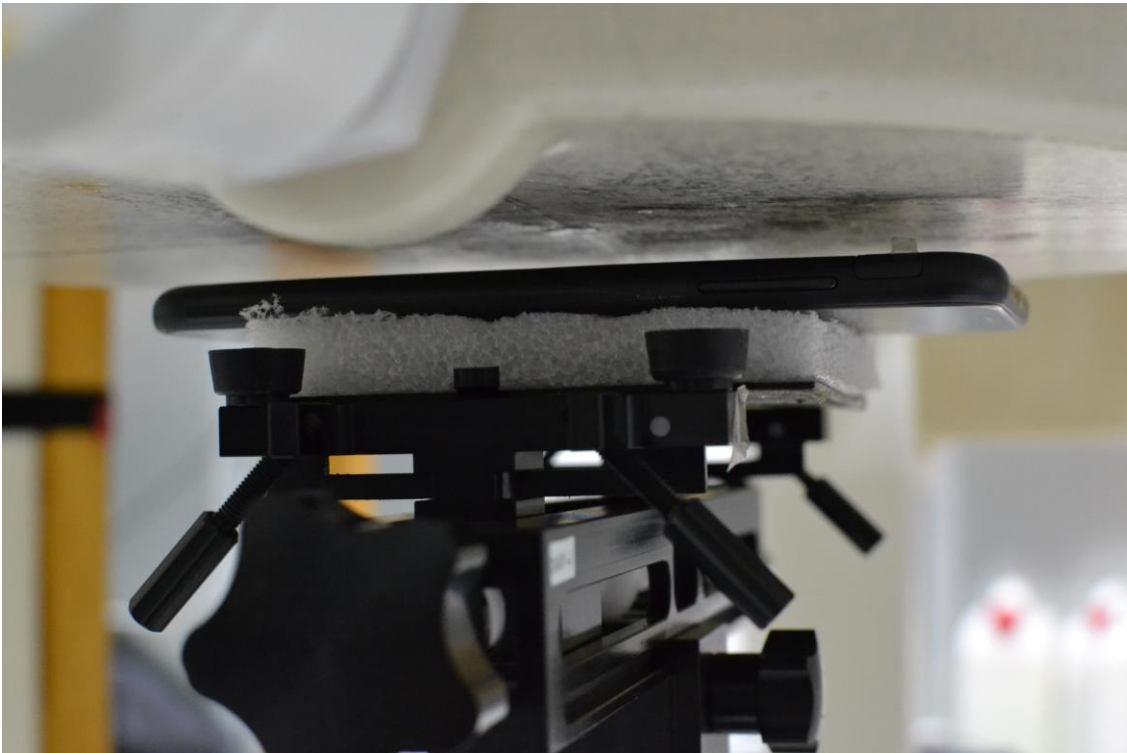
SAR Test Setup Photo 6- Back at 1.0 cm (Hotspot)
