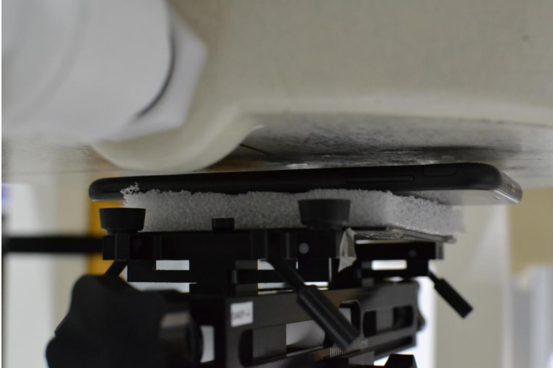
SAR Test Setup Photo 7- Back at 0.4 cm (Phablet)
