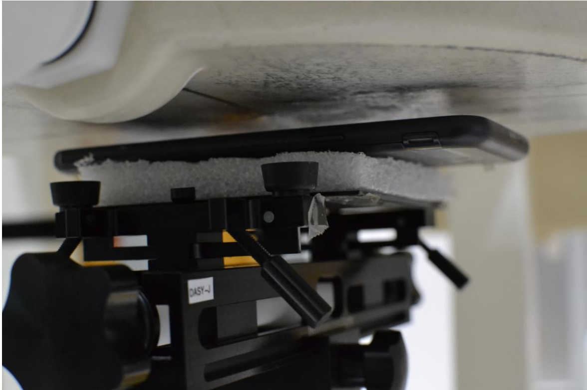
SAR Test Setup Photo 9- Front at 1.0 cm (Hotspot)
