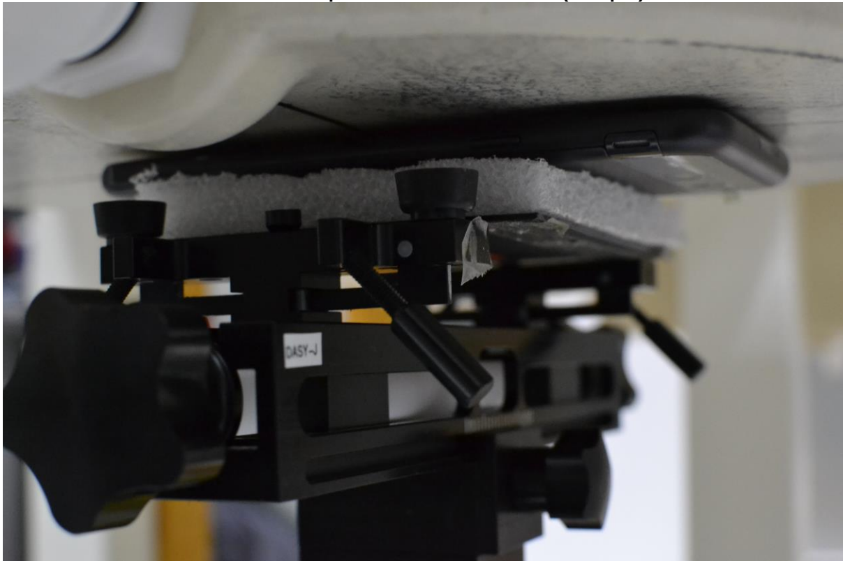
SAR Test Setup Photo 10- Front at 0.2 cm (Phablet)
