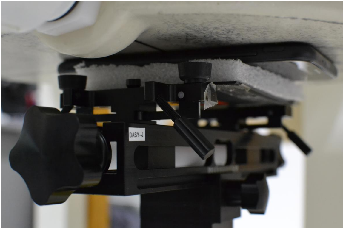
SAR Test Setup Photo 8- Back at 0.0 cm (Phablet)
