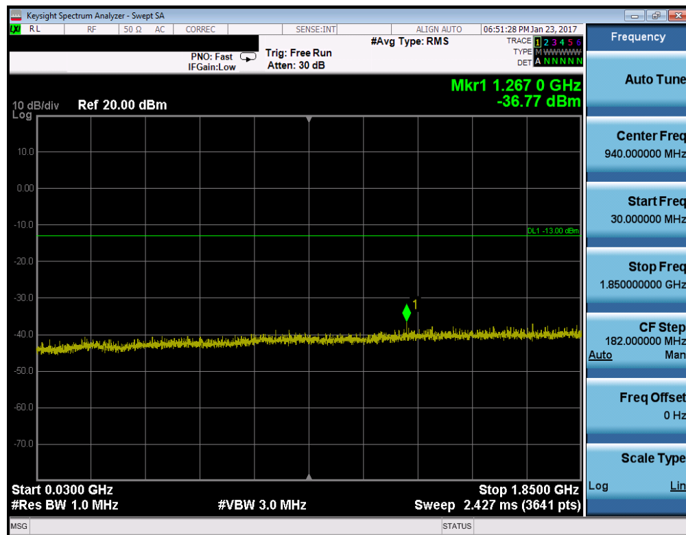
Plot 7-8. Conducted Spurious Plot (PCS GSM Mode – Ch. 661)
