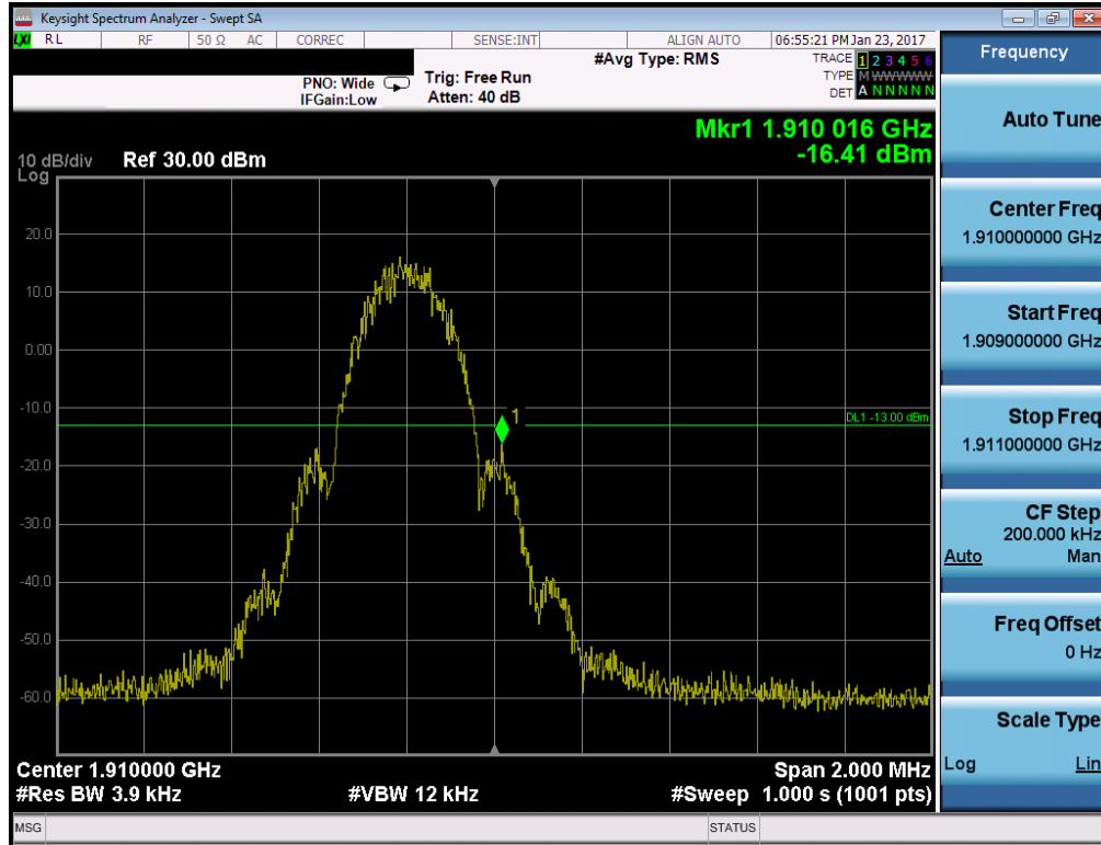
Plot 7-34. Band Edge Plot (PCS GSM Mode – Ch. 810)
