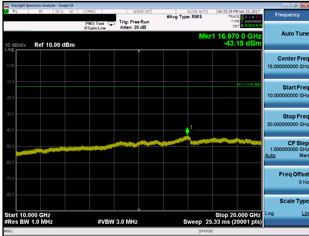
Plot 7-25. Conducted Spurious Plot (PCS WCDMA Mode – Ch. 9262)
