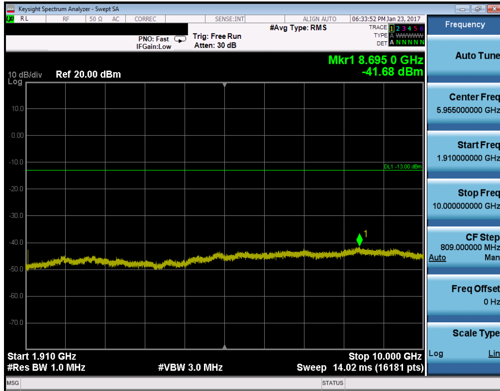
Plot 7-27. Conducted Spurious Plot (PCS WCDMA Mode – Ch. 9400)
