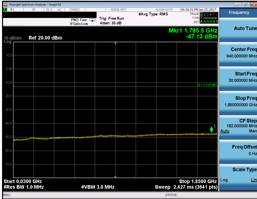
Plot 7-29. Conducted Spurious Plot (PCS WCDMA Mode – Ch. 9538)
