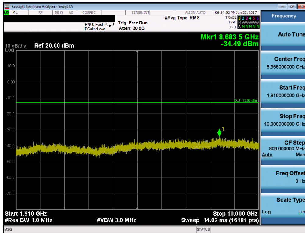
Plot 7-6. Conducted Spurious Plot (PCS GSM Mode – Ch. 512)
