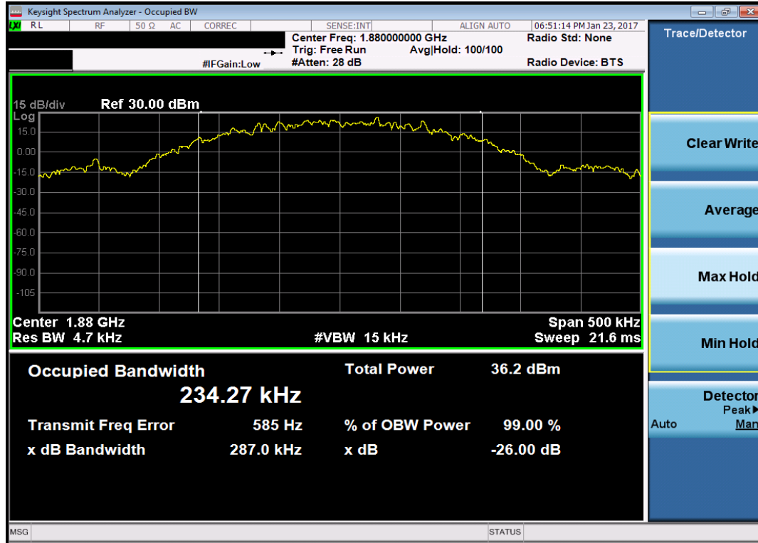
Plot 7-1. Occupied Bandwidth Plot (PCS GSM Mode – Ch. 661)
