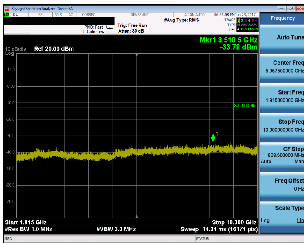
Plot 7-12. Conducted Spurious Plot (PCS GSM Mode – Ch. 810)
