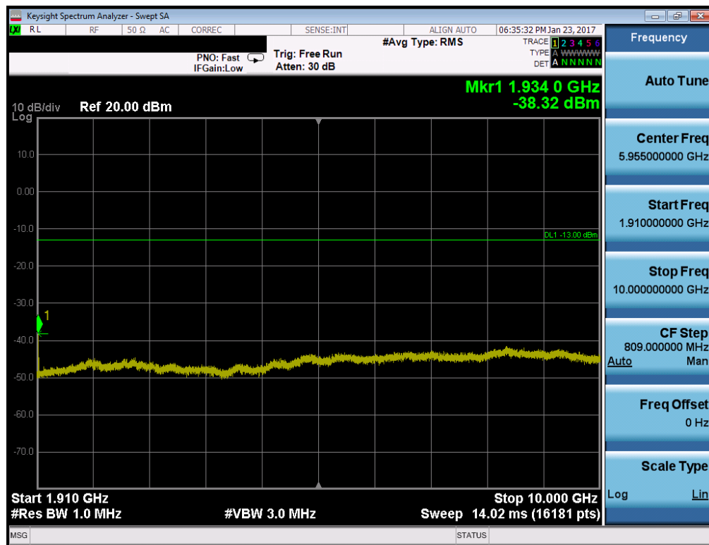
Plot 7-24. Conducted Spurious Plot (PCS WCDMA Mode – Ch. 9262)
