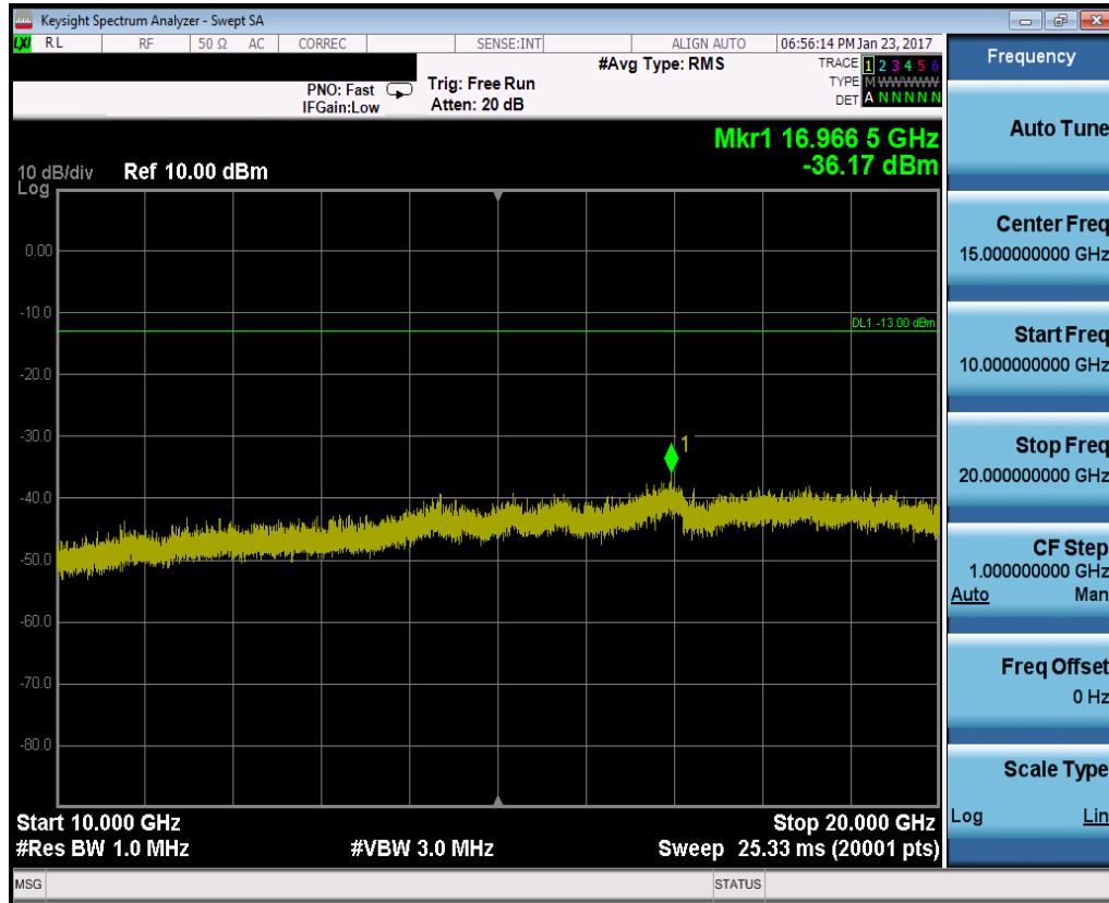
Plot 7-13. Conducted Spurious Plot (PCS GSM Mode – Ch. 810)
