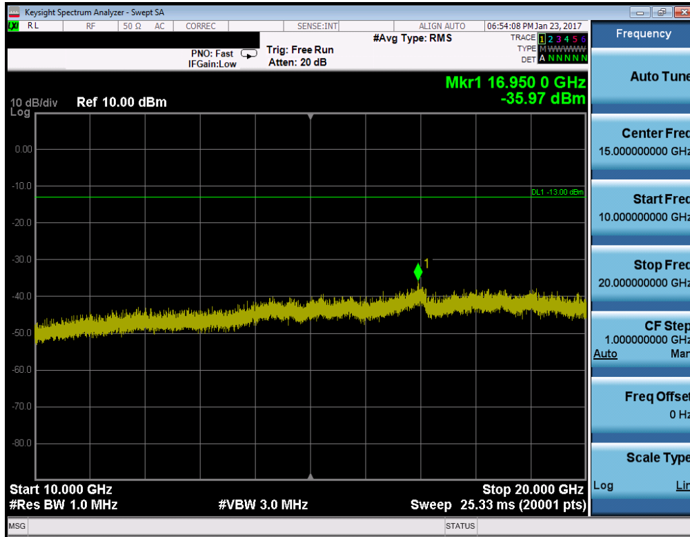
Plot 7-7. Conducted Spurious Plot (PCS GSM Mode – Ch. 512)
