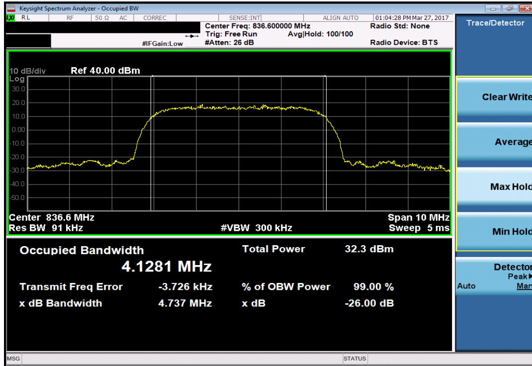
Plot 7-3. Occupied Bandwidth Plot (Cellular WCDMA Mode – Ch. 4183)
