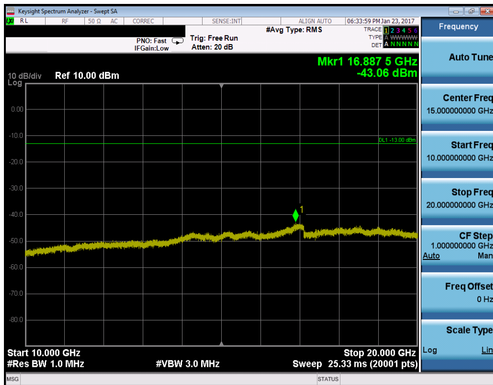
Plot 7-28. Conducted Spurious Plot (PCS WCDMA Mode – Ch. 9400)
