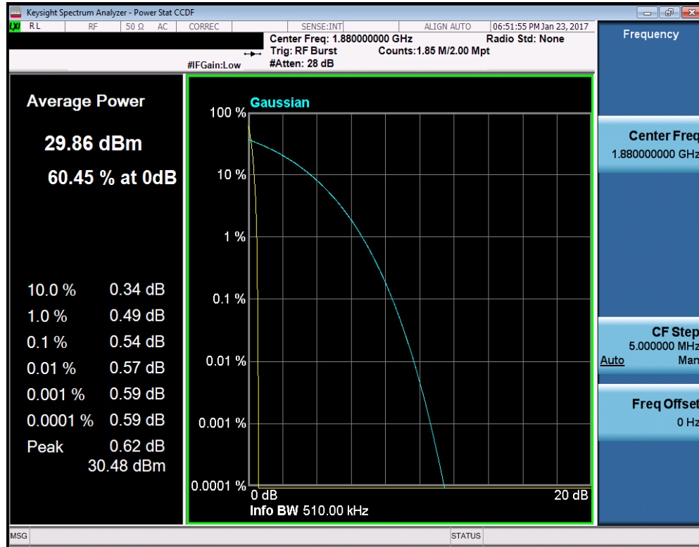
Plot 7-42. Peak-Average Ratio Plot (PCS GSM Mode – Ch. 661)
