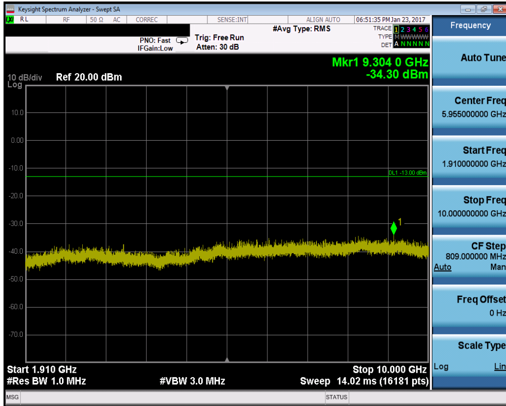
Plot 7-9. Conducted Spurious Plot (PCS GSM Mode – Ch. 661)
