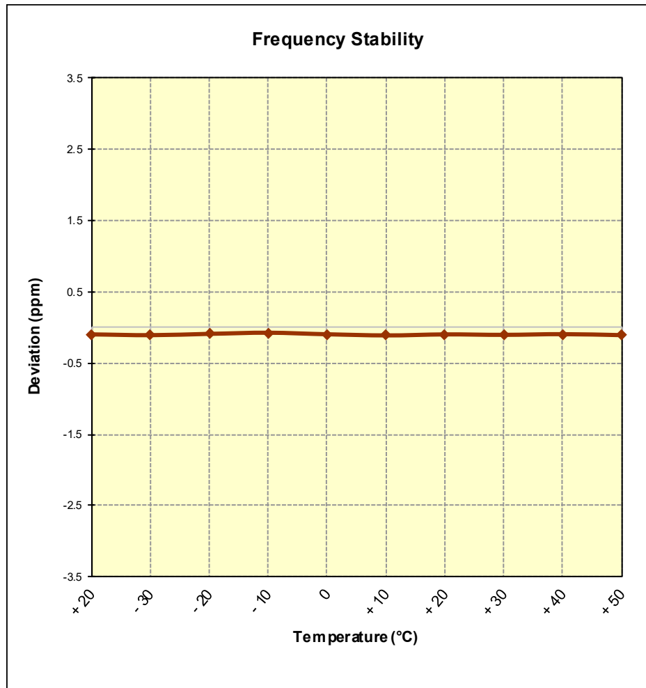
Figure 7-9. Frequency Stability Graph (PCS GSM Mode – Ch. 661)
