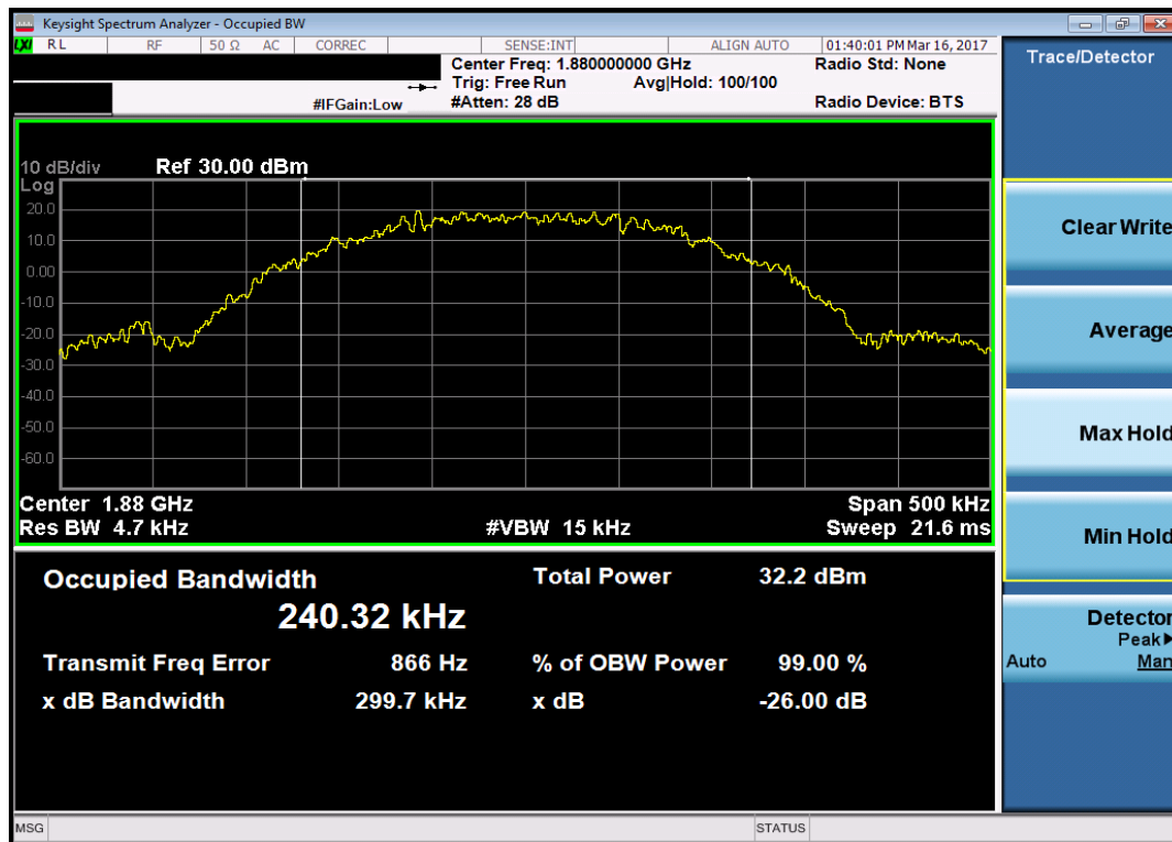
Plot 7-2. Occupied Bandwidth Plot (EDGE1900 Mode – Ch. 661)
