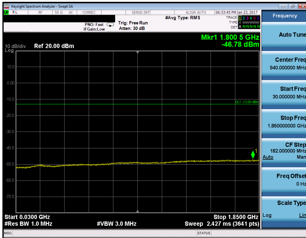
Plot 7-26. Conducted Spurious Plot (PCS WCDMA Mode – Ch. 9400)
