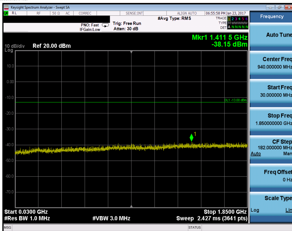
Plot 7-11. Conducted Spurious Plot (PCS GSM Mode – Ch. 810)
