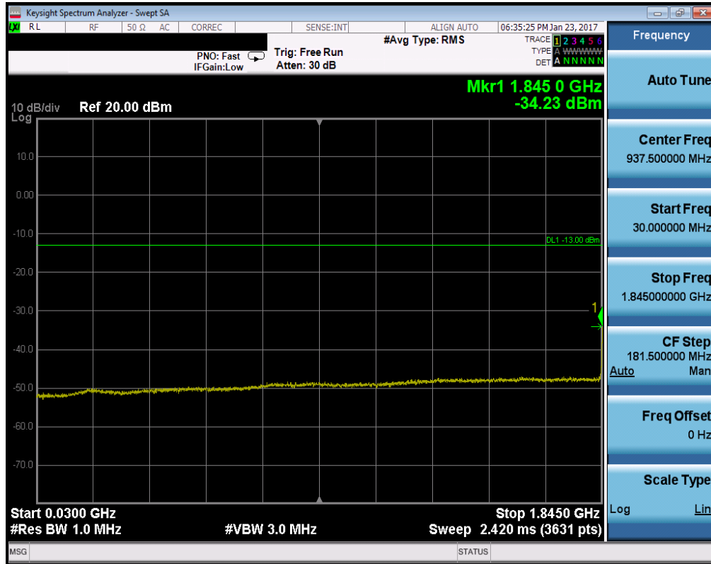
Plot 7-23. Conducted Spurious Plot (PCS WCDMA Mode – Ch. 9262)
