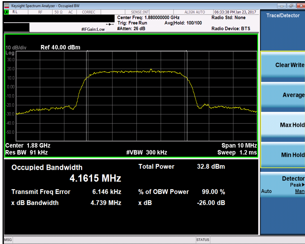
Plot 7-4. Occupied Bandwidth Plot (PCS WCDMA Mode – Ch. 9400)
