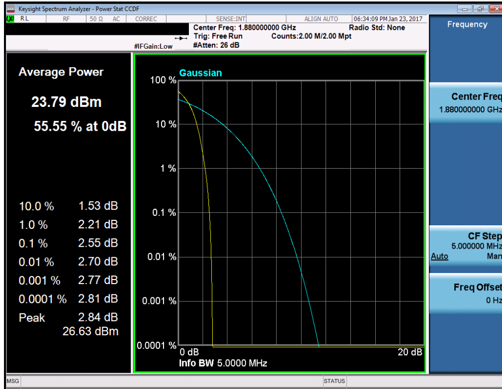
Plot 7-44. Peak-Average Ratio Plot (PCS WCDMA Mode – Ch. 9400)
