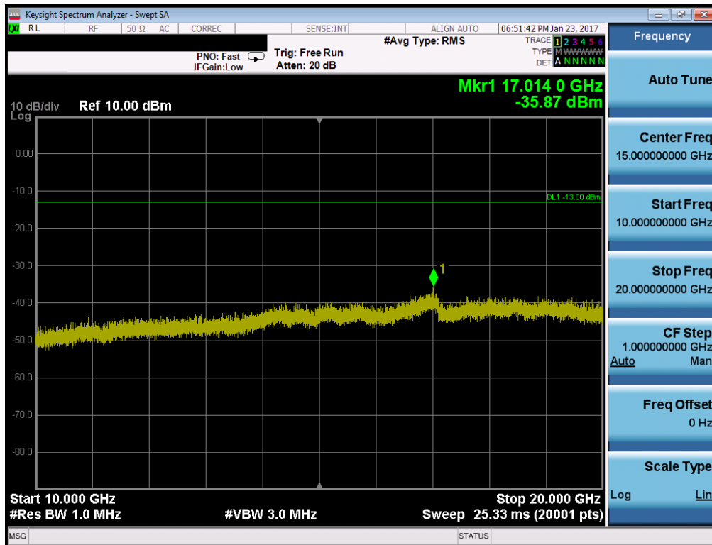
Plot 7-10. Conducted Spurious Plot (PCS GSM Mode – Ch. 661)
