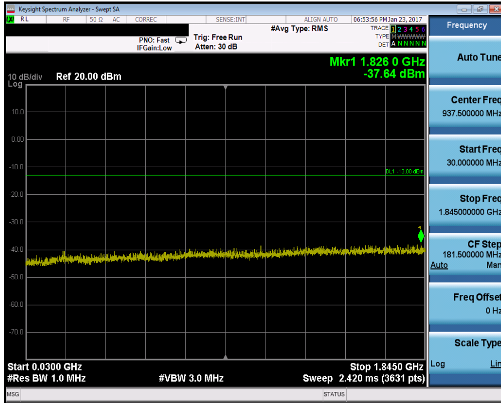
Plot 7-5. Conducted Spurious Plot (PCS GSM Mode – Ch. 512)
