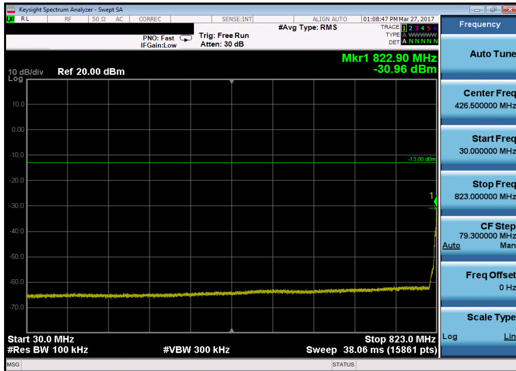
Plot 7-14. Conducted Spurious Plot (Cellular WCDMA Mode – Ch. 4132)
