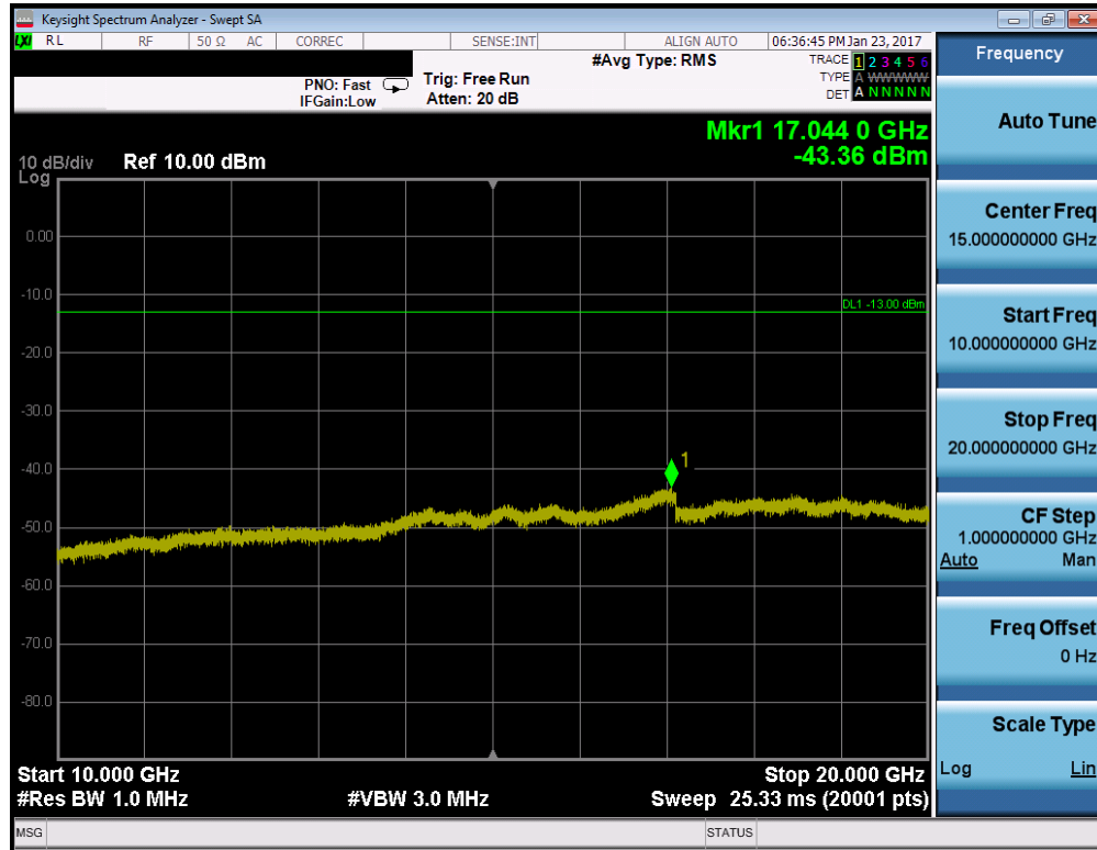
Plot 7-31. Conducted Spurious Plot (PCS WCDMA Mode – Ch. 9538)
