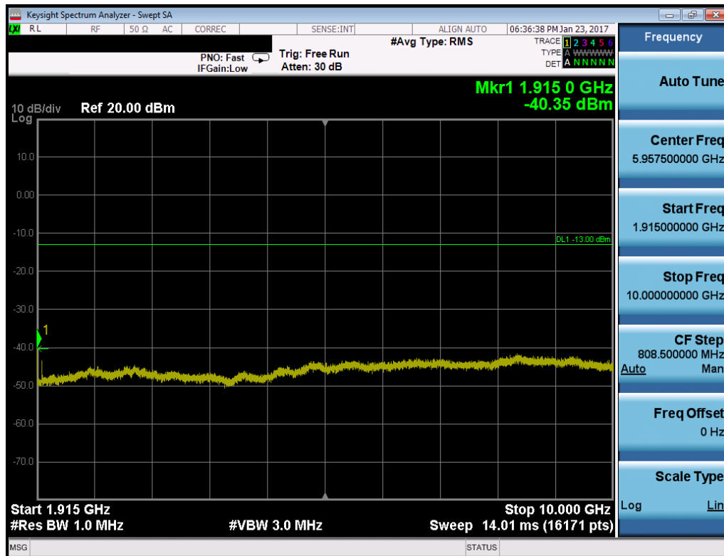
Plot 7-30. Conducted Spurious Plot (PCS WCDMA Mode – Ch. 9538)
