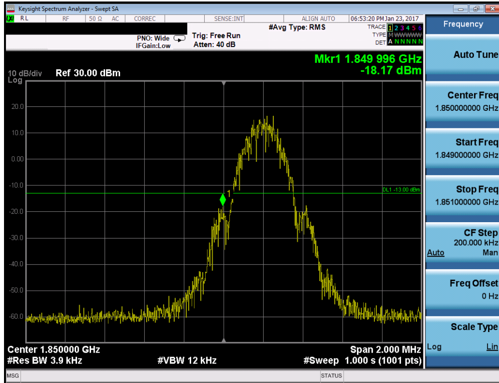
Plot 7-32. Band Edge Plot (PCS GSM Mode – Ch. 512)
