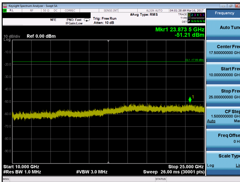
Plot 7-13. Conducted Spurious Plot (Bluetooth (LE), 1Mbps – Ch. 0)
