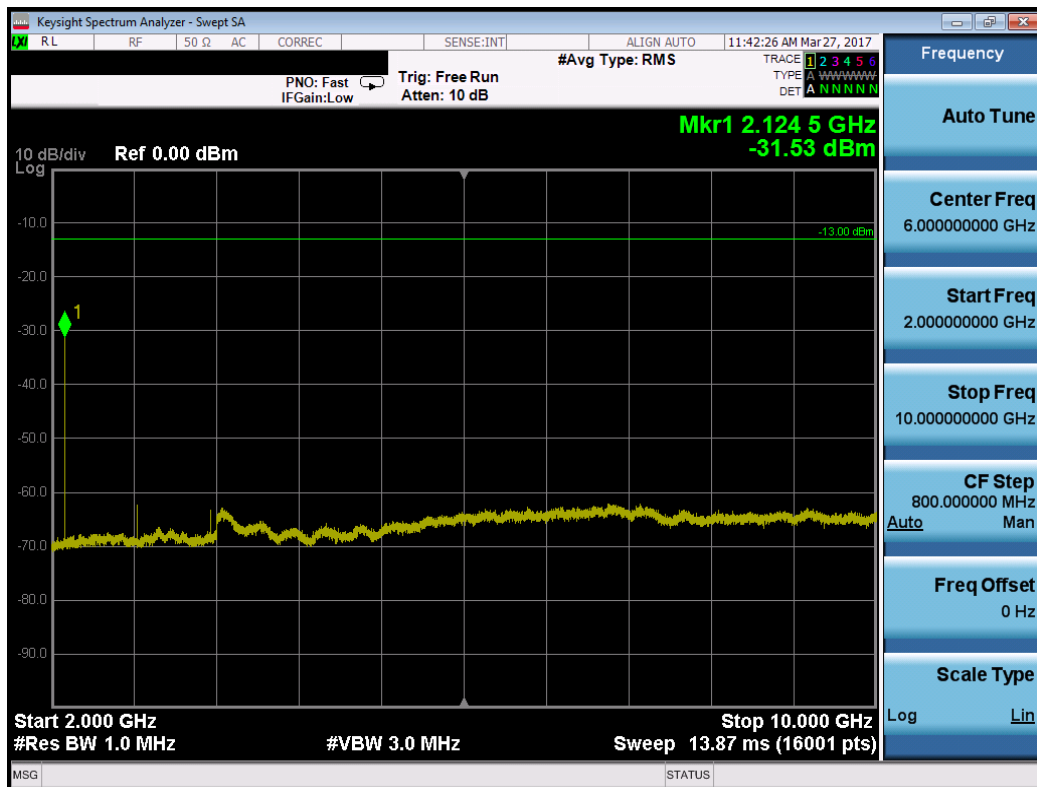
Plot 7-18. Conducted Spurious Plot (Band 17 – 5.0MHz QPSK – RB Size 1, RB Offset 0 – Mid Channel)
