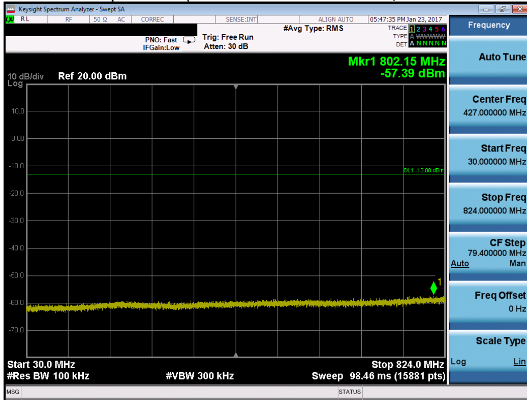
Plot 7-28. Conducted Spurious Plot (Band 5 – 1.4MHz QPSK – RB Size 1, RB Offset 0 – High Channel)
