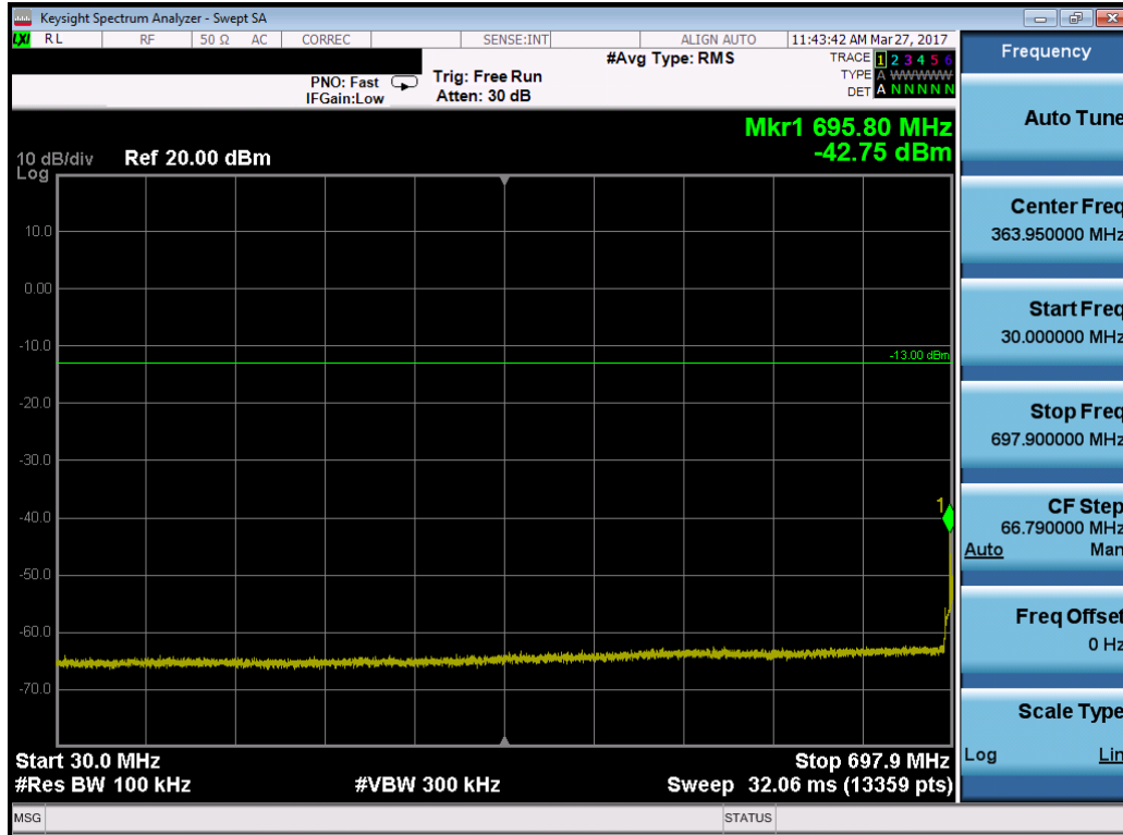
Plot 7-13. Conducted Spurious Plot (Band 17 – 5.0MHz QPSK – RB Size 1, RB Offset 0 – Low Channel)
