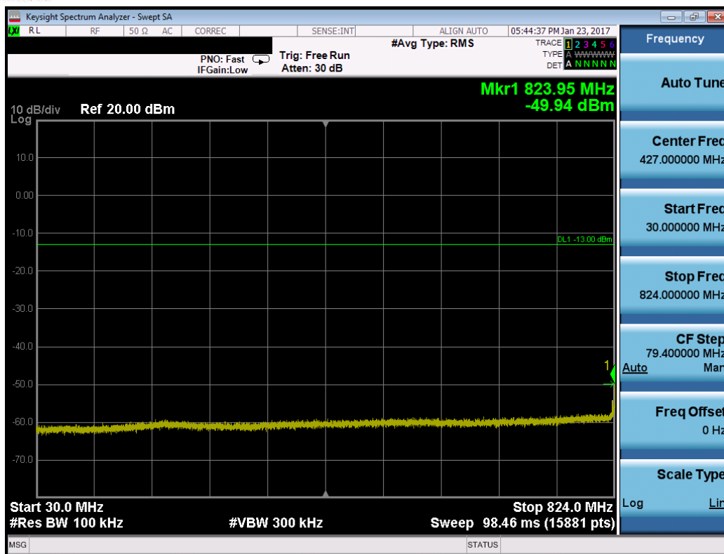
Plot 7-25. Conducted Spurious Plot (Band 5 – 1.4MHz QPSK – RB Size 1, RB Offset 0 – Mid Channel)
