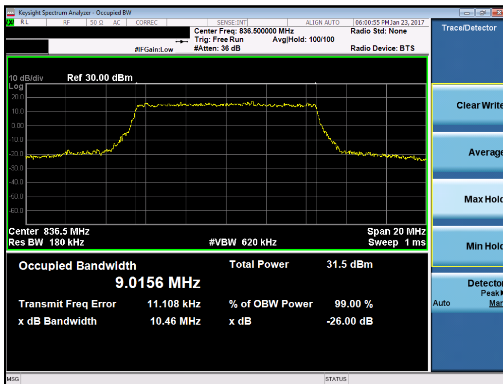
Plot 7-12. Occupied Bandwidth Plot (Band 5 – 10.0MHz 16-QAM – RB Size 50)
