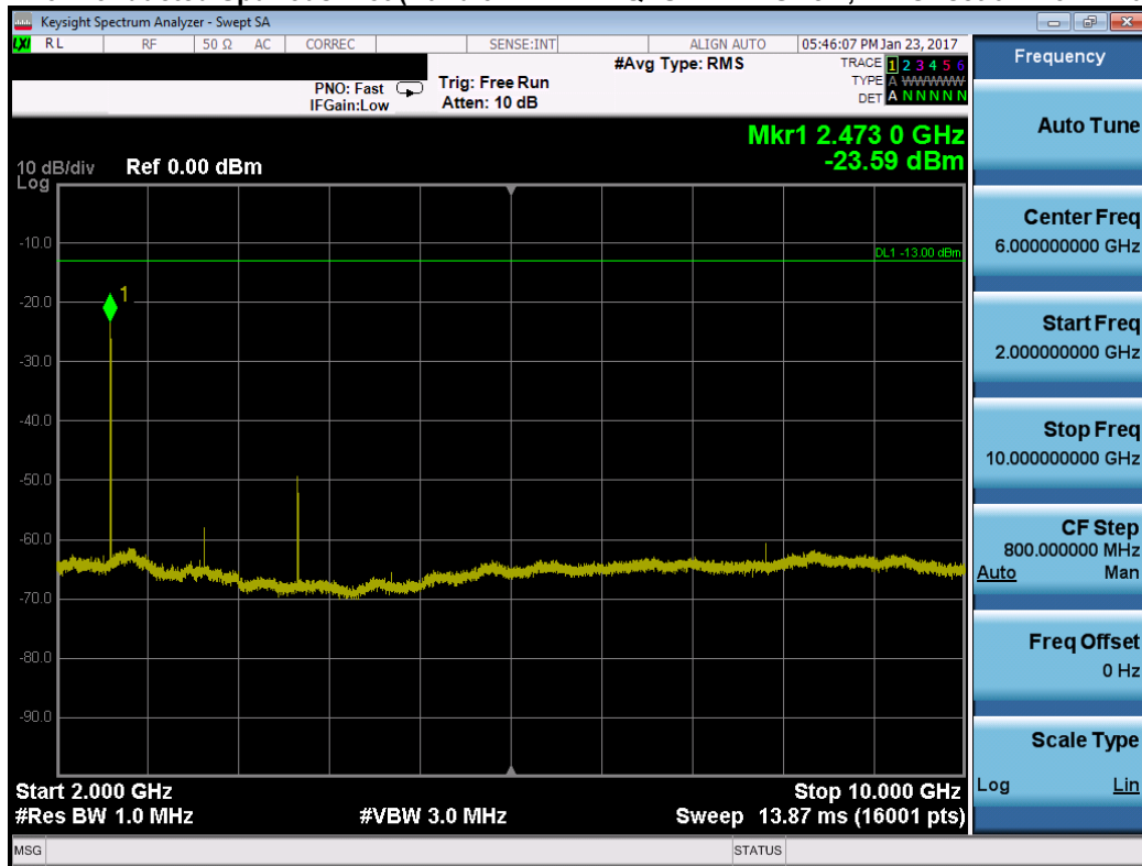
Plot 7-24. Conducted Spurious Plot (Band 5 – 1.4MHz QPSK – RB Size 1, RB Offset 0 – Low Channel)
