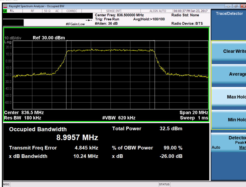
Plot 7-11. Occupied Bandwidth Plot (Band 5 – 10.0MHz QPSK – RB Size 50)
