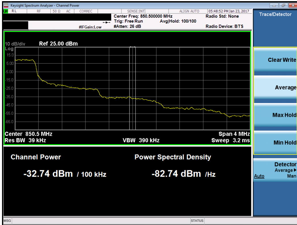
Plot 7-39. Upper Extended Band Edge Plot (Band 5 – 1.4MHz QPSK – RB Size 6)
