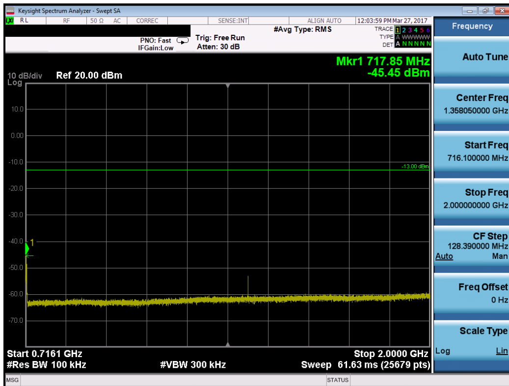
Plot 7-20. Conducted Spurious Plot (Band 17 – 5.0MHz QPSK – RB Size 1, RB Offset 0 – High Channel)
