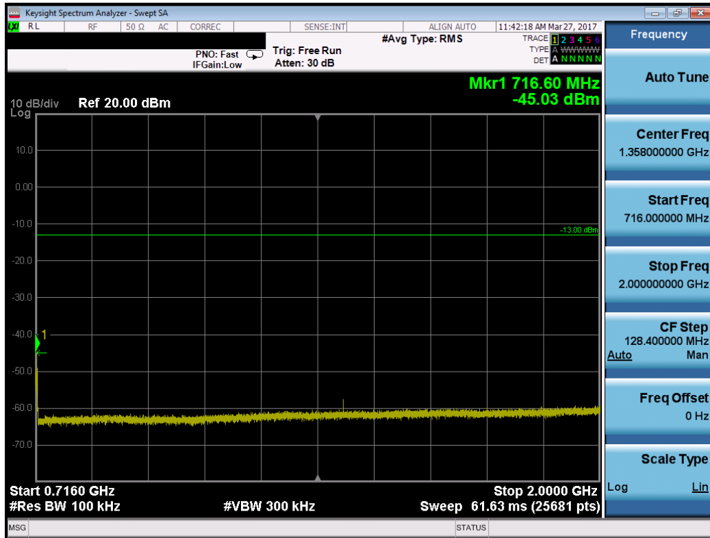
Plot 7-17. Conducted Spurious Plot (Band 17 – 5.0MHz QPSK – RB Size 1, RB Offset 0 – Mid Channel)
