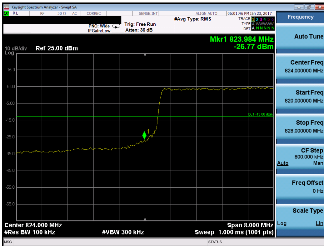
Plot 7-44. Lower Band Edge Plot (Band 5 – 10.0MHz QPSK – RB Size 50)
