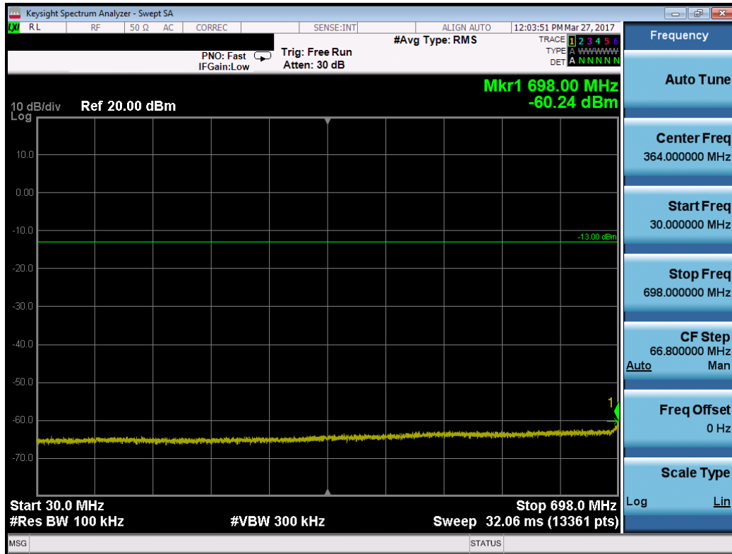
Plot 7-19. Conducted Spurious Plot (Band 17 – 5.0MHz QPSK – RB Size 1, RB Offset 0 – High Channel)
