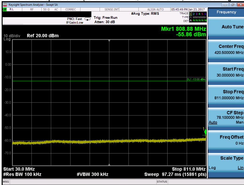
Plot 7-22. Conducted Spurious Plot (Band 5 – 1.4MHz QPSK – RB Size 1, RB Offset 0 – Low Channel)
