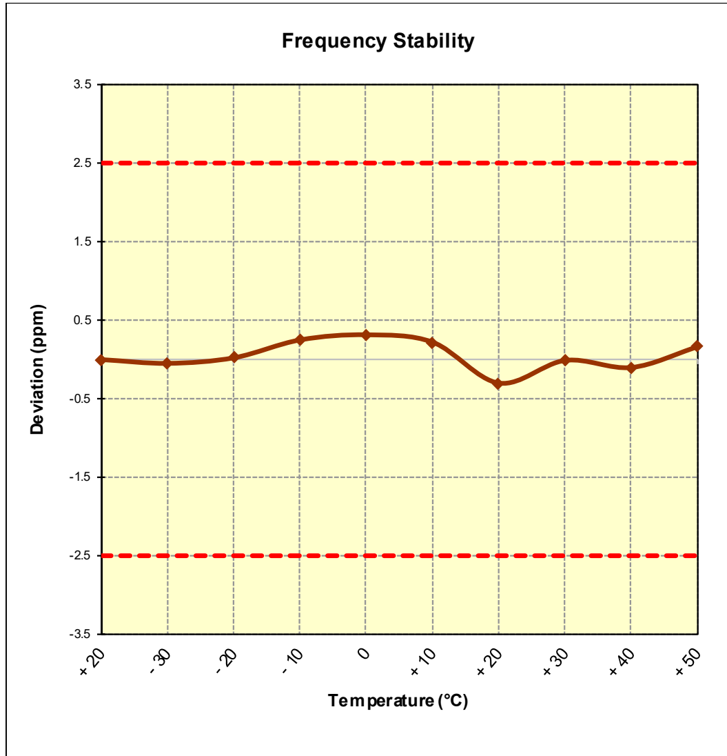
Figure 7-8. Frequency Stability Graph (Band 5)
