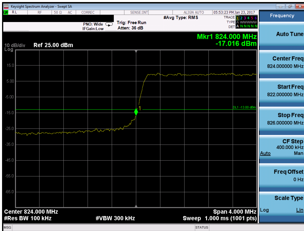
Plot 7-40. Lower Band Edge Plot (Band 5 – 3.0MHz QPSK – RB Size 15)
