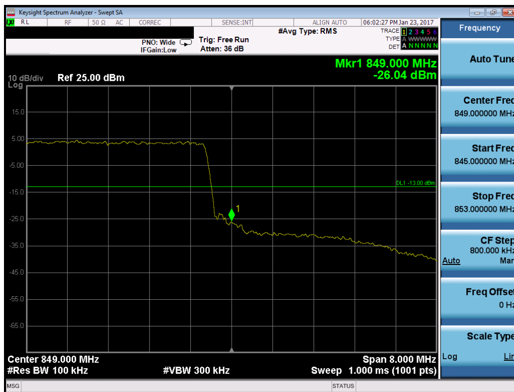
Plot 7-45. Upper Band Edge Plot (Band 5 – 10.0MHz QPSK – RB Size 50)
