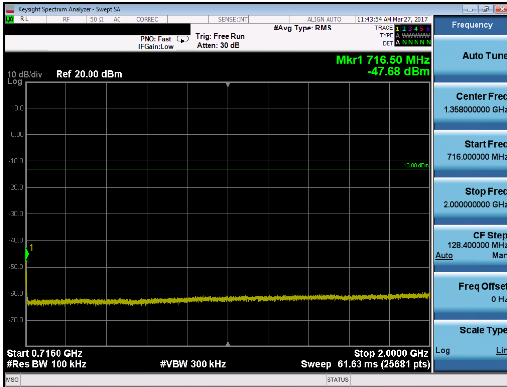
Plot 7-14. Conducted Spurious Plot (Band 17 – 5.0MHz QPSK – RB Size 1, RB Offset 0 – Low Channel)
