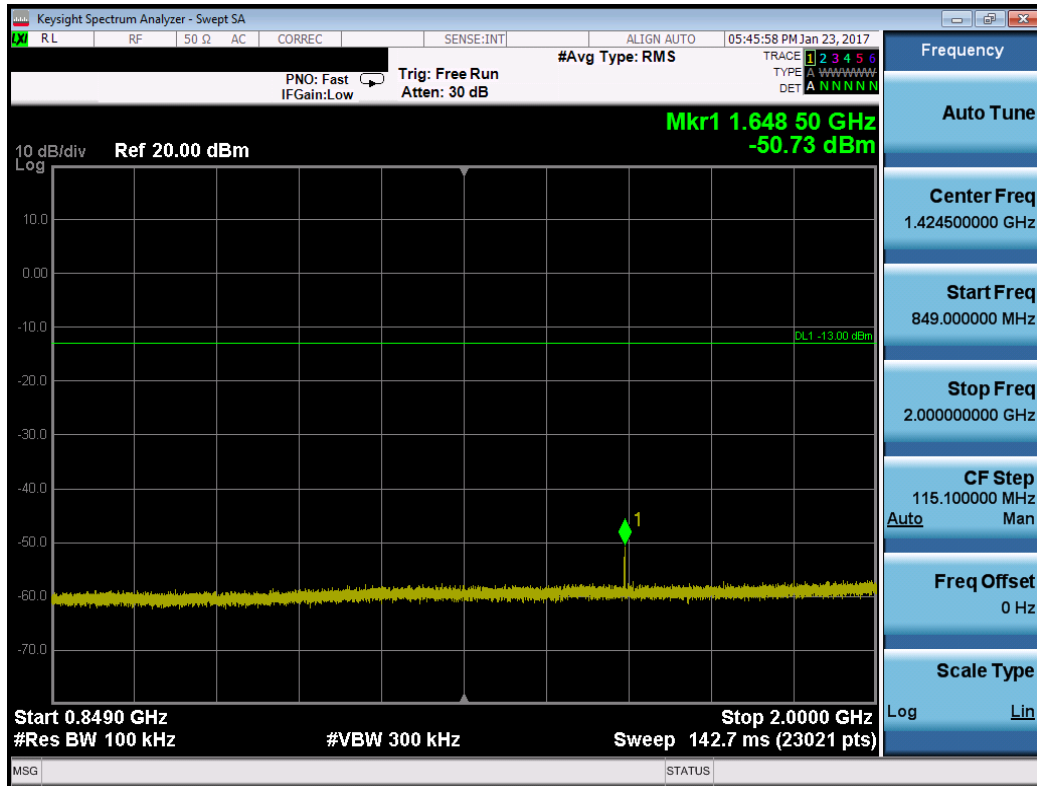
Plot 7-23. Conducted Spurious Plot (Band 5 – 1.4MHz QPSK – RB Size 1, RB Offset 0 – Low Channel)
