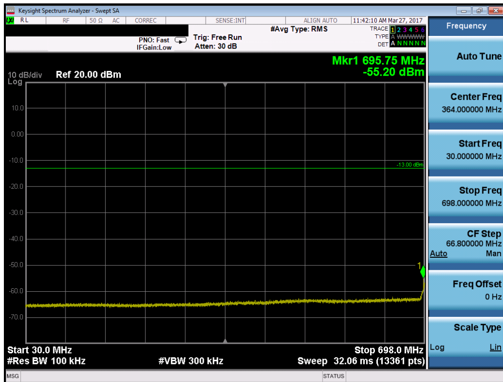
Plot 7-16. Conducted Spurious Plot (Band 17 – 5.0MHz QPSK – RB Size 1, RB Offset 0 – Mid Channel)
