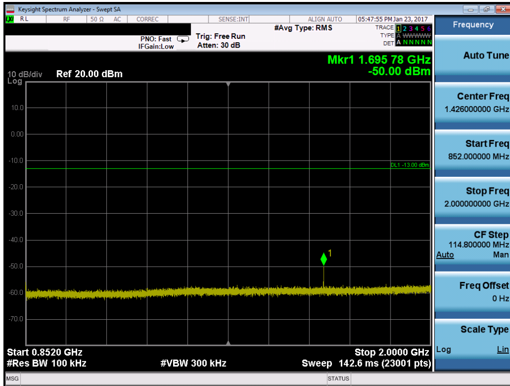
Plot 7-29. Conducted Spurious Plot (Band 5 – 1.4MHz QPSK – RB Size 1, RB Offset 0 – High Channel)
