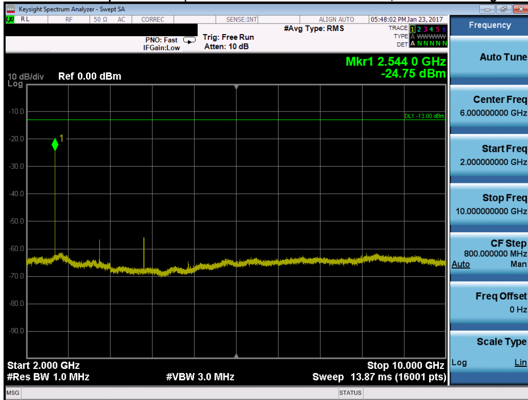
Plot 7-30. Conducted Spurious Plot (Band 5 – 1.4MHz QPSK – RB Size 1, RB Offset 0 – High Channel)
