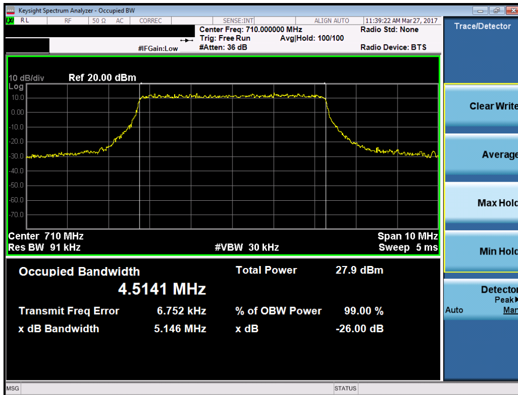
Plot 7-2. Occupied Bandwidth Plot (Band 17 – 5.0MHz 16-QAM – RB Size 25)
