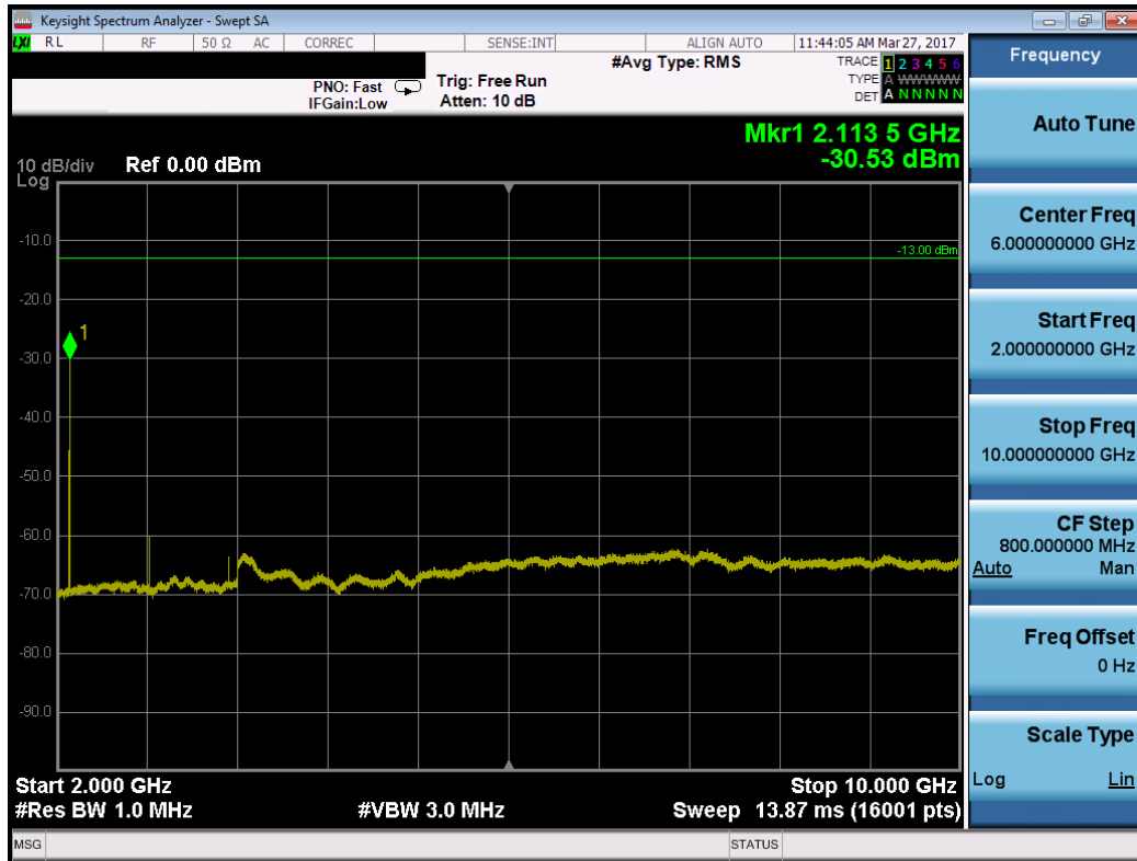
Plot 7-15. Conducted Spurious Plot (Band 17 – 5.0MHz QPSK – RB Size 1, RB Offset 0 – Low Channel)
