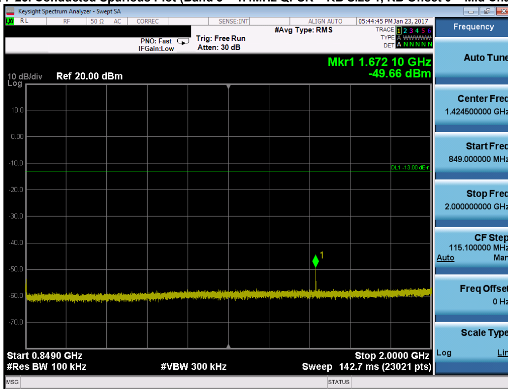
Plot 7-26. Conducted Spurious Plot (Band 5 – 1.4MHz QPSK – RB Size 1, RB Offset 0 – Mid Channel)
