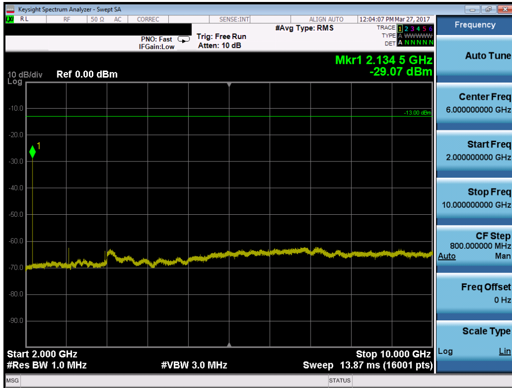
Plot 7-21. Conducted Spurious Plot (Band 17 – 5.0MHz QPSK – RB Size 1, RB Offset 0 – High Channel)
