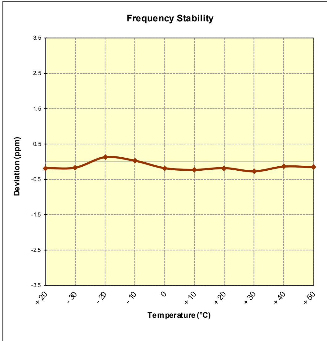
Figure 7-7. Frequency Stability Graph (Band 17)
