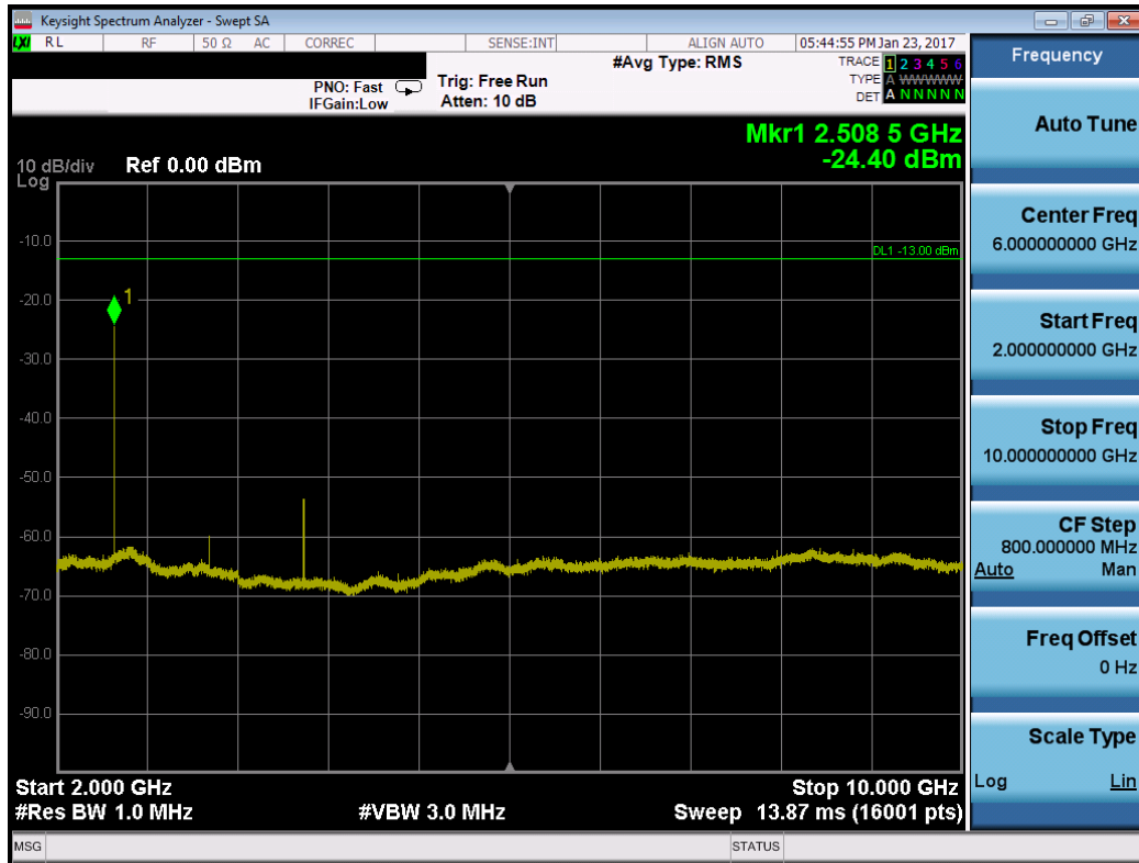
Plot 7-27. Conducted Spurious Plot (Band 5 – 1.4MHz QPSK – RB Size 1, RB Offset 0 – Mid Channel)
