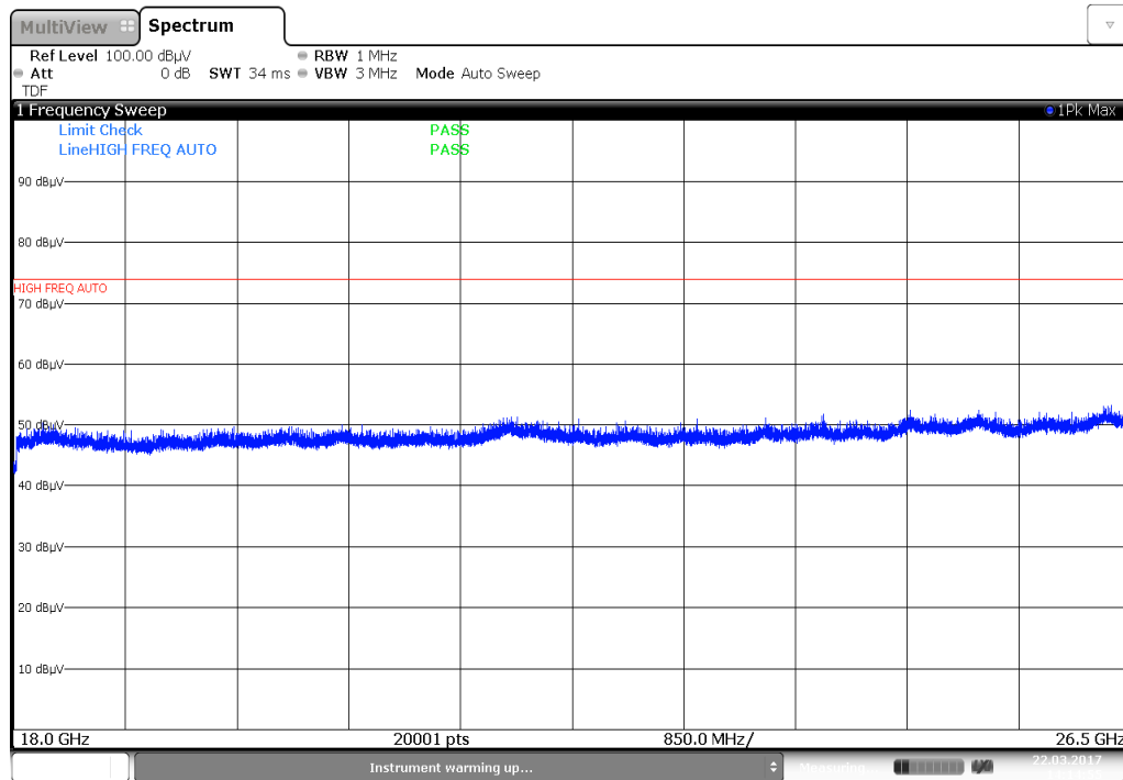
Plot 7-48. Radiated Spurious Plot above 18GHz (Pol. H)
