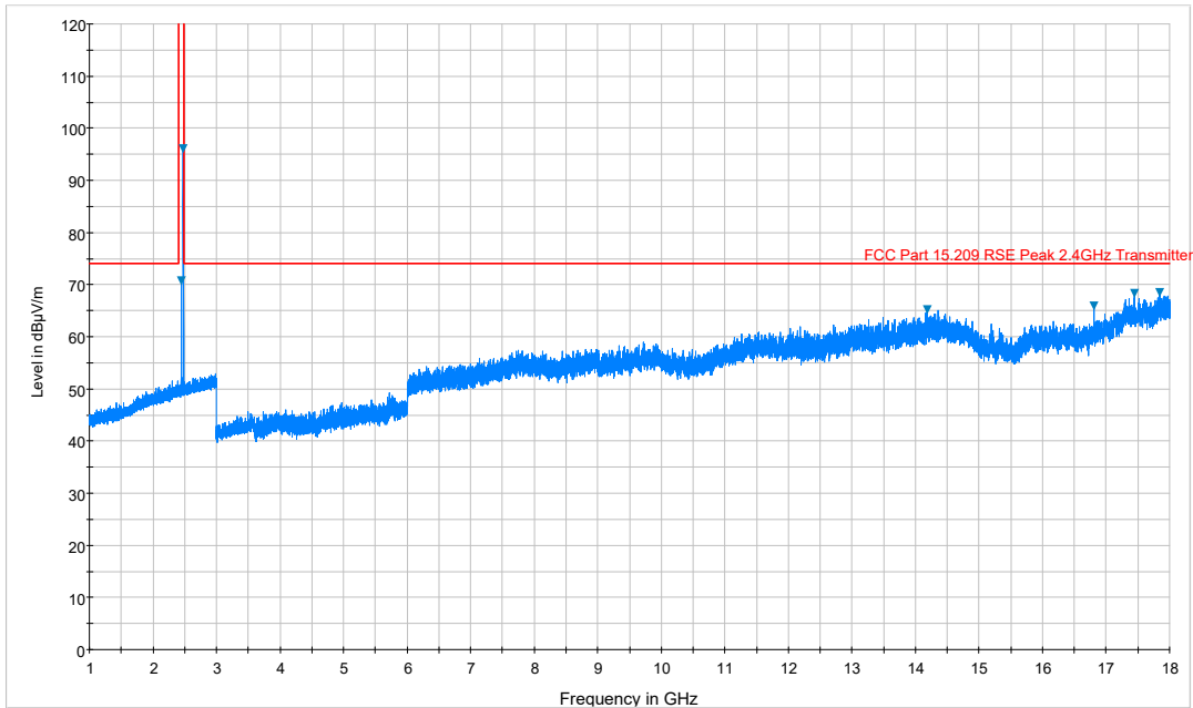
Plot 7-47. Radiated Spurious Plot above 1GHz (BT – Ch. 78, Ant. Pol. V)
