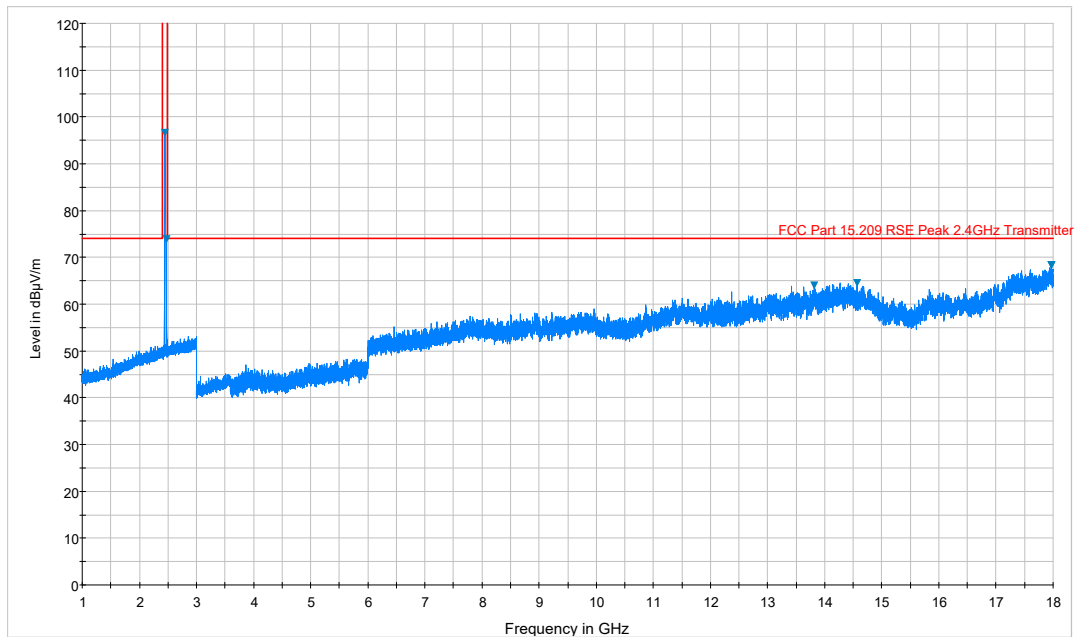
Plot 7-45. Radiated Spurious Plot above 1GHz (BT – Ch. 39, Ant. Pol. V)
