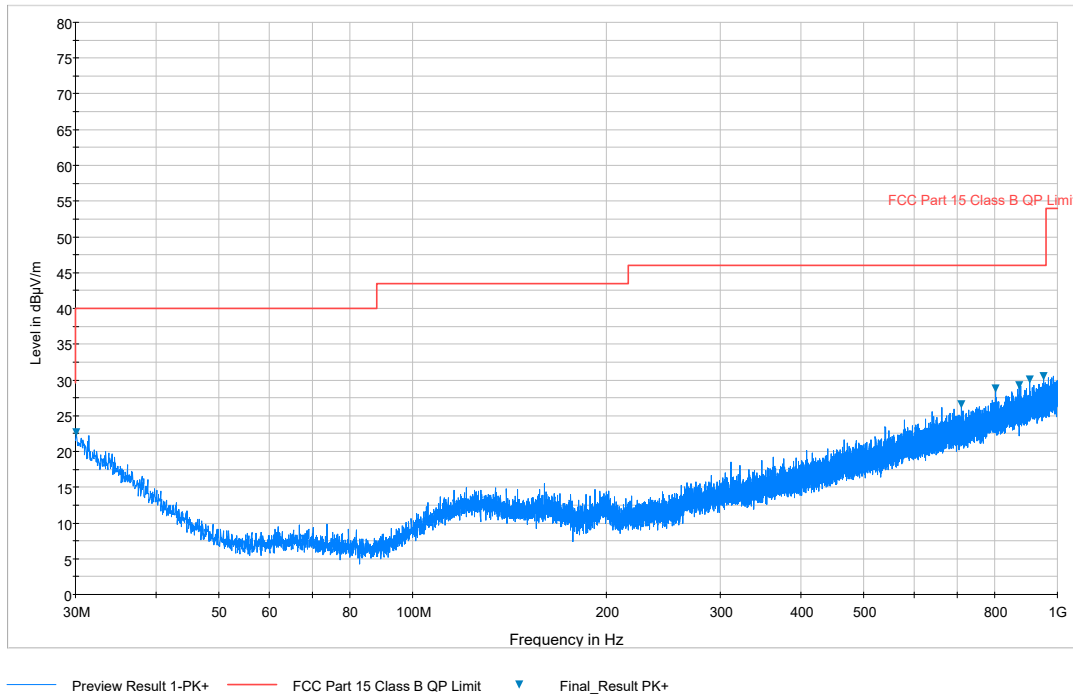
Plot 7-112. Radiated Spurious Plot below 1GHz (802.11a – U3 Ch. 157, Ant. Pol. V)
