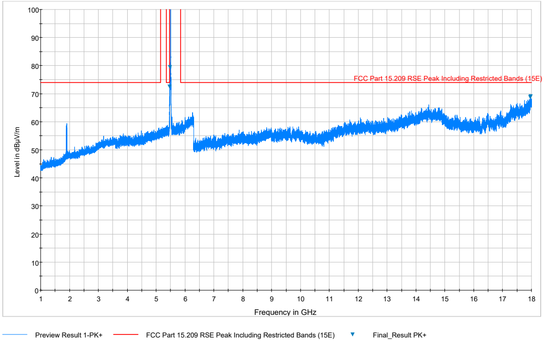
Plot 7-83. Radiated Spurious Plot above 1GHz (802.11a – U2C Ch. 120, Ant. Pol. H)
