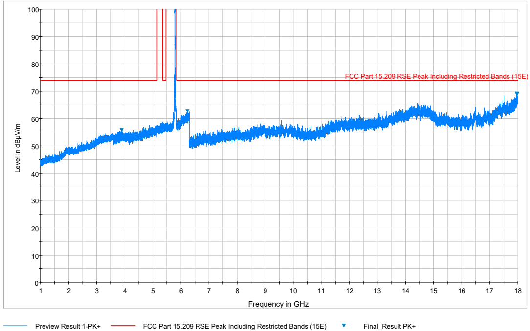
Plot 7-85. Radiated Spurious Plot above 1GHz (802.11a – U3 Ch. 157, Ant. Pol. H)
