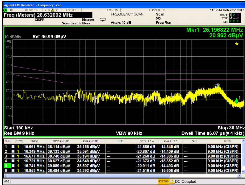
Plot 7-119. Line Conducted Plot with 802.11a UNII Band 3 (L1)
