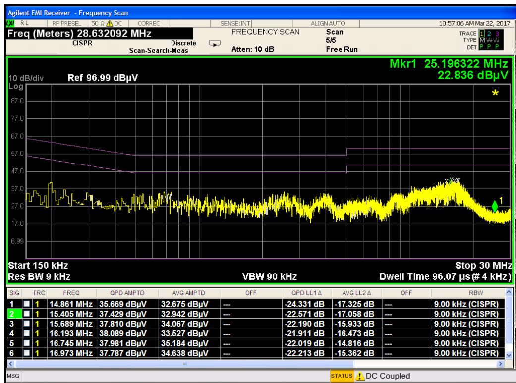
Plot 7-116. Line Conducted Plot with 802.11a UNII Band 2A (N)
