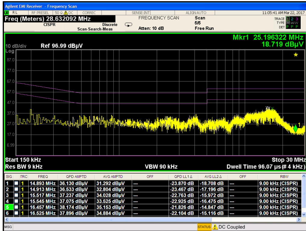
Plot 7-118. Line Conducted Plot with 802.11a UNII Band 2C (N)
