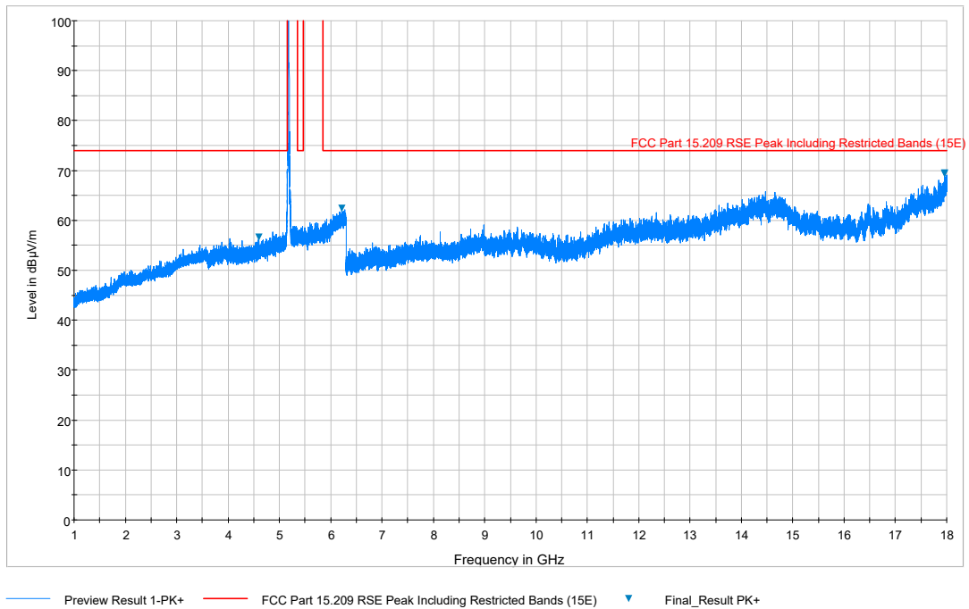
Plot 7-79. Radiated Spurious Plot above 1GHz (802.11a – U1 Ch. 40, Ant. Pol. H)
