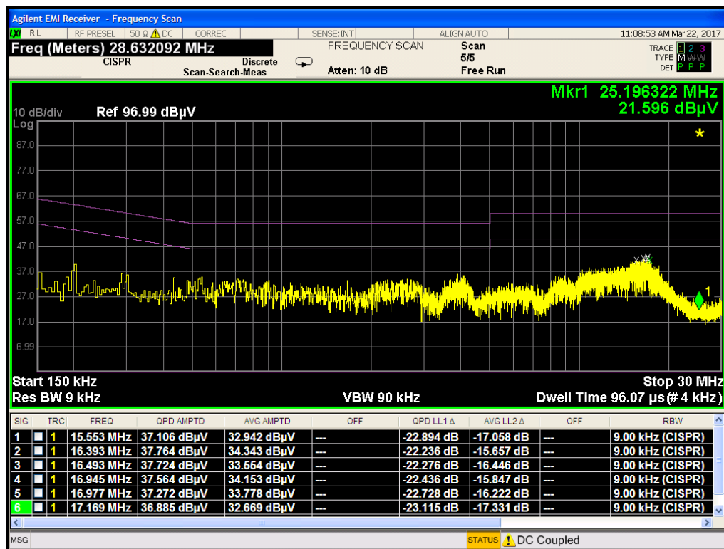
Plot 7-120. Line Conducted Plot with 802.11a UNII Band 3 (N)
