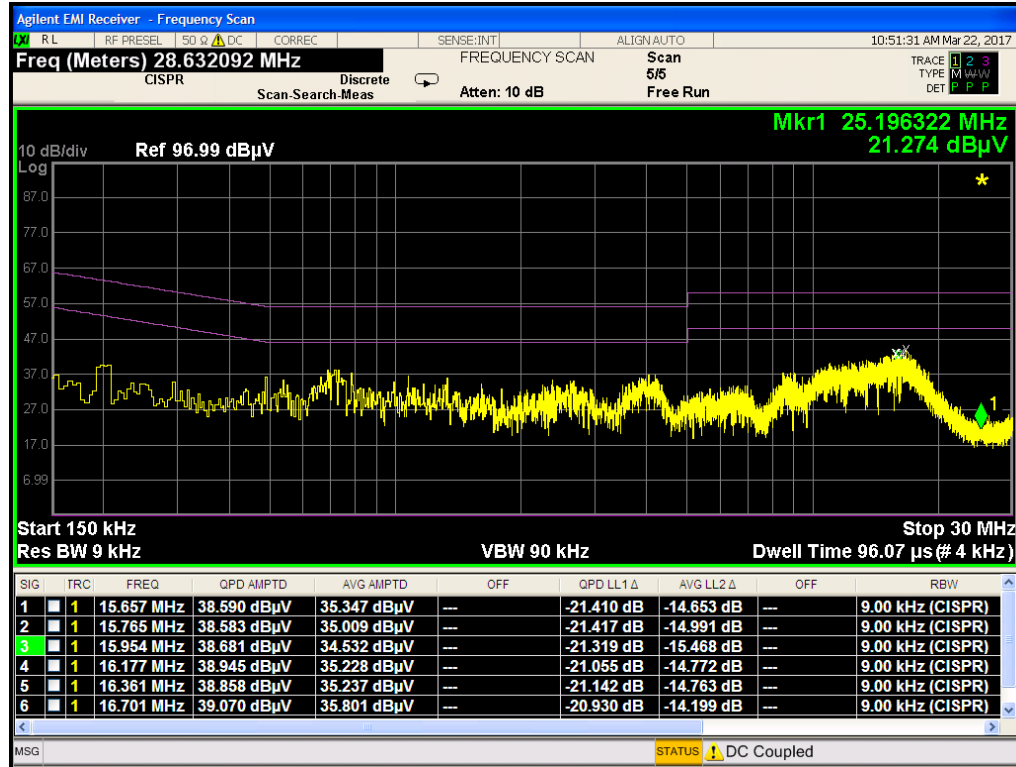
Plot 7-113. Line Conducted Plot with 802.11a UNII Band 1 (L1)
