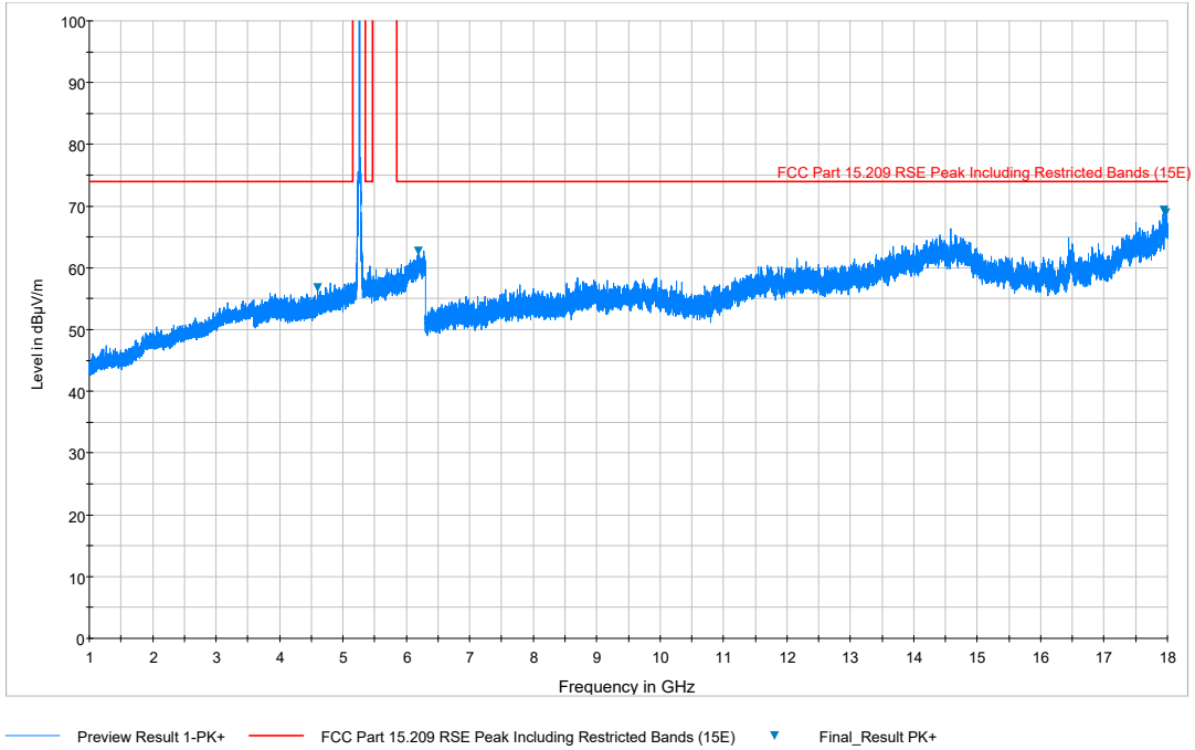
Plot 7-81. Radiated Spurious Plot above 1GHz (802.11a – U2A Ch. 56, Ant. Pol. H)
