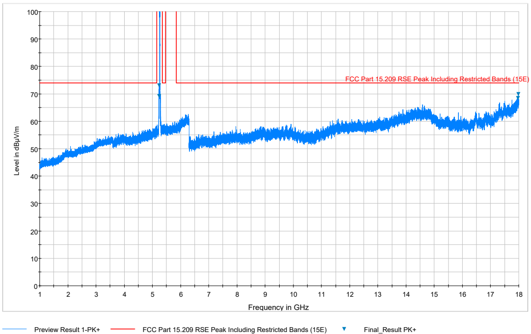
Plot 7-82. Radiated Spurious Plot above 1GHz (802.11a – U2A Ch. 56, Ant. Pol. V)
