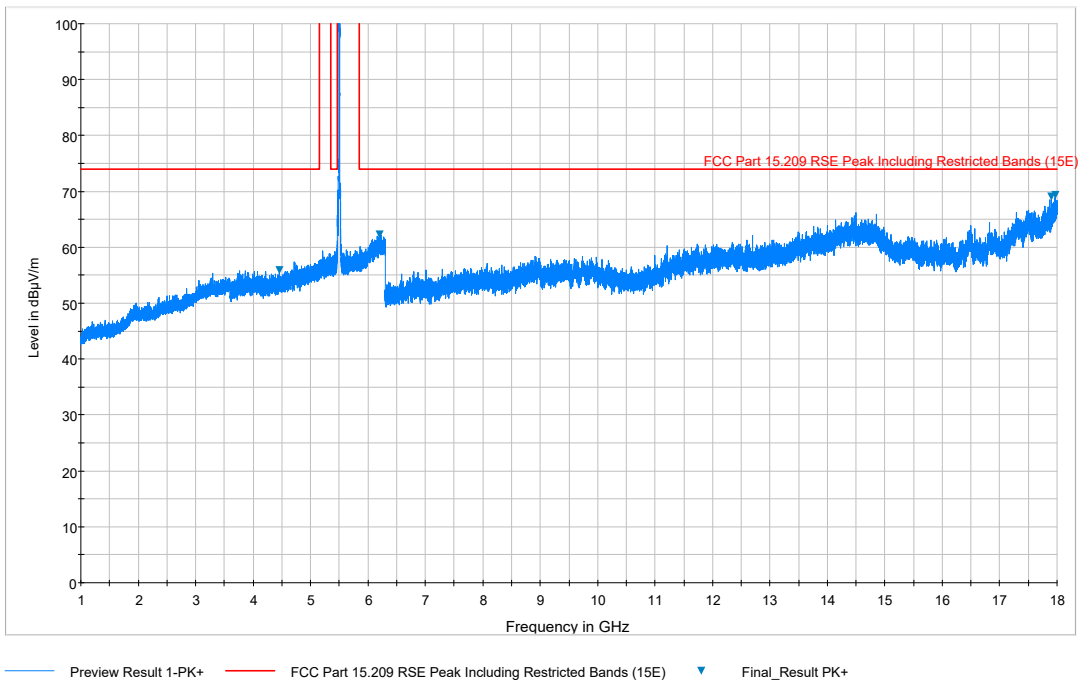
Plot 7-84. Radiated Spurious Plot above 1GHz (802.11a – U2C Ch. 120, Ant. Pol. V)
