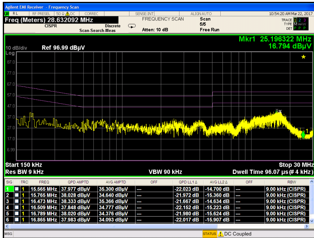
Plot 7-114. Line Conducted Plot with 802.11a UNII Band 1 (N)
