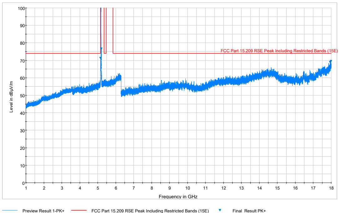
Plot 7-80. Radiated Spurious Plot above 1GHz (802.11a – U1 Ch. 40, Ant. Pol. V)
