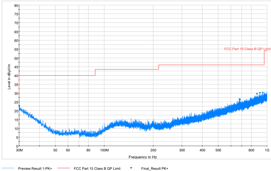
Plot 7-111. Radiated Spurious Plot below 1GHz (802.11a – U3 Ch. 157, Ant. Pol. H)
