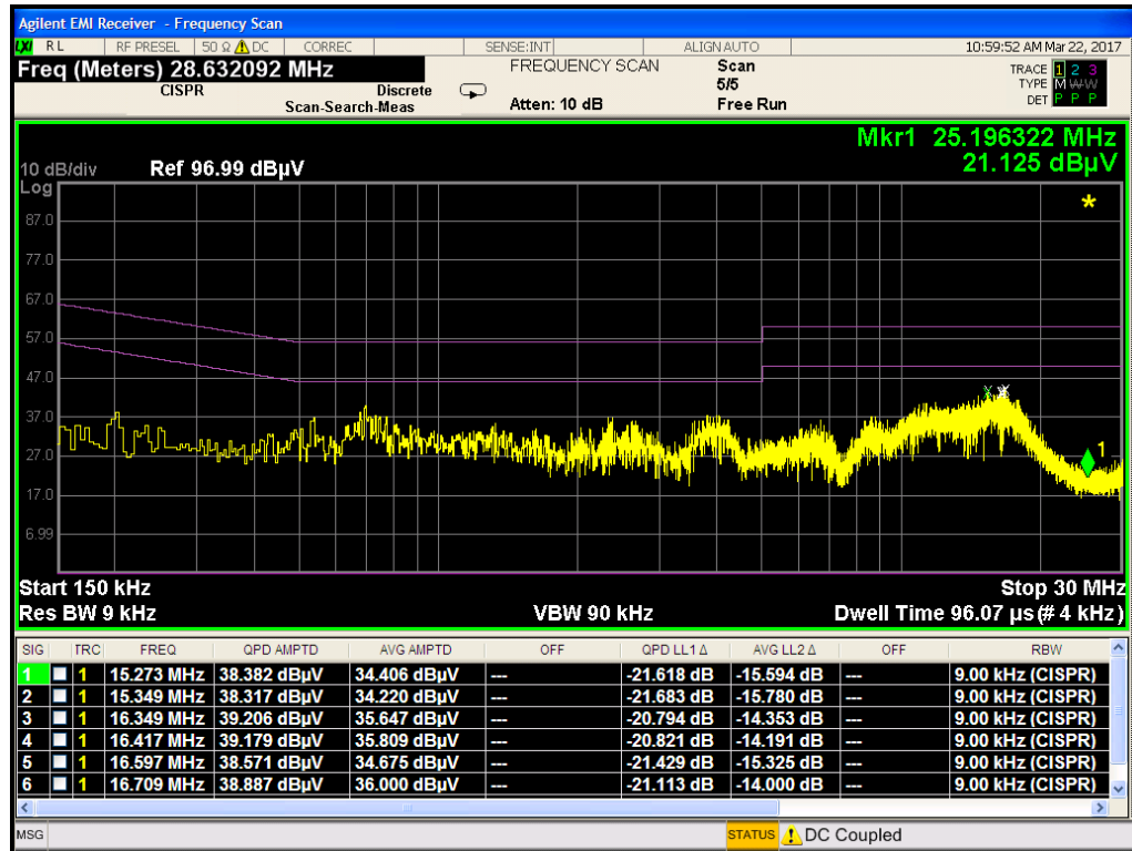
Plot 7-115. Line Conducted Plot with 802.11a UNII Band 2A (L1)
