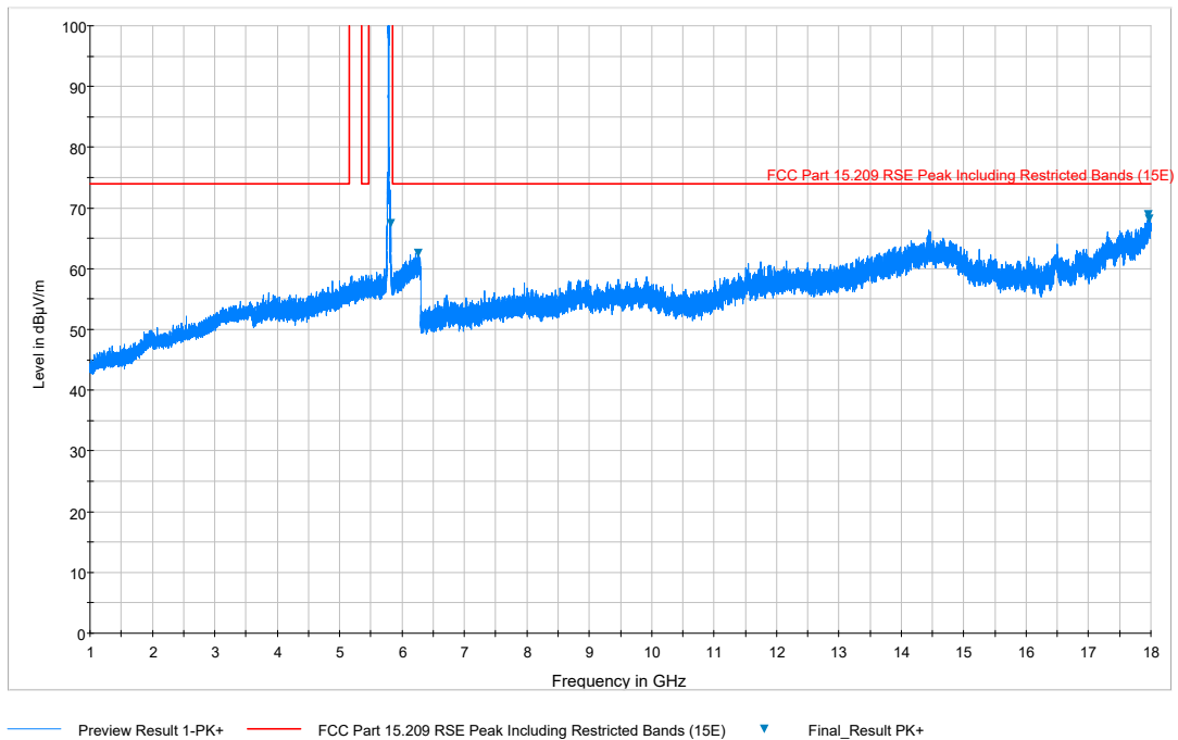
Plot 7-86. Radiated Spurious Plot above 1GHz (802.11a – U3 Ch. 157, Ant. Pol. V)
