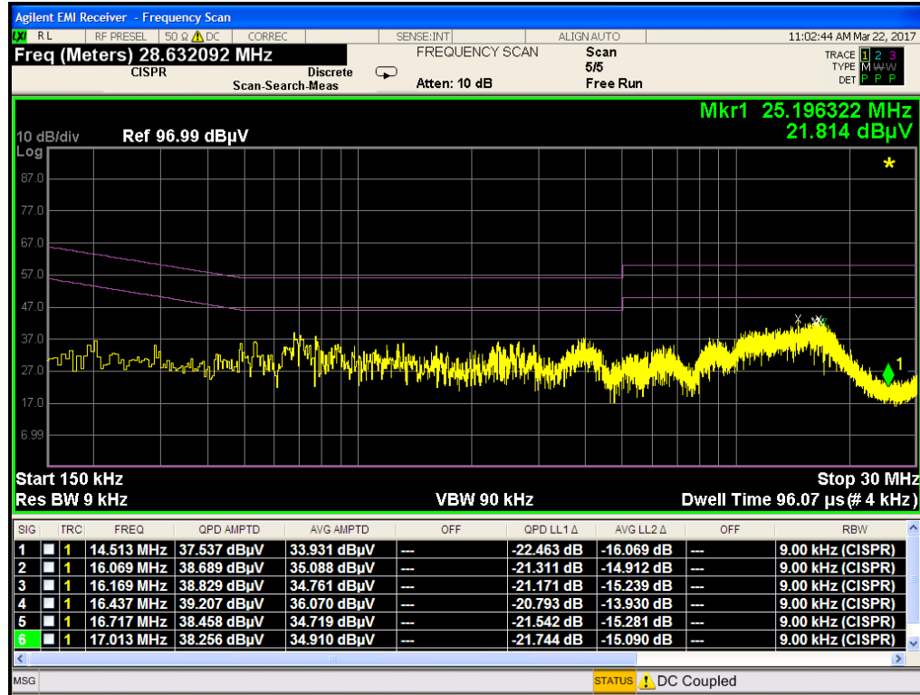
Plot 7-117. Line Conducted Plot with 802.11a UNII Band 2C (L1)
