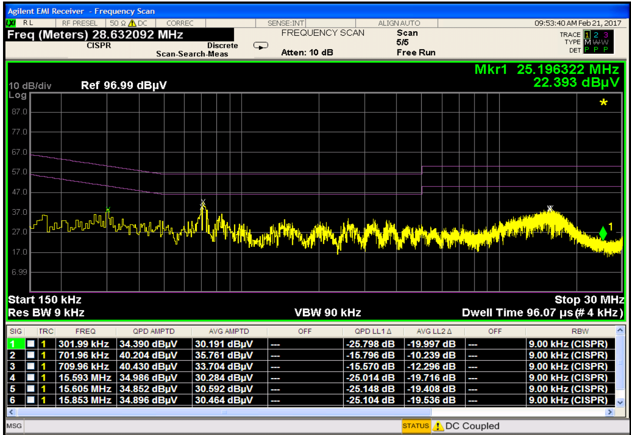
Plot 7-53. Line-Conducted Test Plot (N)
