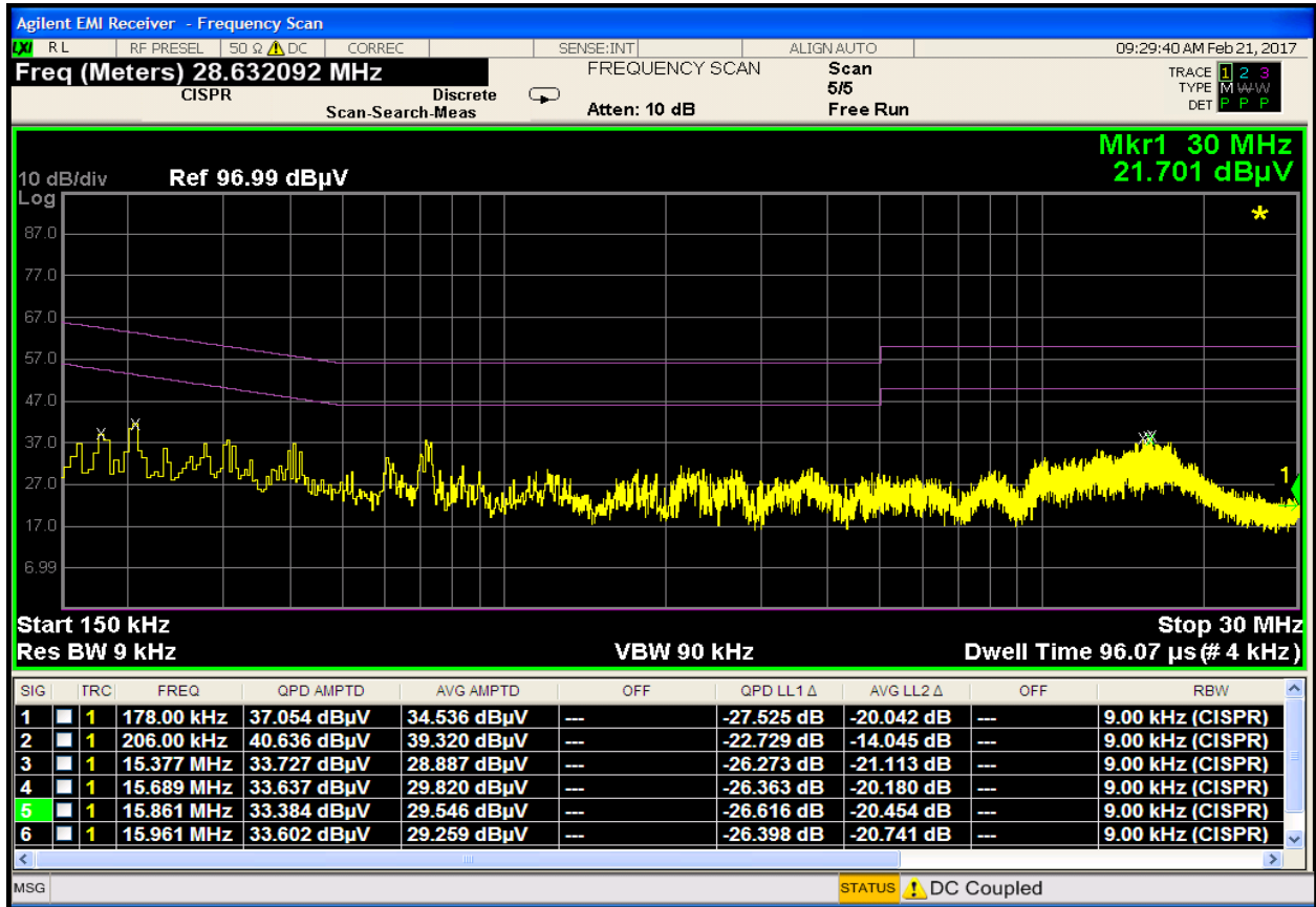
Plot 7-52. Line-Conducted Test Plot (L1)
