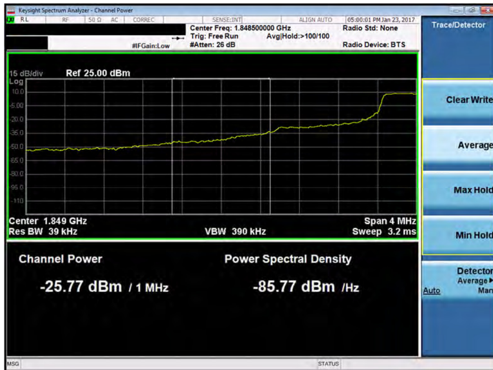
Plot 7-120. Lower Extended Band Edge Plot (Band 2 – 1.4MHz QPSK – RB Size 6)
