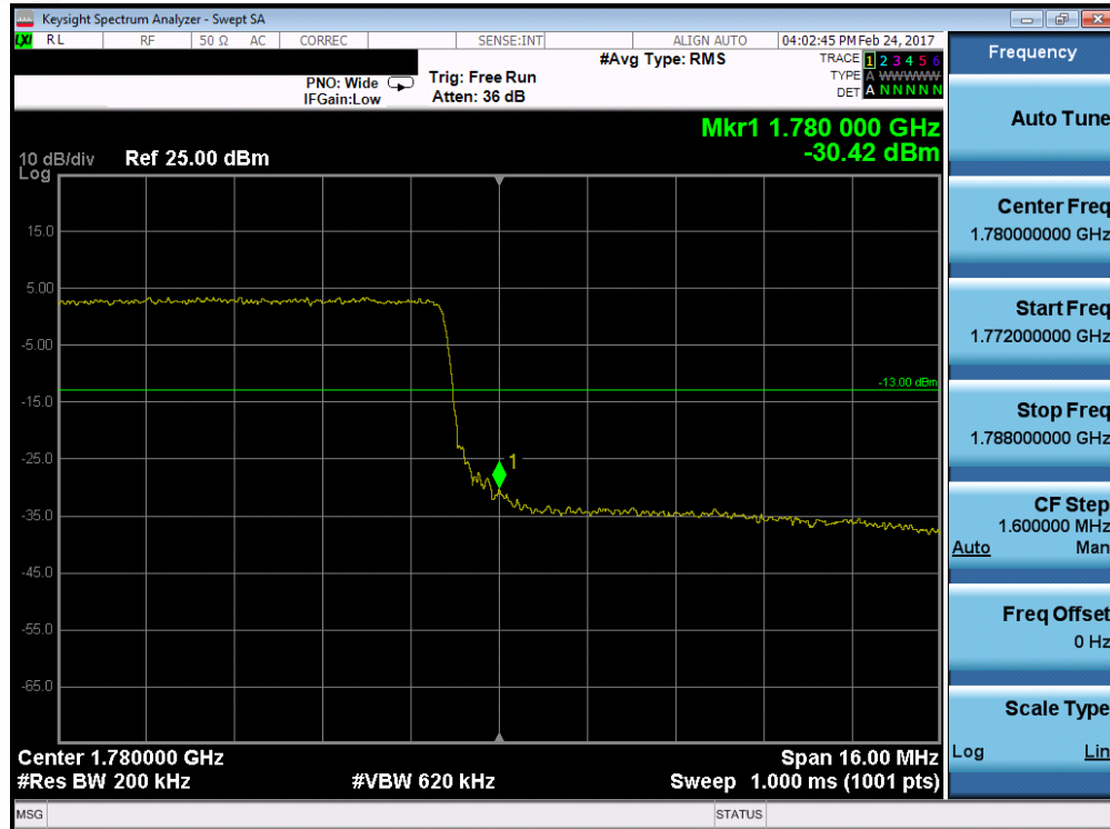
Plot 7-117. Upper Band Edge Plot (Band 4/66 – 20.0MHz QPSK – RB Size 100)
