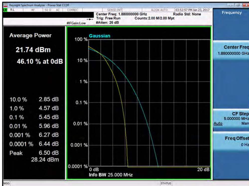
Plot 7-154. PAR Plot (Band 2 – 20.0MHz 16-QAM – RB Size 100)
