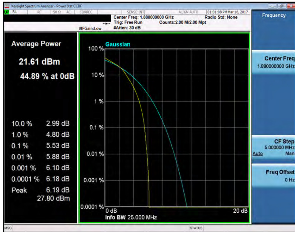
Plot 7-152. PAR Plot (Band 2 – 15.0MHz 16-QAM – RB Size 75)
