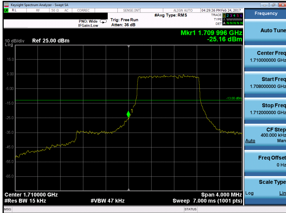
Plot 7-95. Lower Band Edge Plot (Band 4/66 – 1.4MHz QPSK – RB Size 6)
