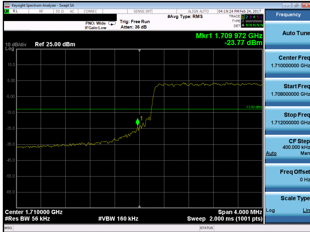
Plot 7-103. Lower Band Edge Plot (Band 4/66 – 5.0MHz QPSK – RB Size 25)
