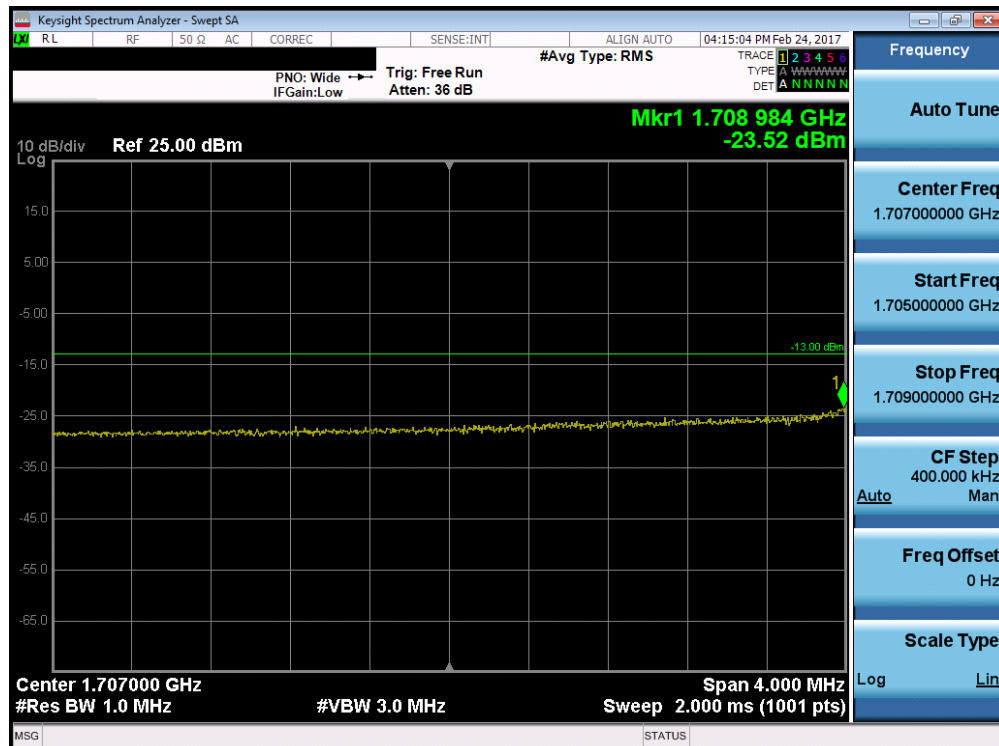
Plot 7-108. Lower Extended Band Edge Plot (Band 4/66 – 10.0MHz QPSK – RB Size 50)
