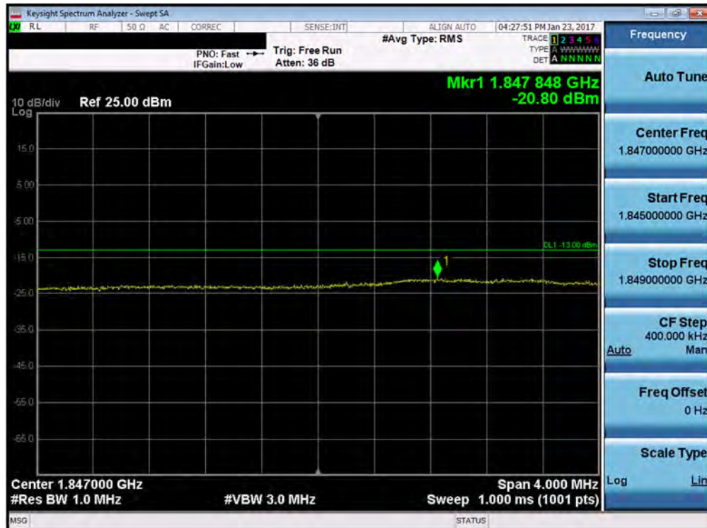
Plot 7-136. Lower Extended Band Edge Plot (Band 2 – 15.0MHz QPSK – RB Size 75)
