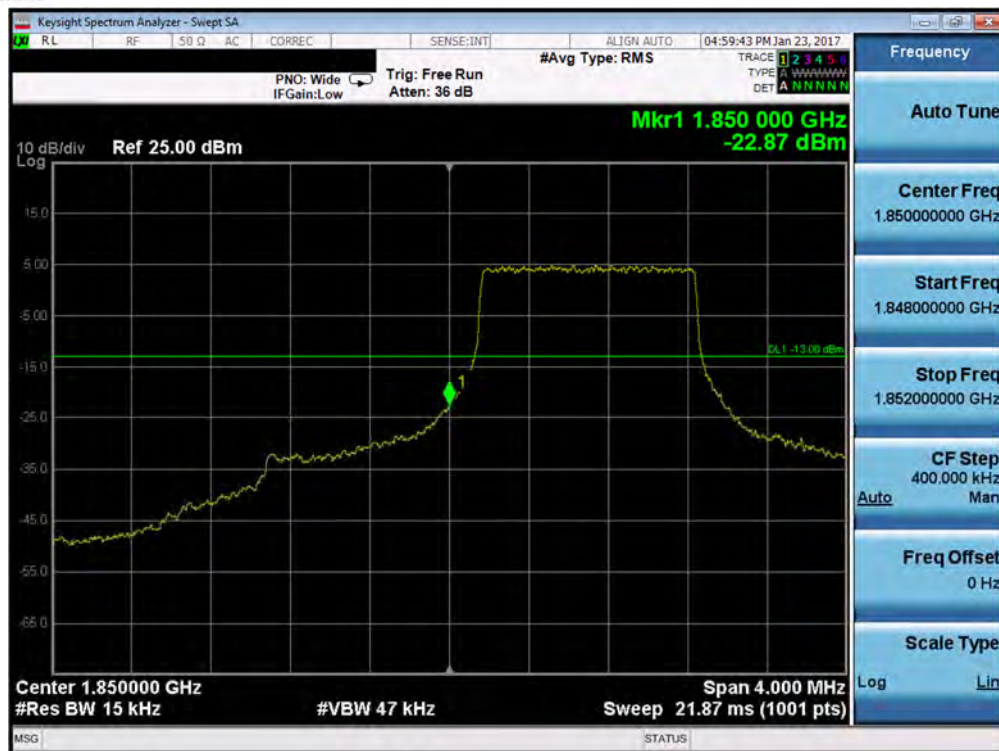
Plot 7-119. Lower Band Edge Plot (Band 2 – 1.4MHz QPSK – RB Size 6)
