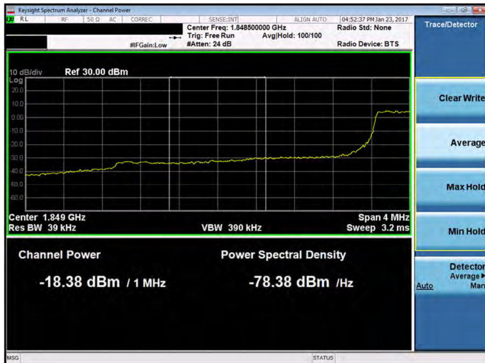
Plot 7-124. Lower Extended Band Edge Plot (Band 2 – 3.0MHz QPSK – RB Size 15)
