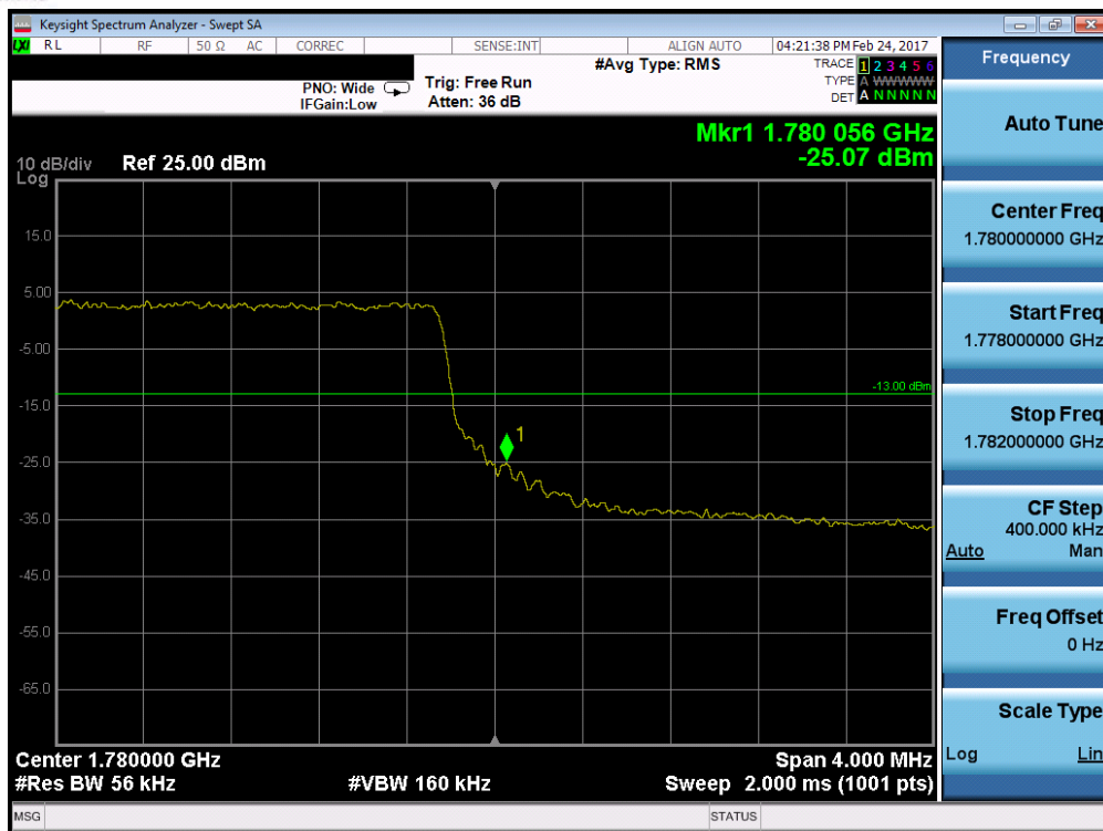
Plot 7-105. Upper Band Edge Plot (Band 4/66 – 5.0MHz QPSK – RB Size 25)
