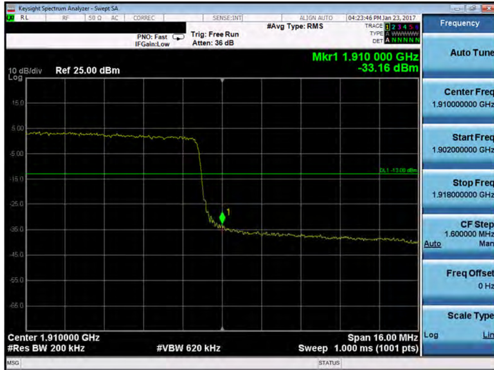
Plot 7-141. Upper Band Edge Plot (Band 2 – 20.0MHz QPSK – RB Size 100)
