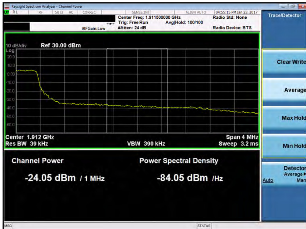
Plot 7-126. Upper Extended Band Edge Plot (Band 2 – 3.0MHz QPSK – RB Size 15)
