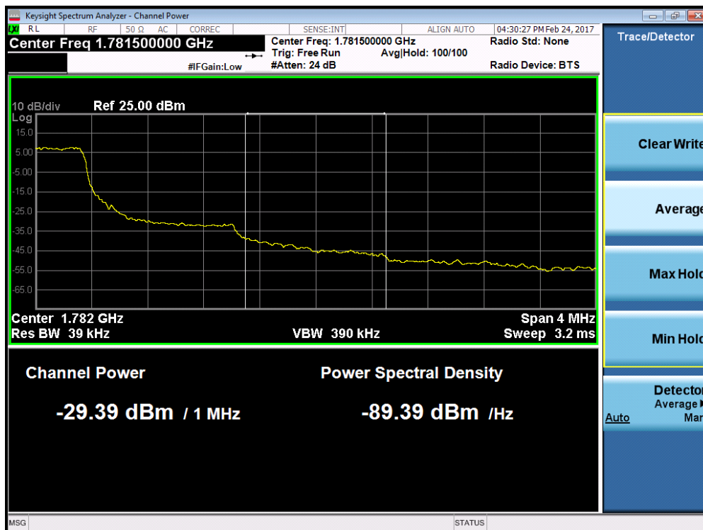
Plot 7-98. Upper Extended Band Edge Plot (Band 4/66 – 1.4MHz QPSK – RB Size 6)
