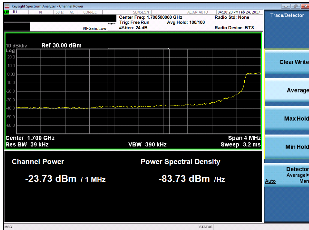
Plot 7-104. Lower Extended Band Edge Plot (Band 4/66 – 5.0MHz QPSK – RB Size 25)
