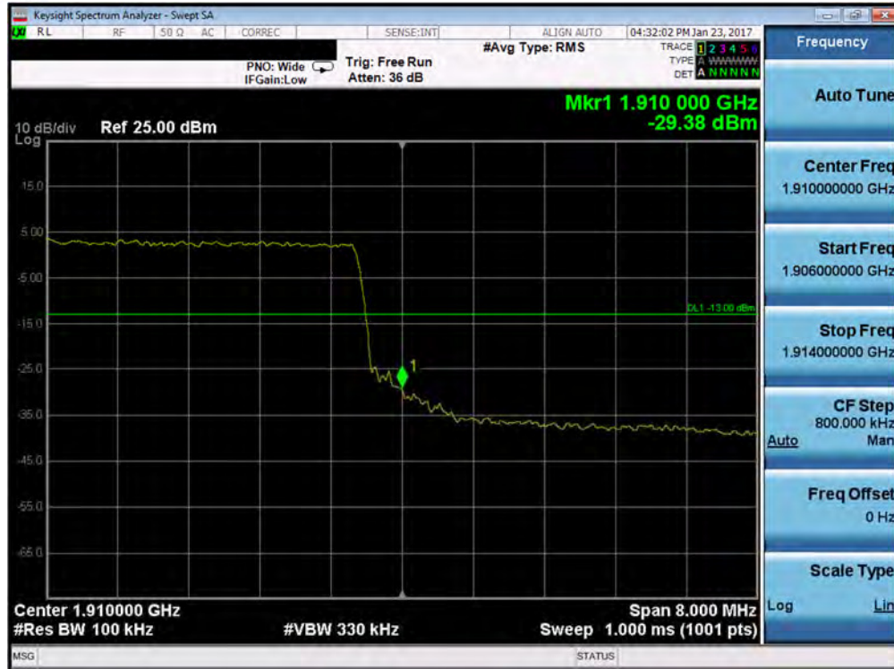
Plot 7-133. Upper Band Edge Plot (Band 2 – 10.0MHz QPSK – RB Size 50)
