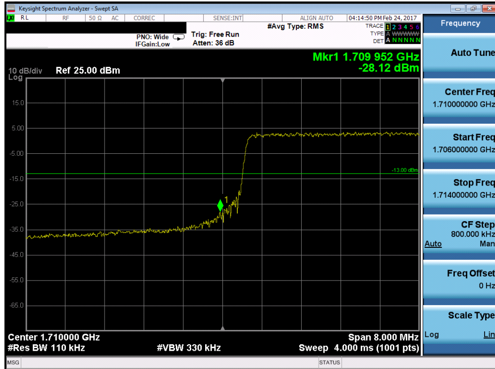
Plot 7-107. Lower Band Edge Plot (Band 4/66 – 10.0MHz QPSK – RB Size 50)
