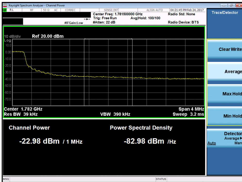
Plot 7-106. Upper Extended Band Edge Plot (Band 4/66 – 5.0MHz QPSK – RB Size 25)
