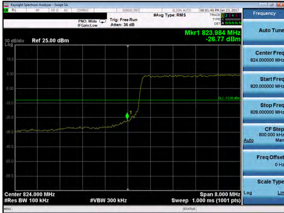
Plot 7-93. Lower Band Edge Plot (Band 5 - 10.0MHz QPSK - RB Size 50)
