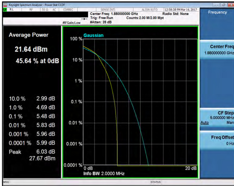
Plot 7-144. PAR Plot (Band 2 – 1.4MHz 16-QAM – RB Size 6)
