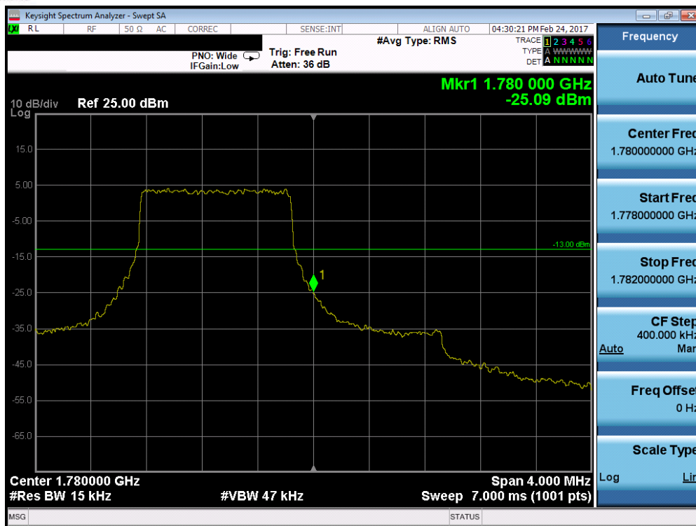
Plot 7-97. Upper Band Edge Plot (Band 4/66 – 1.4MHz QPSK – RB Size 6)
