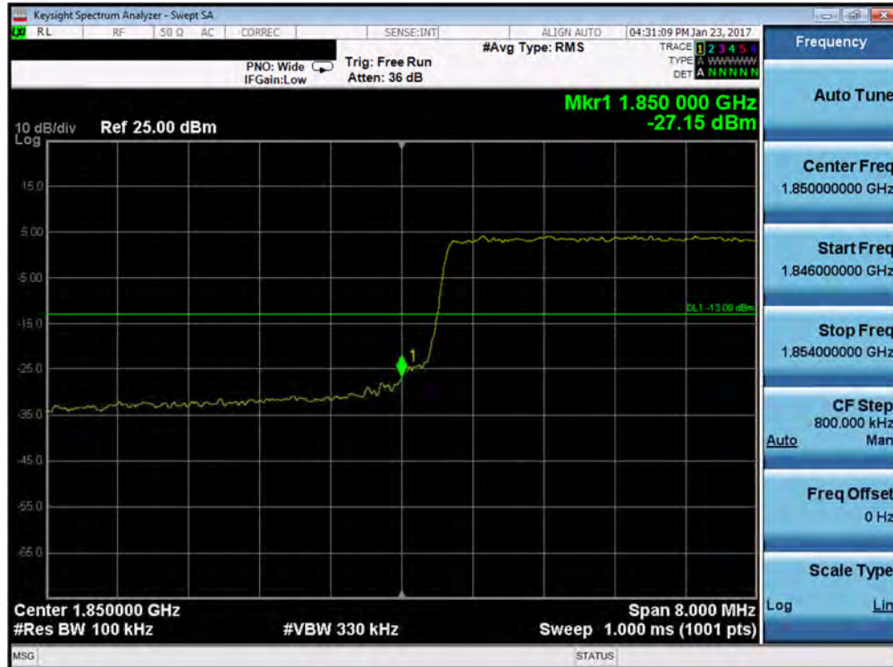
Plot 7-131. Lower Band Edge Plot (Band 2 – 10.0MHz QPSK – RB Size 50)
