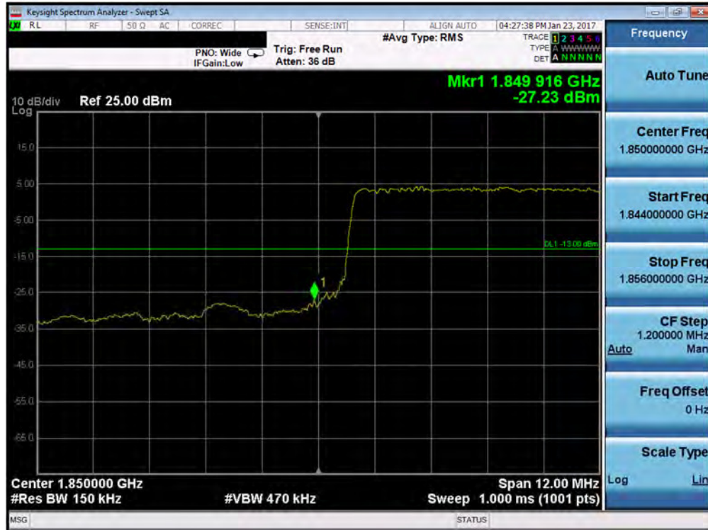
Plot 7-135. Lower Band Edge Plot (Band 2 – 15.0MHz QPSK – RB Size 75)
