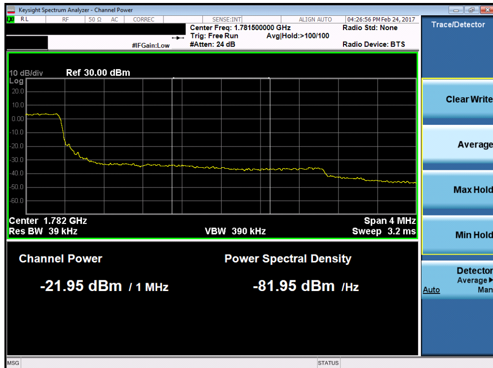
Plot 7-102. Upper Extended Band Edge Plot (Band 4/66 – 3.0MHz QPSK – RB Size 15)
