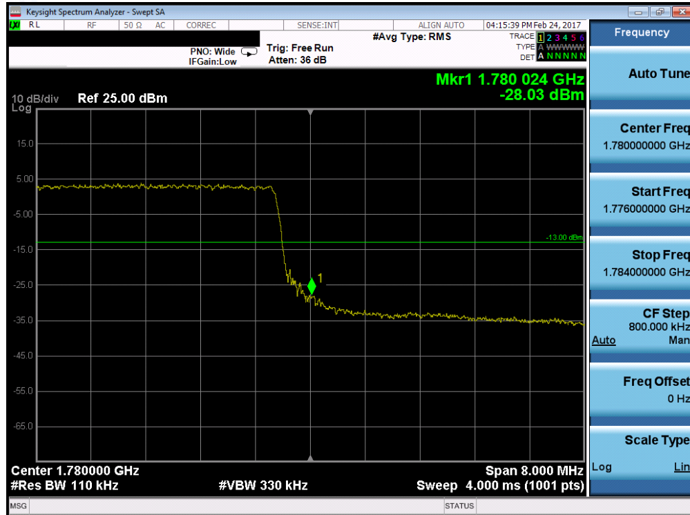
Plot 7-109. Upper Band Edge Plot (Band 4/66 – 10.0MHz QPSK – RB Size 50)
