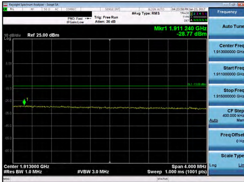
Plot 7-142. Upper Extended Band Edge Plot (Band 2 – 20.0MHz QPSK – RB Size 100)
