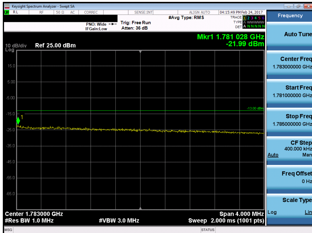
Plot 7-110. Upper Extended Band Edge Plot (Band 4/66 – 10.0MHz QPSK – RB Size 50)
