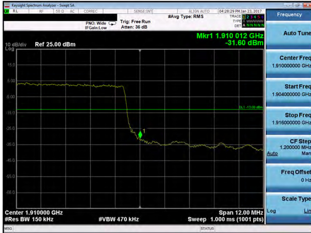
Plot 7-137. Upper Band Edge Plot (Band 2 – 15.0MHz QPSK – RB Size 75)
