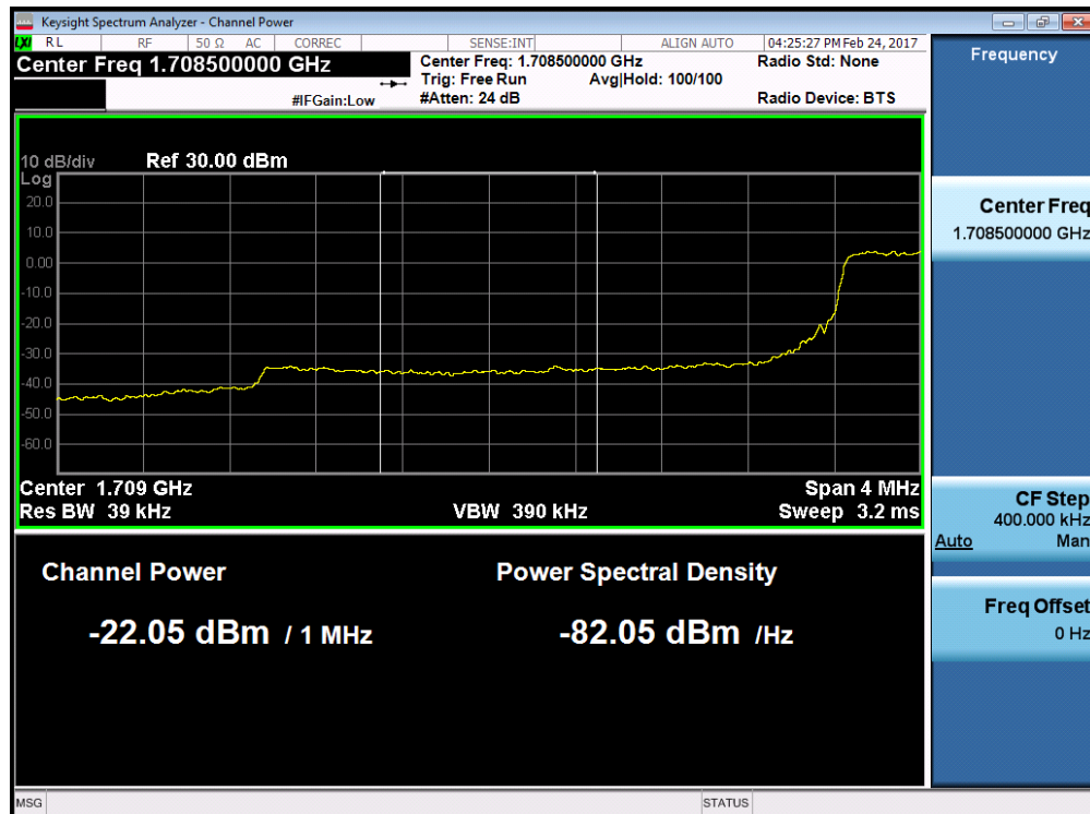
Plot 7-100. Lower Extended Band Edge Plot (Band 4/66 – 3.0MHz QPSK – RB Size 15)
