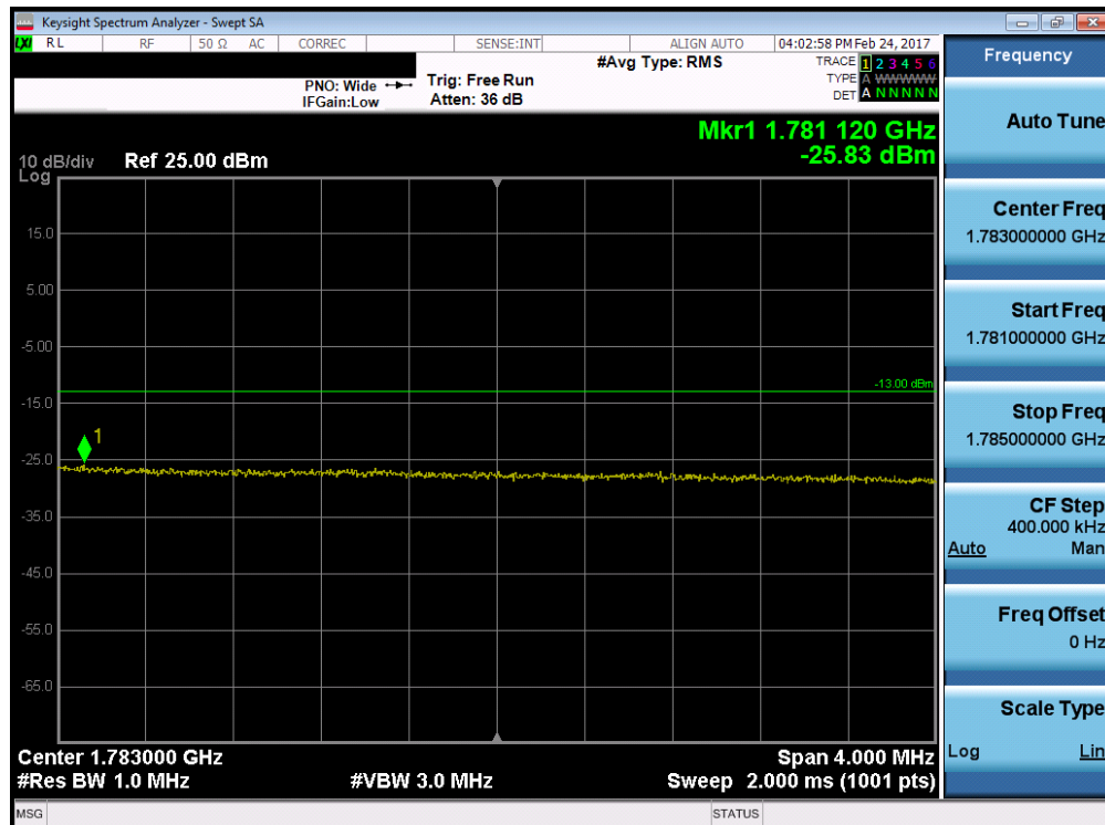
Plot 7-118. Upper Extended Band Edge Plot (Band 4/66 – 20.0MHz QPSK – RB Size 100)
