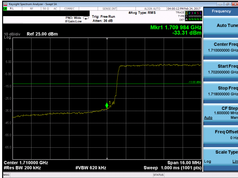
Plot 7-115. Lower Band Edge Plot (Band 4/66 – 20.0MHz QPSK – RB Size 100)
