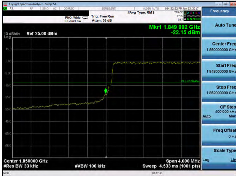
Plot 7-123. Lower Band Edge Plot (Band 2 – 3.0MHz QPSK – RB Size 15)
