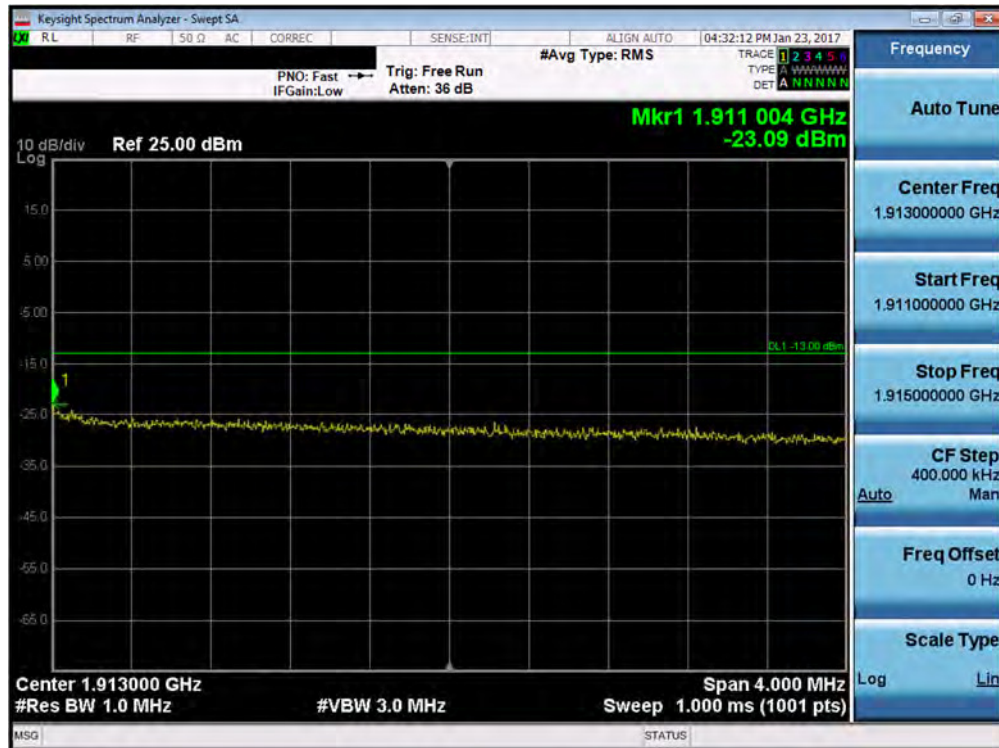
Plot 7-134. Upper Extended Band Edge Plot (Band 2 – 10.0MHz QPSK – RB Size 50)
