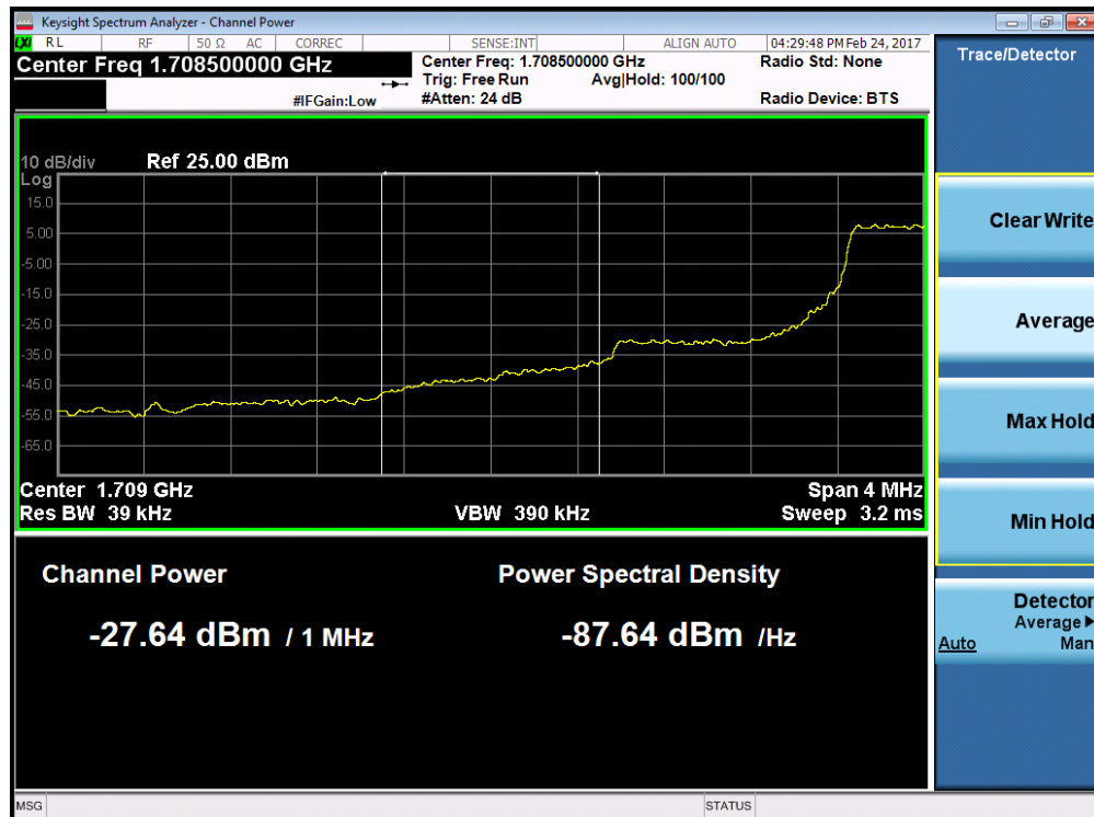
Plot 7-96. Lower Extended Band Edge Plot (Band 4/66 – 1.4MHz QPSK – RB Size 6)
