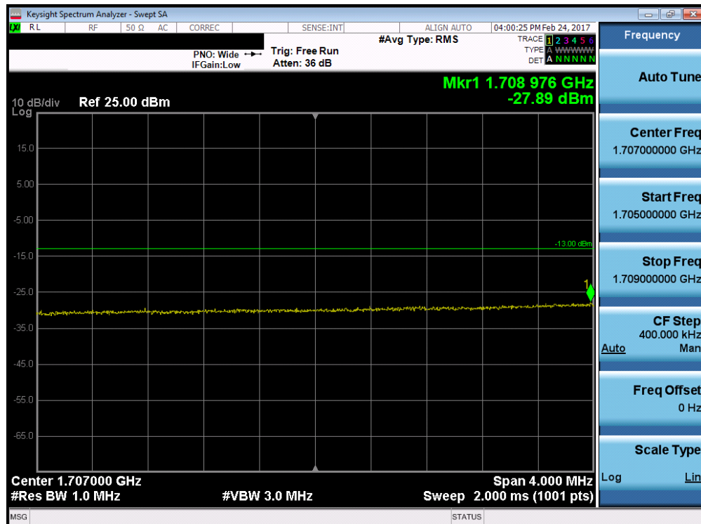
Plot 7-116. Lower Extended Band Edge Plot (Band 4/66 – 20.0MHz QPSK – RB Size 100)
