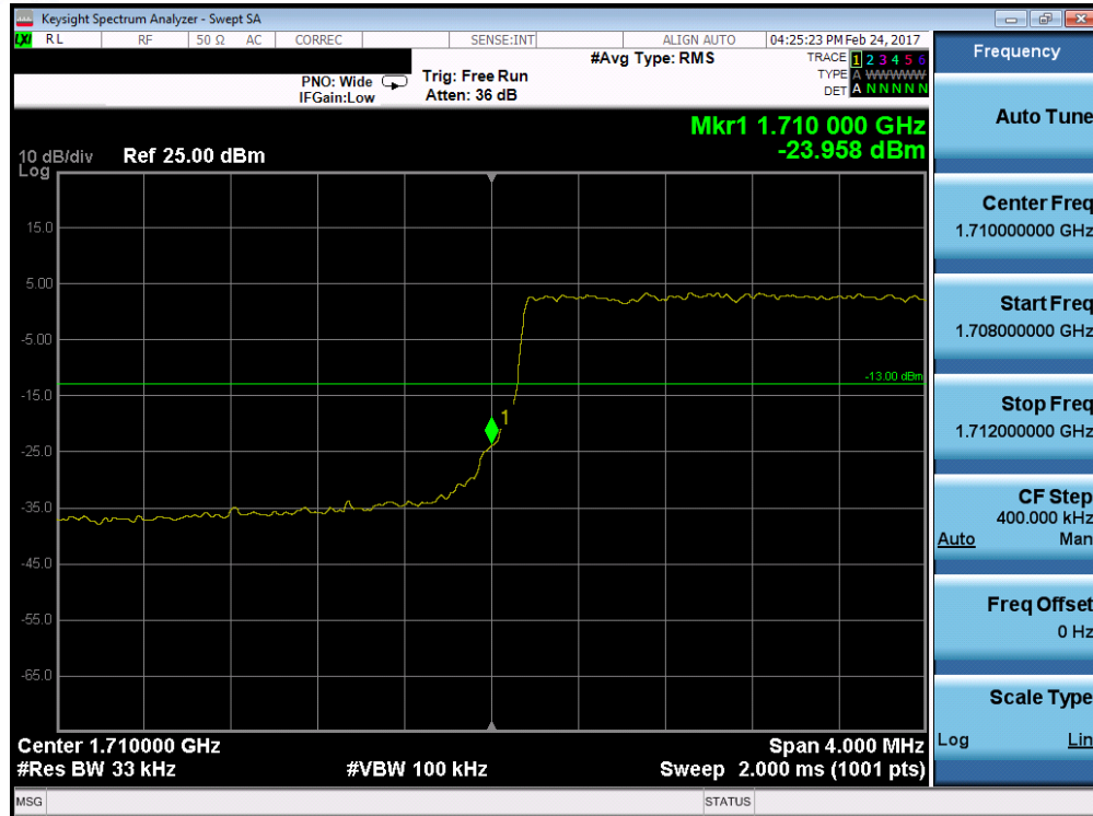
Plot 7-99. Lower Band Edge Plot (Band 4/66 – 3.0MHz QPSK – RB Size 15)
