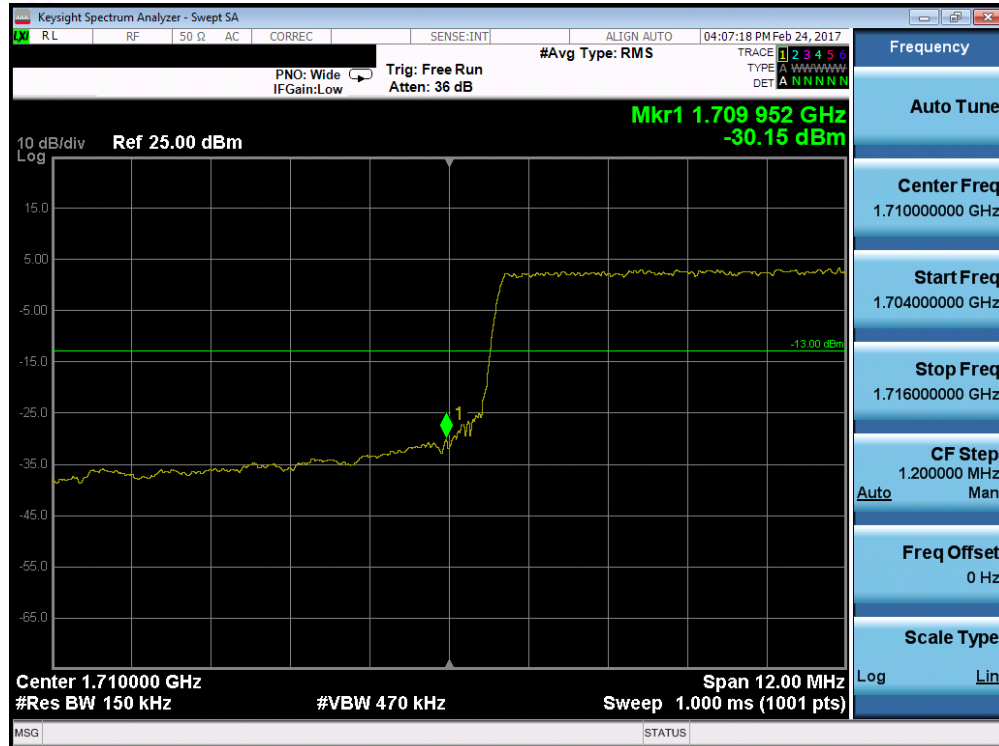
Plot 7-111. Lower Band Edge Plot (Band 4/66 – 15.0MHz QPSK – RB Size 75)
