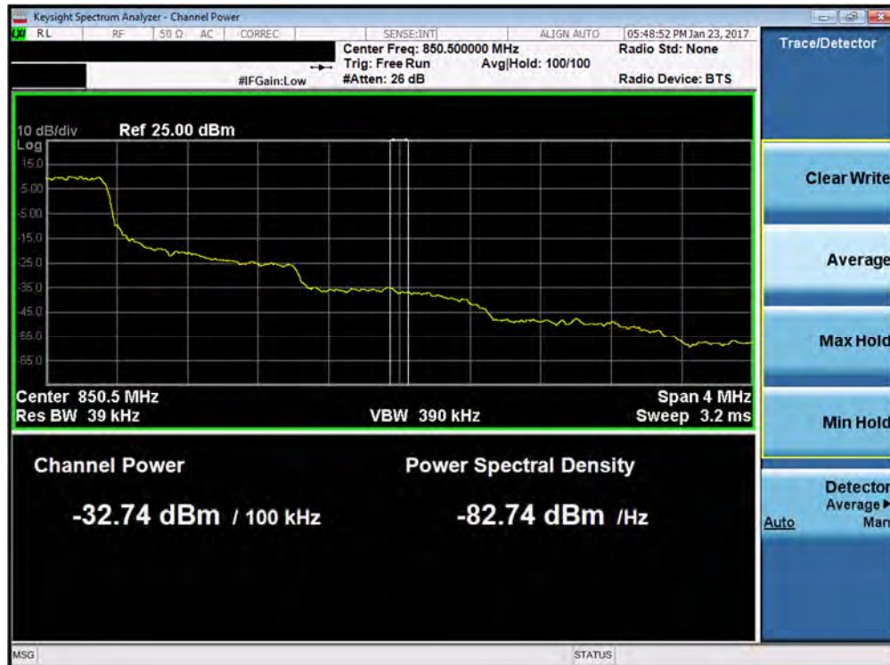
Plot 7-88. Upper Extended Band Edge Plot (Band 5 – 1.4MHz QPSK – RB Size 6)
