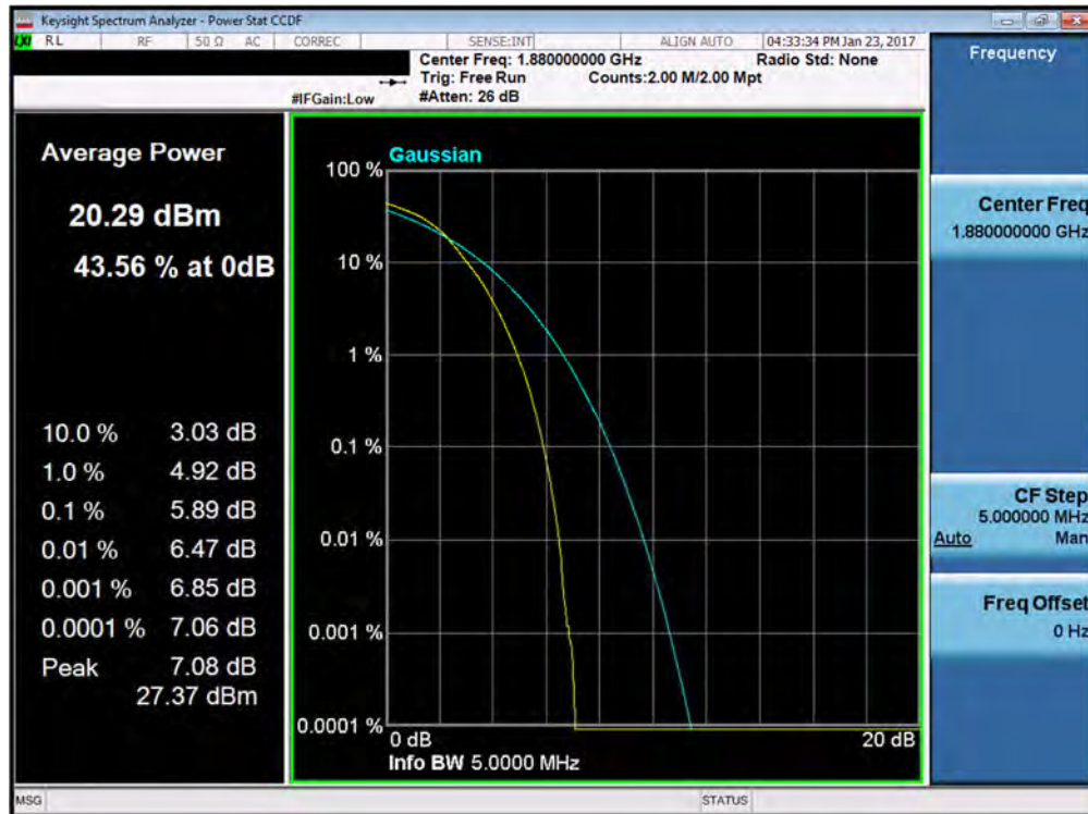
Plot 7-148. PAR Plot (Band 2 – 5.0MHz 16-QAM – RB Size 25)
