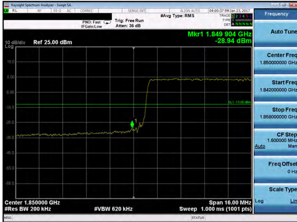
Plot 7-139. Lower Band Edge Plot (Band 2 - 20.0MHz QPSK - RB Size 100)
