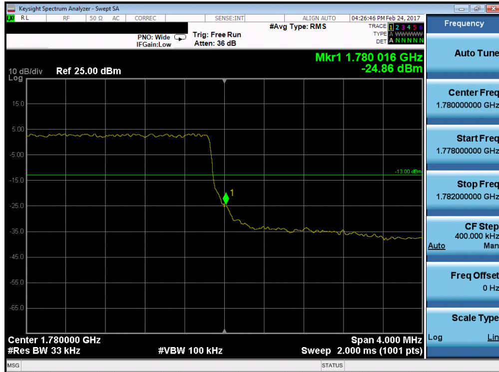
Plot 7-101. Upper Band Edge Plot (Band 4/66 – 3.0MHz QPSK – RB Size 15)
