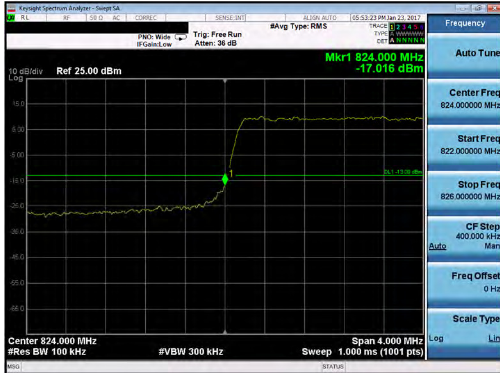
Plot 7-89. Lower Band Edge Plot (Band 5 - 3.0MHz QPSK - RB Size 15)
