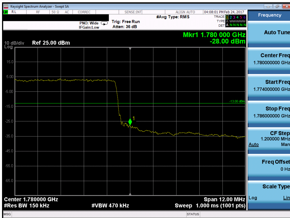
Plot 7-113. Upper Band Edge Plot (Band 4/66 – 15.0MHz QPSK – RB Size 75)
