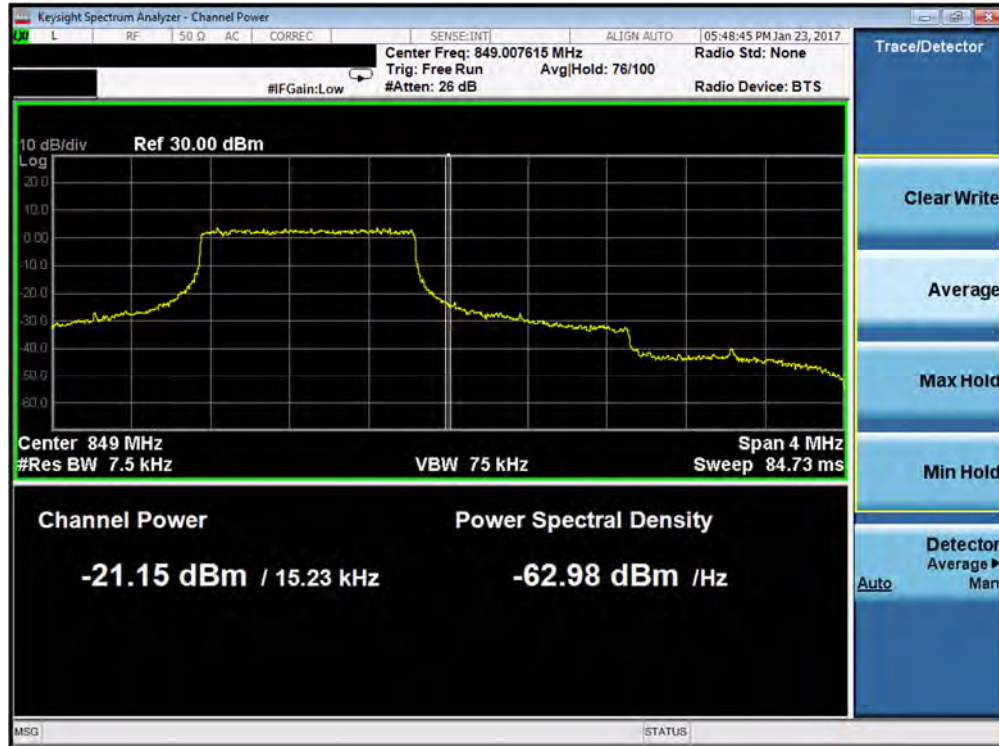
Plot 7-87. Upper Band Edge Plot (Band 5 – 1.4MHz QPSK – RB Size 6)
