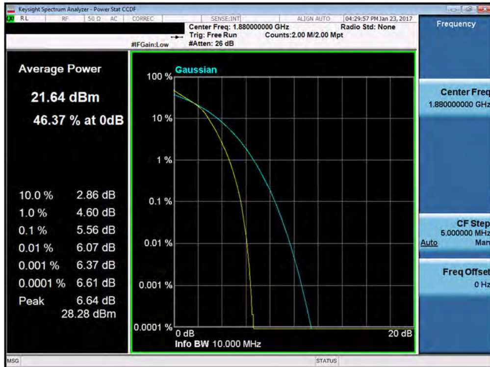
Plot 7-150. PAR Plot (Band 2 – 10.0MHz 16-QAM – RB Size 50)
