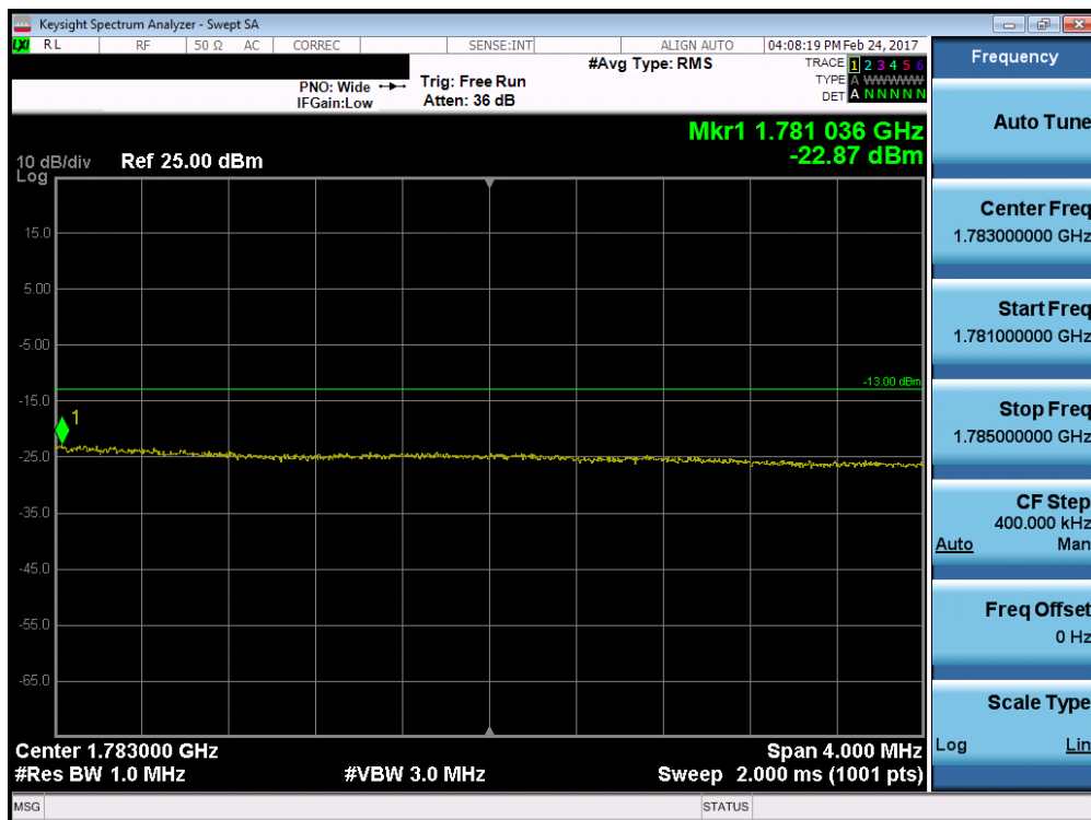
Plot 7-114. Upper Extended Band Edge Plot (Band 4/66 – 15.0MHz QPSK – RB Size 75)
