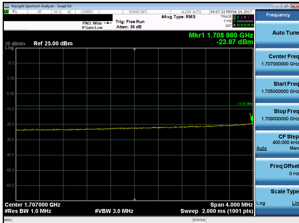
Plot 7-112. Lower Extended Band Edge Plot (Band 4/66 – 15.0MHz QPSK – RB Size 75)
