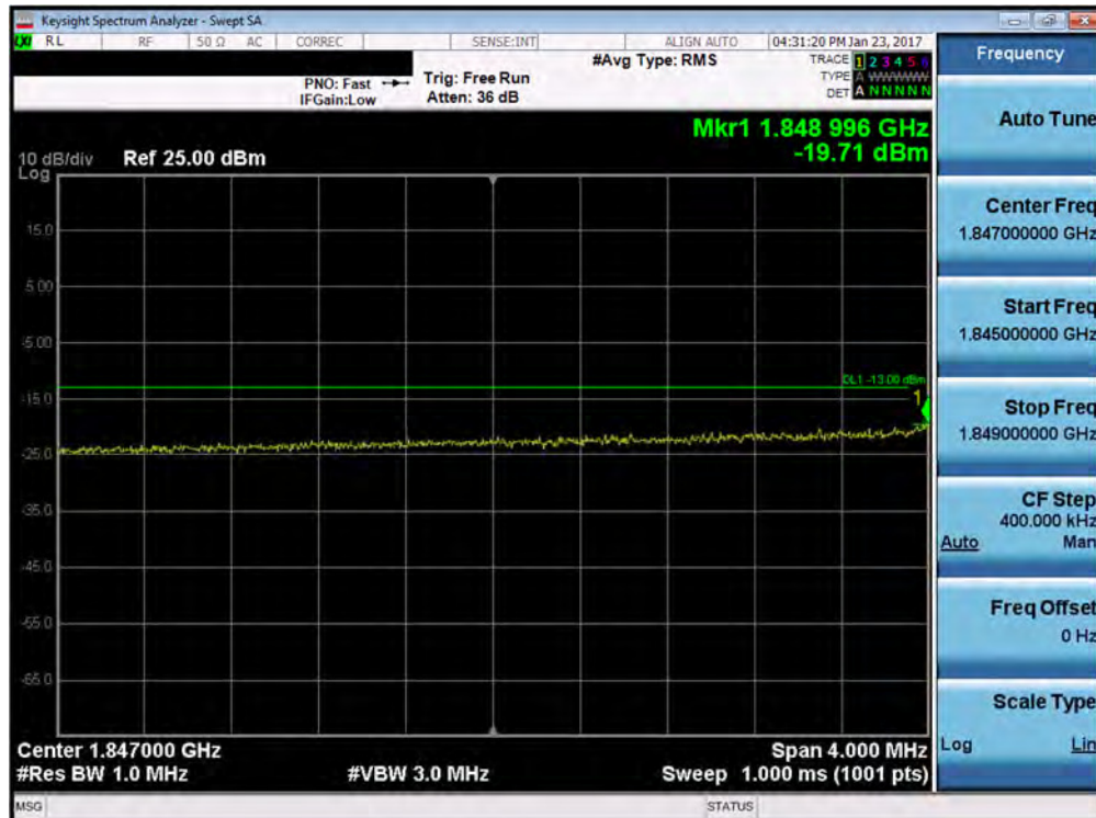
Plot 7-132. Lower Extended Band Edge Plot (Band 2 – 10.0MHz QPSK – RB Size 50)
