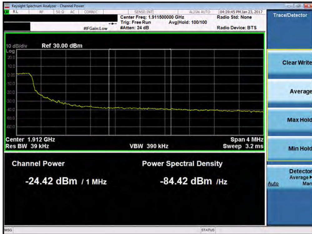
Plot 7-130. Upper Extended Band Edge Plot (Band 2 – 5.0MHz QPSK – RB Size 25)
