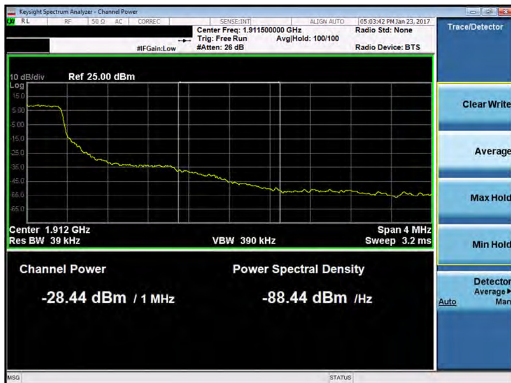
Plot 7-122. Upper Extended Band Edge Plot (Band 2 – 1.4MHz QPSK – RB Size 6)
