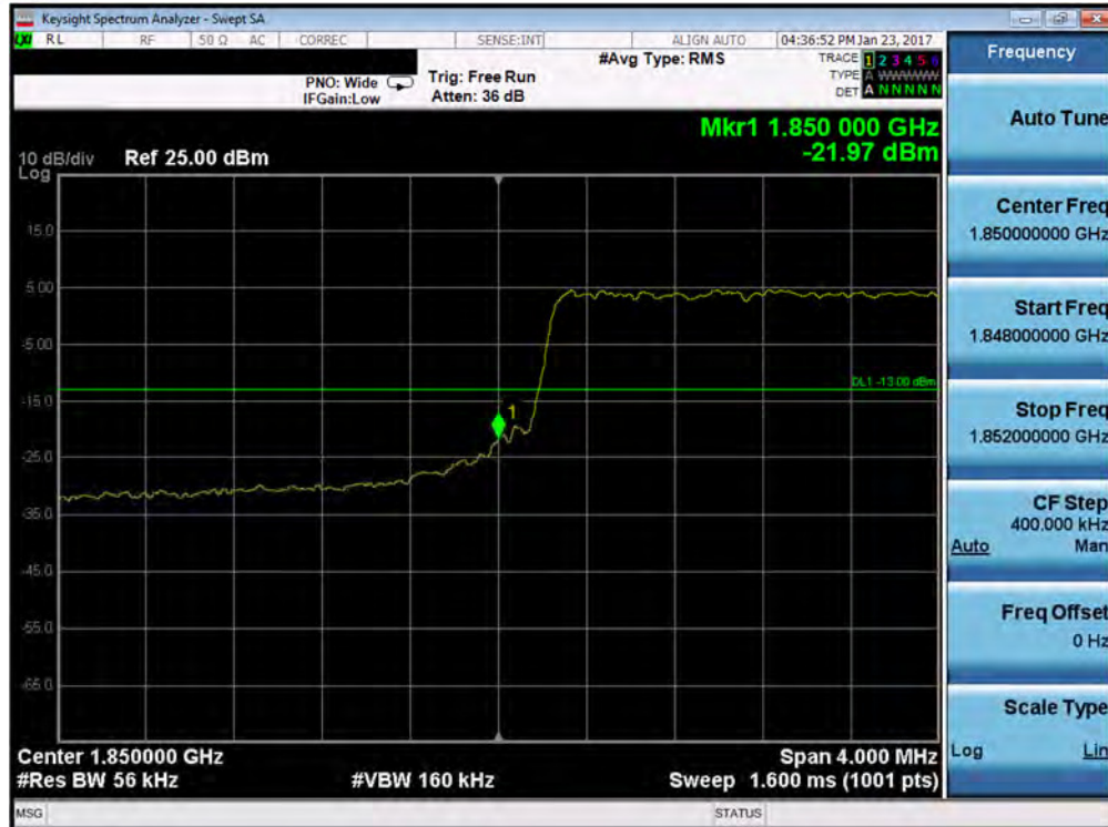
Plot 7-127. Lower Band Edge Plot (Band 2 – 5.0MHz QPSK – RB Size 25)
