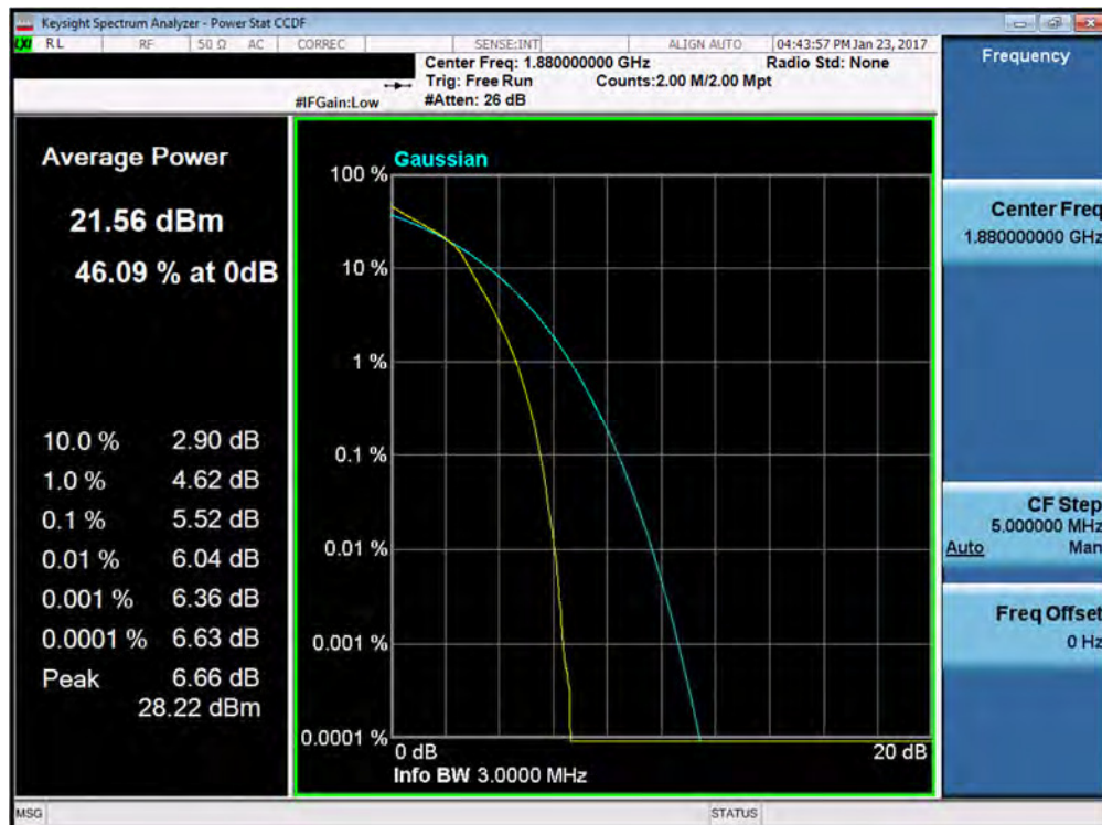
Plot 7-146. PAR Plot (Band 2 – 3.0MHz 16-QAM – RB Size 15)
