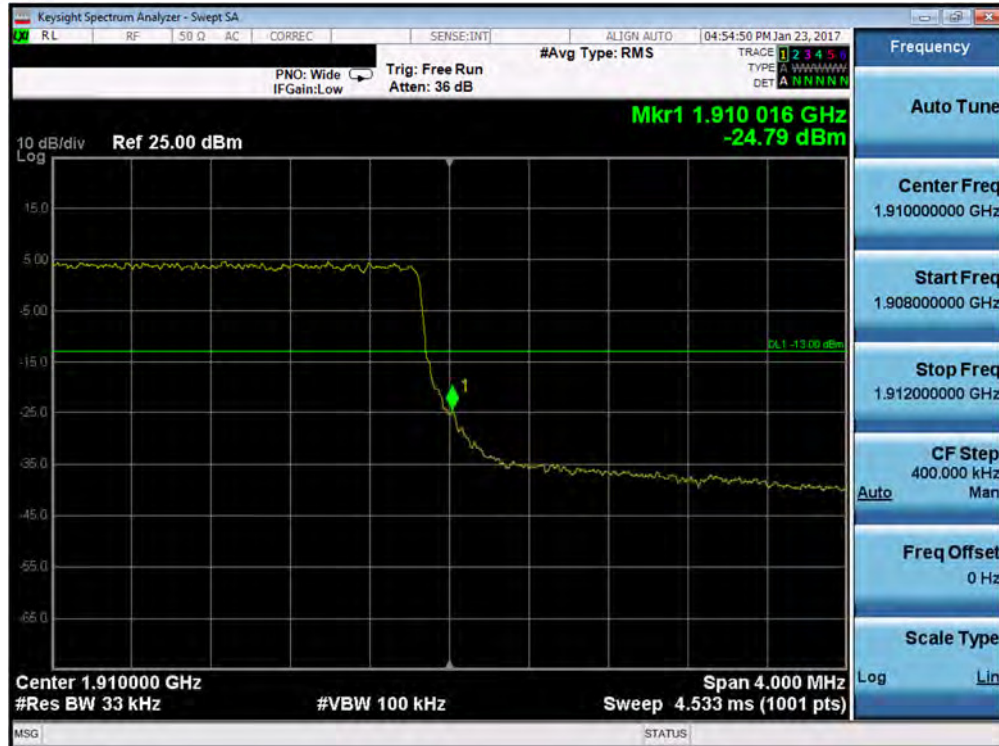
Plot 7-125. Upper Band Edge Plot (Band 2 – 3.0MHz QPSK – RB Size 15)
