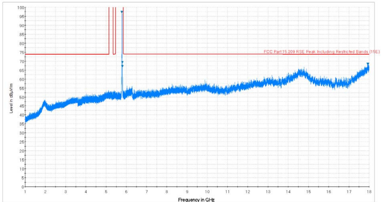
Plot 7-86. Radiated Spurious Plot above 1GHz (802.11a – U3 Ch. 157, Ant. Pol. V)
