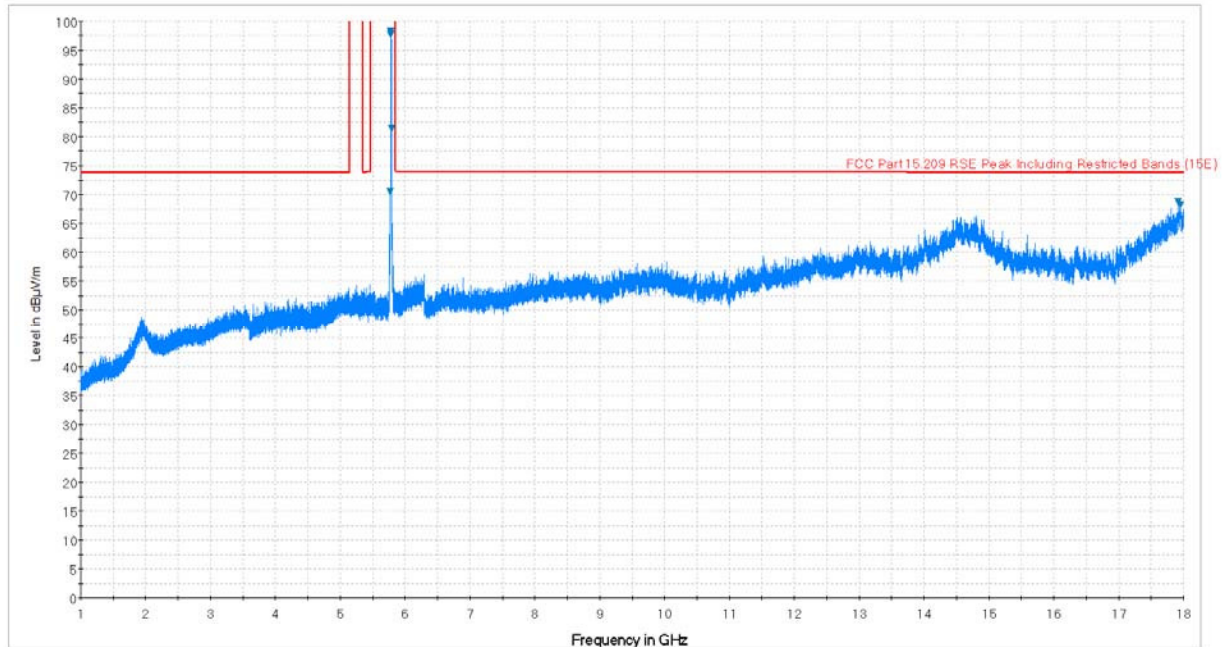
Plot 7-85. Radiated Spurious Plot above 1GHz (802.11a – U3 Ch. 157, Ant. Pol. H)
