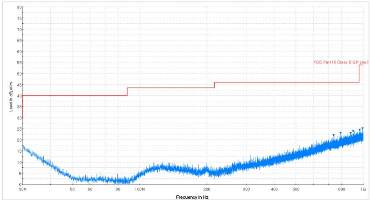
Plot 7-107. Radiated Spurious Plot below 1GHz (802.11a – U3 Ch. 157, Ant. Pol. H)
