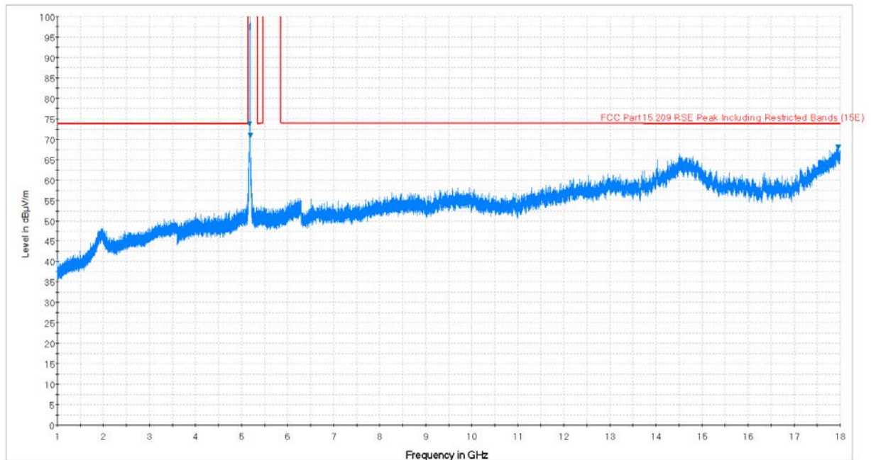
Plot 7-80. Radiated Spurious Plot above 1GHz (802.11a – U1 Ch. 40, Ant. Pol. V)
