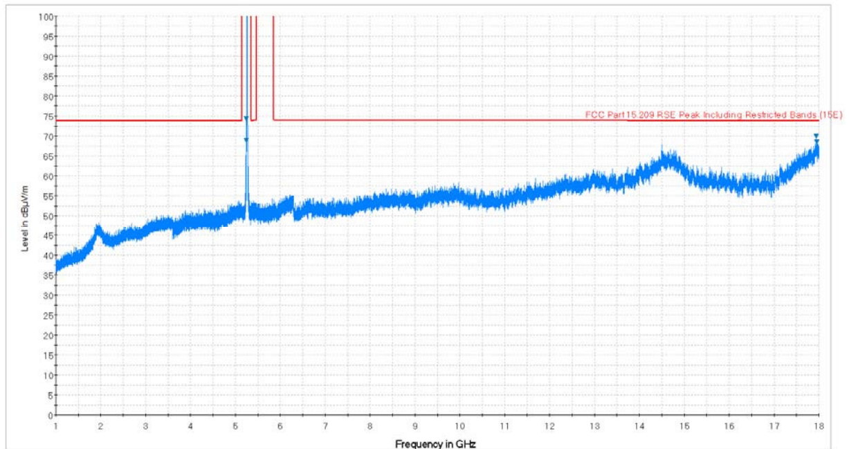
Plot 7-82. Radiated Spurious Plot above 1GHz (802.11a – U2A Ch. 56, Ant. Pol. V)
