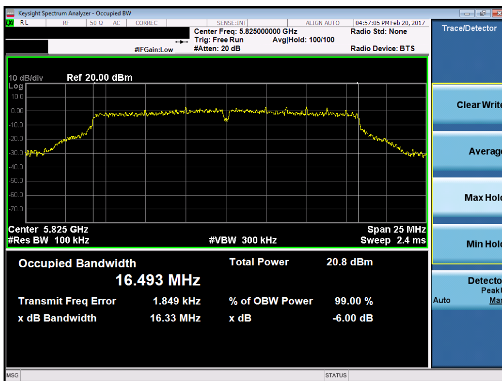
Plot 7-33. 6dB Bandwidth Plot (802.11a (UNII Band 3) – Ch. 165)
