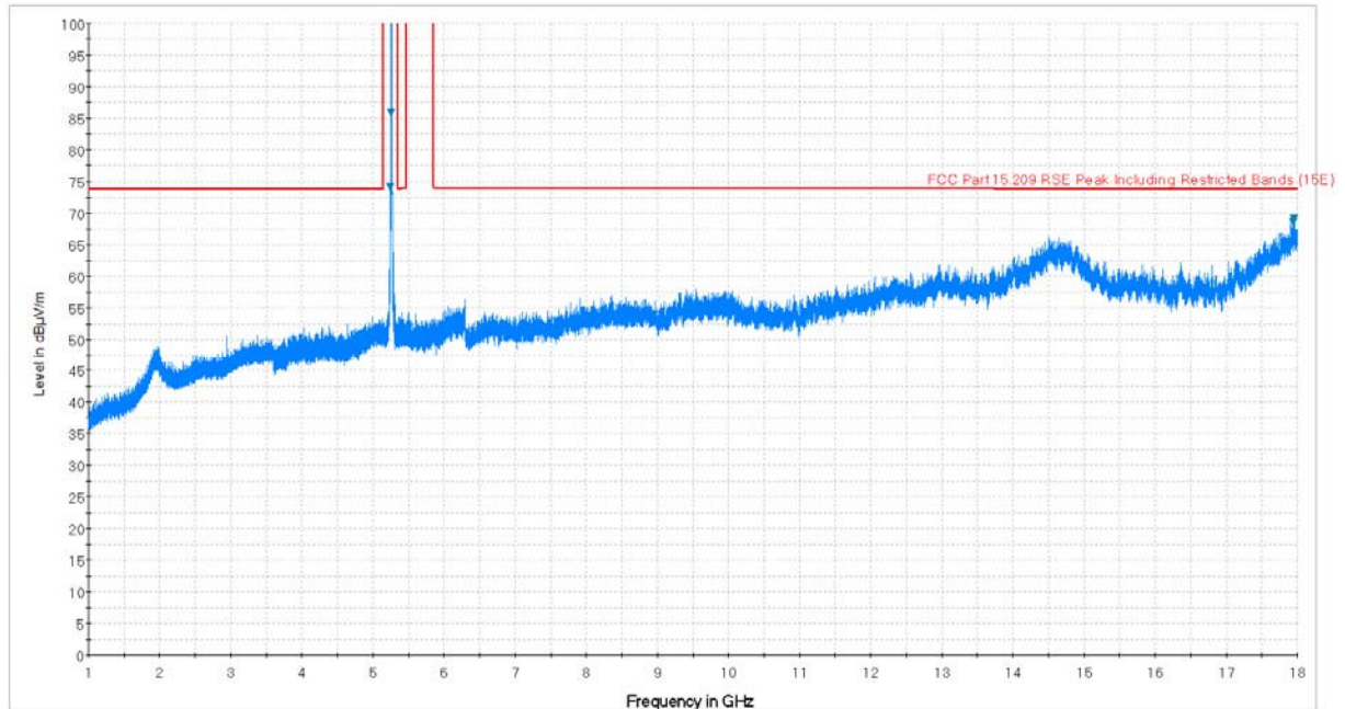
Plot 7-81. Radiated Spurious Plot above 1GHz (802.11a – U2A Ch. 56, Ant. Pol. H)
