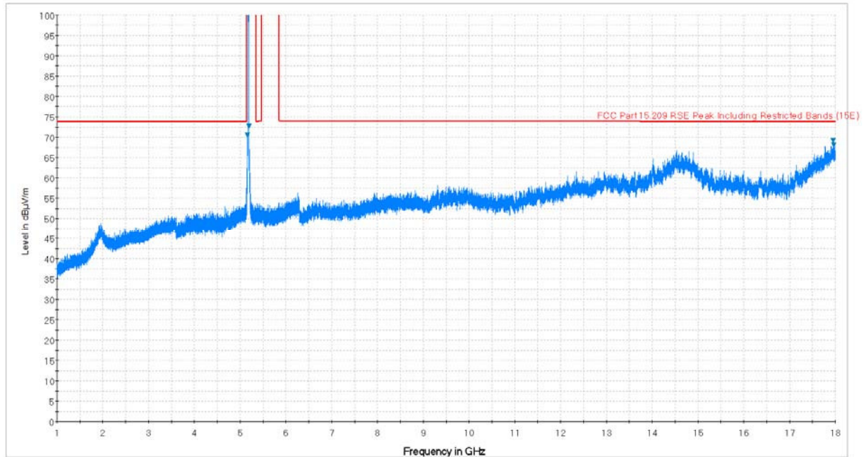
Plot 7-79. Radiated Spurious Plot above 1GHz (802.11a – U1 Ch. 40, Ant. Pol. H)
