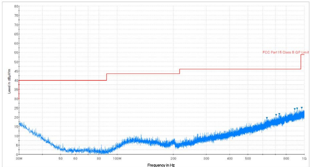
Plot 7-108. Radiated Spurious Plot below 1GHz (802.11a – U3 Ch. 157, Ant. Pol. V)
