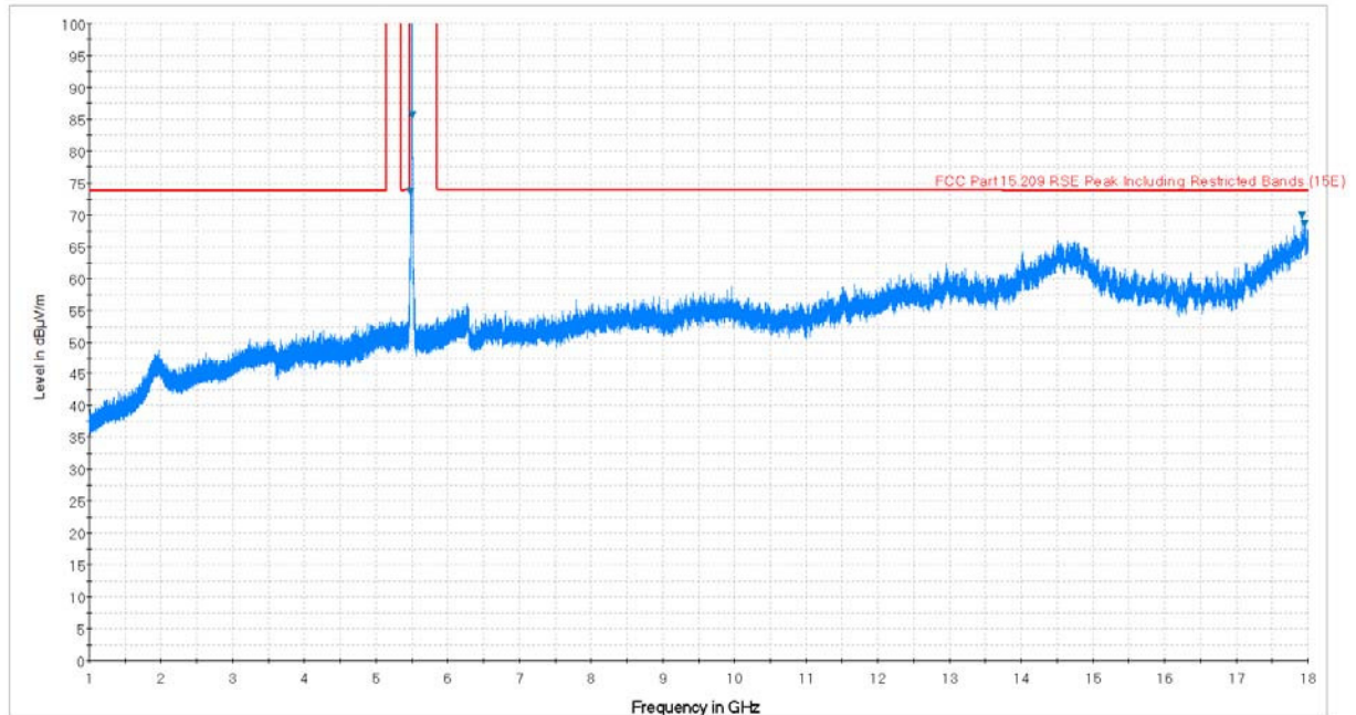
Plot 7-83. Radiated Spurious Plot above 1GHz (802.11a – U2C Ch. 116, Ant. Pol. H)
