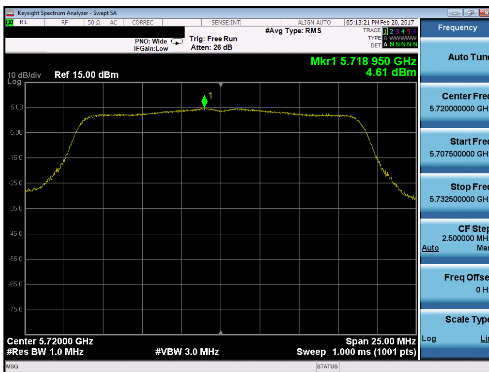
Plot 7-63. Power Spectral Density Plot (20MHz BW 802.11n (UNII Band 2C) – Ch. 144)
