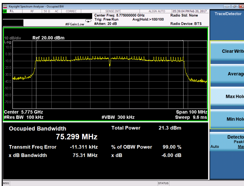
Plot 7-39. 6dB Bandwidth Plot (80MHz BW 802.11ac (UNII Band 3) – Ch. 155)
