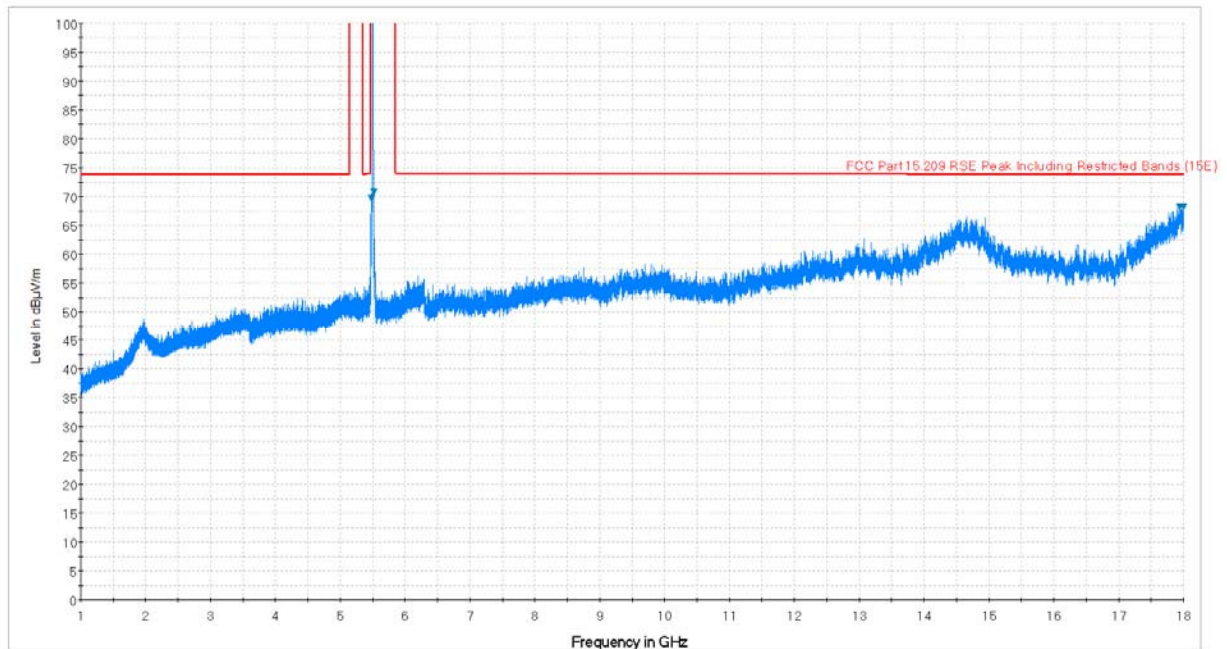
Plot 7-84. Radiated Spurious Plot above 1GHz (802.11a – U2C Ch. 116, Ant. Pol. V)
