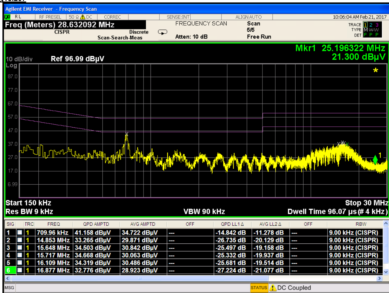
Plot 7-46. Line Conducted Plot with 802.11b (N)
