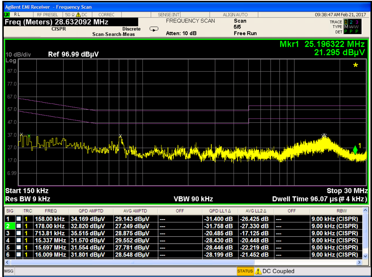
Plot 7-45. Line Conducted Plot with 802.11b (L1)
