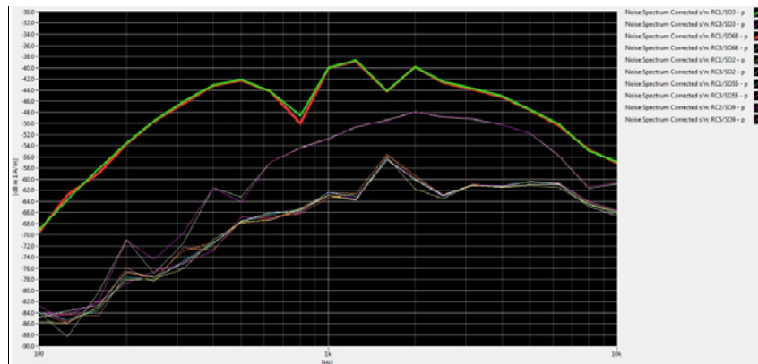
Figure 6-1 CDMA Audio Band Magnetic Noise
