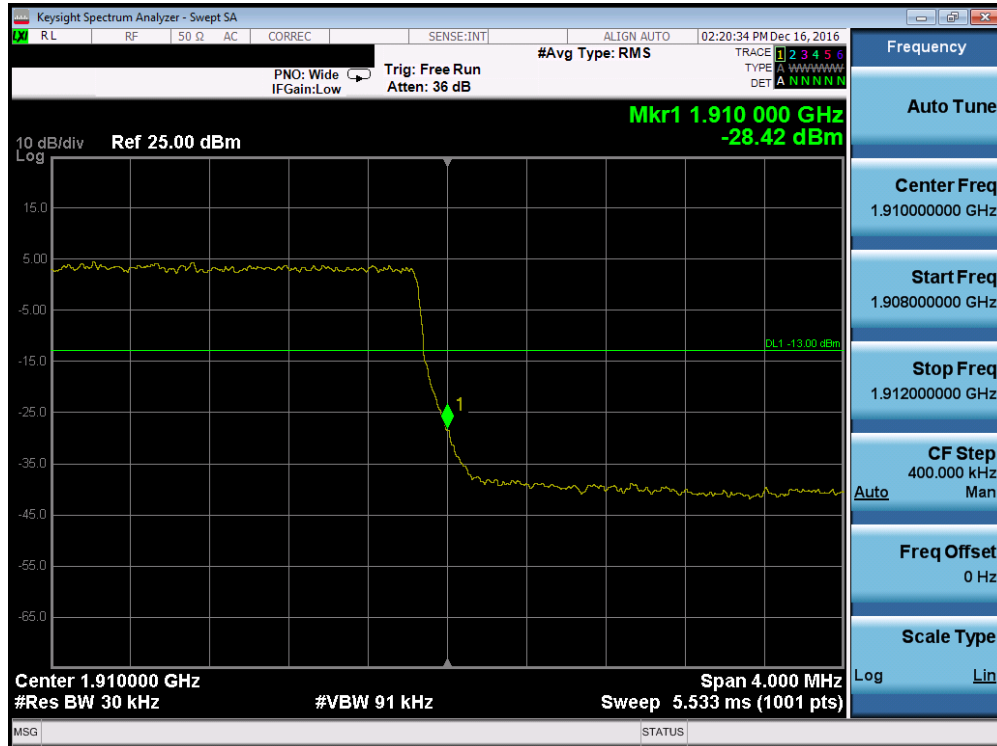
Plot 7-120. Upper Band Edge Plot (Band 2 – 3.0MHz QPSK – RB Size 15)
