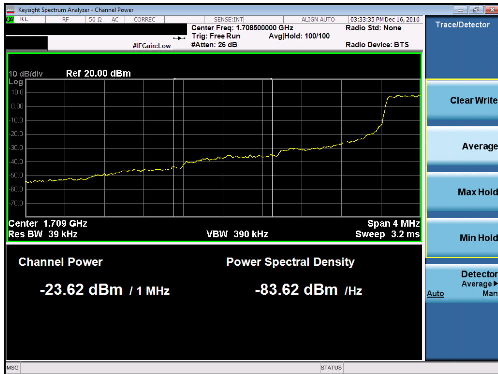
Plot 7-91. Lower Extended Band Edge Plot (Band 4 – 1.4MHz QPSK – RB Size 6)
