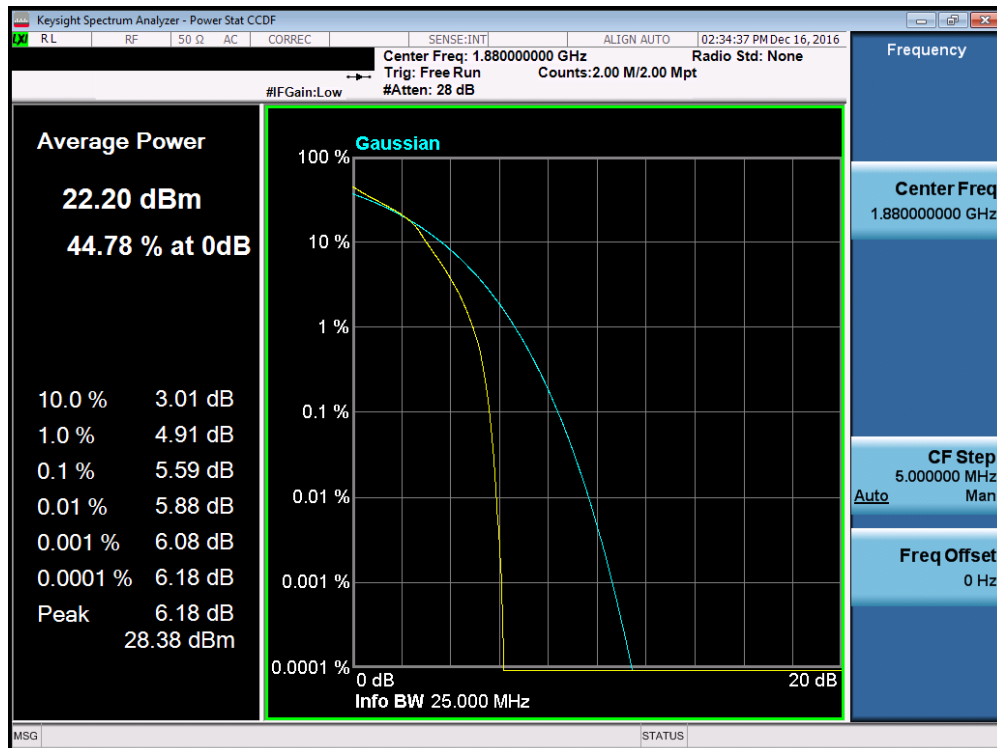
Plot 7-147. PAR Plot (Band 2 – 15.0MHz 16-QAM – RB Size 75)
