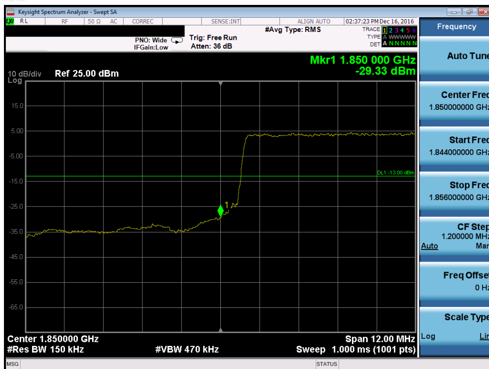
Plot 7-130. Lower Band Edge Plot (Band 2 – 15.0MHz QPSK – RB Size 75)
