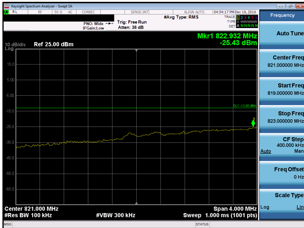
Plot 7-85. Lower Extended Band Edge Plot (Band 5 – 5.0MHz QPSK – RB Size 25)
