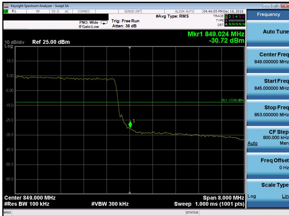
Plot 7-89. Upper Band Edge Plot (Band 5 – 10.0MHz QPSK – RB Size 50)
