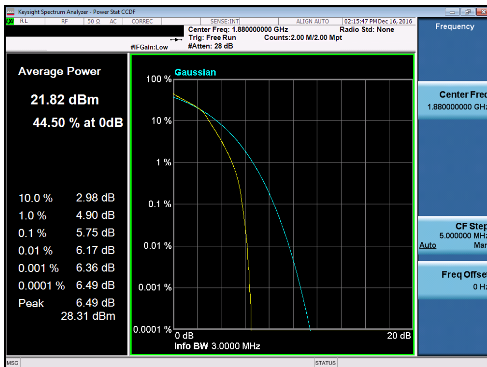
Plot 7-141. PAR Plot (Band 2 – 3.0MHz 16-QAM – RB Size 15)
