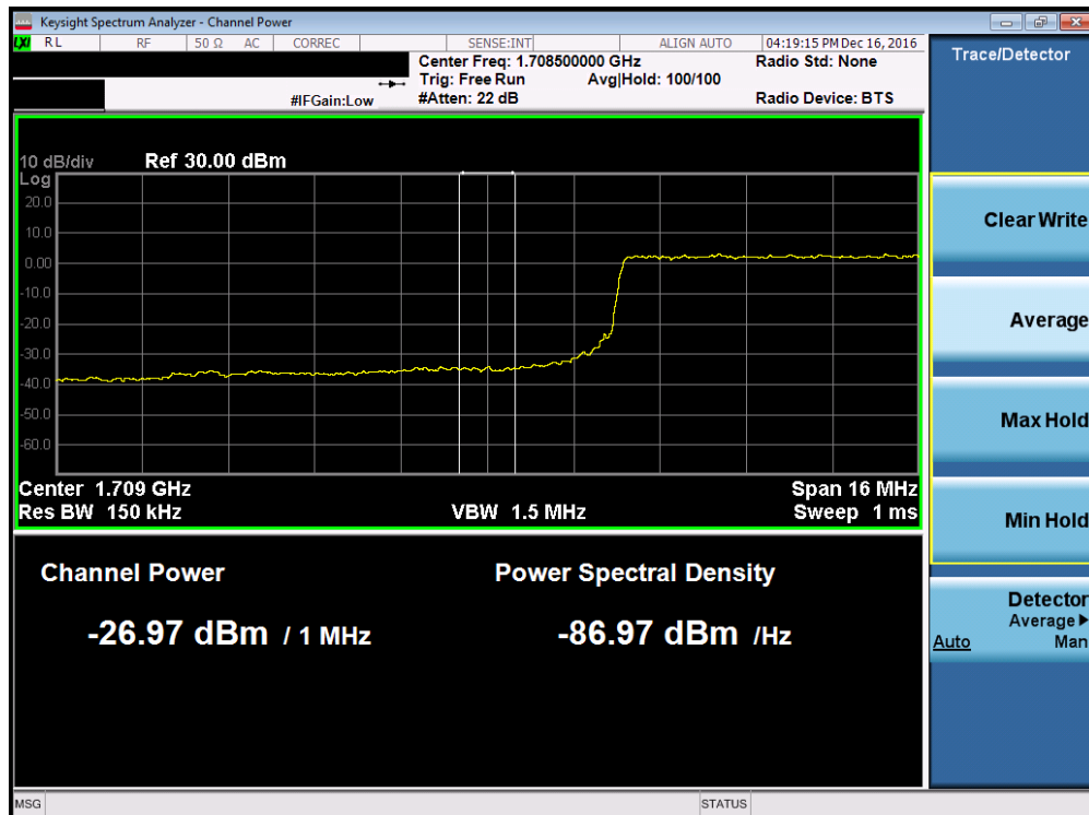
Plot 7-111. Lower Extended Band Edge Plot (Band 4 – 20.0MHz QPSK – RB Size 100)
