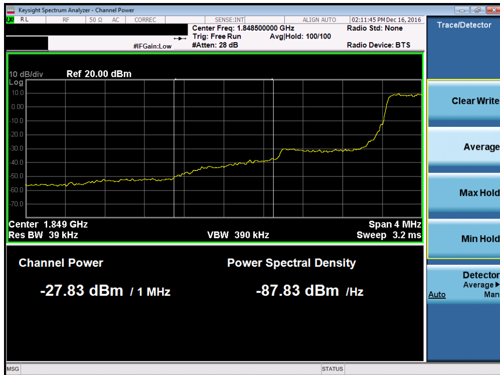
Plot 7-115. Lower Extended Band Edge Plot (Band 2 – 1.4MHz QPSK – RB Size 6)
