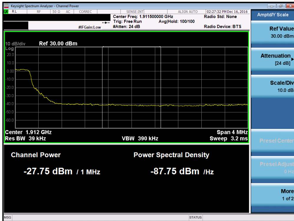
Plot 7-125. Upper Extended Band Edge Plot (Band 2 – 5.0MHz QPSK – RB Size 25)
