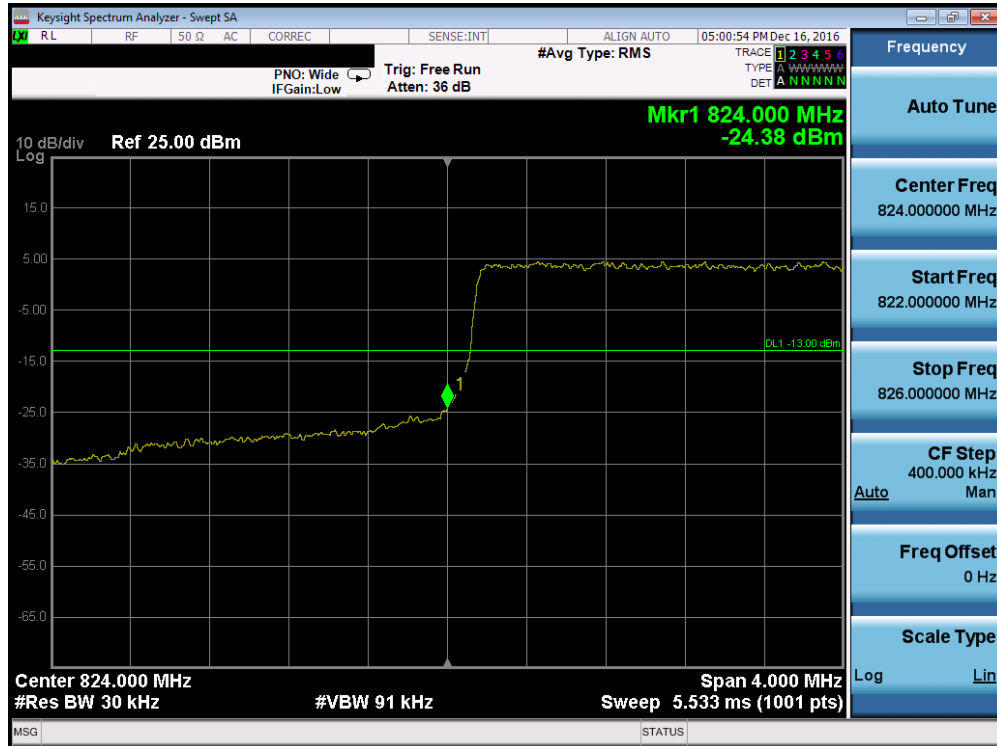
Plot 7-80. Lower Band Edge Plot (Band 5 - 3.0MHz QPSK - RB Size 15)
