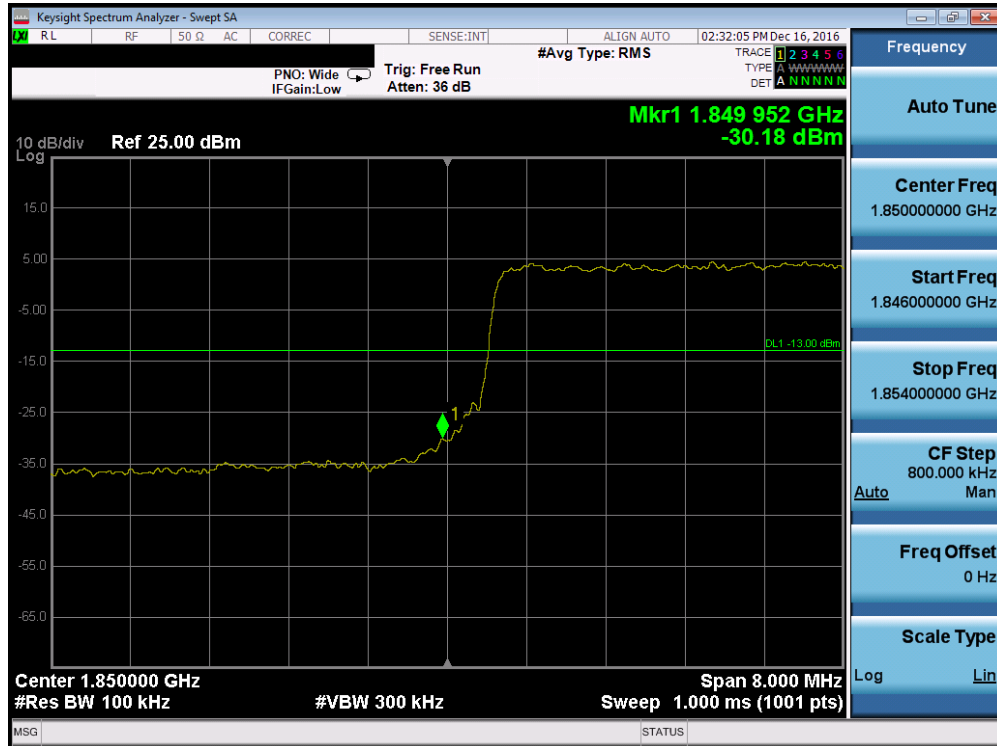
Plot 7-126. Lower Band Edge Plot (Band 2 – 10.0MHz QPSK – RB Size 50)
