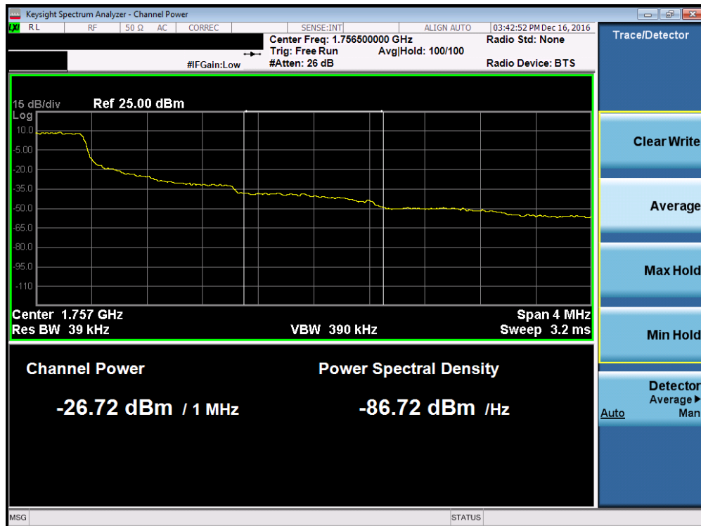
Plot 7-93. Upper Extended Band Edge Plot (Band 4 – 1.4MHz QPSK – RB Size 6)
