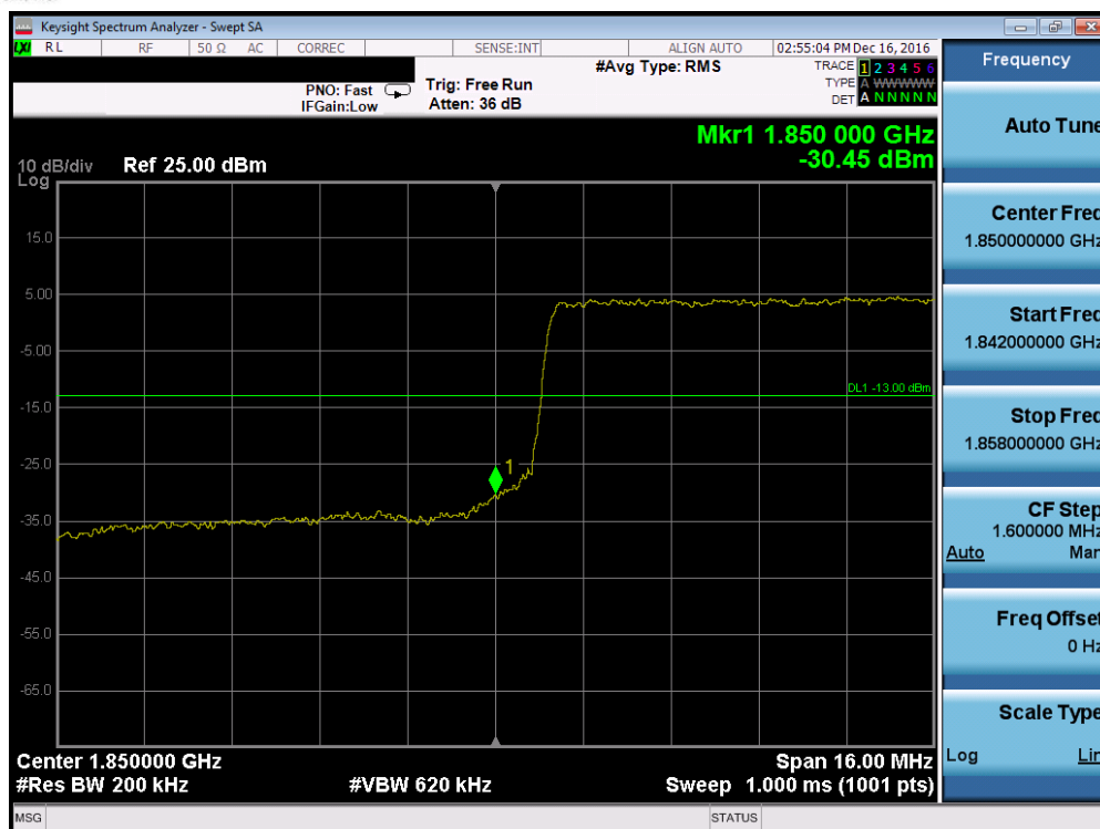
Plot 7-134. Lower Band Edge Plot (Band 2 – 20.0MHz QPSK – RB Size 100)
