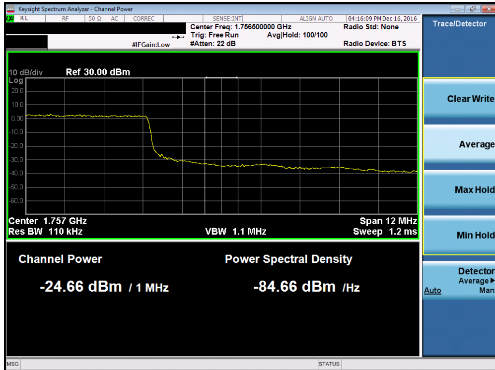
Plot 7-109. Upper Extended Band Edge Plot (Band 4 – 15.0MHz QPSK – RB Size 75)
