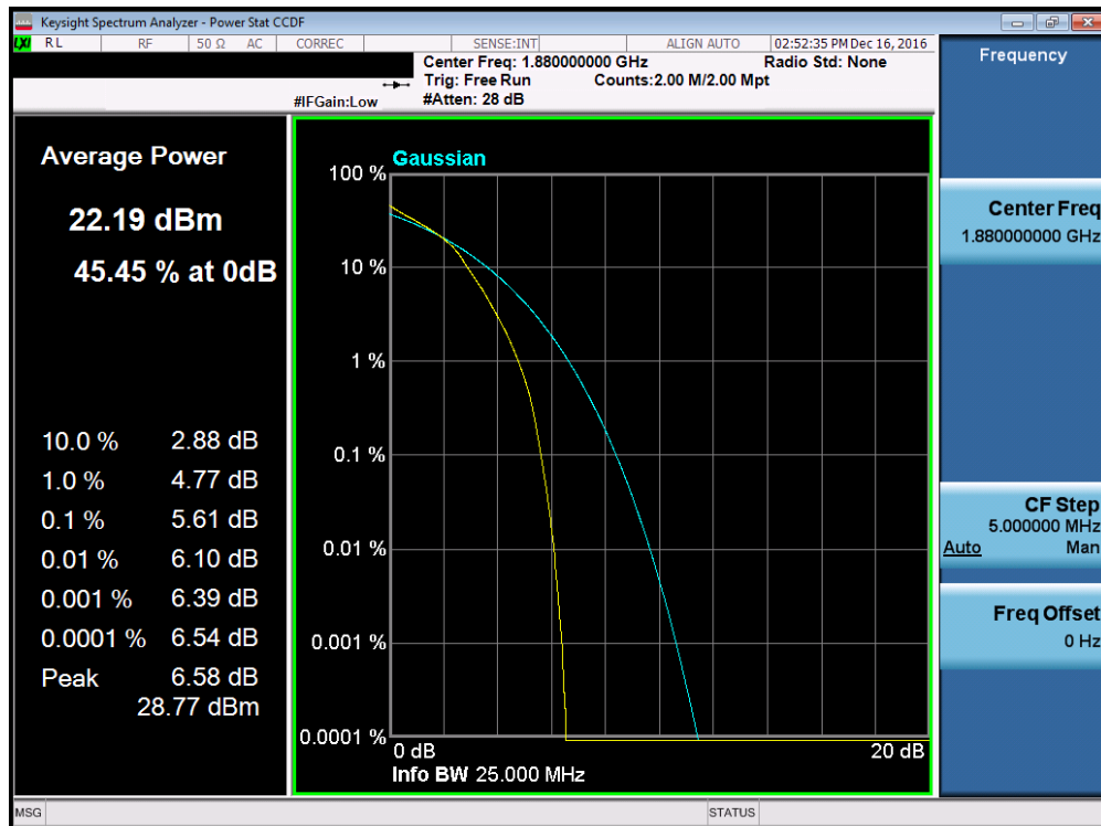
Plot 7-149. PAR Plot (Band 2 – 20.0MHz 16-QAM – RB Size 100)
