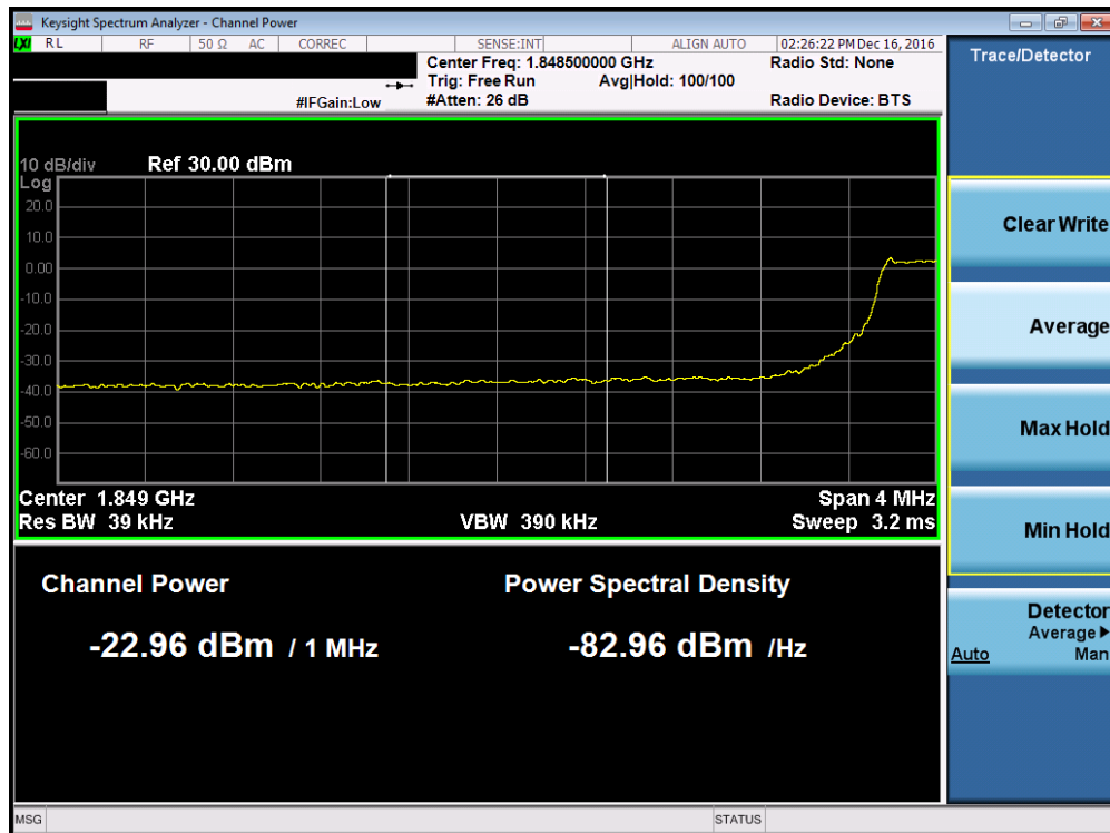
Plot 7-123. Lower Extended Band Edge Plot (Band 2 – 5.0MHz QPSK – RB Size 25)
