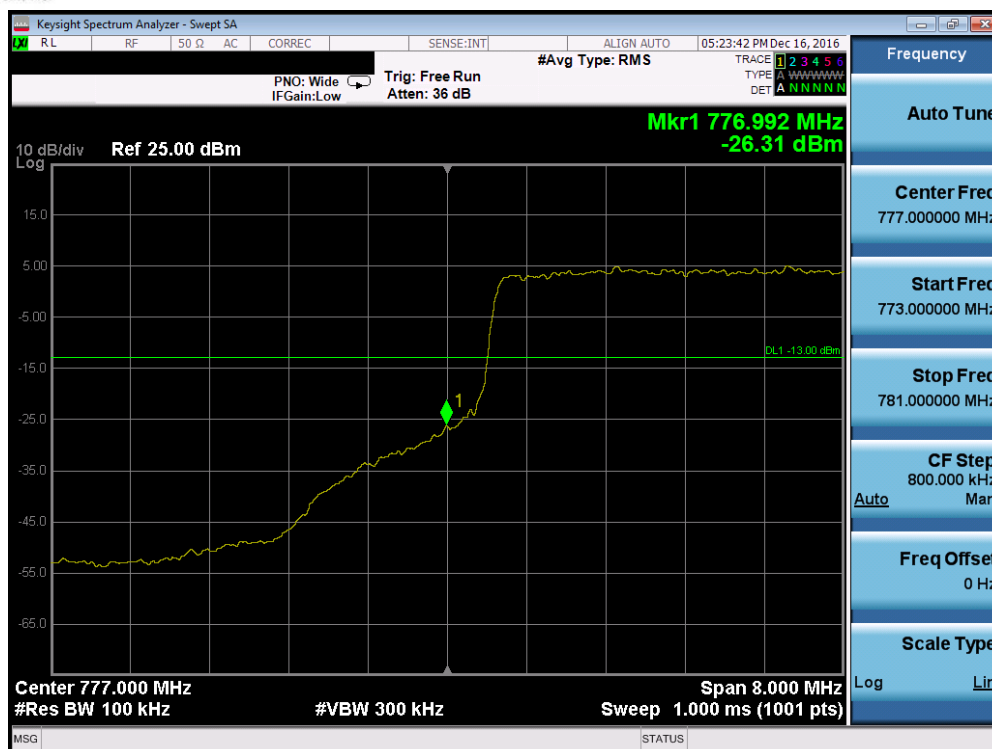
Plot 7-72. Lower Band Edge Plot (Band 13 – 10.0MHz QPSK – RB Size 50)
