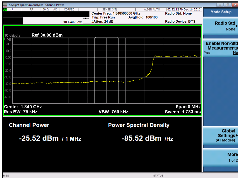
Plot 7-127. Lower Extended Band Edge Plot (Band 2 – 10.0MHz QPSK – RB Size 50)
