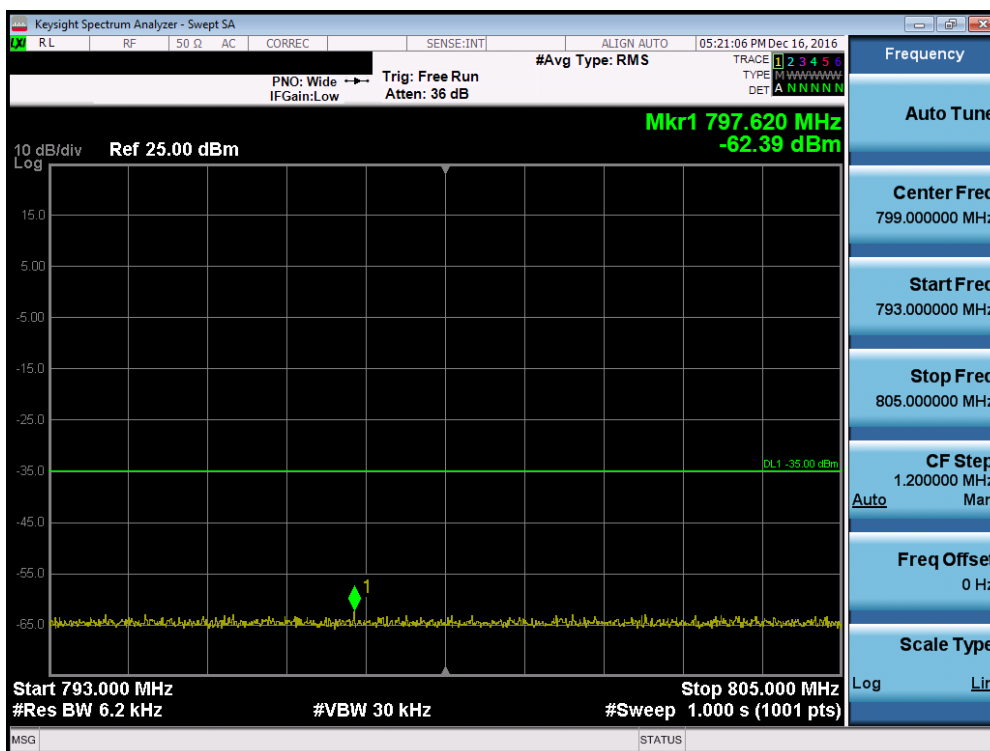
Plot 7-71. Upper Emission Mask Edge Plot (Band 13 – 5.0MHz QPSK – RB Size 25)
