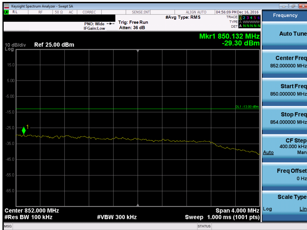
Plot 7-87. Upper Extended Band Edge Plot (Band 5 – 5.0MHz QPSK – RB Size 25)
