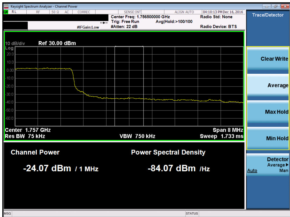
Plot 7-105. Upper Extended Band Edge Plot (Band 4 – 10.0MHz QPSK – RB Size 50)
