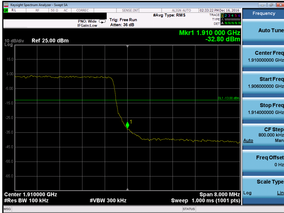
Plot 7-128. Upper Band Edge Plot (Band 2 – 10.0MHz QPSK – RB Size 50)
