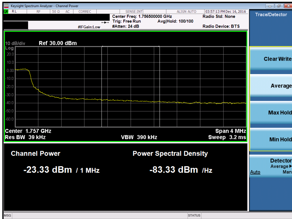
Plot 7-101. Upper Extended Band Edge Plot (Band 4 – 5.0MHz QPSK – RB Size 25)
