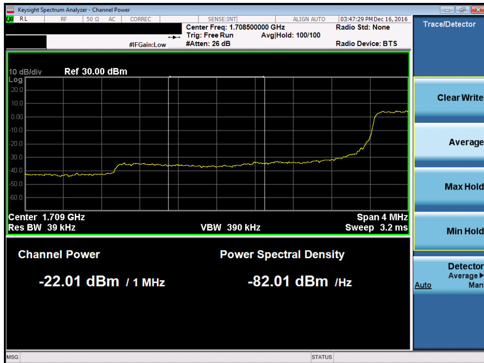
Plot 7-95. Lower Extended Band Edge Plot (Band 4 – 3.0MHz QPSK – RB Size 15)
