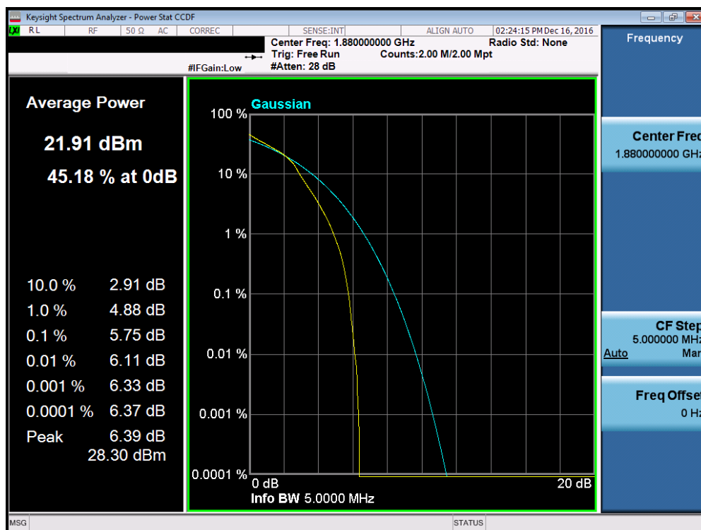
Plot 7-143. PAR Plot (Band 2 – 5.0MHz 16-QAM – RB Size 25)
