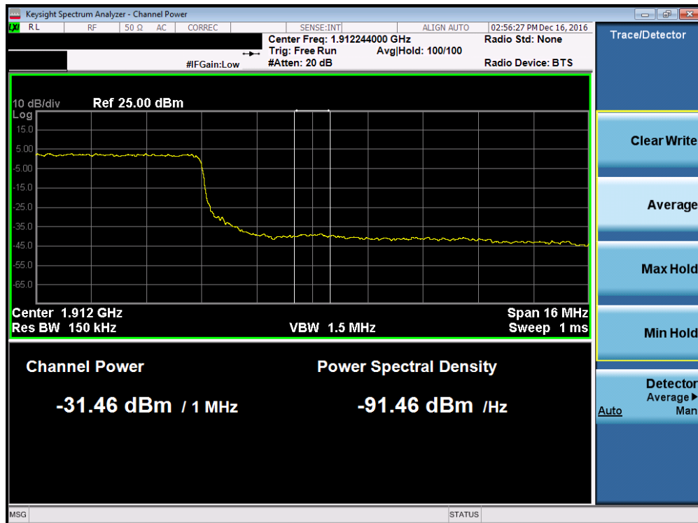
Plot 7-137. Upper Extended Band Edge Plot (Band 2 – 20.0MHz QPSK – RB Size 100)
