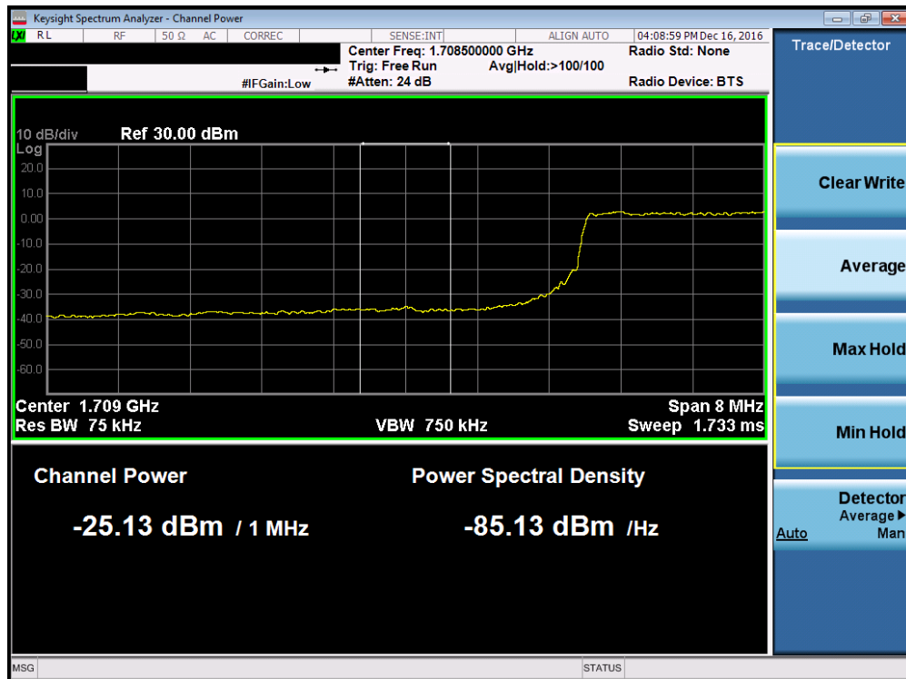
Plot 7-103. Lower Extended Band Edge Plot (Band 4 – 10.0MHz QPSK – RB Size 50)
