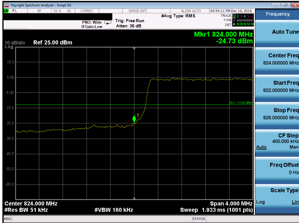
Plot 7-84. Lower Band Edge Plot (Band 5 – 5.0MHz QPSK – RB Size 25)
