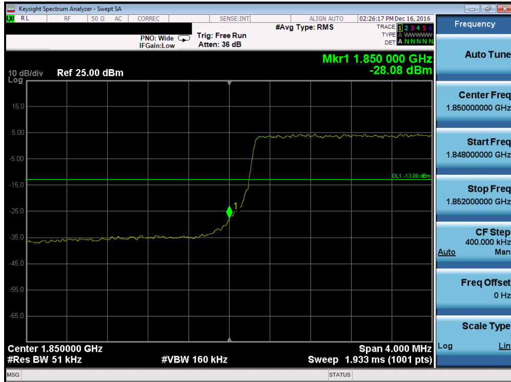
Plot 7-122. Lower Band Edge Plot (Band 2 – 5.0MHz QPSK – RB Size 25)
