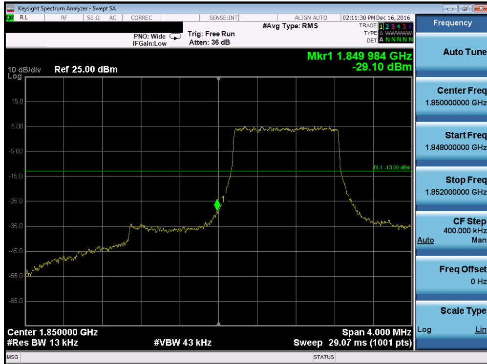
Plot 7-114. Lower Band Edge Plot (Band 2 – 1.4MHz QPSK – RB Size 6)
