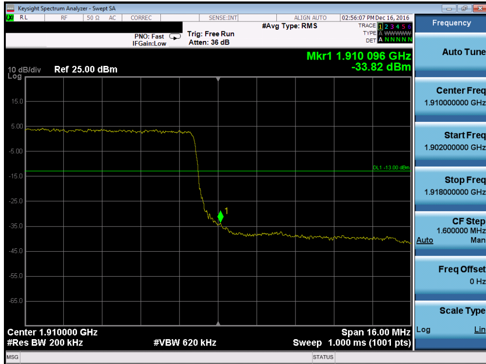
Plot 7-136. Upper Band Edge Plot (Band 2 – 20.0MHz QPSK – RB Size 100)
