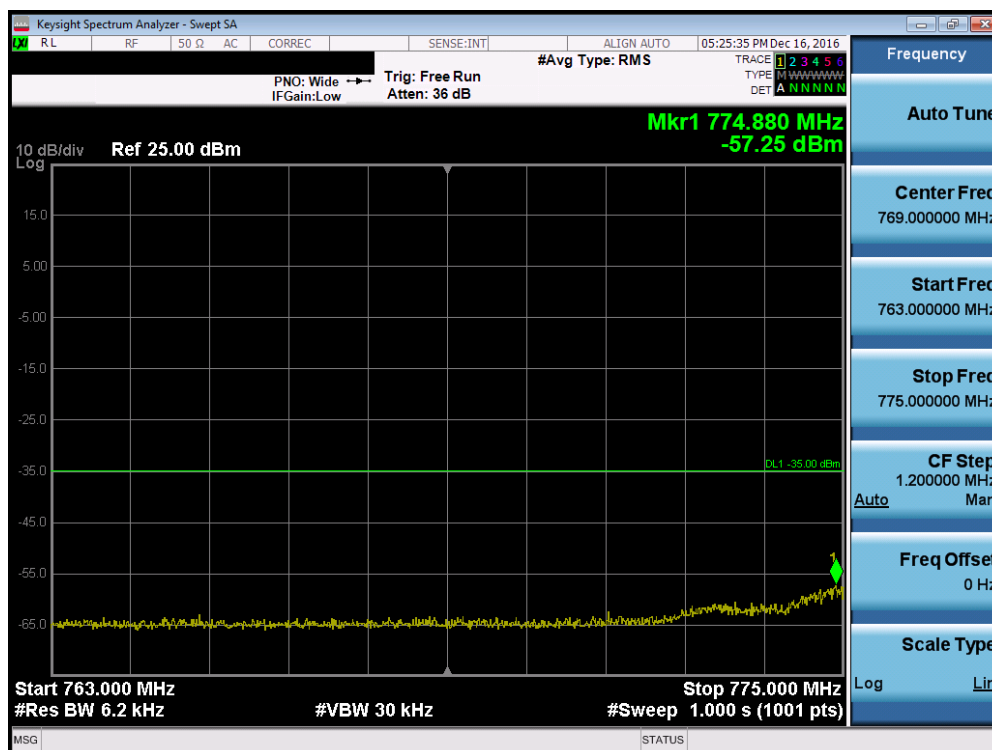
Plot 7-73. Lower Emission Mask Edge Plot (Band 13 – 10.0MHz QPSK – RB Size 50)
