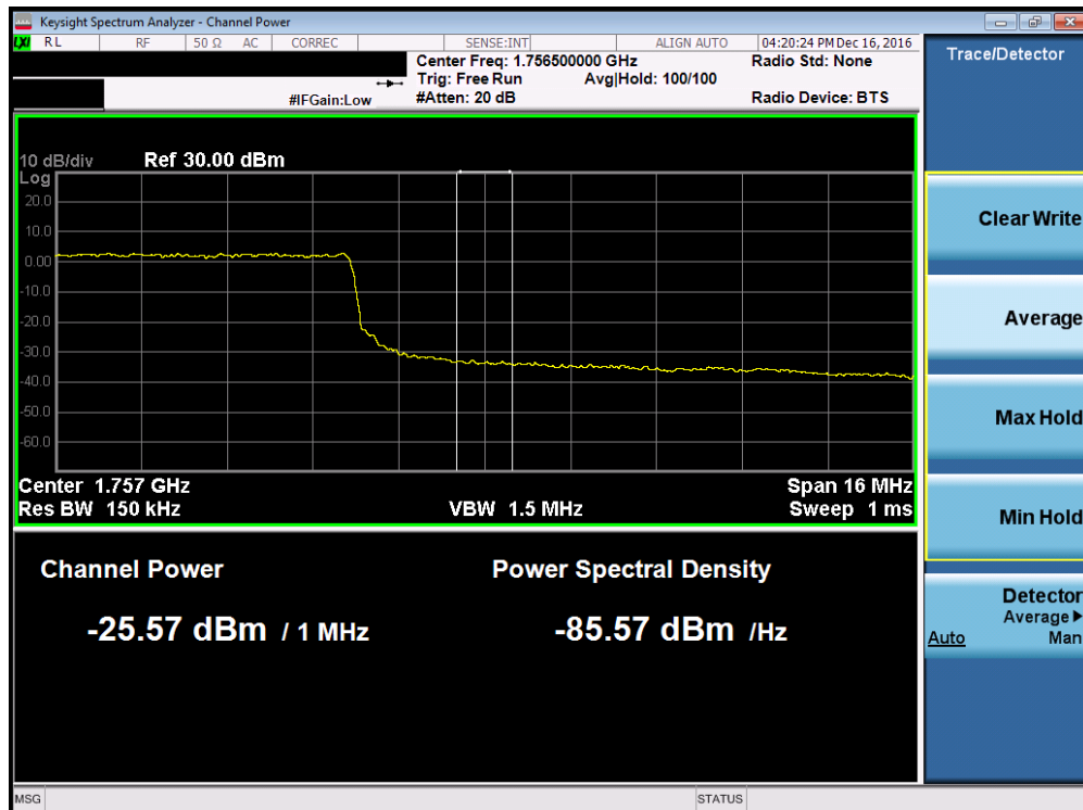
Plot 7-113. Upper Extended Band Edge Plot (Band 4 – 20.0MHz QPSK – RB Size 100)
