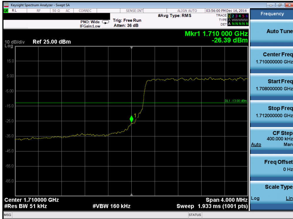
Plot 7-98. Lower Band Edge Plot (Band 4 – 5.0MHz QPSK – RB Size 25)
