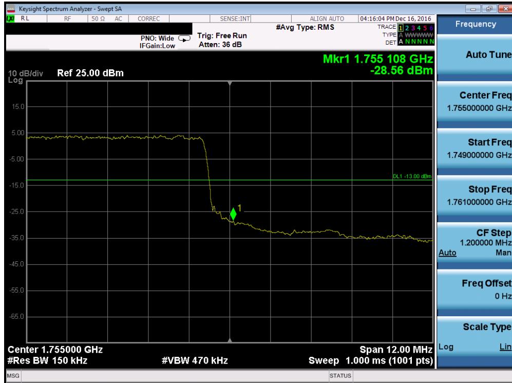
Plot 7-108. Upper Band Edge Plot (Band 4 – 15.0MHz QPSK – RB Size 75)
