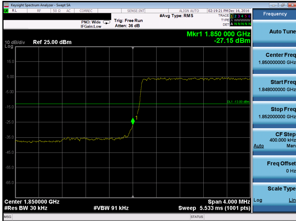
Plot 7-118. Lower Band Edge Plot (Band 2 – 3.0MHz QPSK – RB Size 15)
