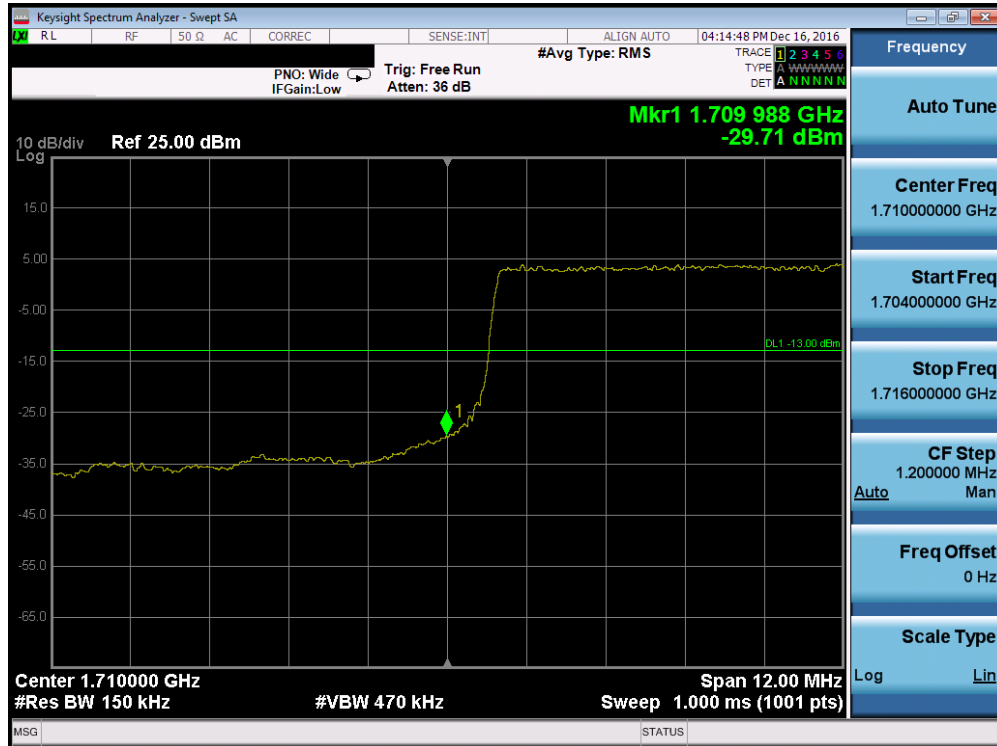
Plot 7-106. Lower Band Edge Plot (Band 4 – 15.0MHz QPSK – RB Size 75)
