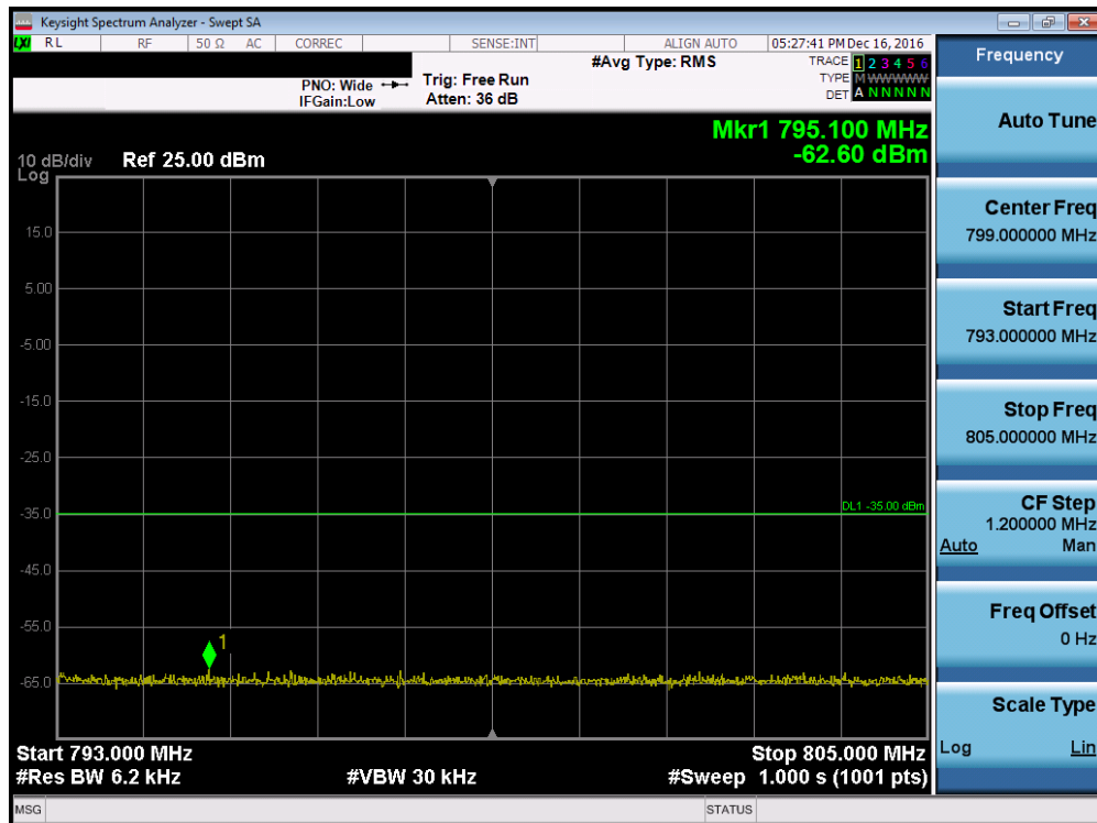
Plot 7-75. Upper Emission Mask Edge Plot (Band 13 – 10.0MHz QPSK – RB Size 50)
