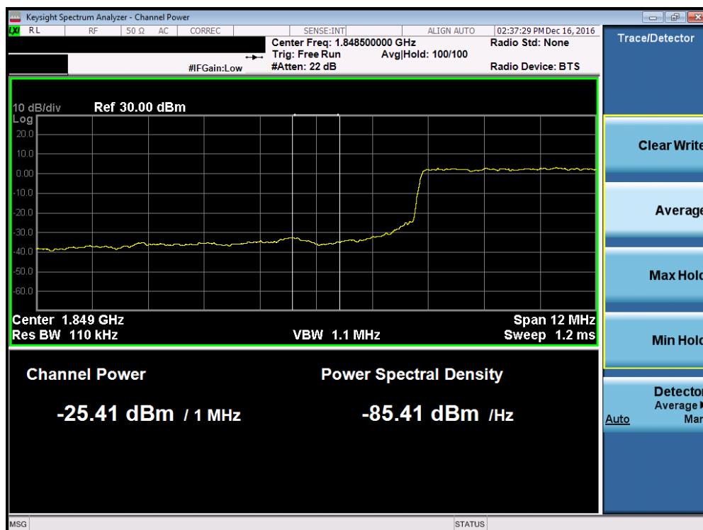
Plot 7-131. Lower Extended Band Edge Plot (Band 2 – 15.0MHz QPSK – RB Size 75)
