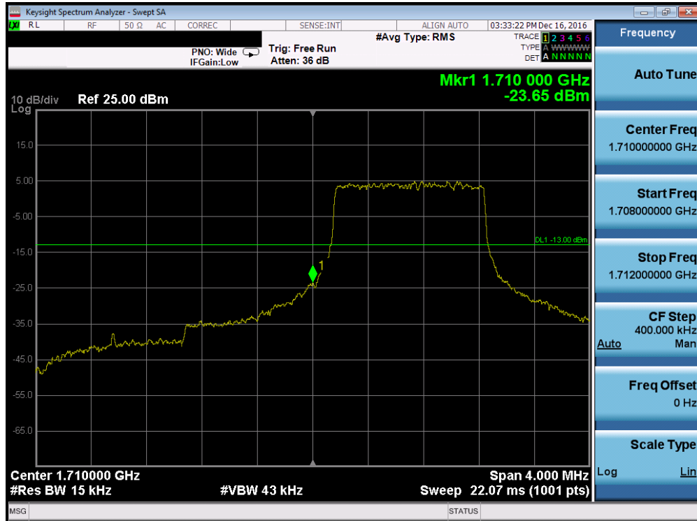
Plot 7-90. Lower Band Edge Plot (Band 4 – 1.4MHz QPSK – RB Size 6)
