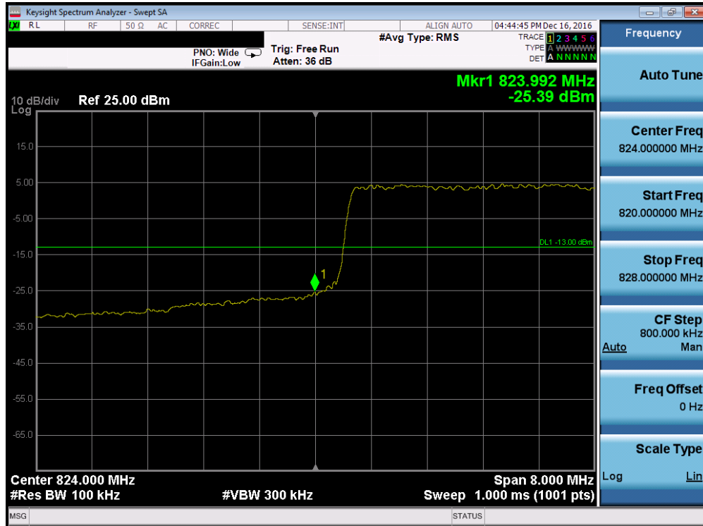
Plot 7-88. Lower Band Edge Plot (Band 5 – 10.0MHz QPSK – RB Size 50)
