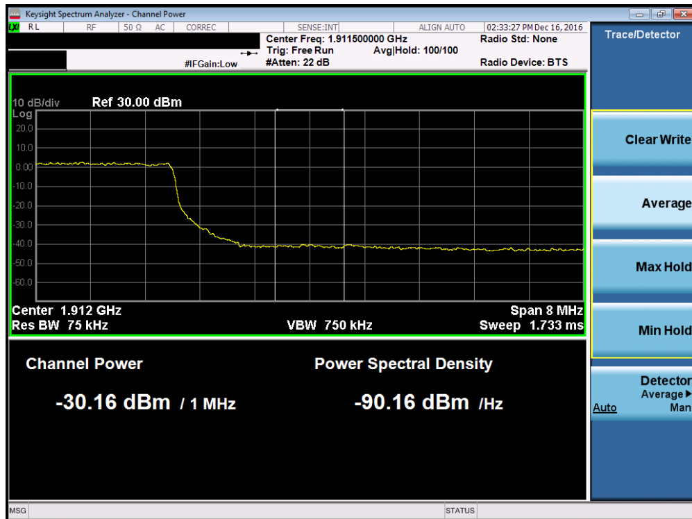
Plot 7-129. Upper Extended Band Edge Plot (Band 2 – 10.0MHz QPSK – RB Size 50)
