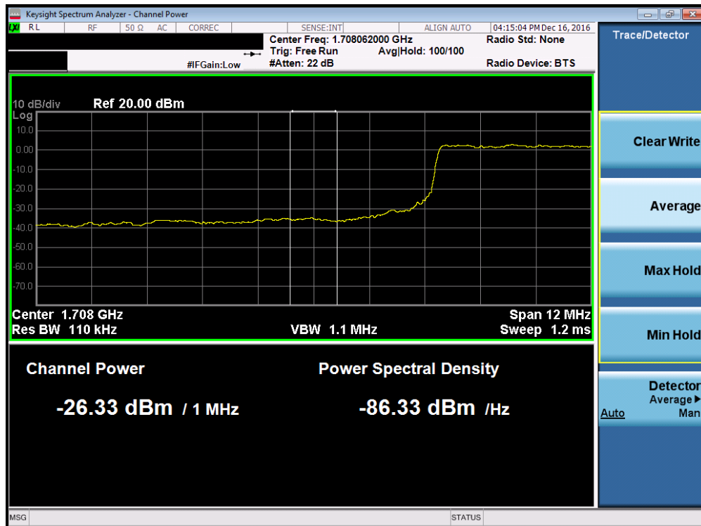
Plot 7-107. Lower Extended Band Edge Plot (Band 4 – 15.0MHz QPSK – RB Size 75)
