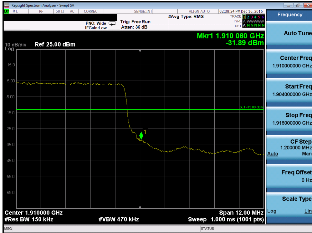
Plot 7-132. Upper Band Edge Plot (Band 2 – 15.0MHz QPSK – RB Size 75)
