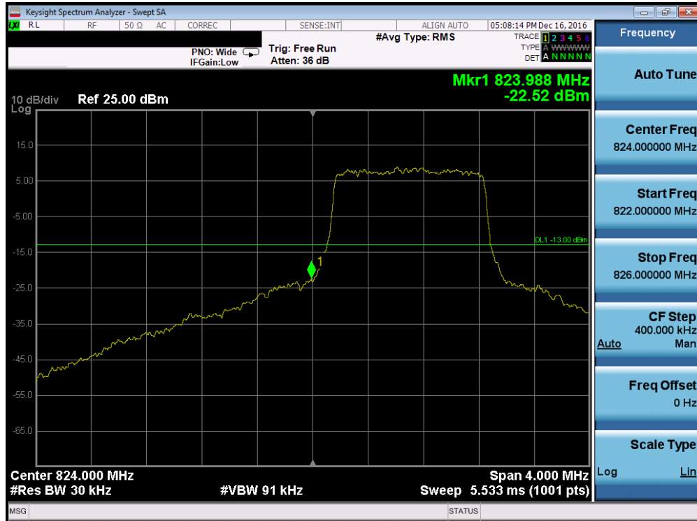
Plot 7-76. Lower Band Edge Plot (Band 5 – 1.4MHz QPSK – RB Size 6)
