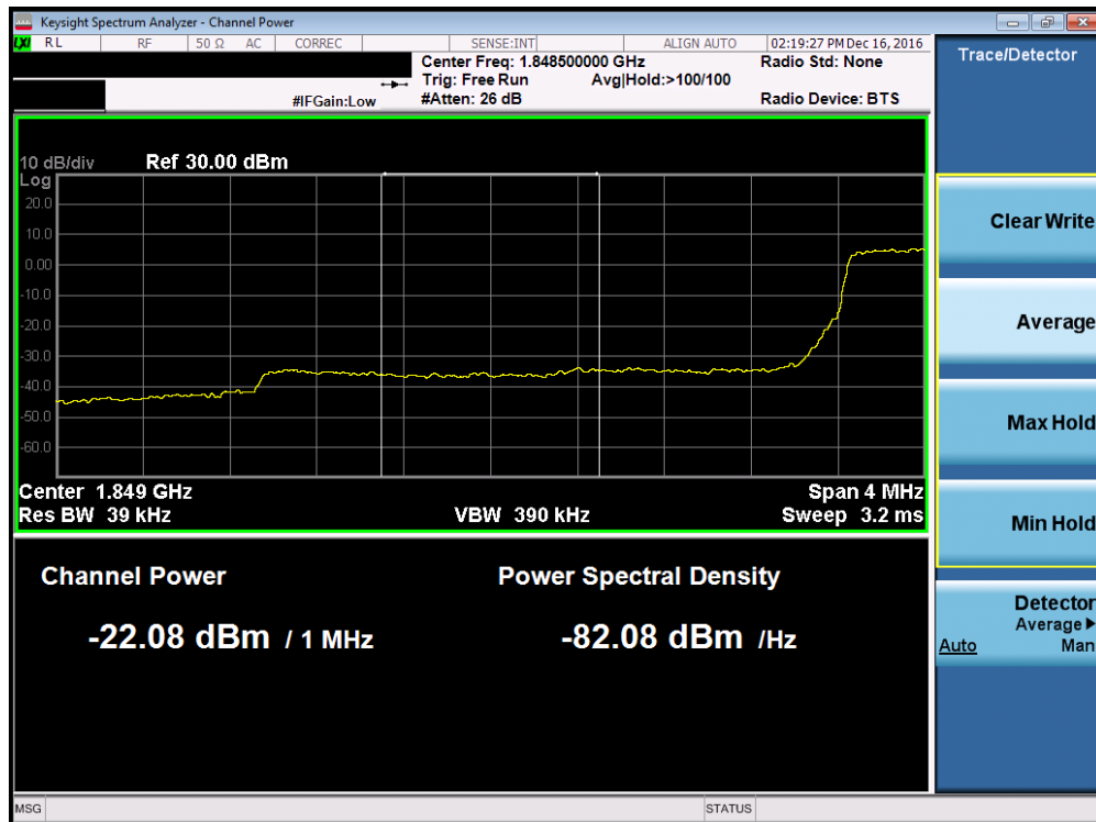
Plot 7-119. Lower Extended Band Edge Plot (Band 2 – 3.0MHz QPSK – RB Size 15)
