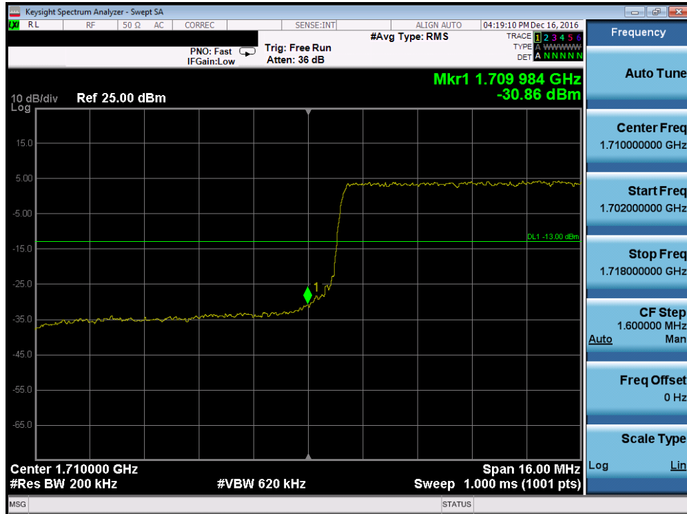
Plot 7-110. Lower Band Edge Plot (Band 4 – 20.0MHz QPSK – RB Size 100)
