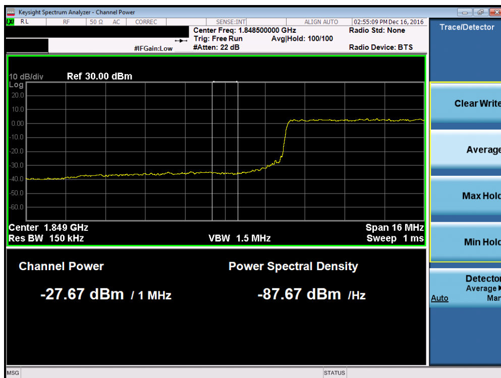
Plot 7-135. Lower Extended Band Edge Plot (Band 2 – 20.0MHz QPSK – RB Size 100)
