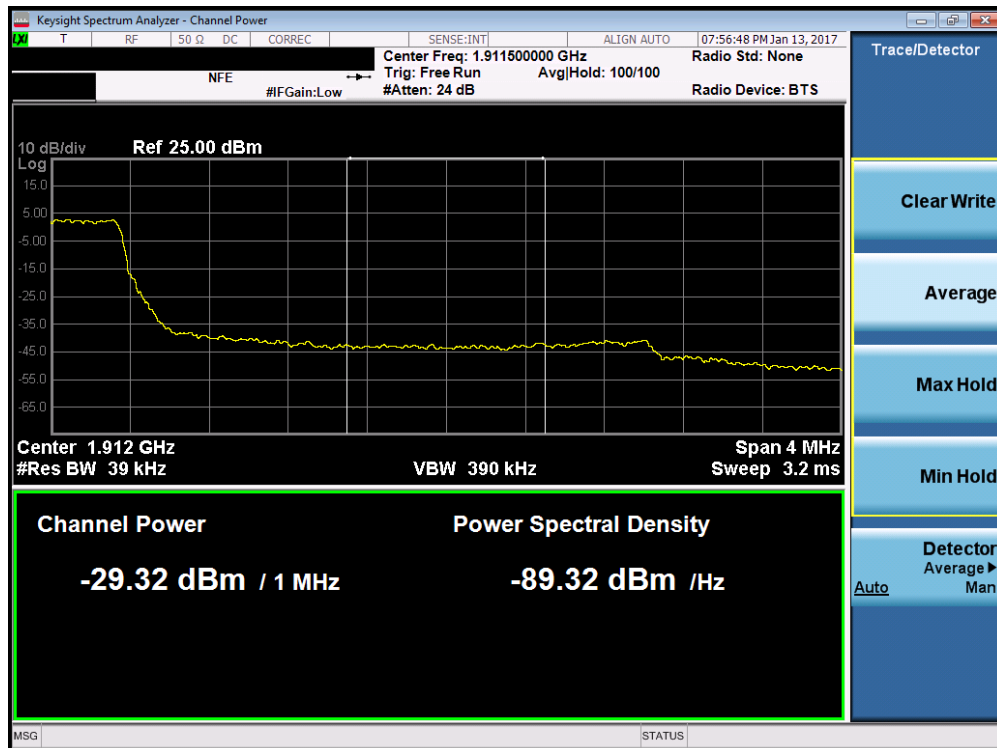
Plot 7-121. Upper Extended Band Edge Plot (Band 2 – 3.0MHz QPSK – RB Size 15)
