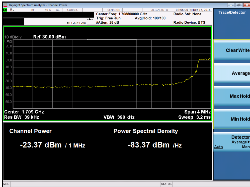
Plot 7-99. Lower Extended Band Edge Plot (Band 4 – 5.0MHz QPSK – RB Size 25)
