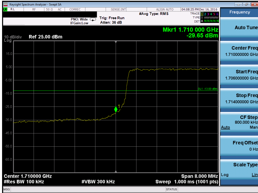
Plot 7-102. Lower Band Edge Plot (Band 4 – 10.0MHz QPSK – RB Size 50)
