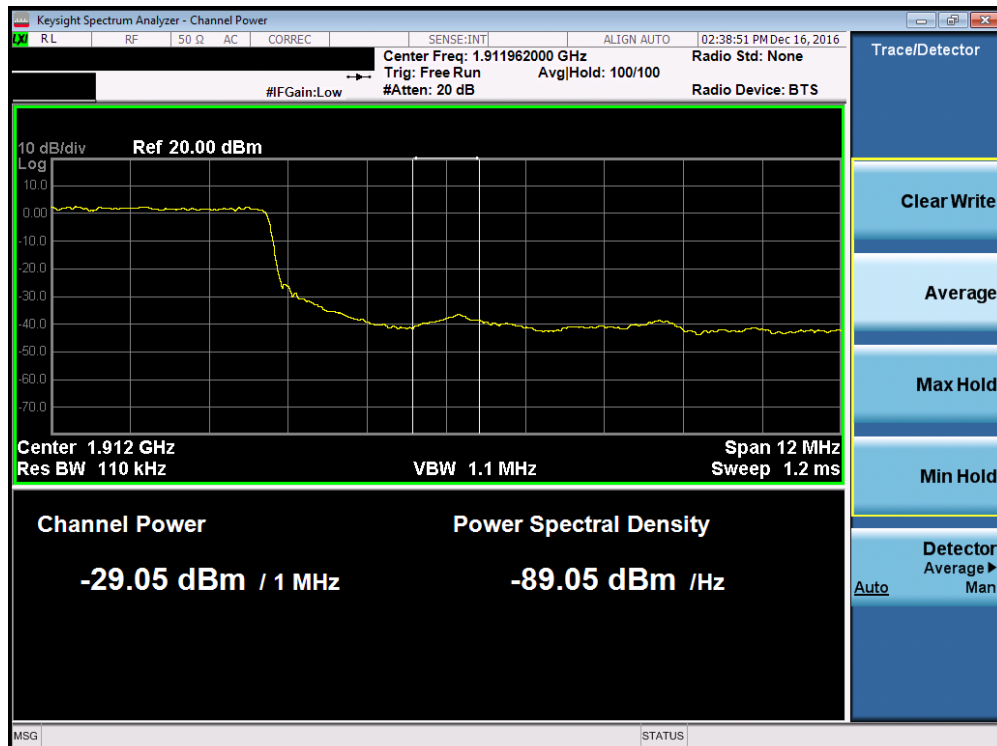
Plot 7-133. Upper Extended Band Edge Plot (Band 2 – 15.0MHz QPSK – RB Size 75)
