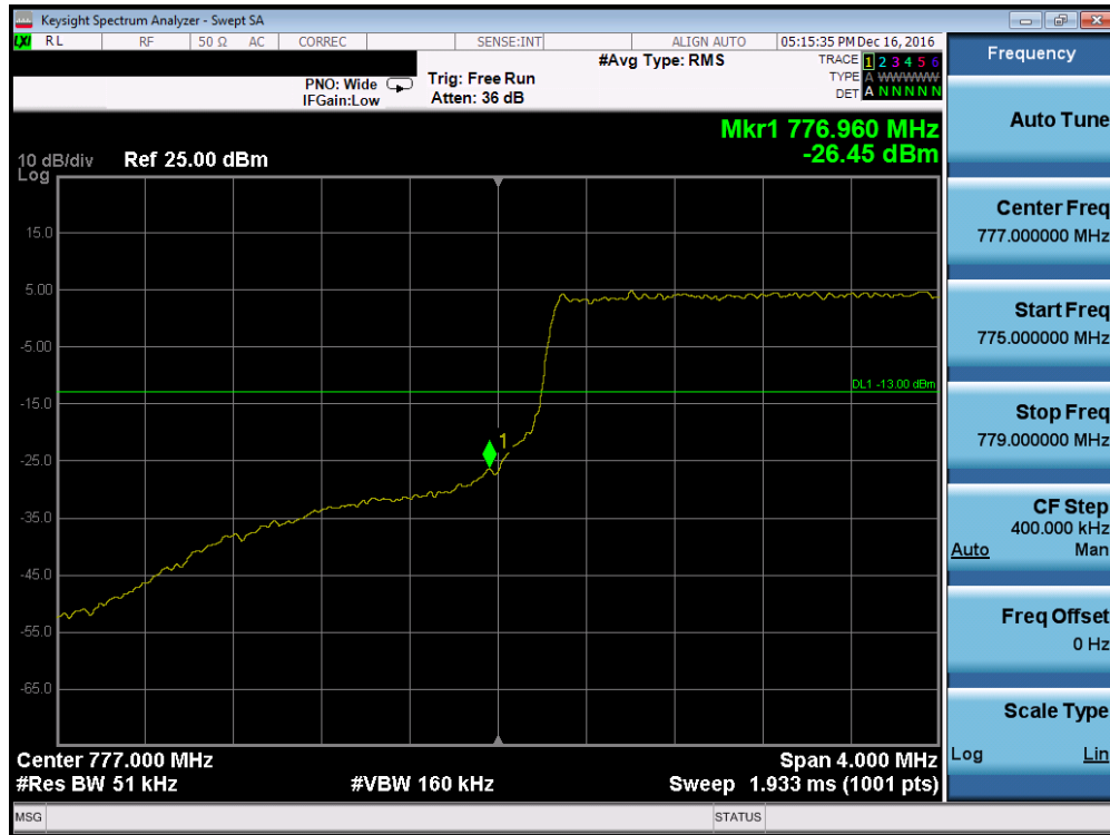
Plot 7-66. Lower Band Edge Plot (Band 13 – 5.0MHz QPSK – RB Size 25)
