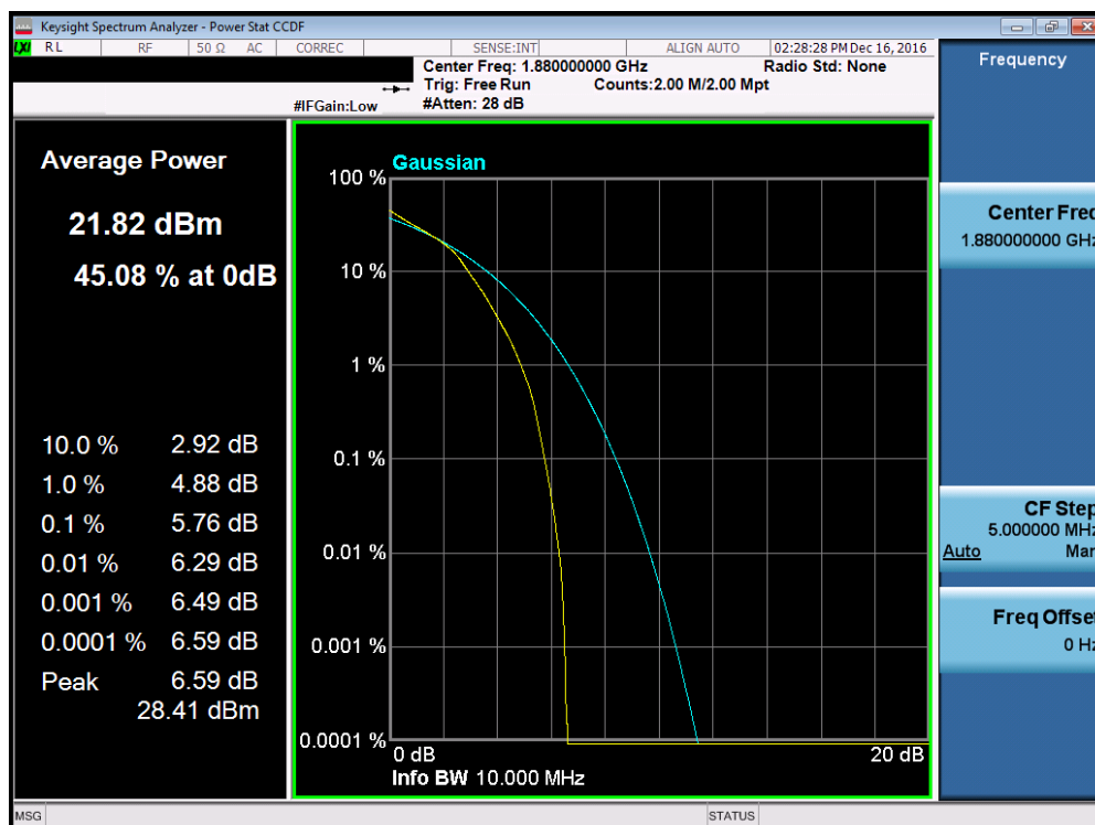
Plot 7-145. PAR Plot (Band 2 – 10.0MHz 16-QAM – RB Size 50)
