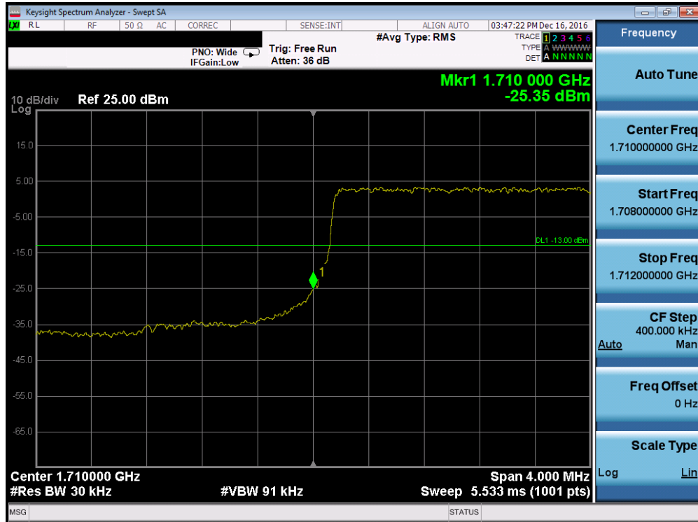
Plot 7-94. Lower Band Edge Plot (Band 4 – 3.0MHz QPSK – RB Size 15)
