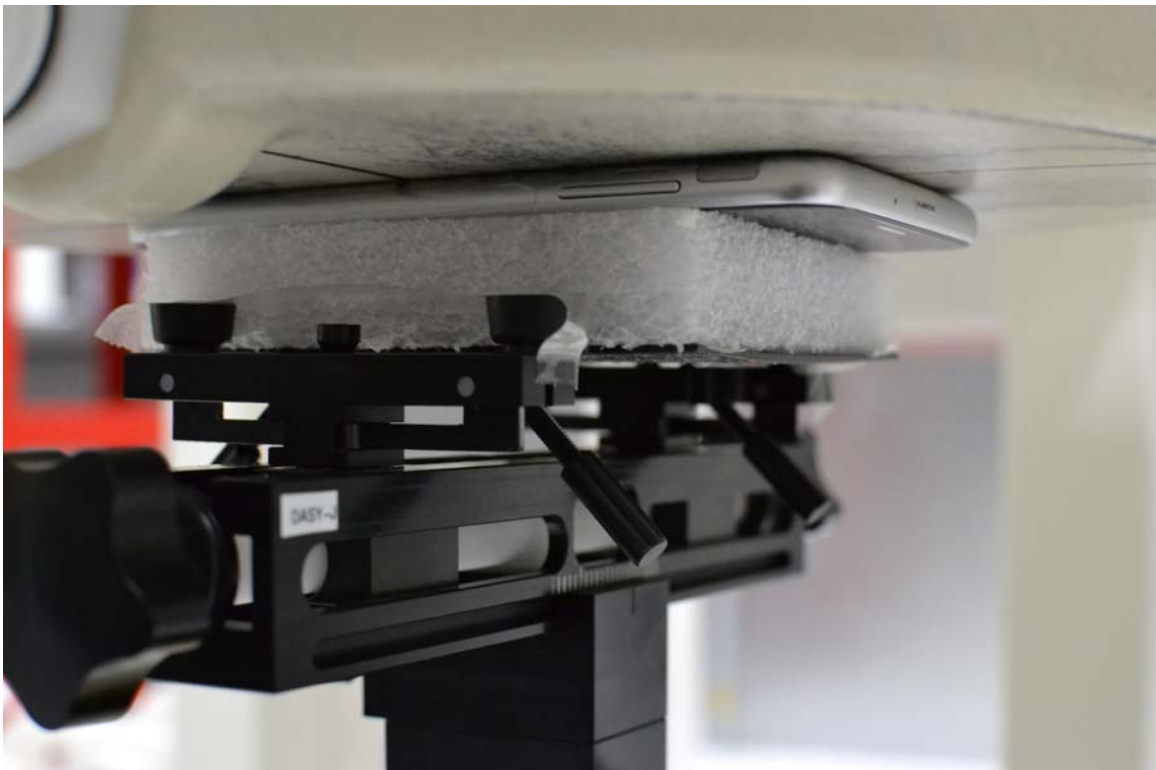
SAR Test Setup Photo 8- Back at 0.0 cm
