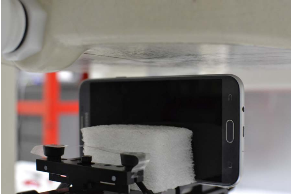
SAR Test Setup Photo 17- Right Edge at 1.0 cm (Hotspot)
