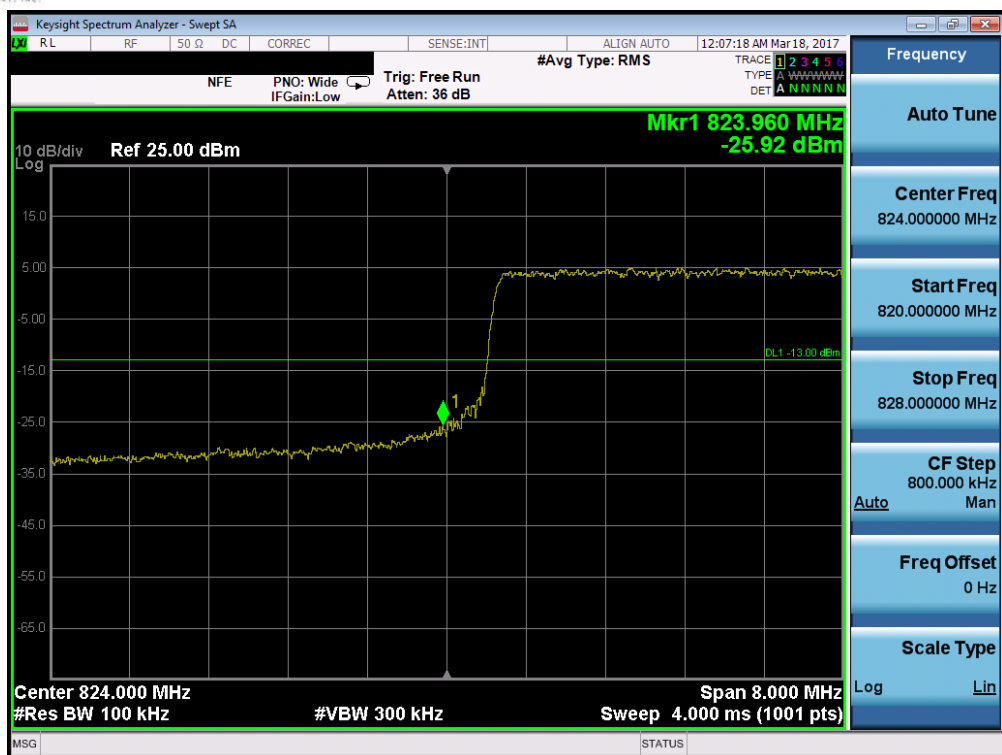
Plot 7-26. Lower Band Edge Plot (Band 5 – 10.0MHz QPSK – RB Size 50)
