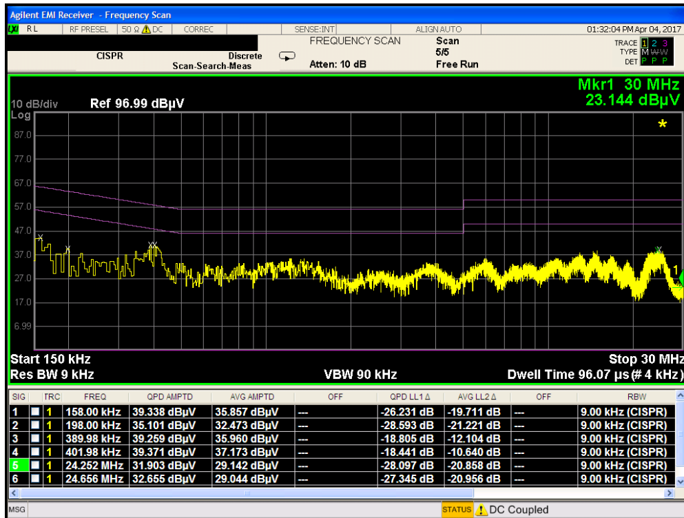
Plot 8-4. Line-Conducted Test Plot – Terminated in 50Ω (N)
