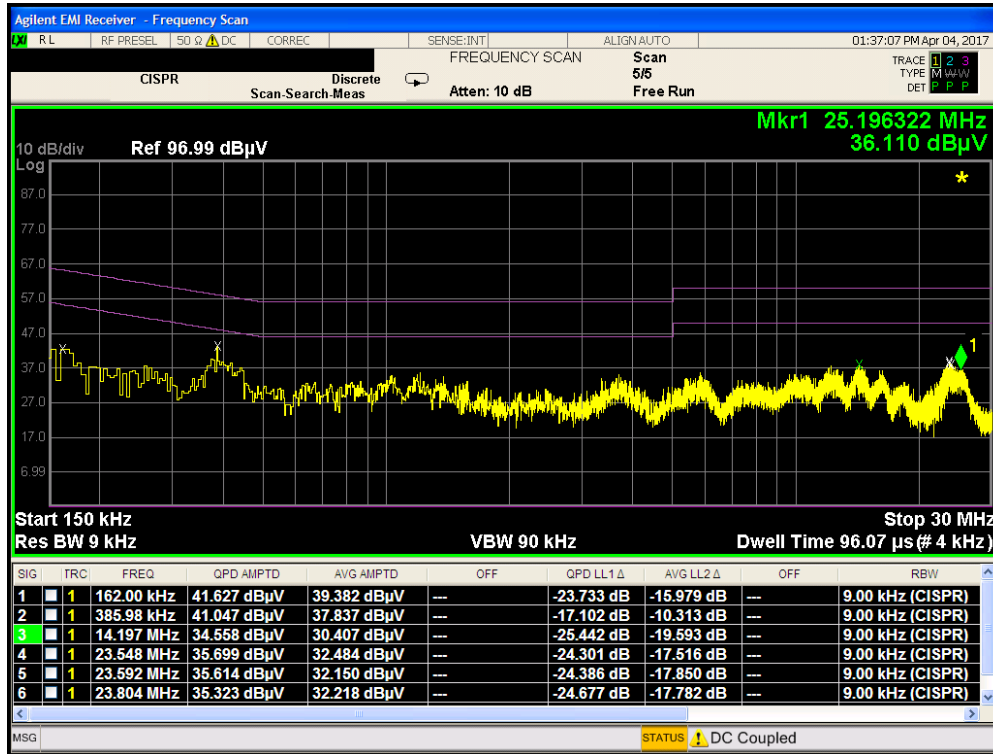
Plot 8-3. Line-Conducted Test Plot – Terminated in 50Ω (L1)
