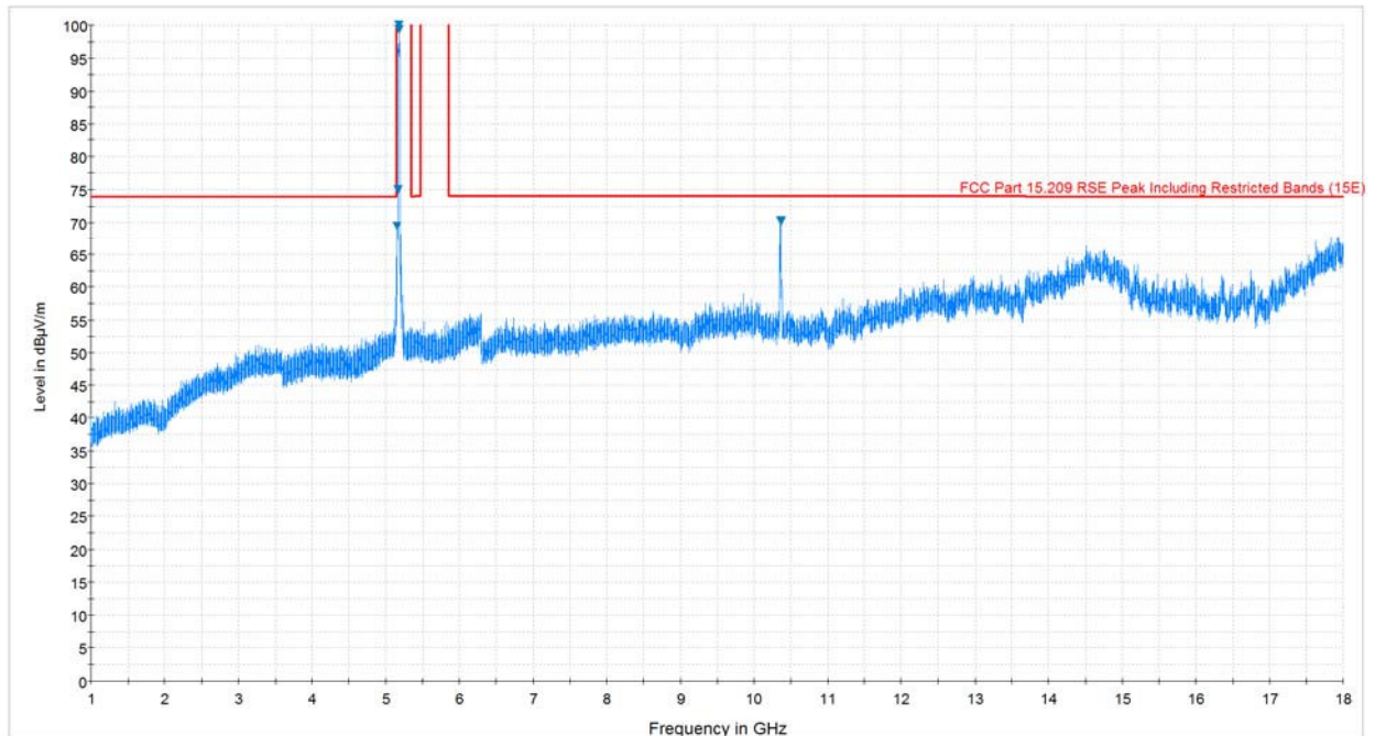
Plot 7-80. Radiated Spurious Plot above 1GHz (802.11a – U1 Ch. 40, Ant. Pol. V)
