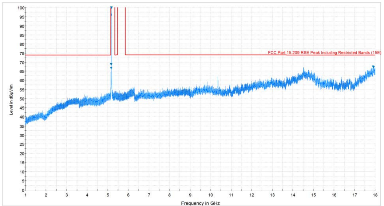
Plot 7-79. Radiated Spurious Plot above 1GHz (802.11a – U1 Ch. 40, Ant. Pol. H)
