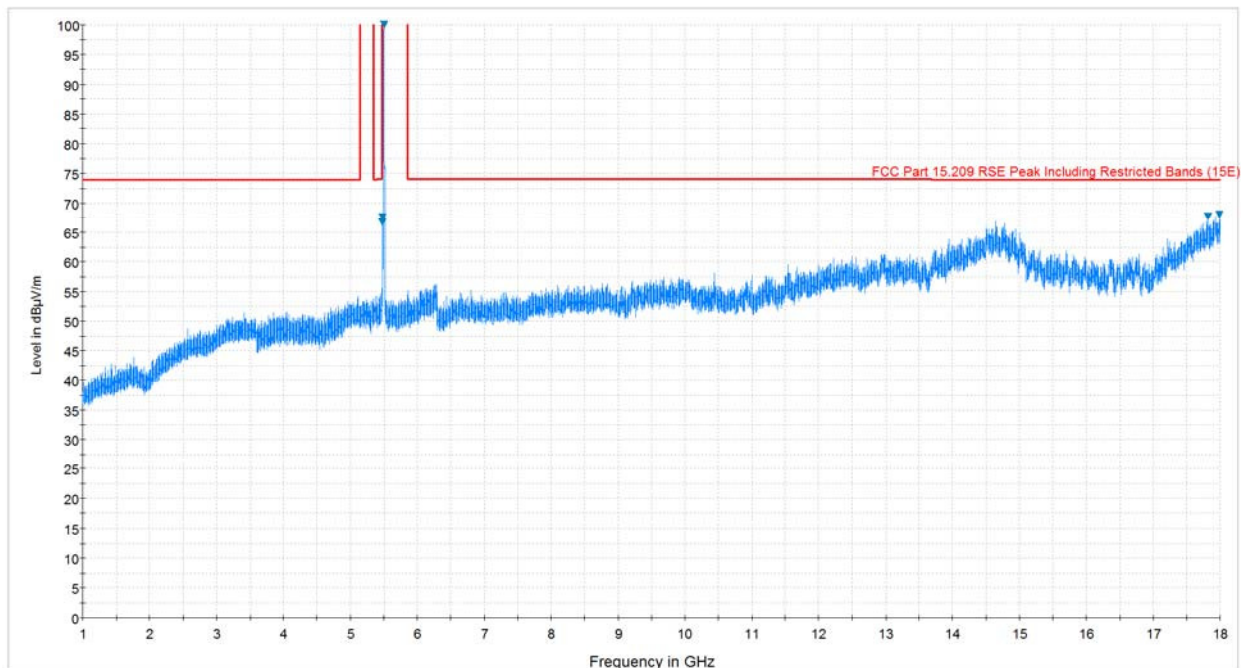
Plot 7-83. Radiated Spurious Plot above 1GHz (802.11a – U2C Ch. 116, Ant. Pol. H)
