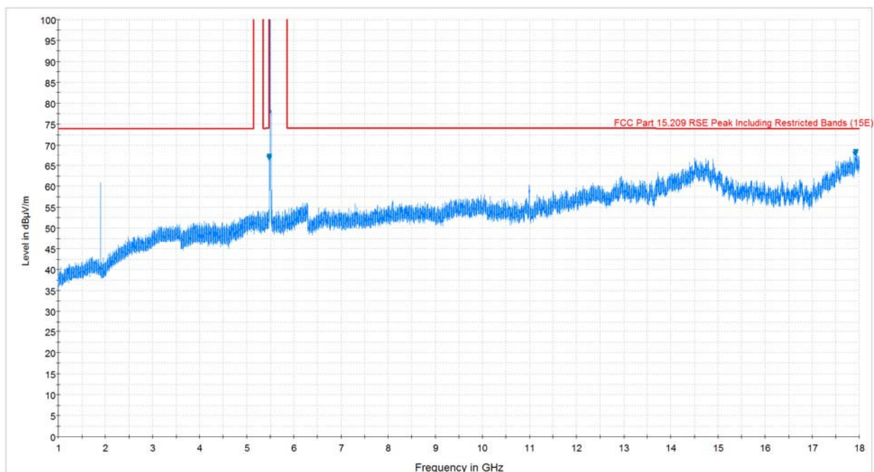
Plot 7-84. Radiated Spurious Plot above 1GHz (802.11a – U2C Ch. 116, Ant. Pol. V)
