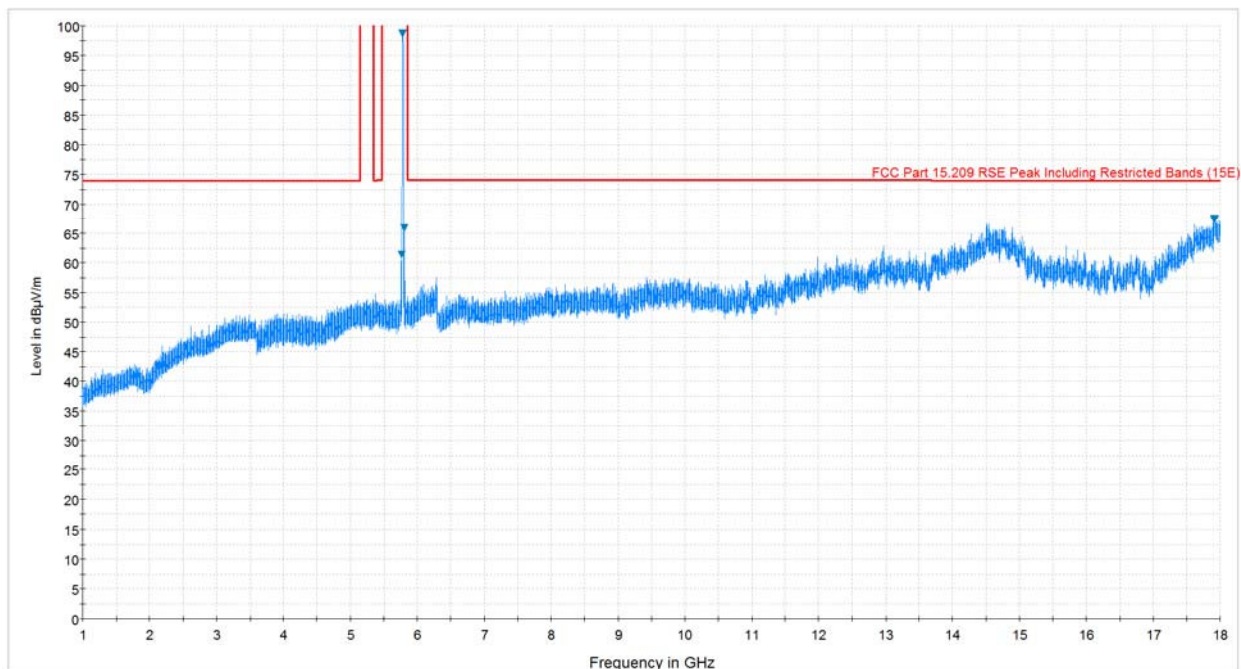
Plot 7-86. Radiated Spurious Plot above 1GHz (802.11a – U3 Ch. 157, Ant. Pol. V)
