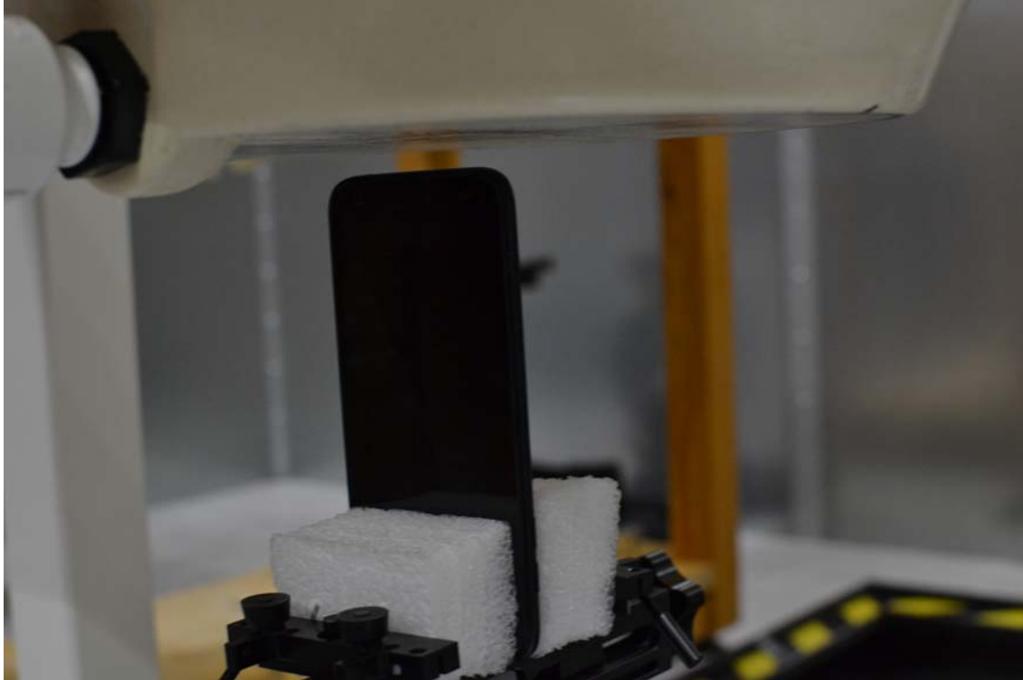
SAR Test Setup Photo 15 – Bottom Edge at 1.3 cm
