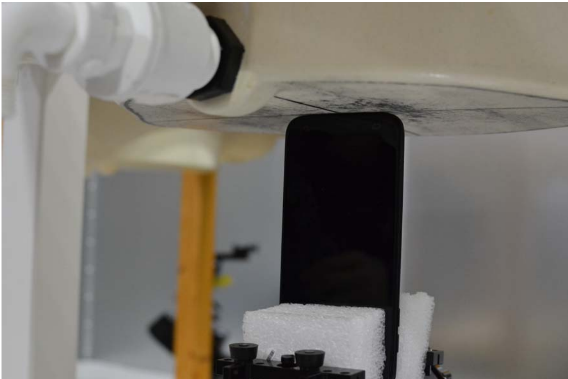
SAR Test Setup Photo 16 – Bottom Edge at 0.0 cm
