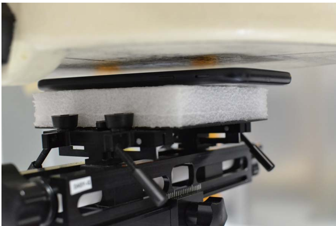
SAR Test Setup Photo 10 – Front Side at 0.7 cm
