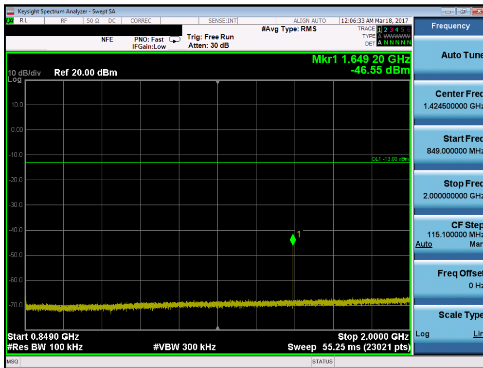
Plot 7-10. Conducted Spurious Plot (Band 5 – 10.0MHz QPSK – RB Size 1, RB Offset 0 – Low Channel)
