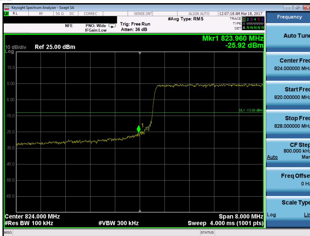
Plot 7-26. Lower Band Edge Plot (Band 5 – 10.0MHz QPSK – RB Size 50)
