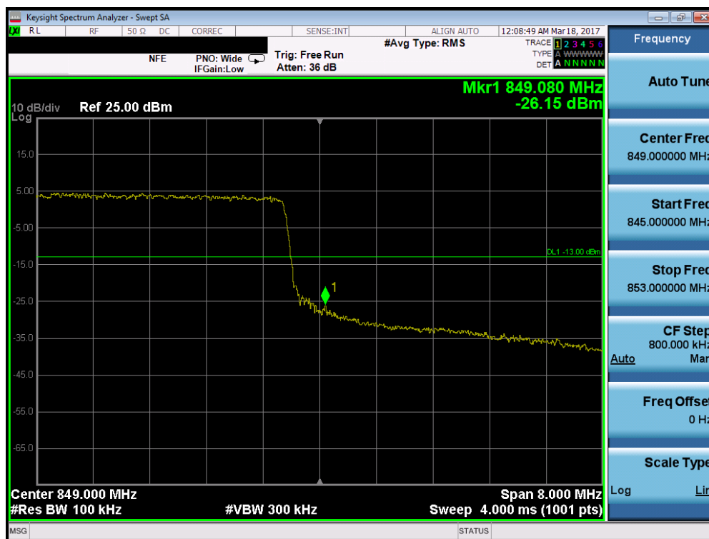
Plot 7-27. Upper Band Edge Plot (Band 5 – 10.0MHz QPSK – RB Size 50)
