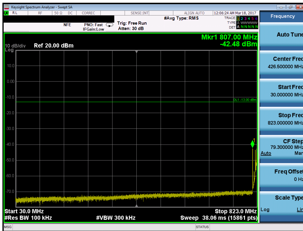
Plot 7-9. Conducted Spurious Plot (Band 5 – 10.0MHz QPSK – RB Size 1, RB Offset 0– Low Channel)
