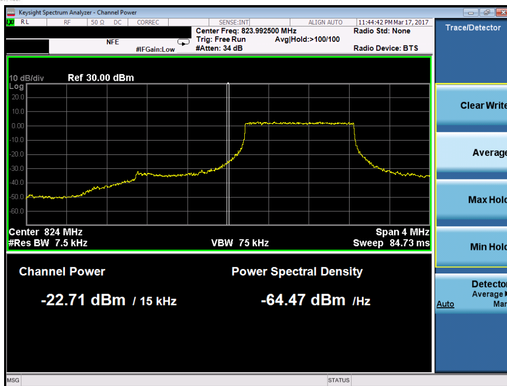
Plot 7-18. Lower Band Edge Plot (Band 5 – 1.4MHz QPSK – RB Size 6)
