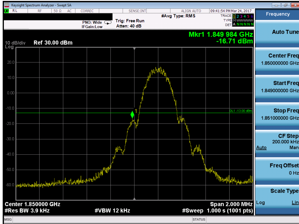
Plot 7-45. Band Edge Plot (PCS GSM Mode – Ch. 512)
