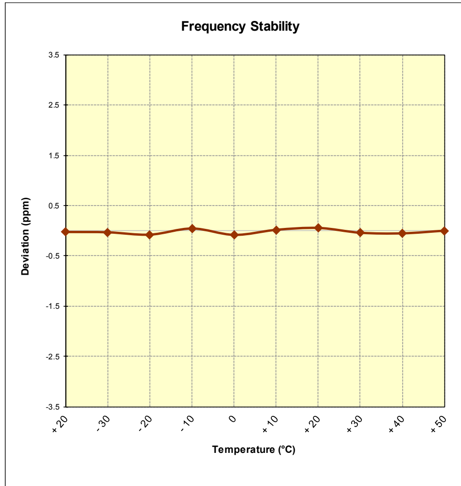
Figure 7-10. Frequency Stability Graph (PCS GSM Mode – Ch. 661)
