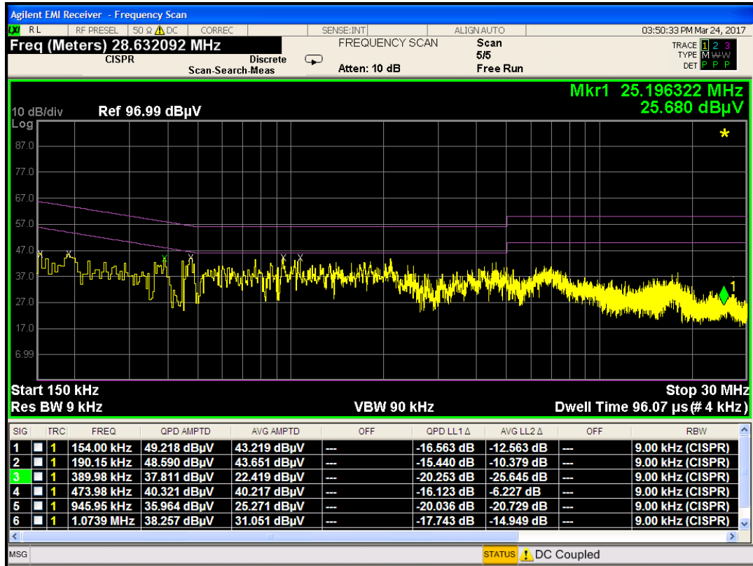
Plot 7-1. Line Conducted Plot (L1)
