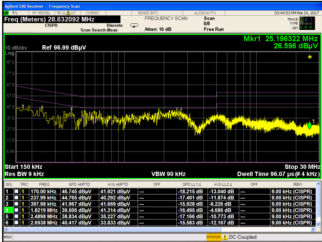
Plot 7-2. Line Conducted Plot (N)
