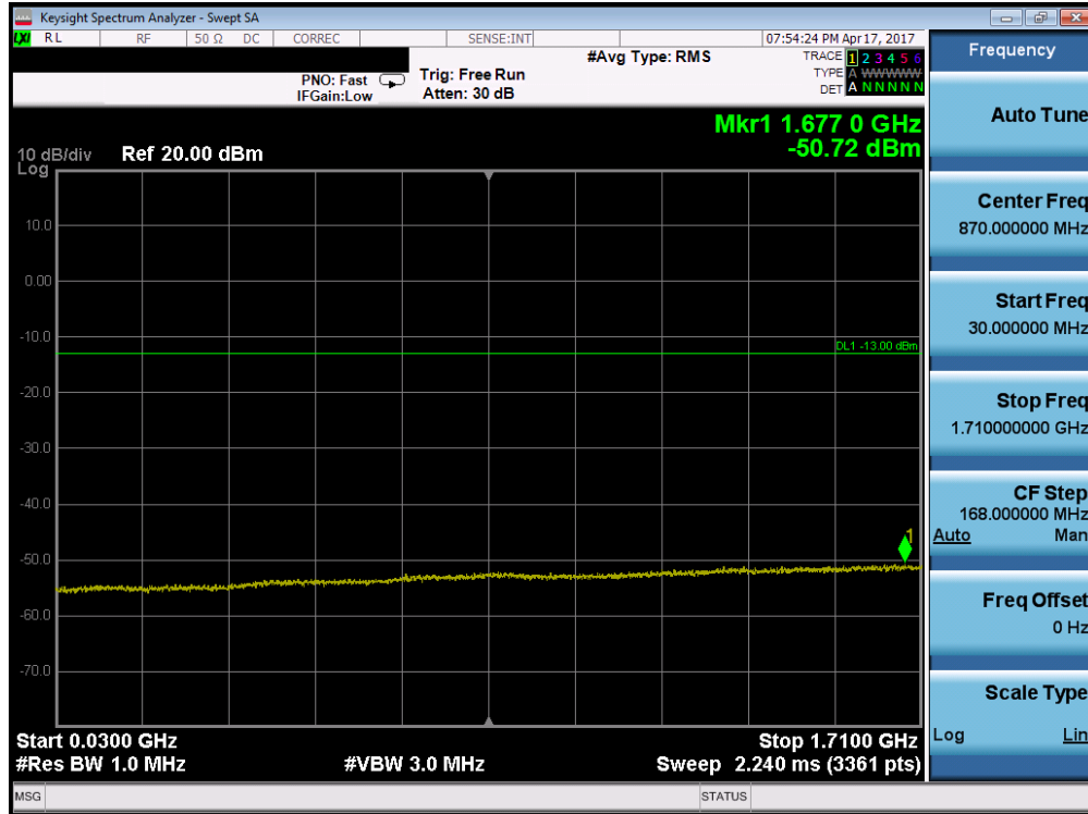
Plot 7-8. Conducted Spurious Plot (AWS WCDMA Mode – Ch. 1513)
