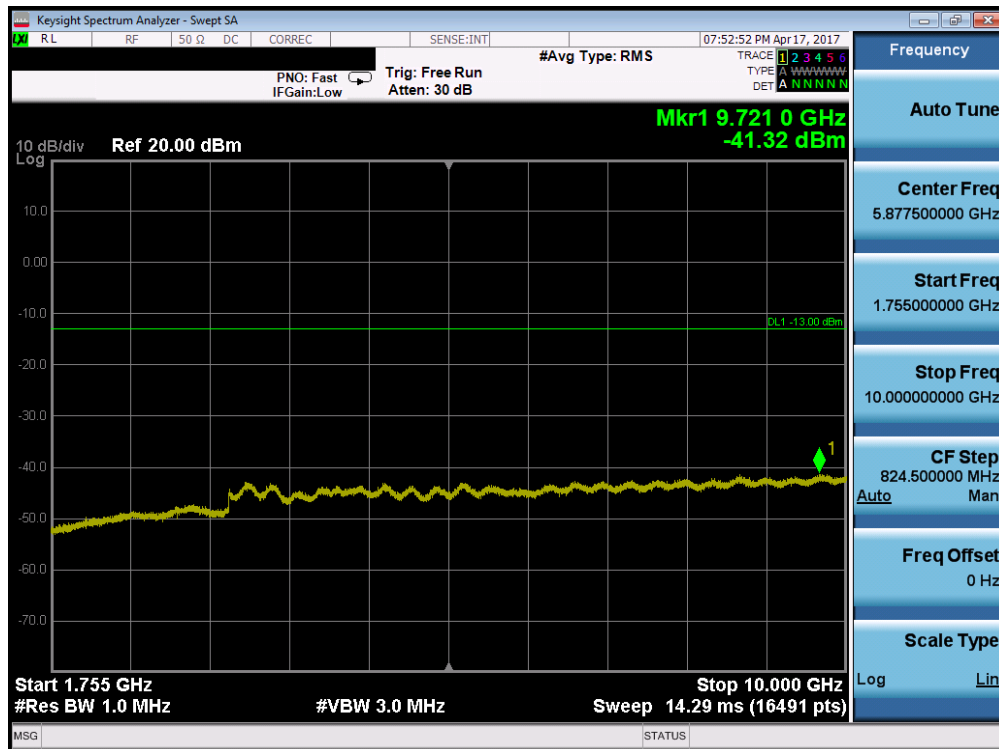
Plot 7-3. Conducted Spurious Plot (AWS WCDMA Mode – Ch. 1312)
