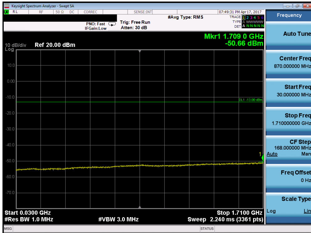
Plot 7-5. Conducted Spurious Plot (AWS WCDMA Mode – Ch. 1413)
