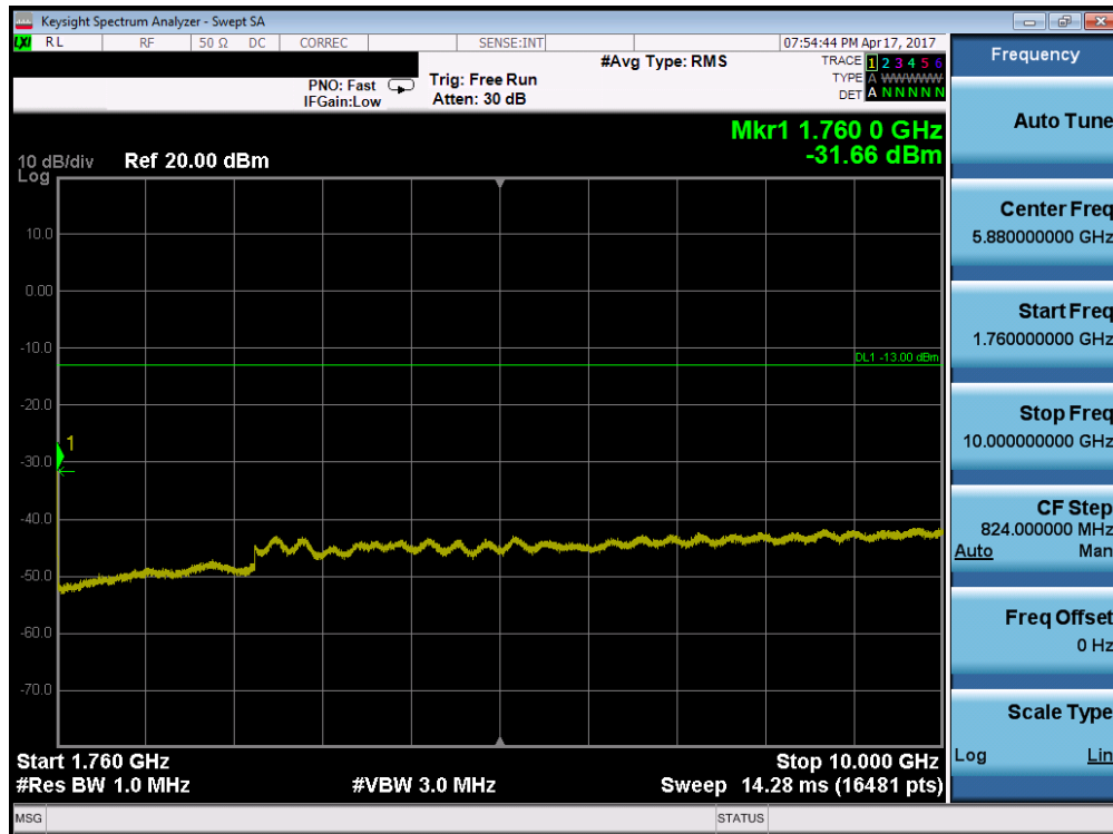
Plot 7-9. Conducted Spurious Plot (AWS WCDMA Mode – Ch. 1513)
