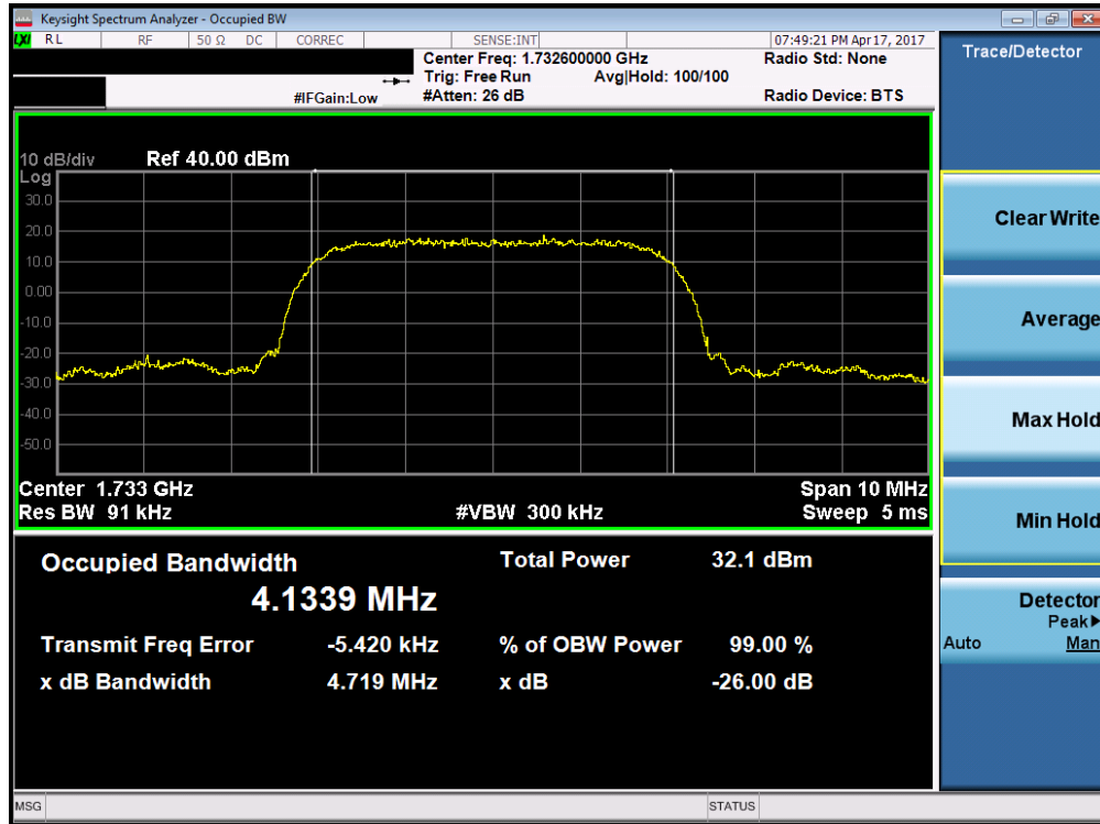
Plot 7-1. Occupied Bandwidth Plot (AWS WCDMA Mode – Ch. 1413)
