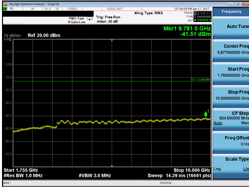
Plot 7-6. Conducted Spurious Plot (AWS WCDMA Mode – Ch. 1413)
