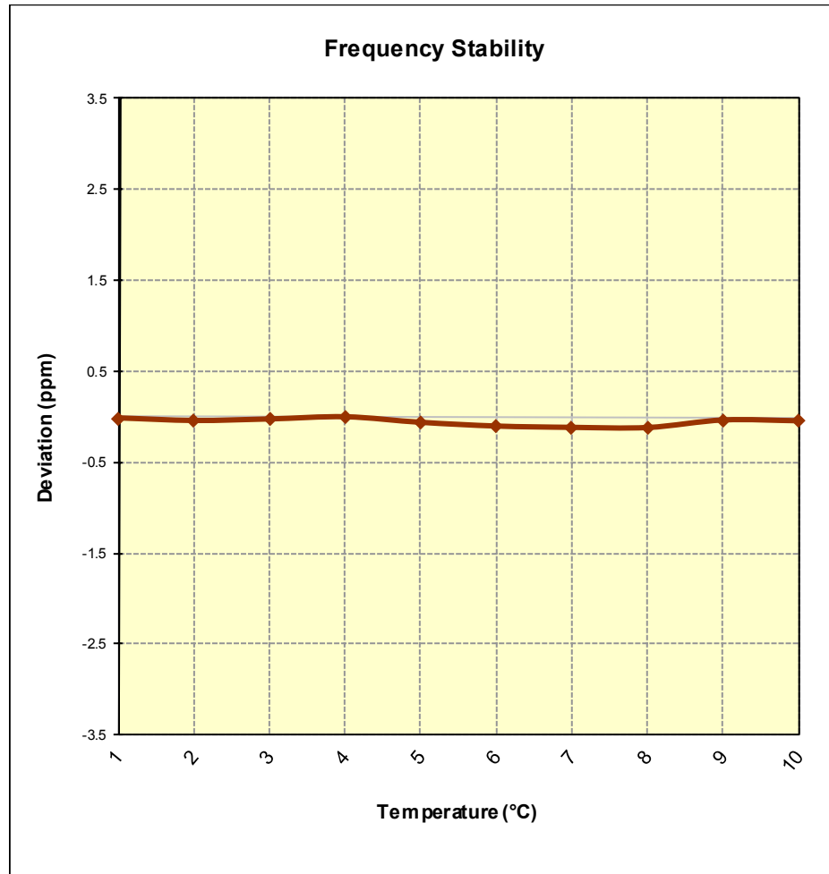
Figure 7-7. Frequency Stability Graph (AWS WCDMA Mode – Ch. 1413)
