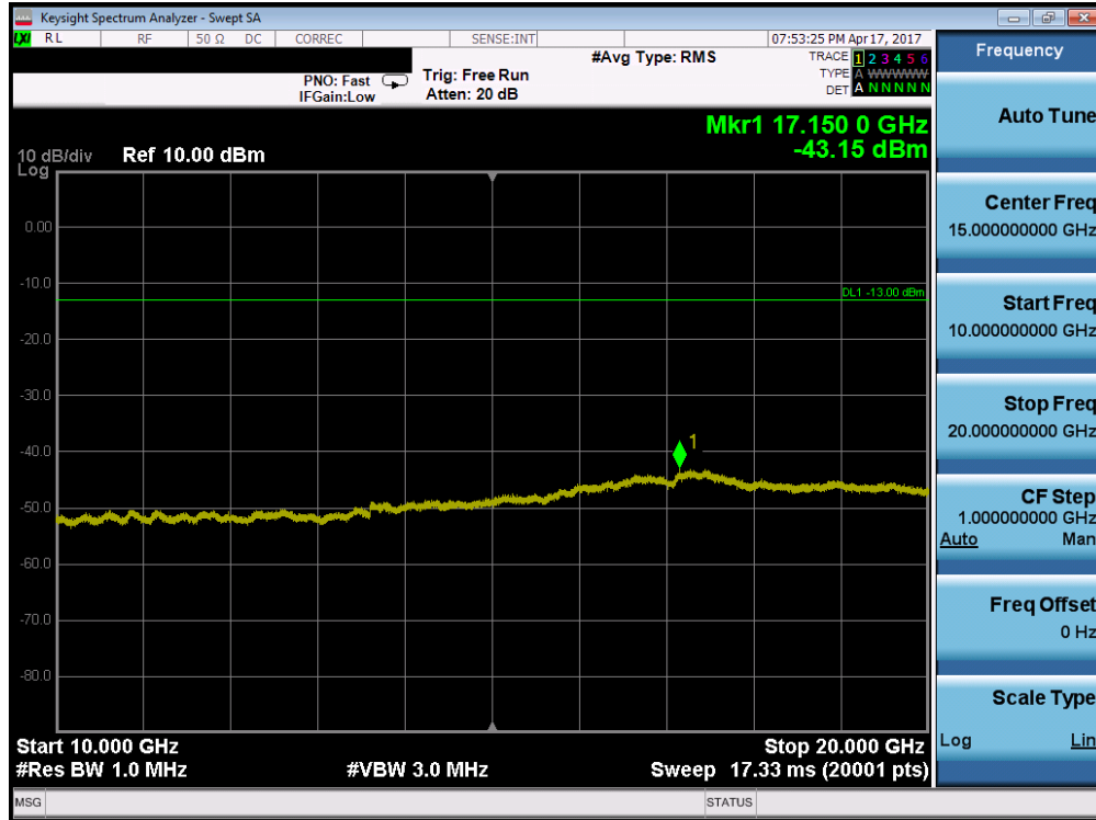
Plot 7-4. Conducted Spurious Plot (AWS WCDMA Mode – Ch. 1312)
