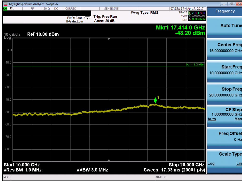
Plot 7-10. Conducted Spurious Plot (AWS WCDMA Mode - Ch. 1513)
