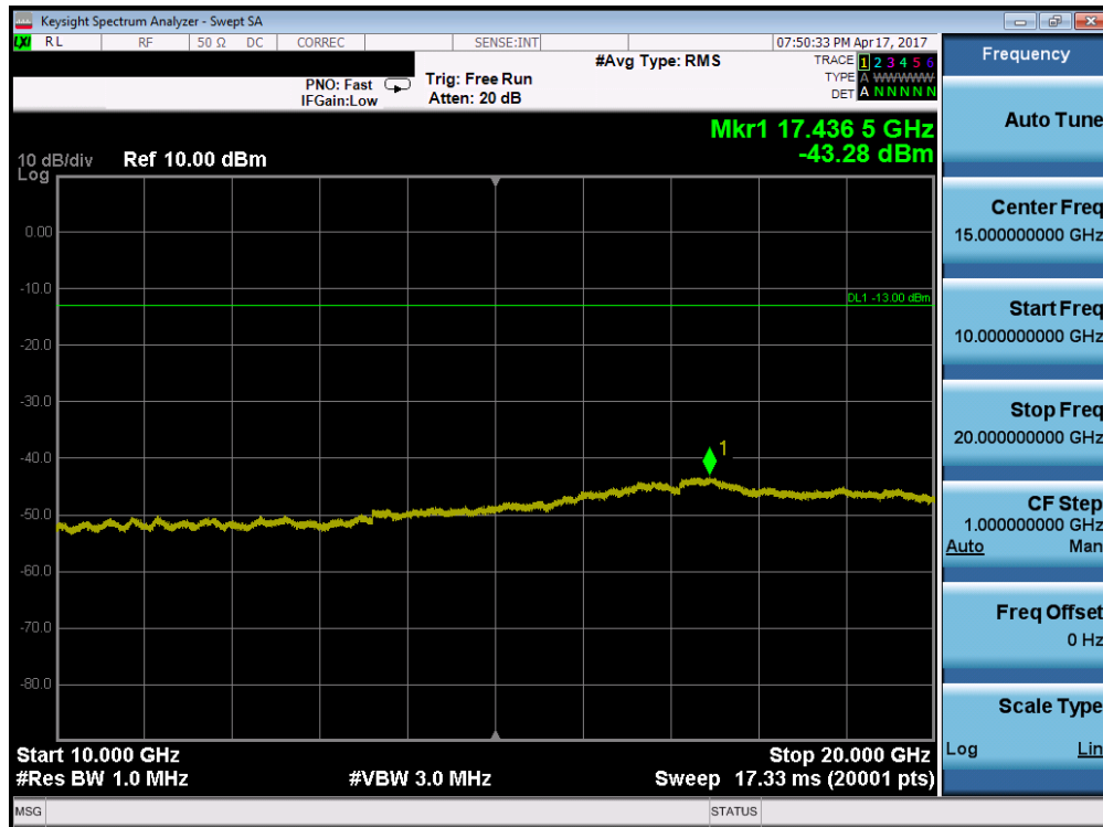
Plot 7-7. Conducted Spurious Plot (AWS WCDMA Mode – Ch. 1413)
