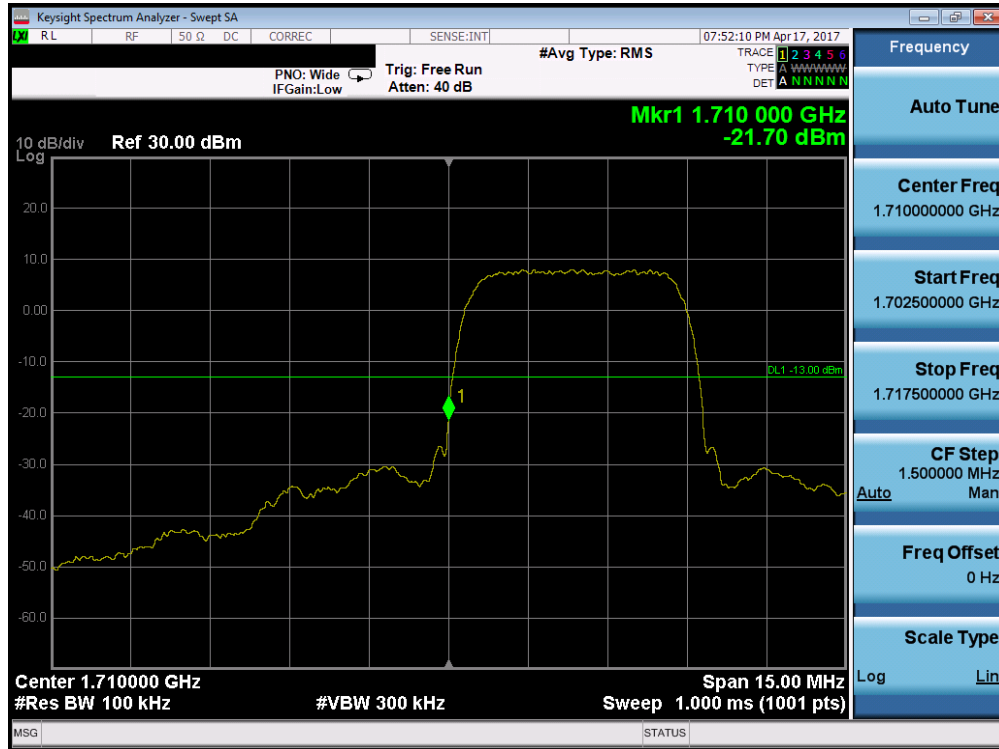
Plot 7-11. Band Edge Plot (AWS WCDMA Mode – Ch. 1312)
