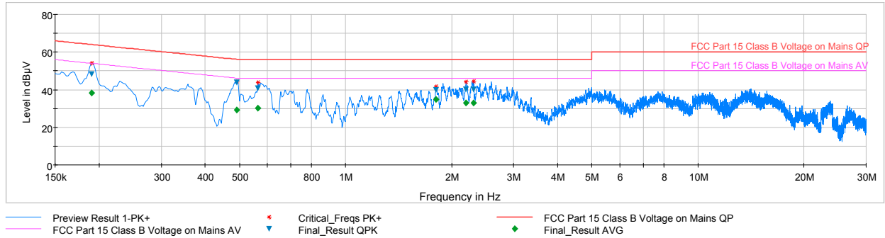
Plot 7-5. Line Conducted Plot (L1)
