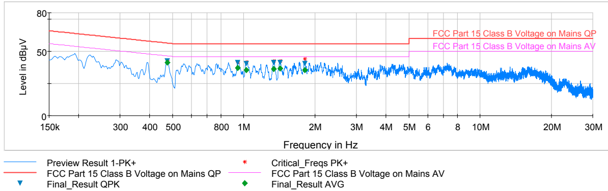
Plot 7-6. Line Conducted Plot (L1)
